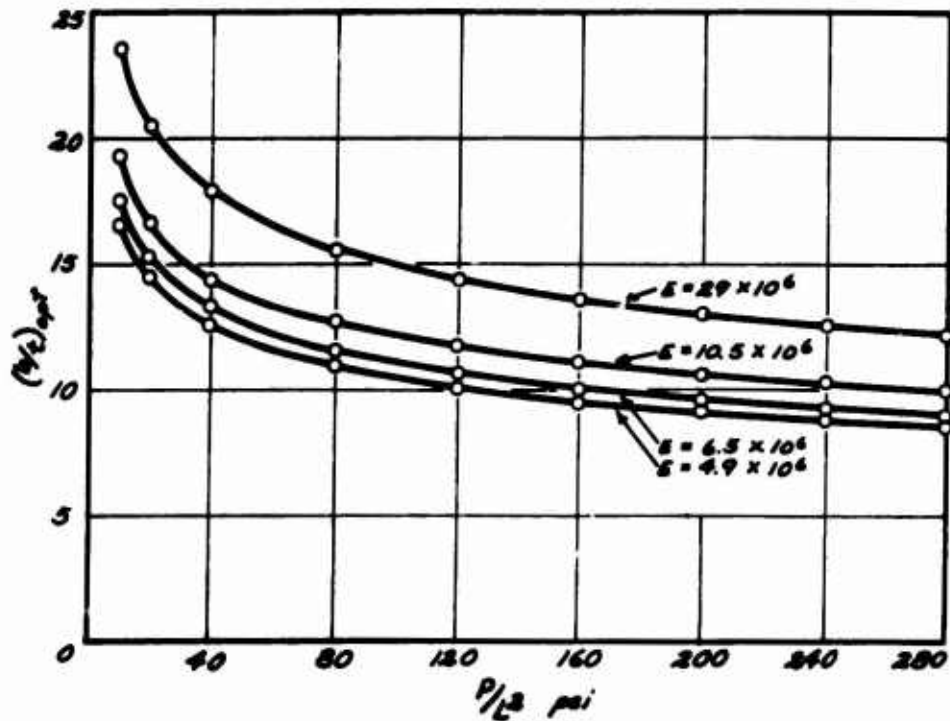
Figure 27a. Optimum Ratio of Applied Load to Column Length Squared Versus Ratio of Semi-Width of Cross Section to Thickness for Rectangular Cross Section Having a Ratio of Semi-Depth of Cross Section to Semi-Width of Cross Section Equal to 0.5.
