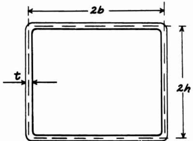
Figure 19b. Rectangular Section.
