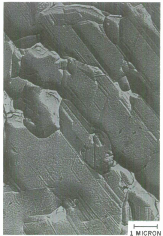
This electron micrograph of the surface of a silicon film grown epitaxially on sapphire has a magnification of 10,000 times. The ridge lines are the boundaries between adjacent silicon crystallites. The dislocation lines and triangles are visible in each crystallite. The silicon film is six microns thick, and it is oriented in the "111" direction.
