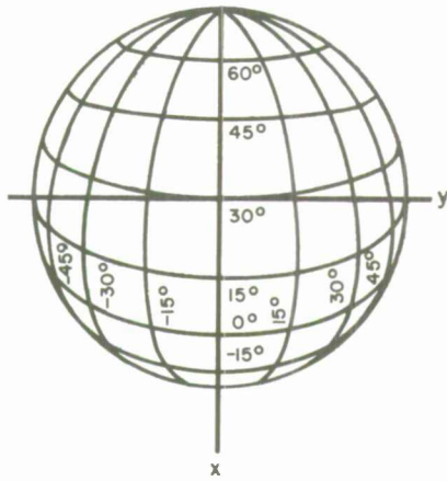
Geometric Projection of the geographic grid with the point of projection in a satellite 4000 milcs above 0° longitude, 30° latitude.
