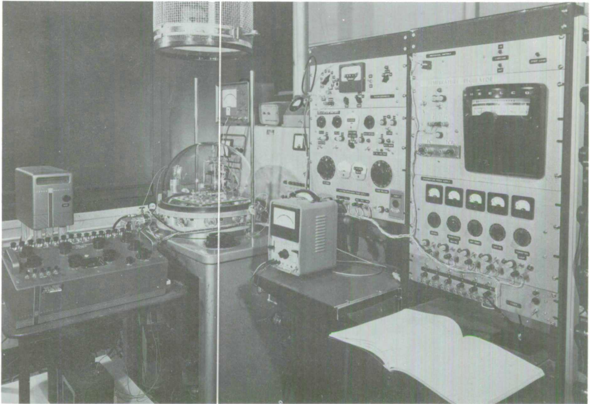
The bell jar vacuum system is used for measuring the system pressure, outgassing some of the interior parts, heating and controlling the temperature of the substrate, heating and evaporating the various source metals, and measuring the resistance of the films during deposition.
