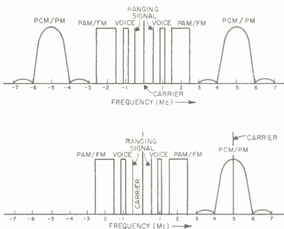
Comparison of single- and double-carrier baseband design for a unified tracking, telemetry, and command system downlink illustrates the reduction in spectrum occupancy for the two-carrier configuration.
