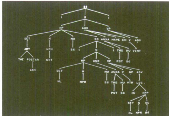
This computer-generated display shows a stage in the development of an automatic linguistic analysis for the sentence, "The general that Johnson met in Washington had traveled 8000 miles."
