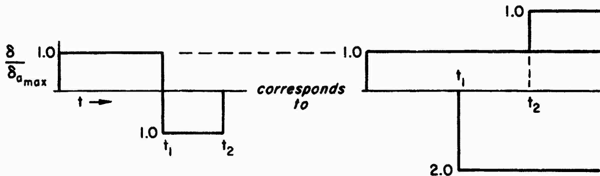
Sketch 3. Maximum-Performance Bank and Stop Aileron Inputs
