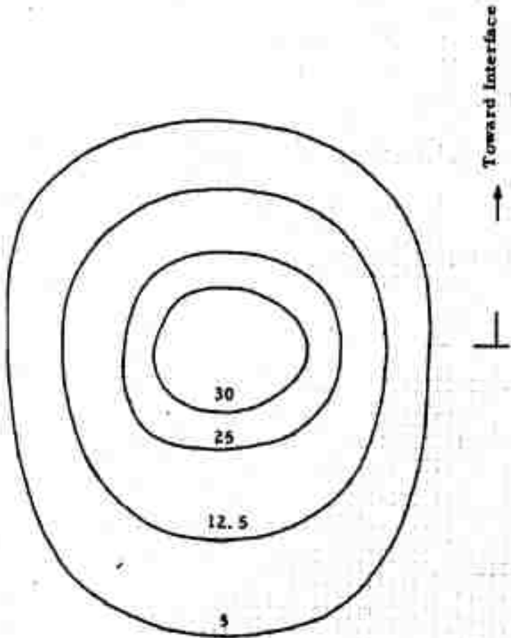
Radiation Field of E_{mcs} with \alpha = 24.5^\circ
