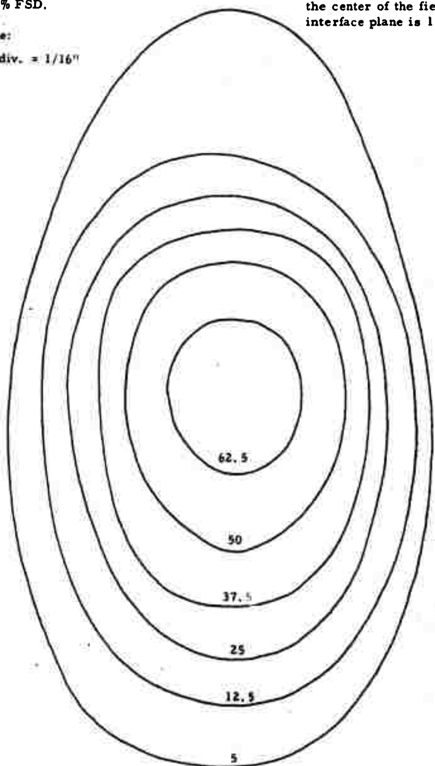
Radiation Field of E_{mer} with \alpha = 23.5\%
