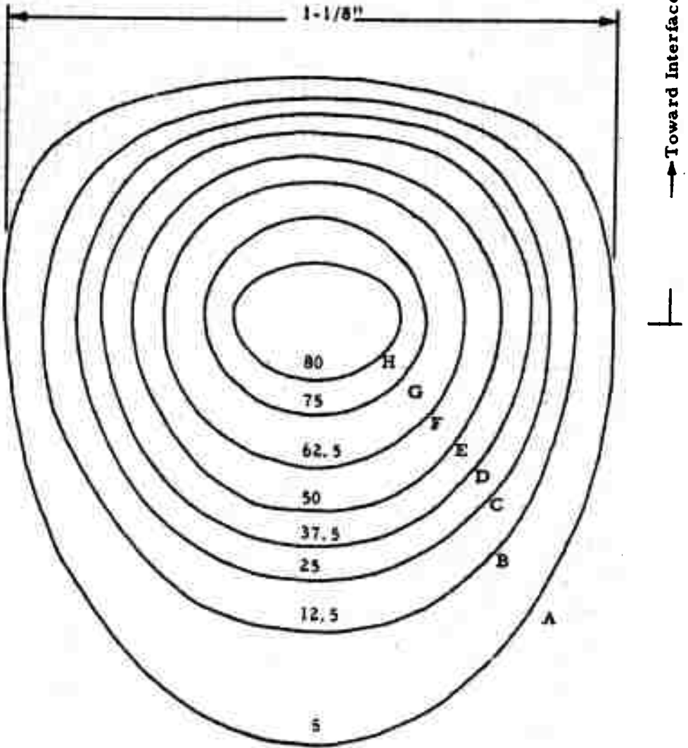
Radiation Field for E_{mcr} with \alpha = 23^\circ
