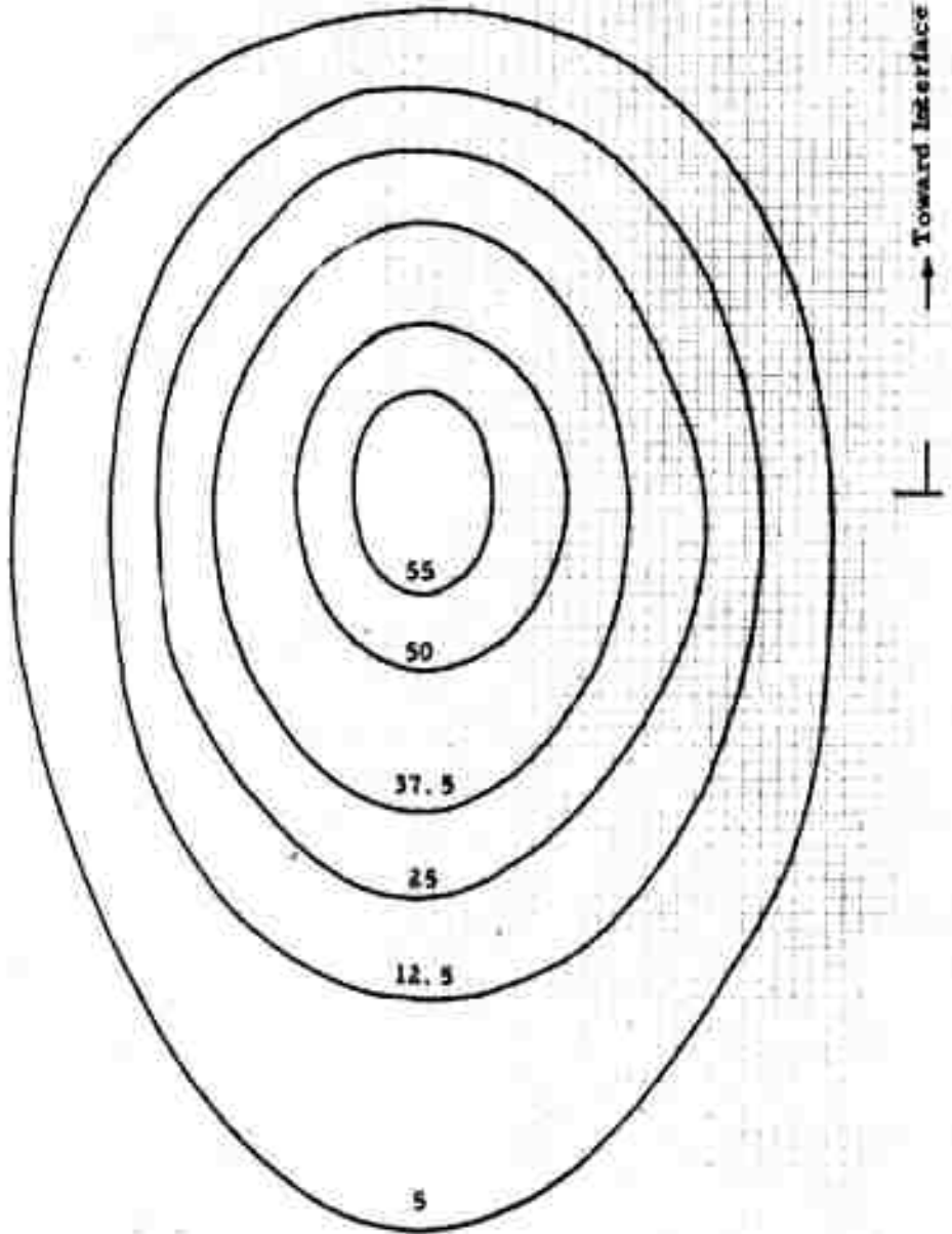
Radiation Field of E_{mcr} with \alpha = 24.5^\circ
