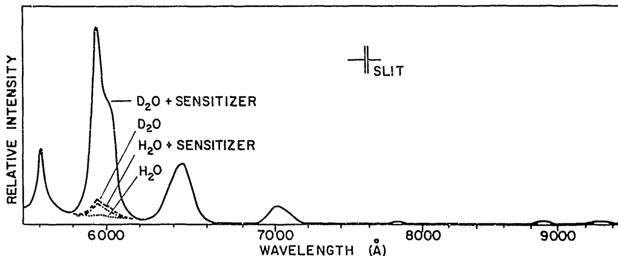
Fig. 2. Emission spectrum of 0.1 M \text{SmCl}_3 in \text{D}_2\text{O} sensitized by 0.1 M dipotassium 1,5-dibenzoylnaphthalene disulfonate. The relative intensities of the non-sensitized \text{D}_2\text{O} , sensitized \text{H}_2\text{O} and non-sensitized \text{H}_2\text{O} solutions are indicated for the strongest emission line.
