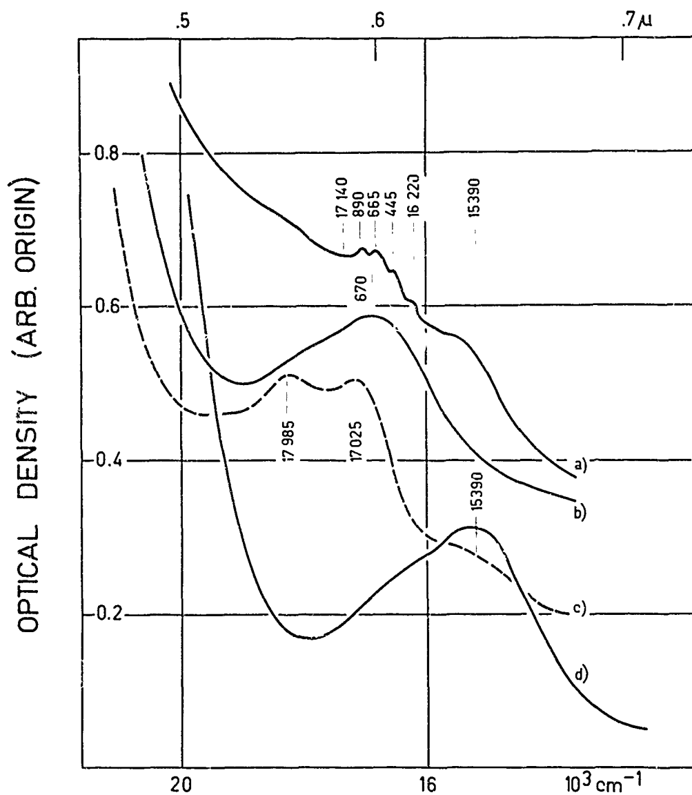
Fig.5. Detail of the absorption in the red region of the spectrum for various Yb 3+ tricyclopentadienides. a) Sublimed Yb cp 3 at 78°K. b) Sublimed Yb cp 3 ·nNH 3 at room temperature. c) Same, at 78°K. d) Yb cp 3 ·THF in THF solution, room temp.
