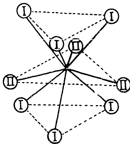
Fig. 3. Arrangement of Halide Ions in nine-coordinate \text{LnX}_3 Structures. (The distances \text{M-X}_I and \text{M-X}_{II} are shown as equal for clarity.)
