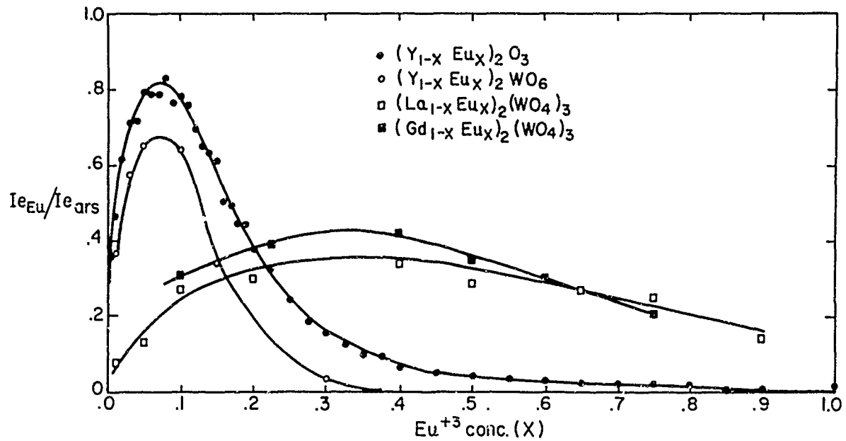
Fig. 1 FLUORESCENCE EMISSION INTENSITY AS A FUNCTION OF Eu^{+3} CONCENTRATION. RELATIVE TO MAGNESIUM ARSENATE: Mn. EXCITATION: 2537A U.V. T = 25°C.
