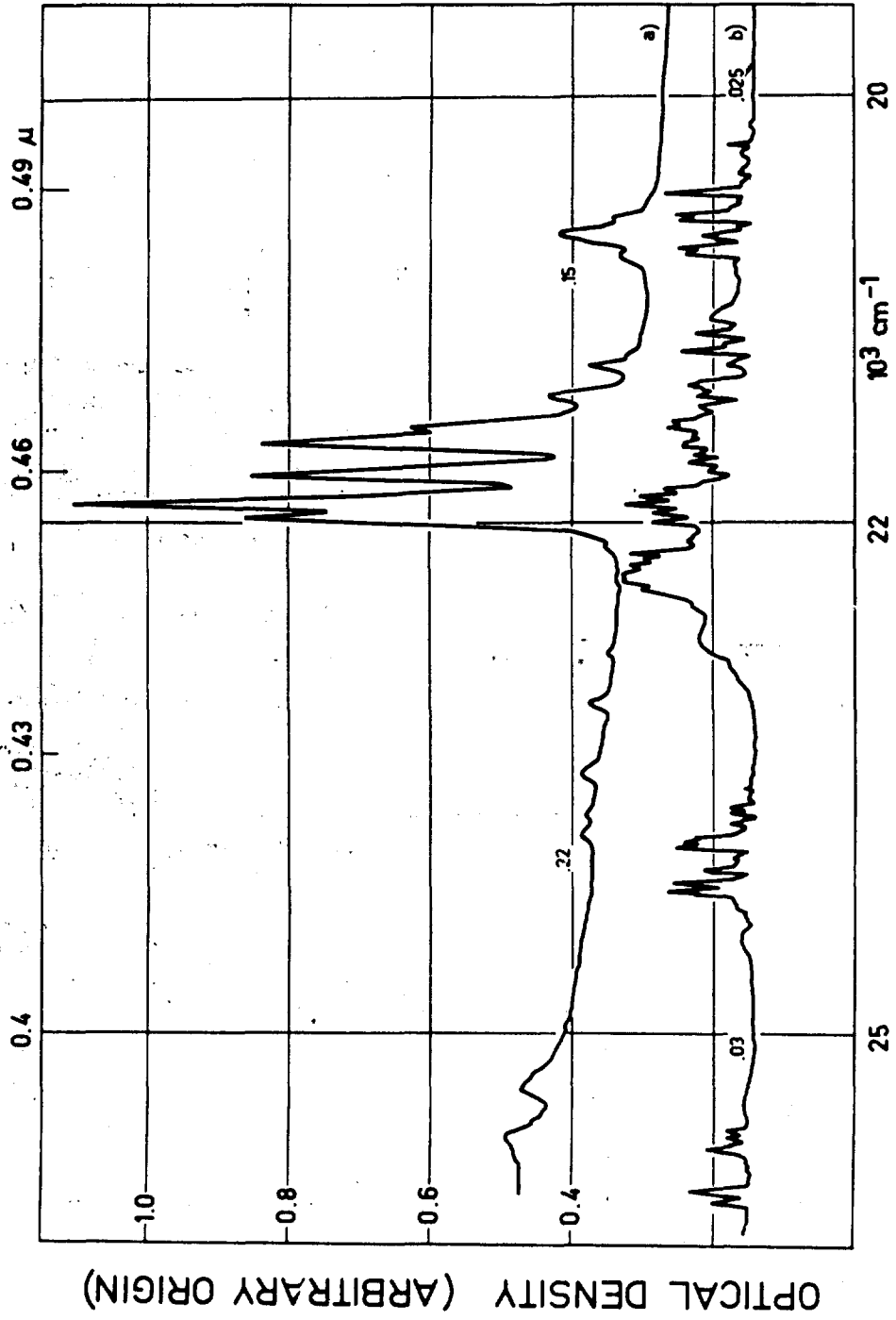
Fig.1. (Top). Diffuse transmission at 78° K. of sublimed Ho ep 3 . (Bottom). For comparison, reflection spectrum of Ho 2 O 3 at 78° K.
