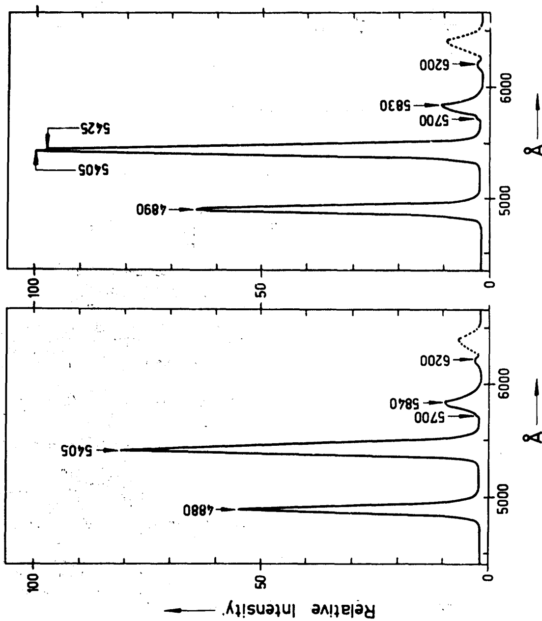
Fig. 2. Fluorescence spectra of \text{Tb}(\text{Dip})_2(\text{NO}_3)_3 and \text{Tb}(\text{Dimp})_2(\text{NO}_3)_3 . The dotted portion shows the second order contribution of the excitation radiation.
