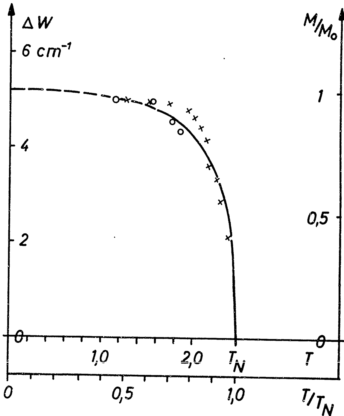
Fig.5: Magnetization curve of DyAlG \circ = {}^6H_{15/2} \rightarrow {}^6F_{5/2} \times = {}^6H_{15/2} \rightarrow {}^6F_{3/2} ; the straight line is the square root of the neutron intensity.
