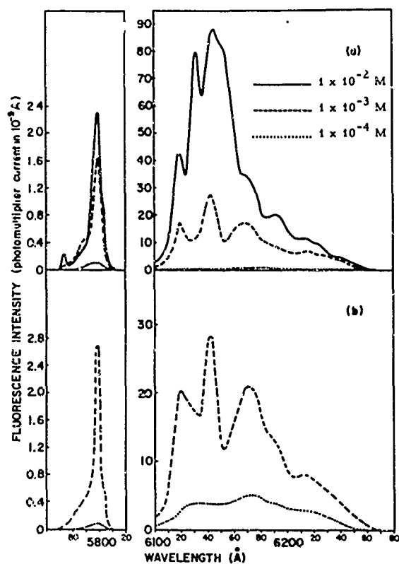
Fig. 7. Benzoylacetate chelates of Eu in EPA solvent at -180^{\circ}\text{C} : (a) tetrakis compound, (b) tris compound.
