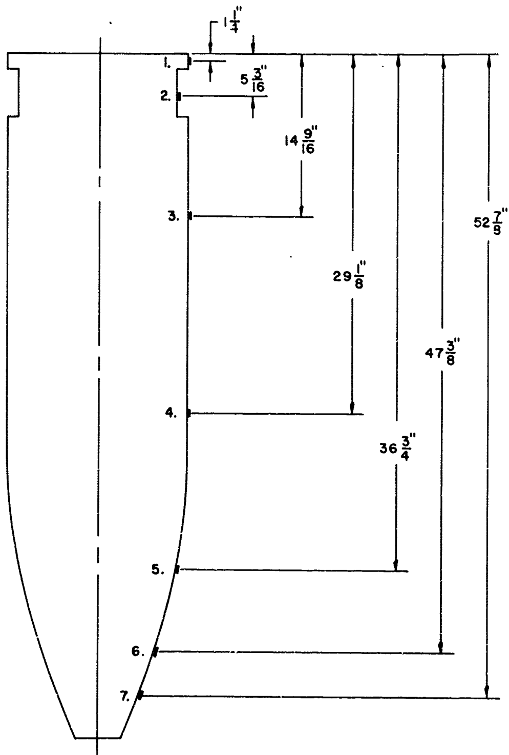
Figure 43. Location of 90° SR-4 strain gage rosettes on Mk-I pressure vessel during proof testing.
