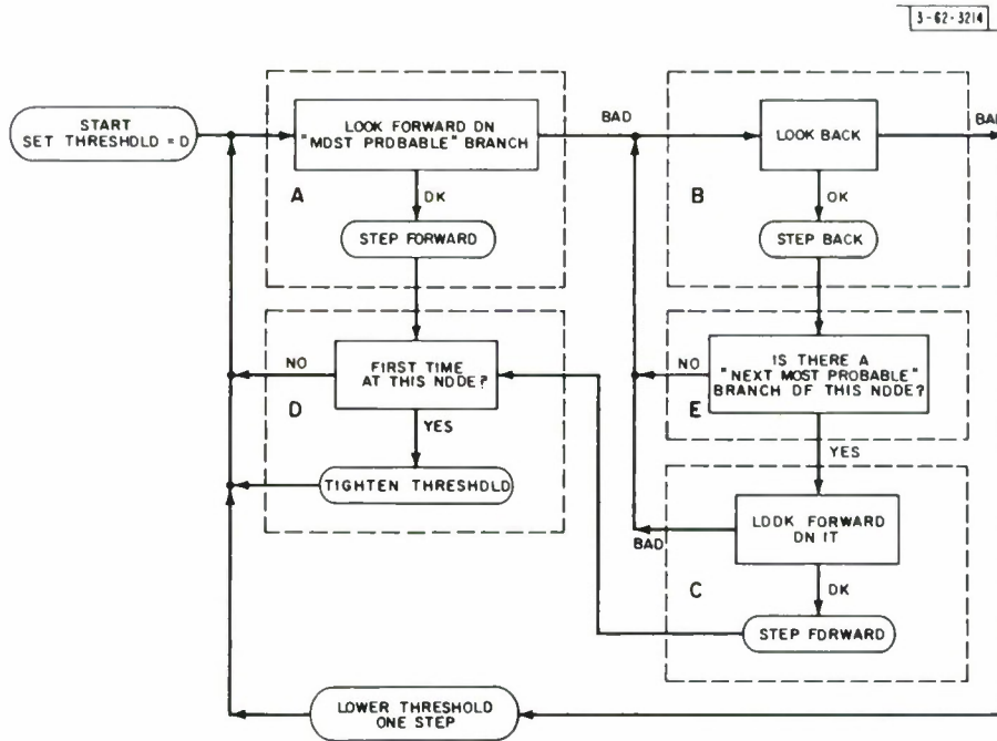
Fig. 4. Flow chart of Fano algorithm.
