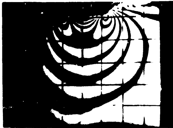
ISOCHROMATICS 2 1/2" WIDE PLATE WITH ROUNDED EDGES (a)
