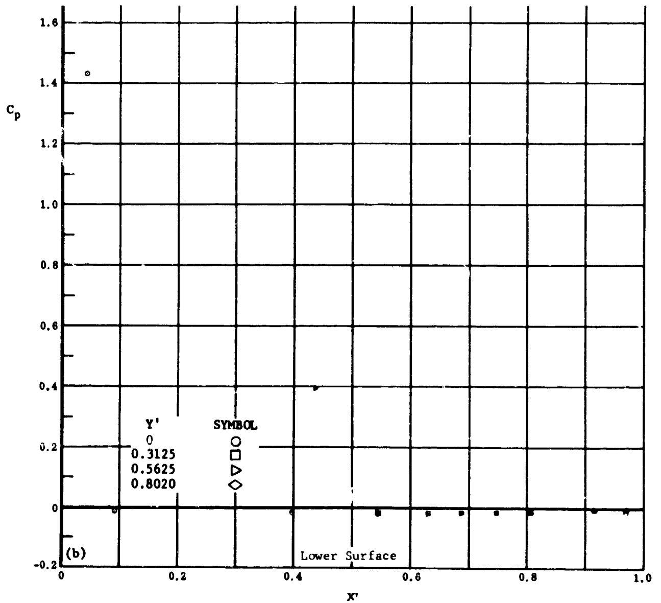
Fig. 21 Configuration I, \alpha = -25 , \delta_2 = \delta_3 = 0
