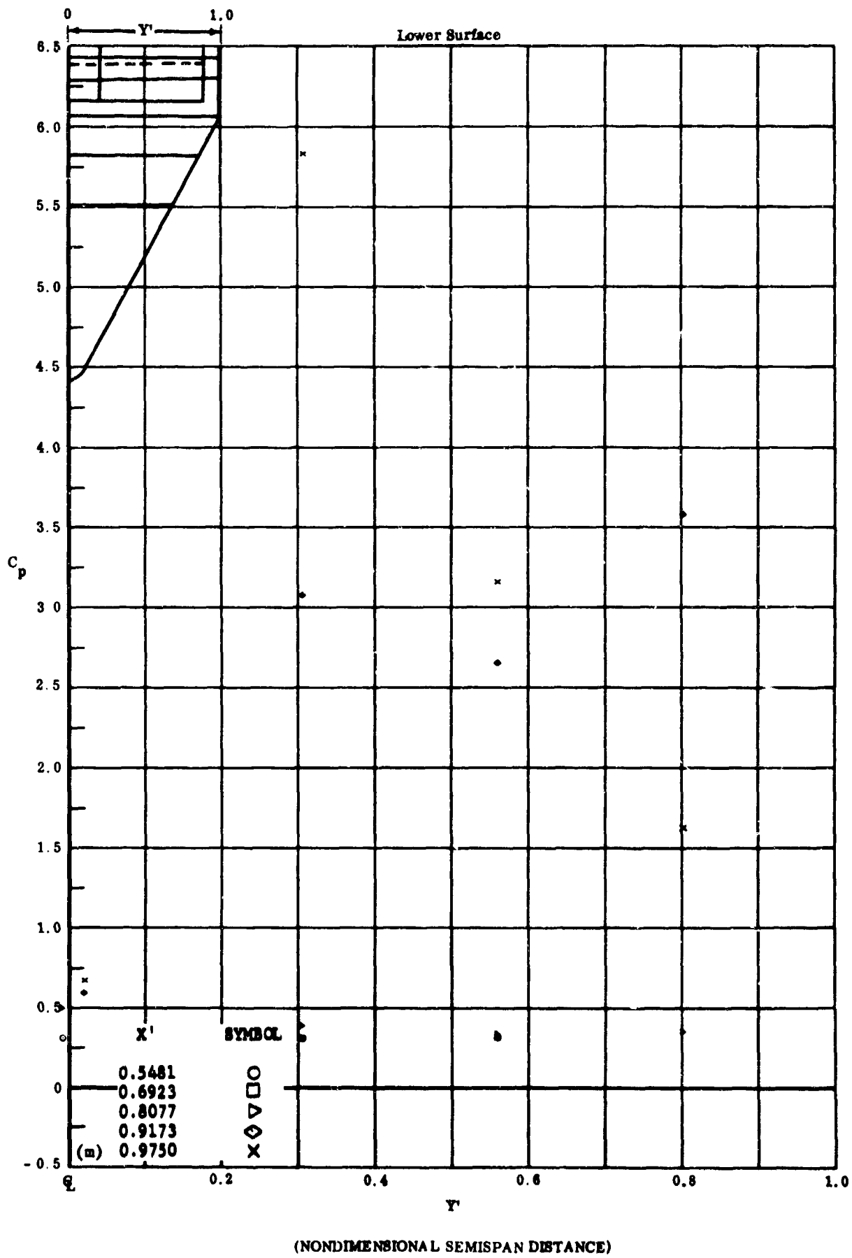
Fig. 7m Configuration X, \alpha = +20 , \delta_2 = \delta_3 = +30
