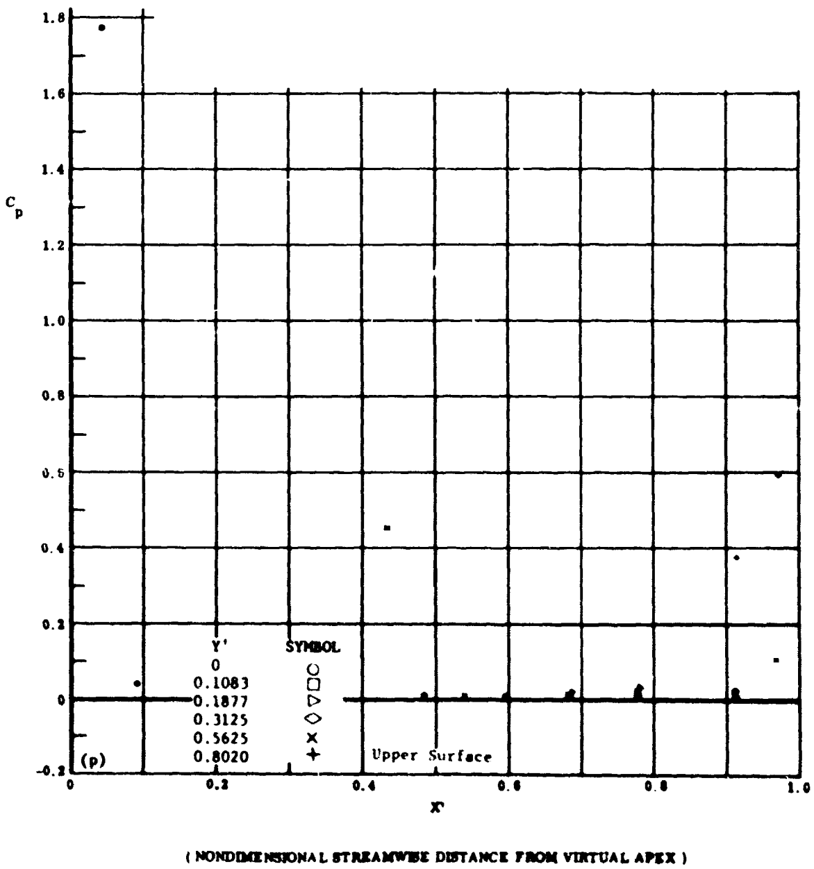
Fig. 32 Configuration IV, \alpha = +10 , \delta_2 = \delta_3 = -39 o) C_p vs. Y' , upper surface p) C_p vs. X' , upper surface
