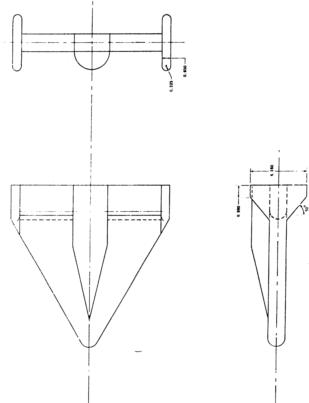
Fig. 1c Configuration IV - Basic Wing-Body + Tip Fins (for dimensions see Figure 1b)
