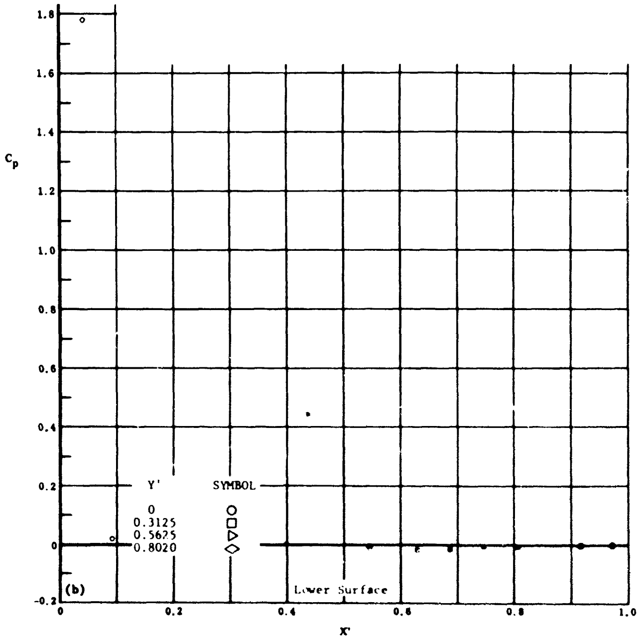
Fig. 17 Configuration I, \alpha = -10^\circ , b_2 = b_3 = -10
