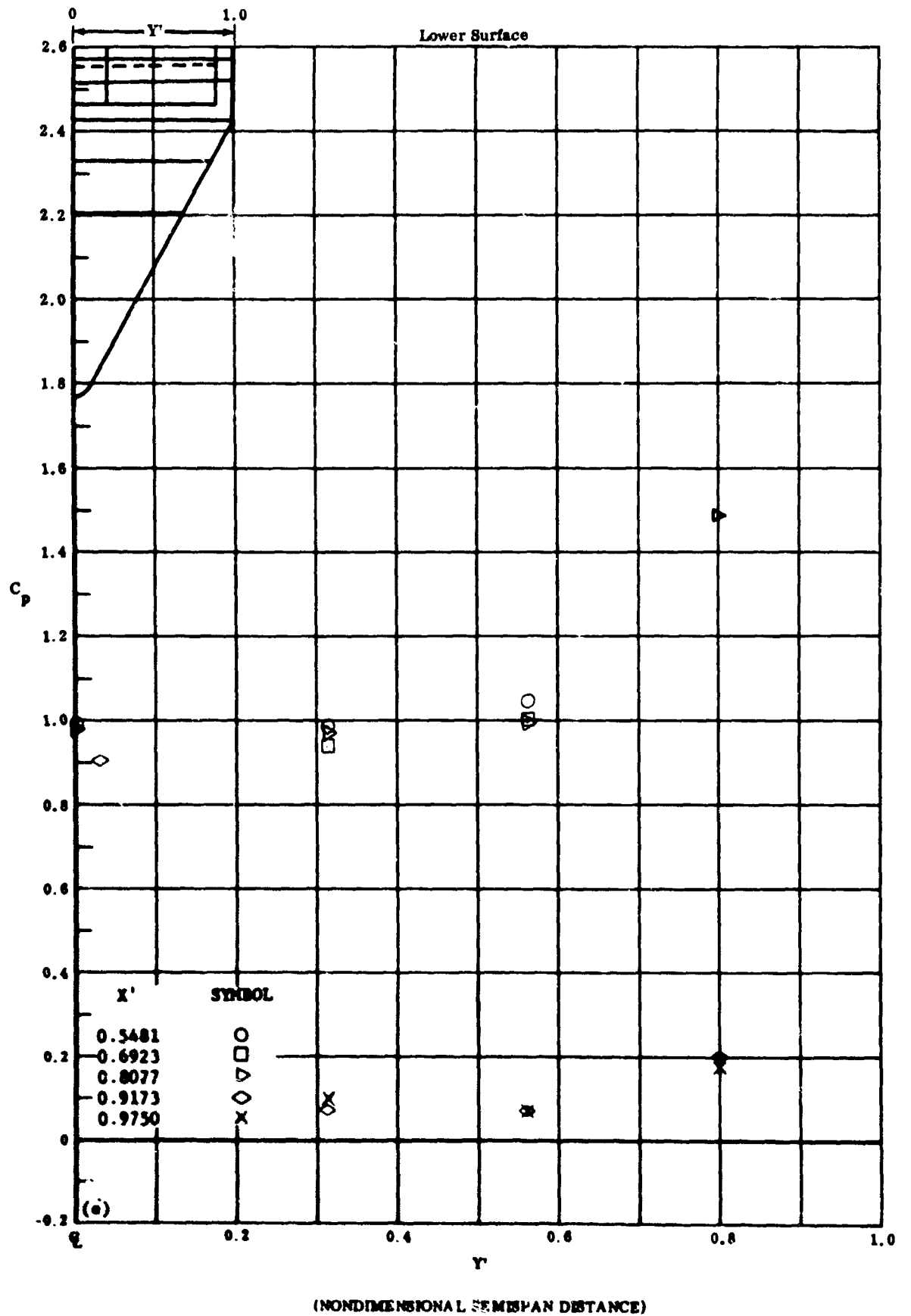
Fig. 38e Configuration IV, \alpha = +40 , \delta_2 = \delta_3 = -39
