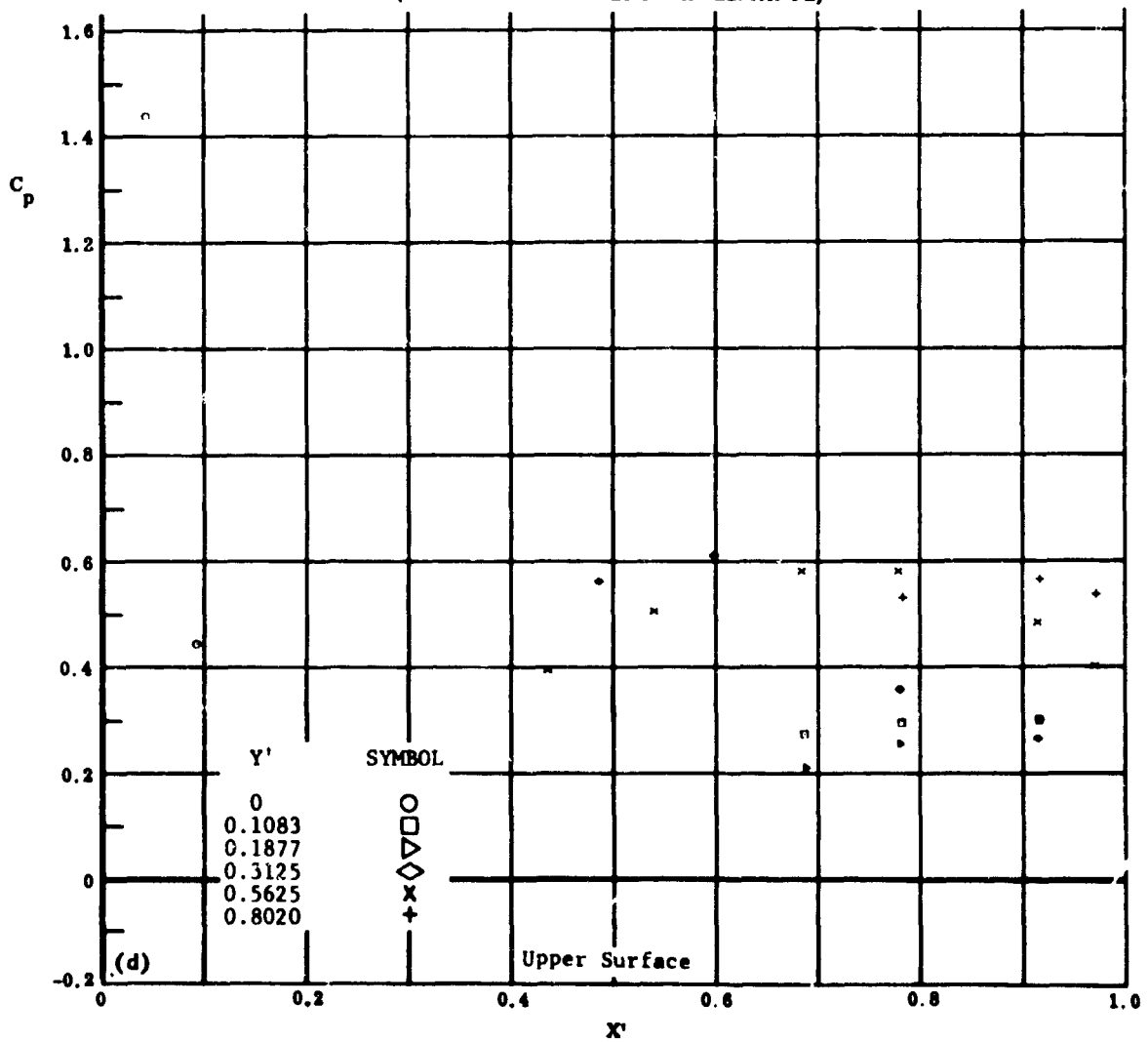
Fig. 21 Configuration I, \alpha = -25 , \delta_2 = \delta_3 = 0
