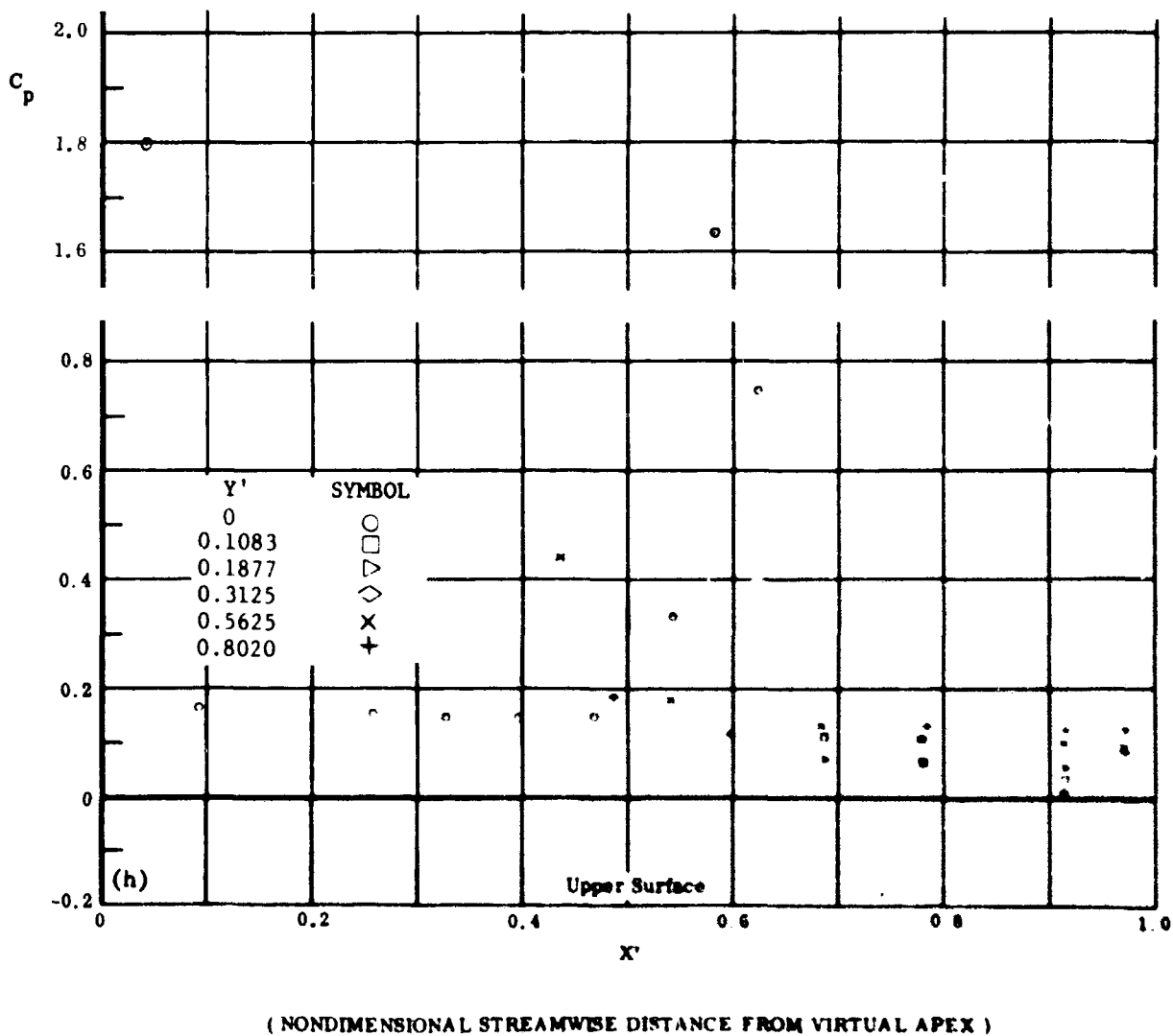
Fig. 50 Configuration VII, Spoiler On
