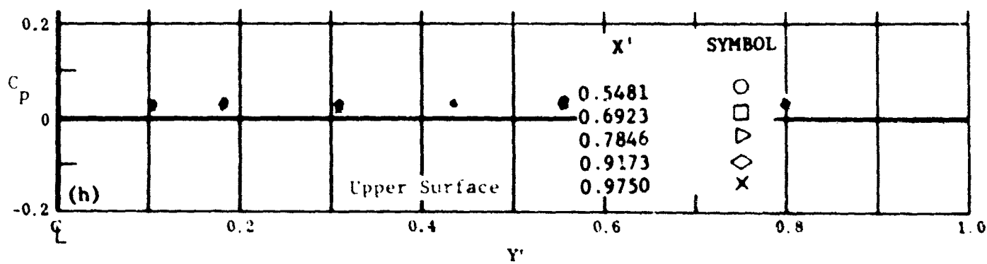
Fig. 9 Configuration I, \alpha = +30 , \xi_2 = \xi_3 = +10
