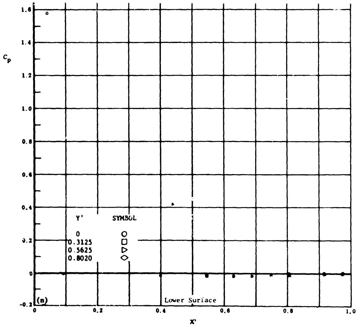
FIG. 11 Configuration IV, \alpha = -20 , \epsilon_2 = \epsilon_3 = -39
