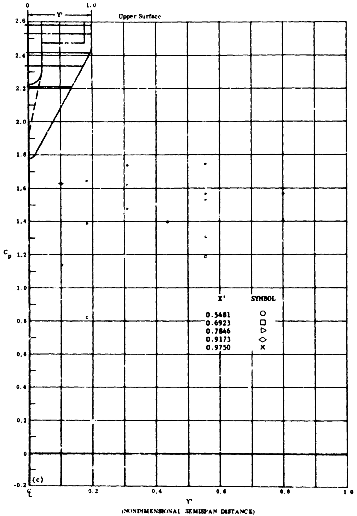
Fig. 28c Configuration I, \alpha = -50^\circ , \beta_2 = \beta_3 = -10^\circ
