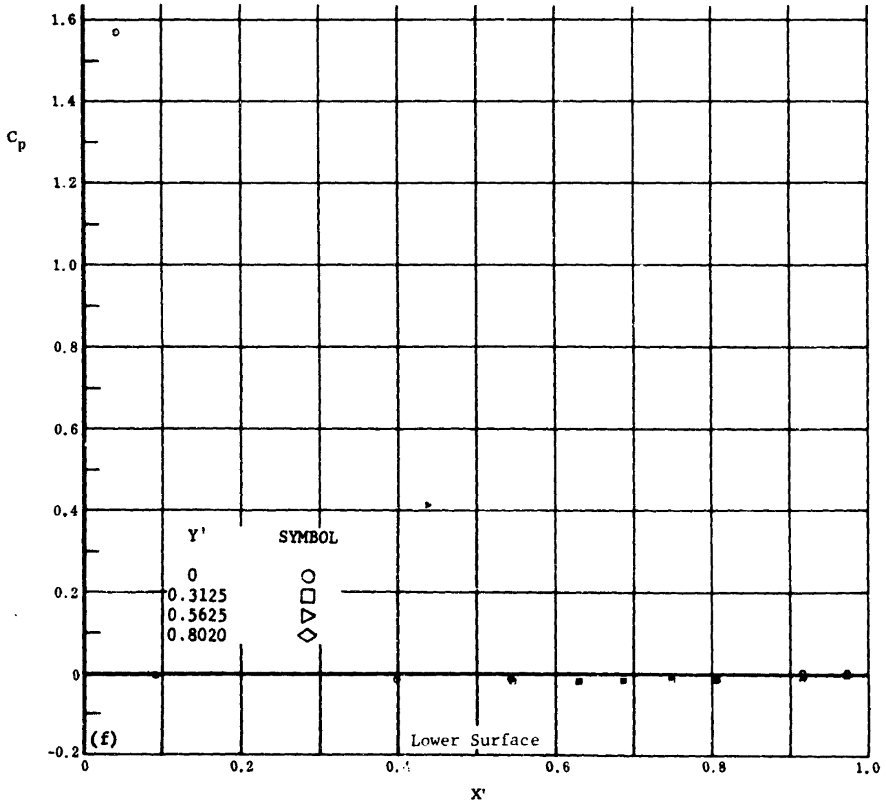
Fig. 43 Configuration IV, \alpha = -20 , b_2 = \delta_3 = -20
