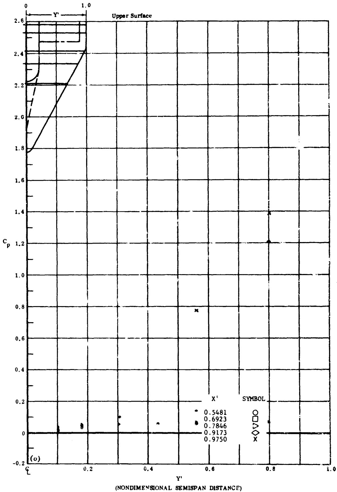
Fig. 30 Configuration IV, \alpha = 0 , \delta_2 = \delta_3 = -39
