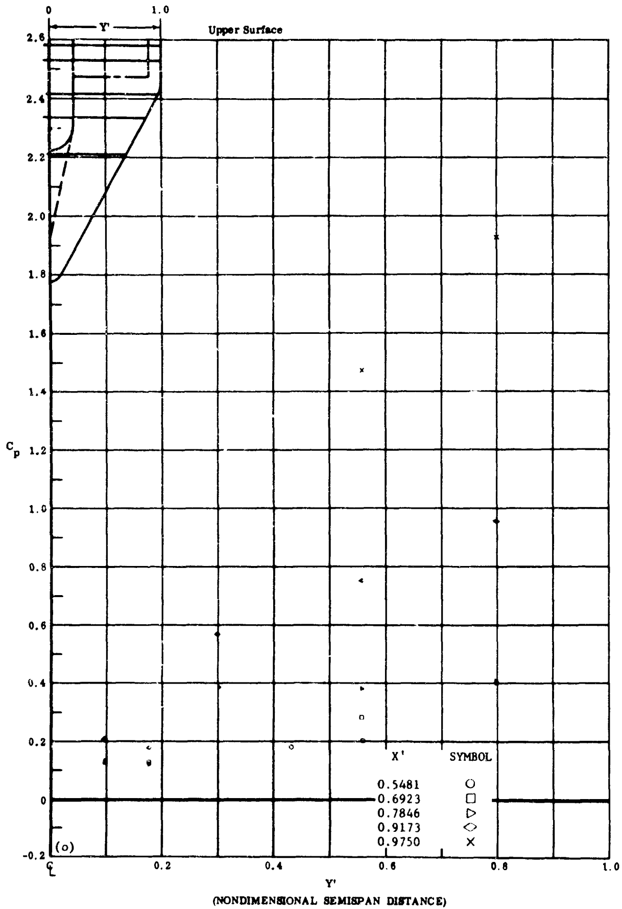
Fig. 17o Configuration I, \alpha = -10 , b_2 = b_3 = -39
