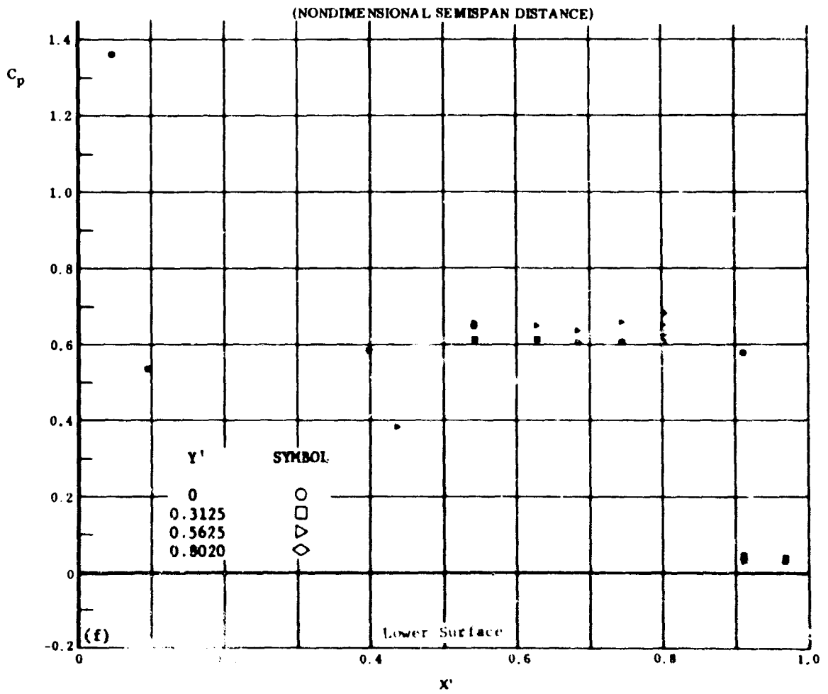
Fig. 10 Configuration I, \alpha = +30 , \beta_2 = \beta_3 = -39
