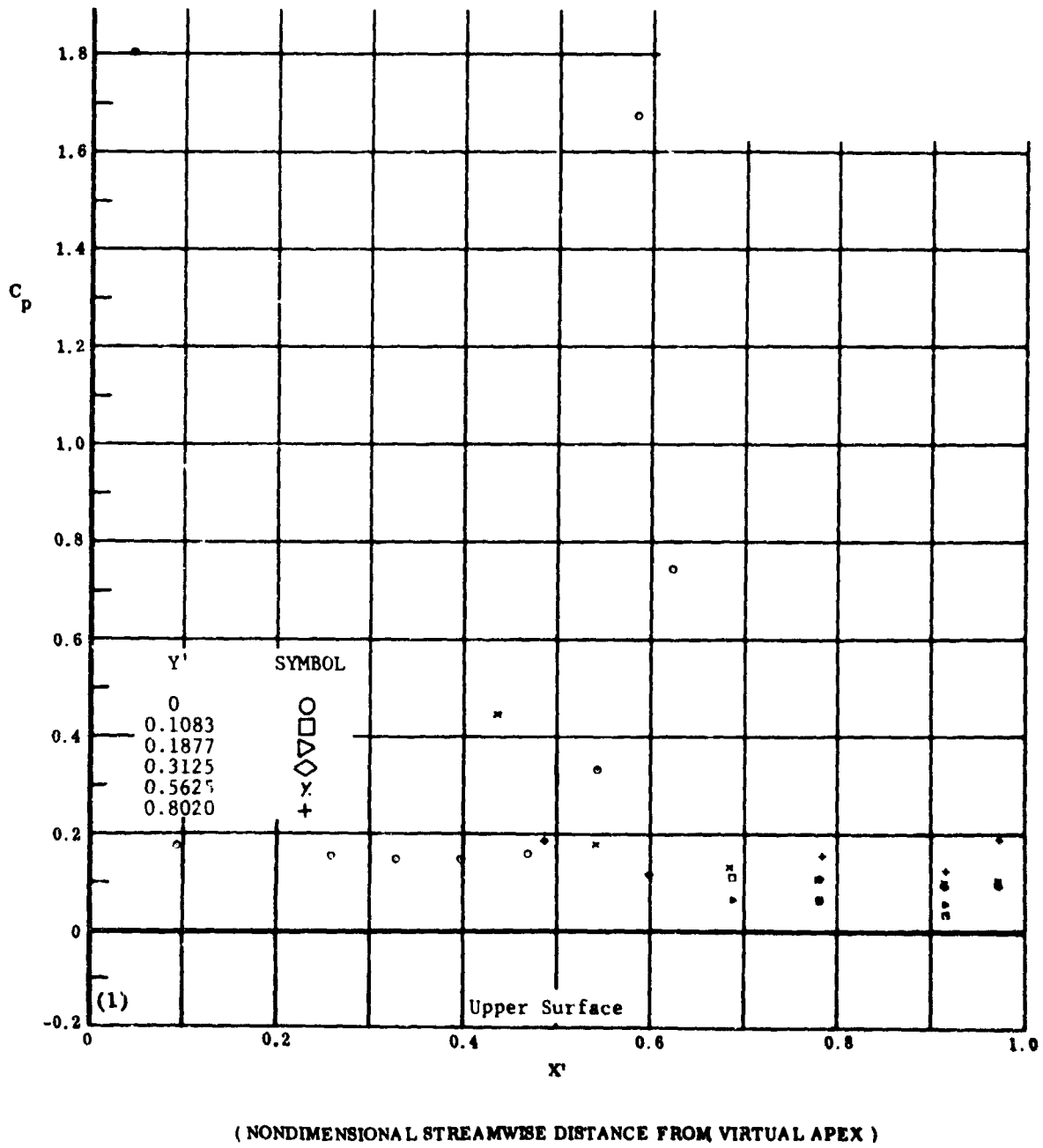
Fig. 51 Configuration VIII, Spoiler on, Re_\infty / ft \times 10^{-6} = 3.3
