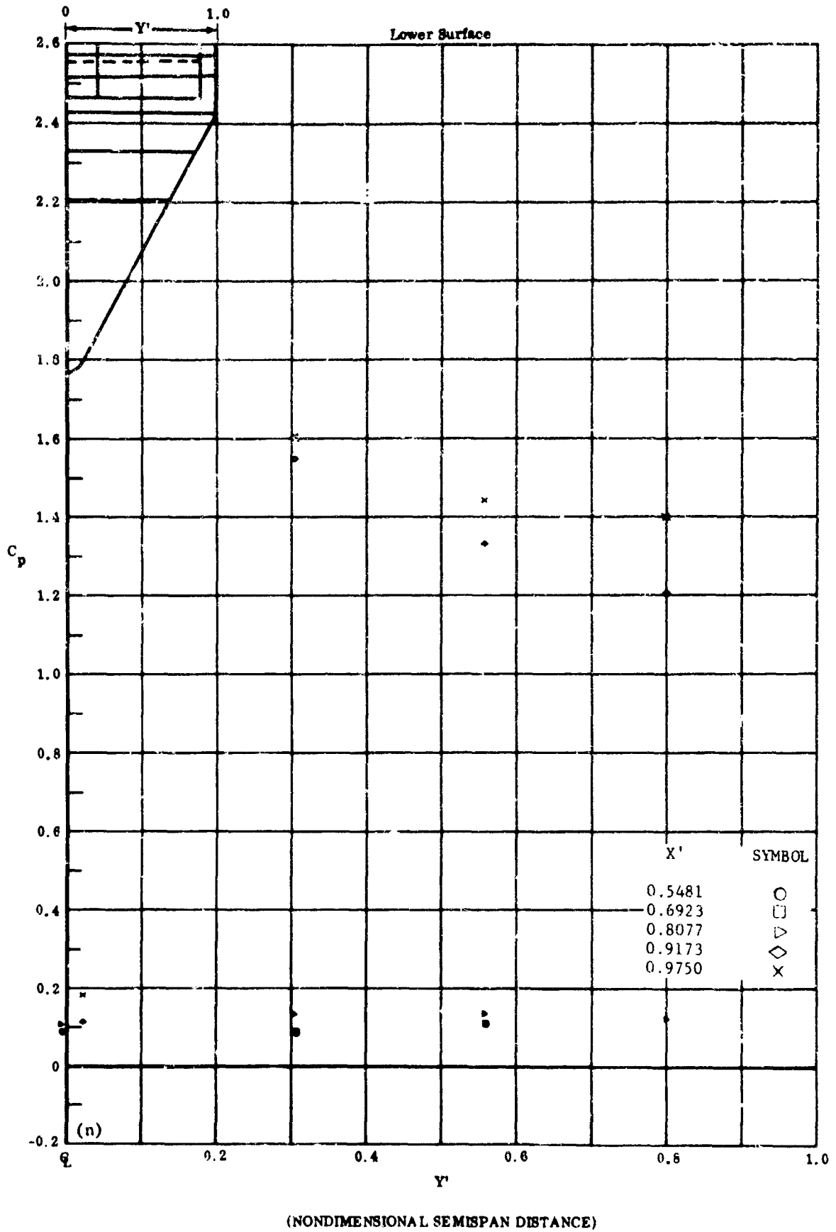
Fig. 5n Configuration I, \alpha = +10 , \delta_2 = \delta_3 = +30 C_p vs. Y' , lower surface
