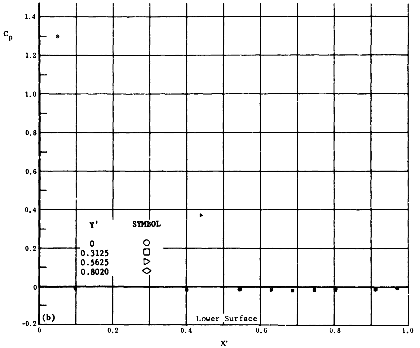
Fig. 22 Configuration I, \alpha = -30 , \delta_2 = \delta_3 = 0
