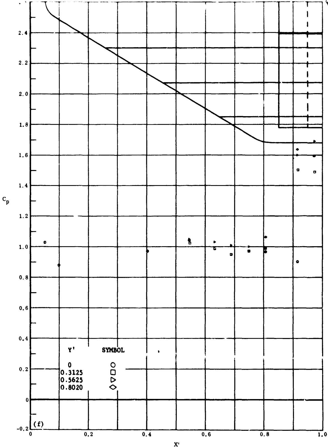
Fig. 11f Configuration I, \alpha = +40 , \delta_2 = \delta_3 = +10
