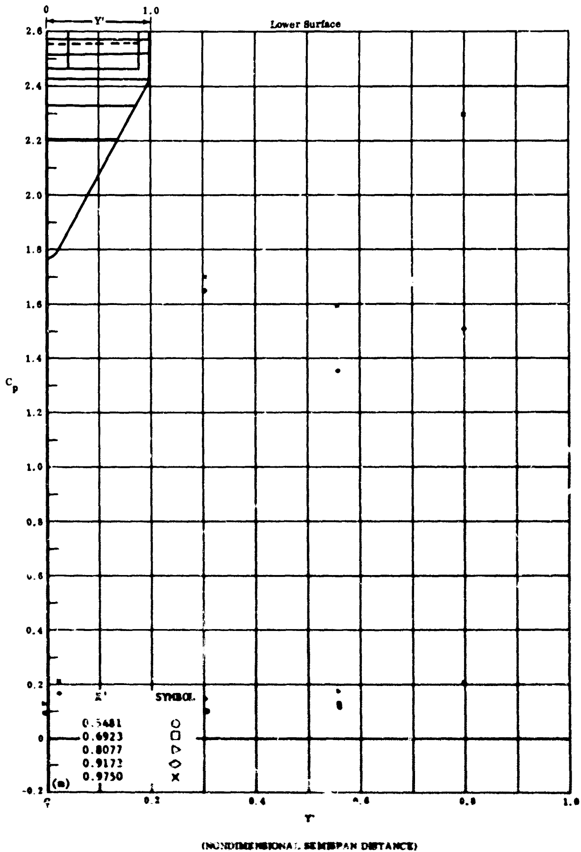
Fig. 11a Configuration IV, \alpha = +10 , \theta_2 = \theta_3 = +30 C_p vs. Y' , lower surface
