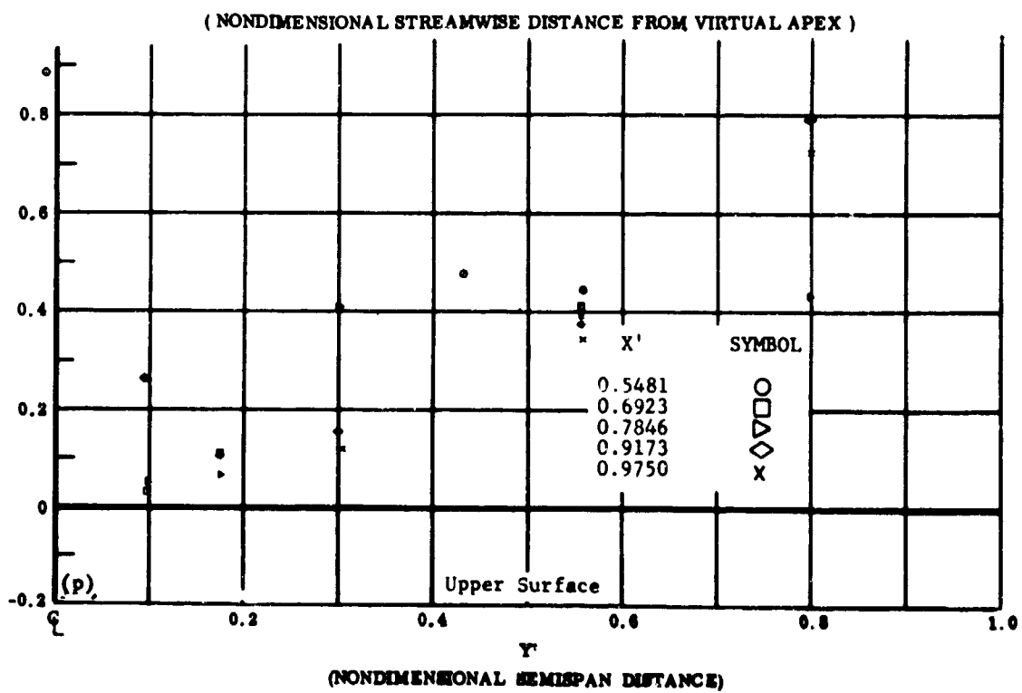
Fig. 51 Configuration VIII, Spoiler on, Re_{\rho}/ft \times 10^{-6} = 3.3
