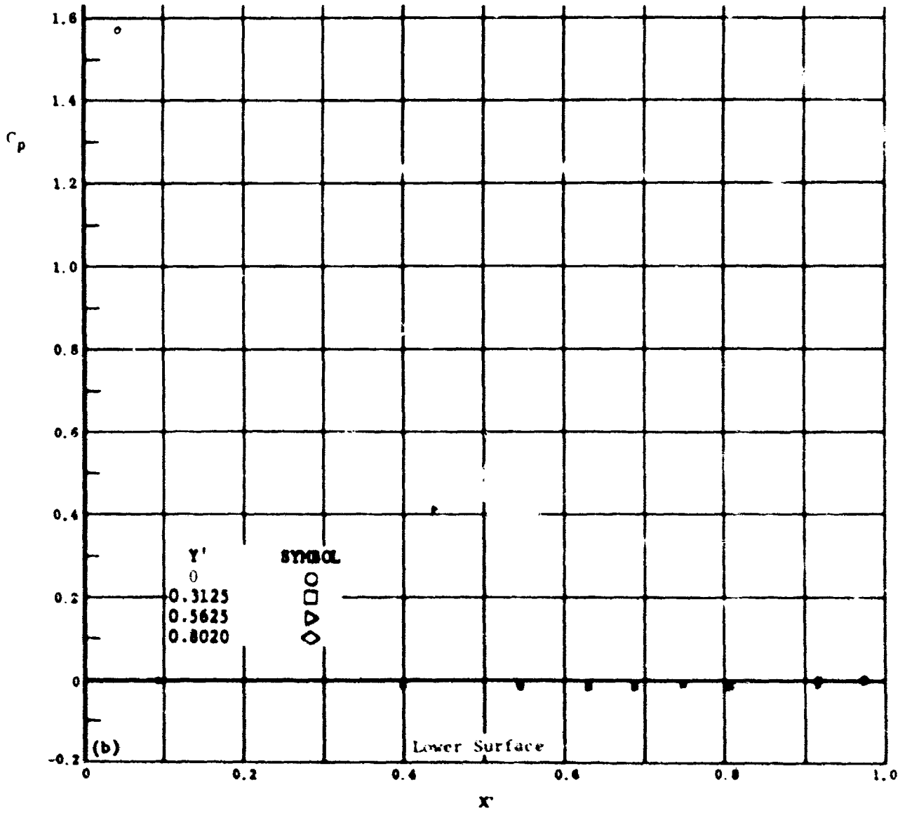
Fig. 43 Configuration IV, \alpha_1 = -20 , \alpha_2 = \alpha_3 = -10
