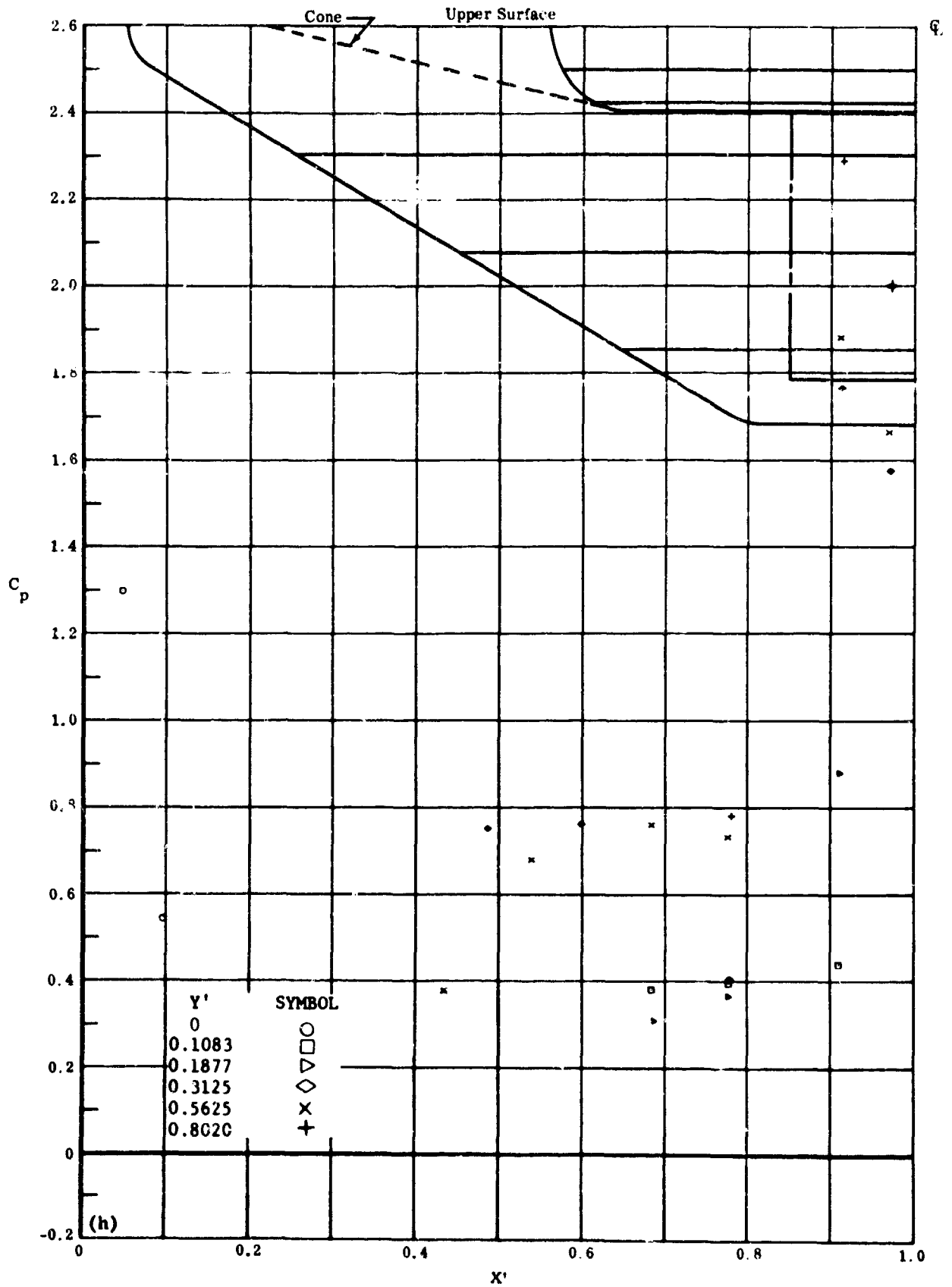
Fig. 23h Configuration I, \alpha = -30 , \delta_2 = \delta_3 = -20
