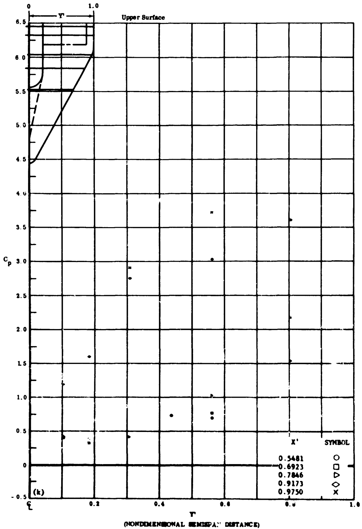
Fig. 23k Configuration I, \alpha = -30 , b_2 = b_3 = -30
