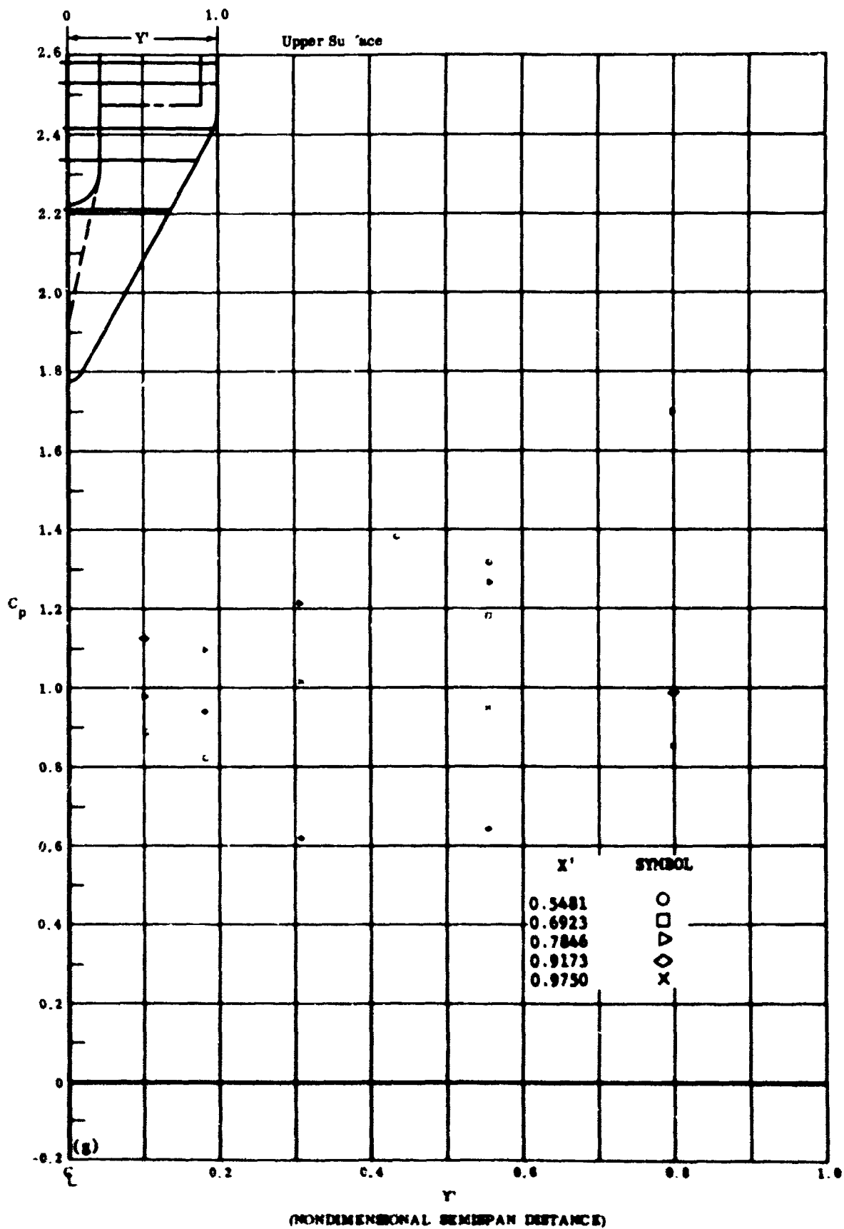
Fig. 48g Configuration IV, \alpha = -50 , \delta_2 = \delta_3 = +20
