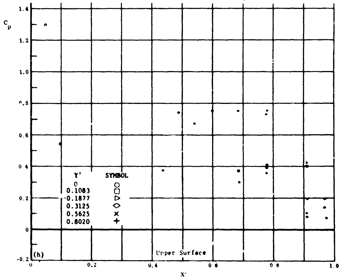
Fig. 22 Configuration I, \alpha_1 = -30 , \alpha_2 = \alpha_3 = +20
