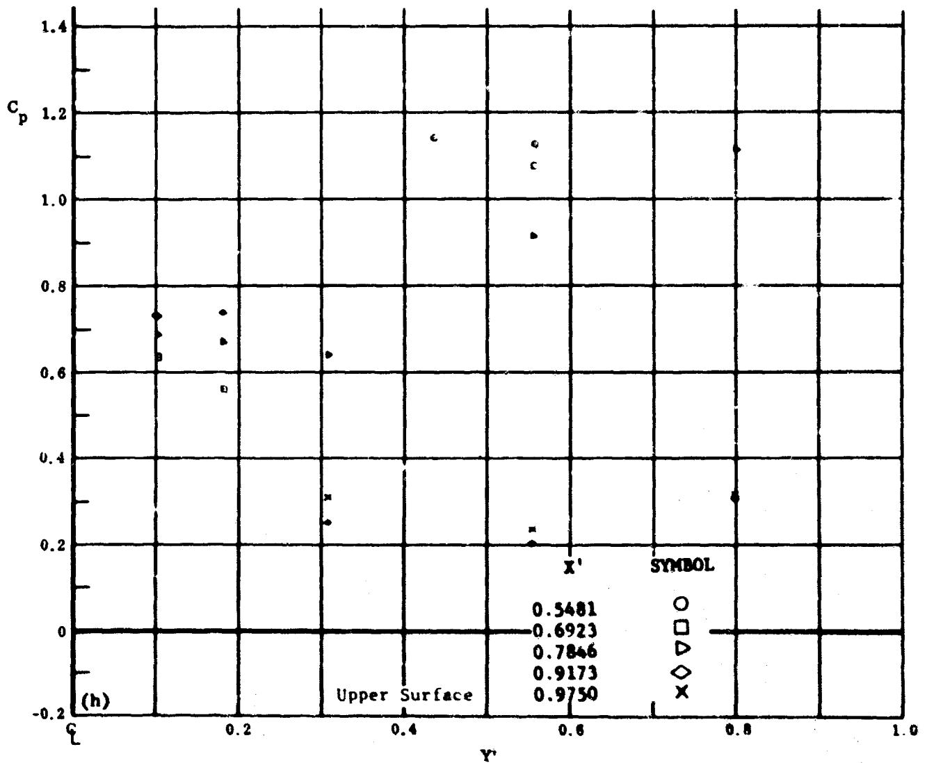
Fig. 25 Configuration I, \alpha = -40 , \delta_2 = \delta_3 = +20
