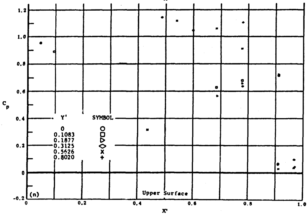
Fig. 25 Configuration I, \alpha = -40 , \delta_2 = \delta_3 = +39
