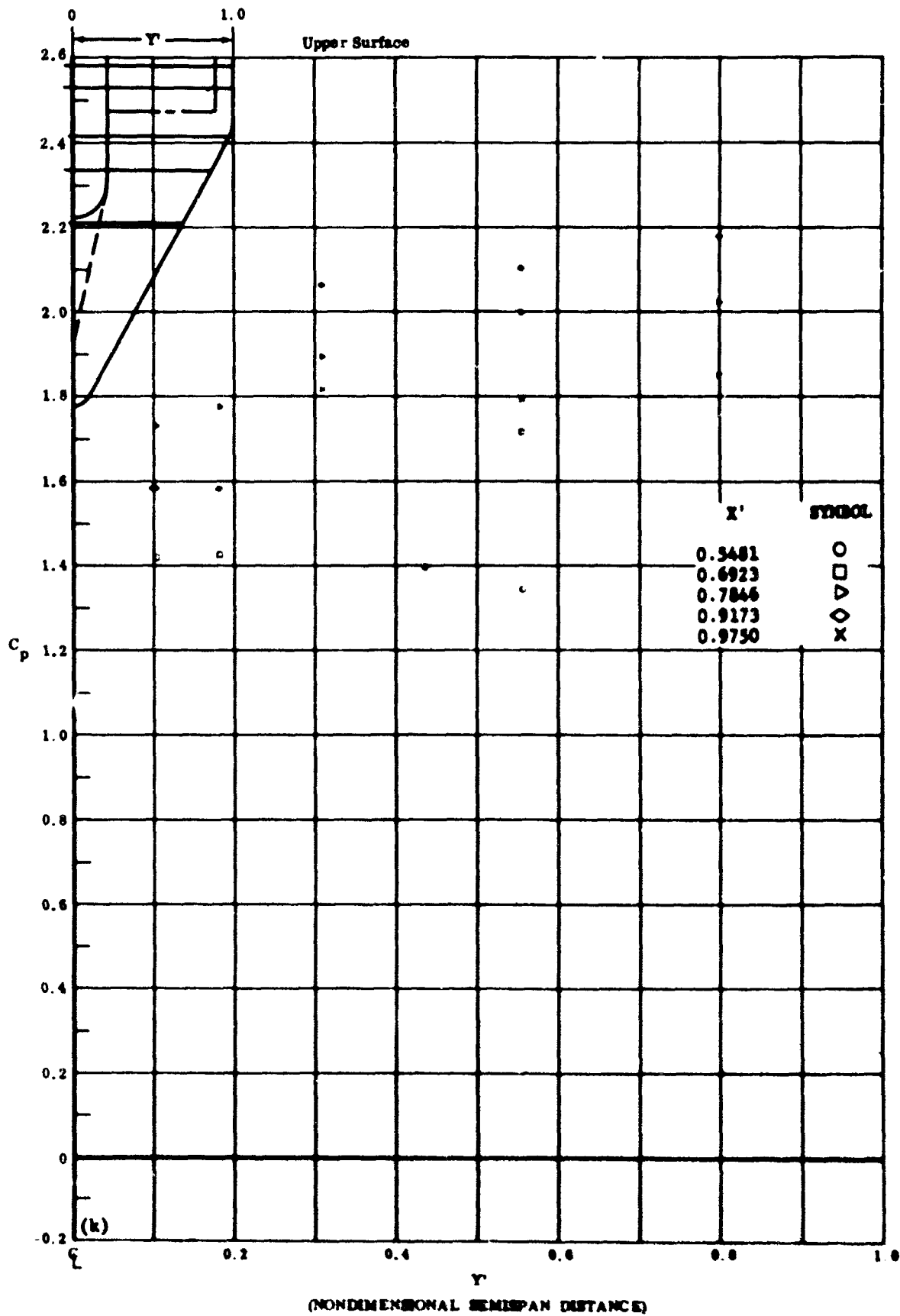
Fig. 49k Configuration IV, \alpha = -50 , \beta_2 = \beta_3 = -30
