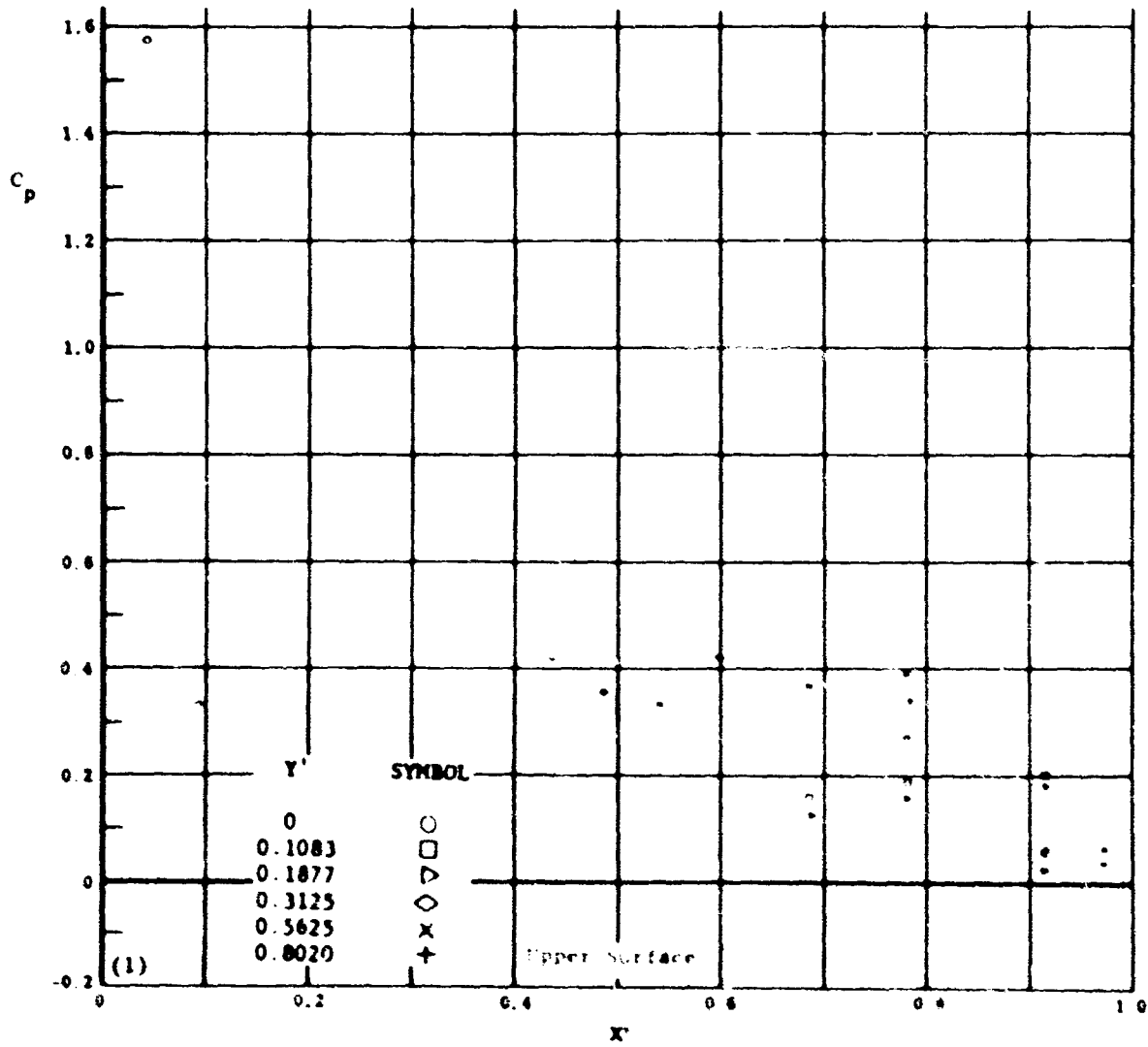
Fig. 19 Configuration I, \alpha_1 = -20^\circ , \alpha_2 = \alpha_3 = +20^\circ
