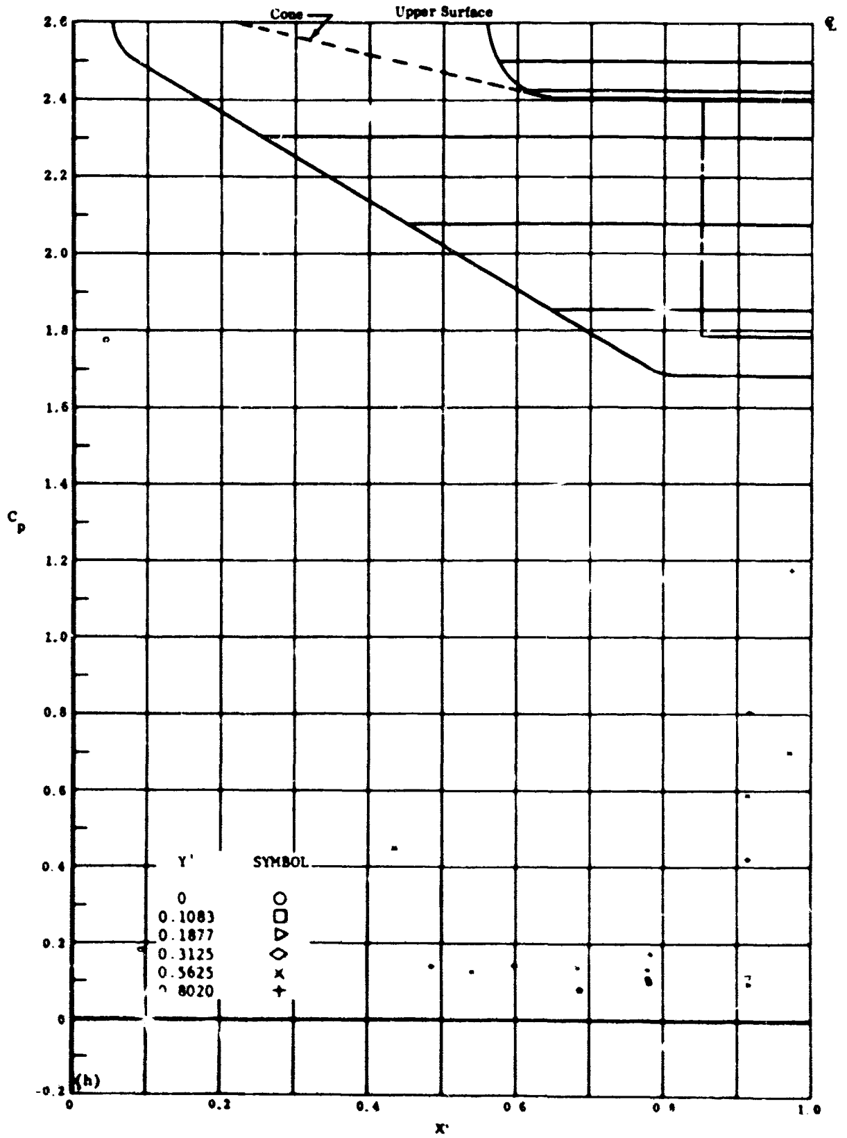
Fig. 41h Configuration IV, \alpha = -10^\circ , \beta_2 = \beta_3 = -20^\circ
