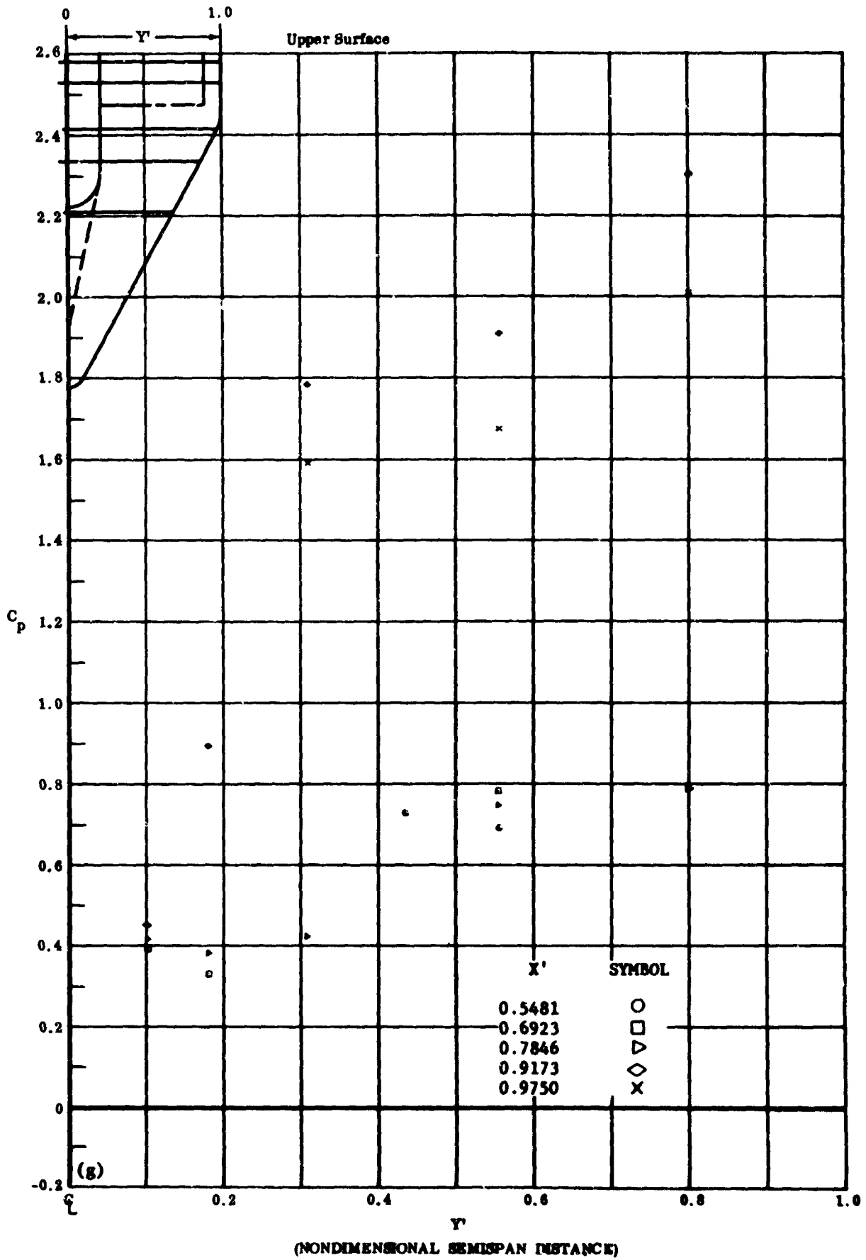
Fig. 23g Configuration I, \alpha = -30 , b_2 = b_3 = -20 C_p vs. Y' , upper surface
