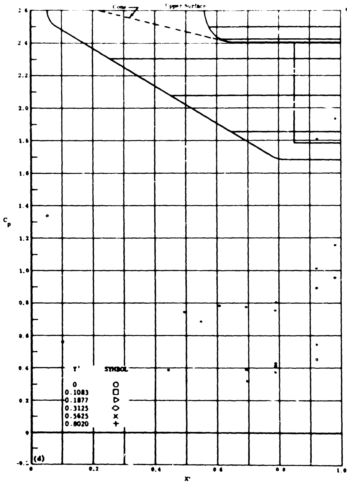
Fig. 45d Configuration IV, \alpha = -30 , \epsilon_2 = \epsilon_3 = -10
