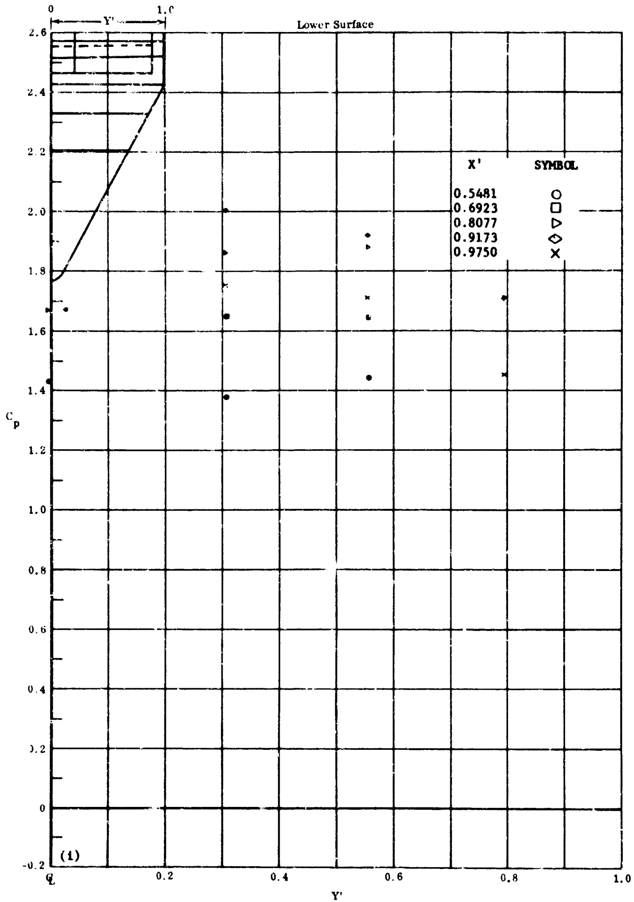
Fig. 131 Configuration I, \alpha = +50 , \delta_2 = \delta_3 = +20
