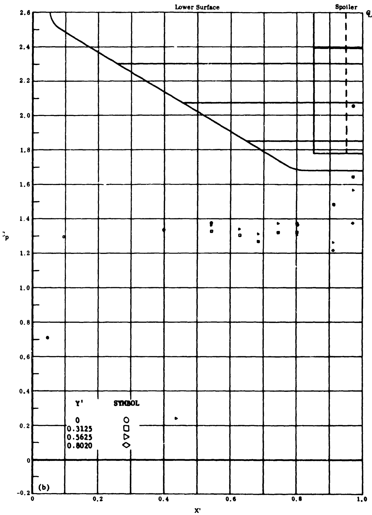
Fig. 13b Configuration I, \alpha = +50 , \delta_2 = \delta_3 = 0
