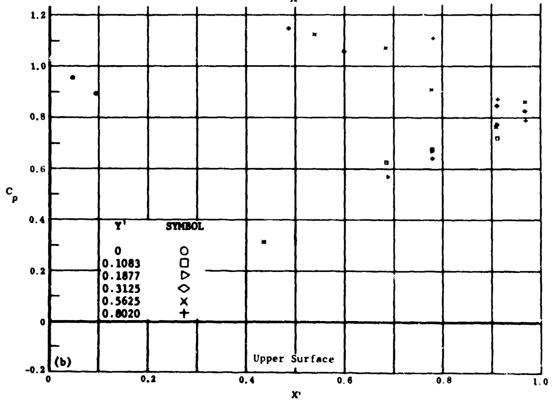
Fig. 25 Configuration I, \alpha = -40 , \delta_2 = \delta_3 = 0
