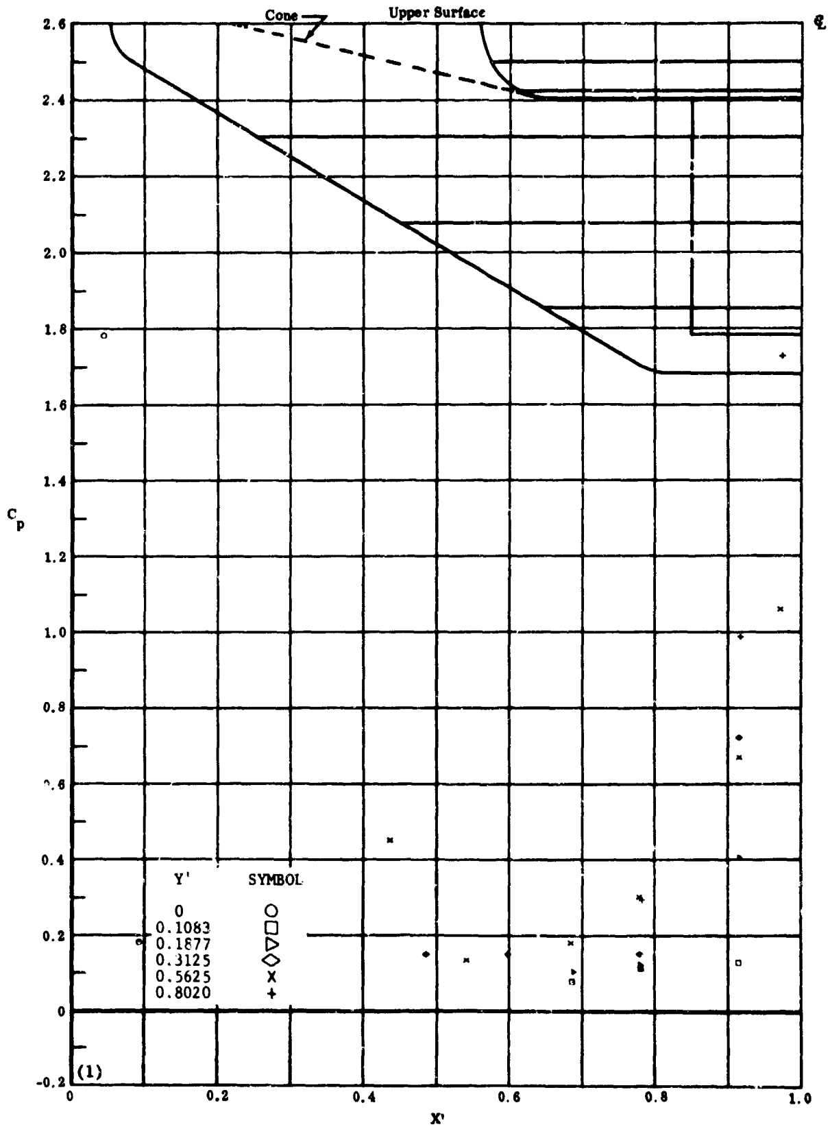
Fig. 411 Configuration IV, \alpha = -10 , \delta_2 = \delta_3 = -30
