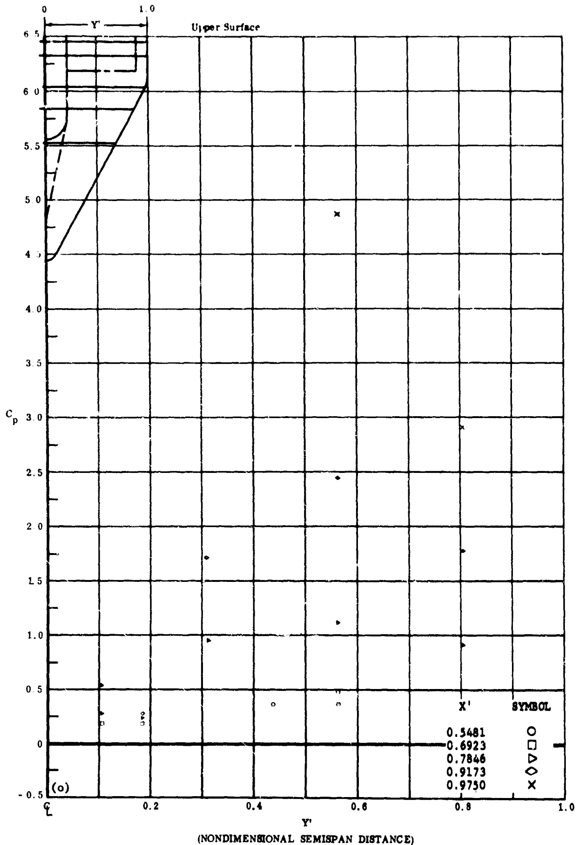
Fig. 20o Configuration I, \alpha = -20 , \delta_2 = \delta_3 = -39 C_p vs. Y' , upper surface
