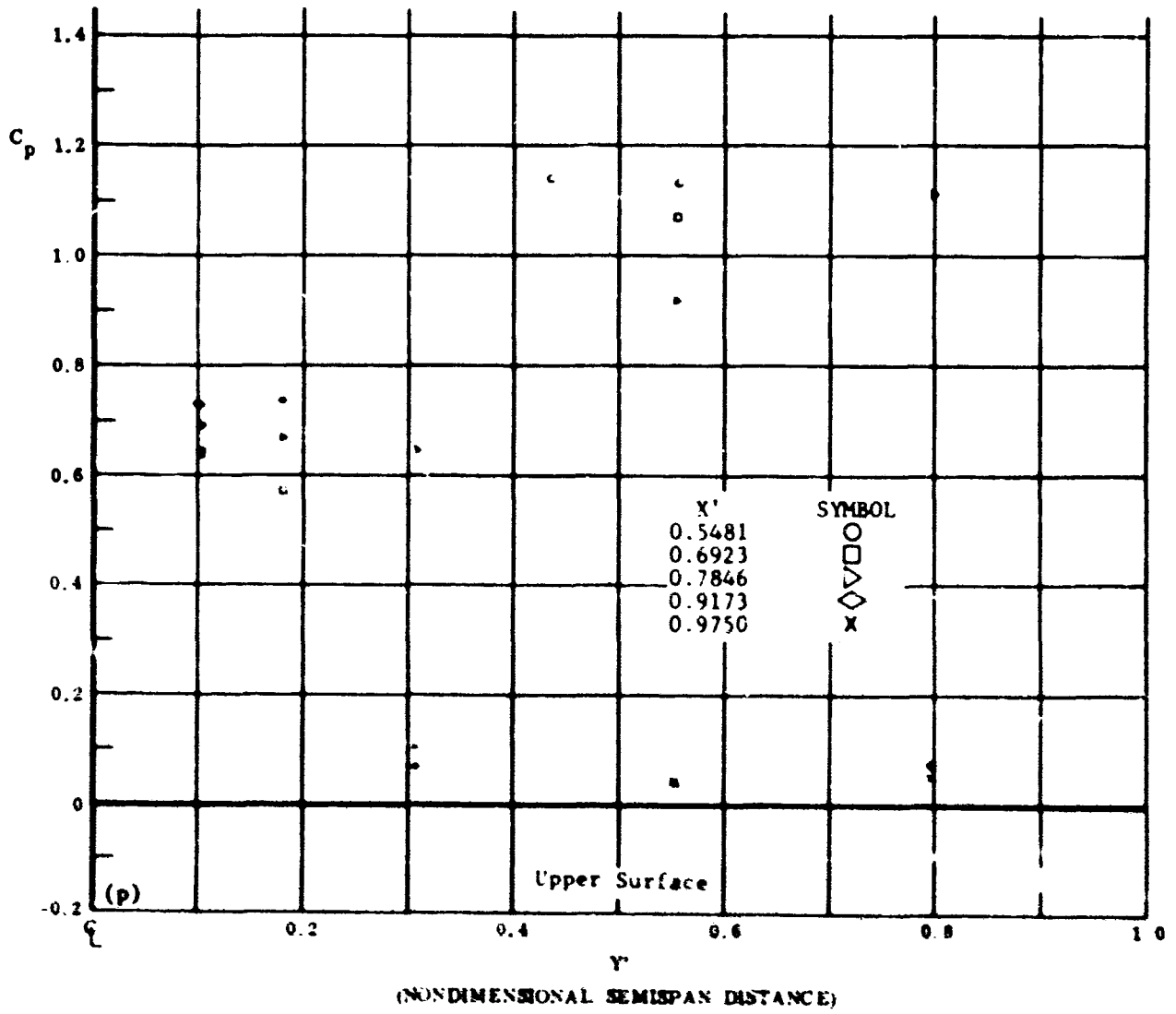
Fig. 25 Configuration I, \alpha_1 = -40 , \alpha_2 = \alpha_3 = +39
