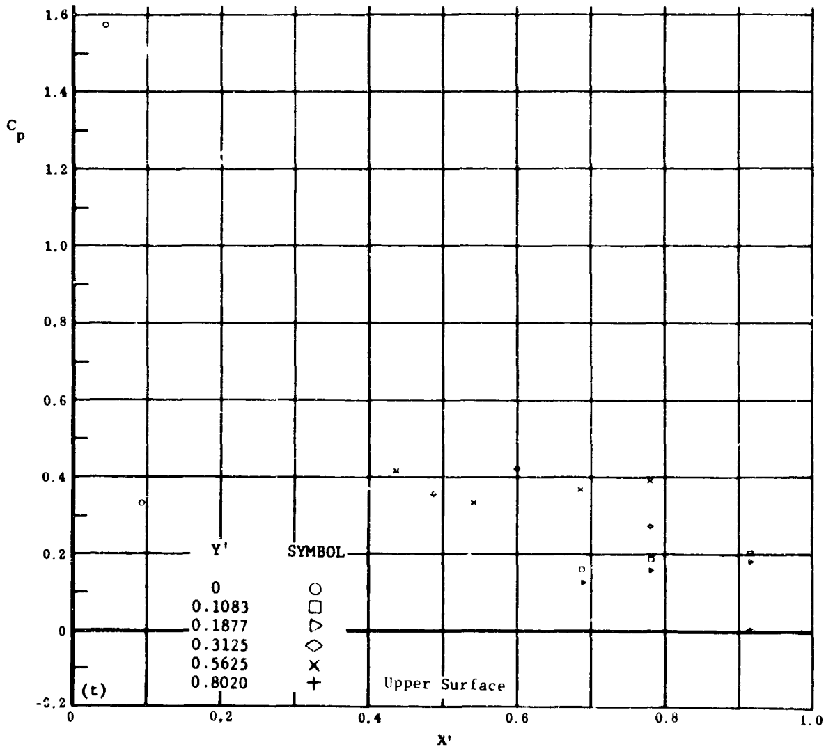
Fig. 19 Configuration I, \alpha = -20 , \delta_2 = \delta_3 = +39
