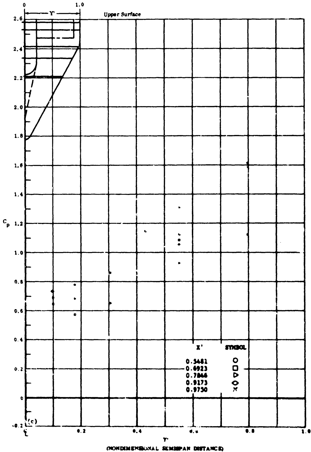
Fig. 46c Configuration IV, \alpha = -40^\circ , \beta_2 = \beta_3 = 0
