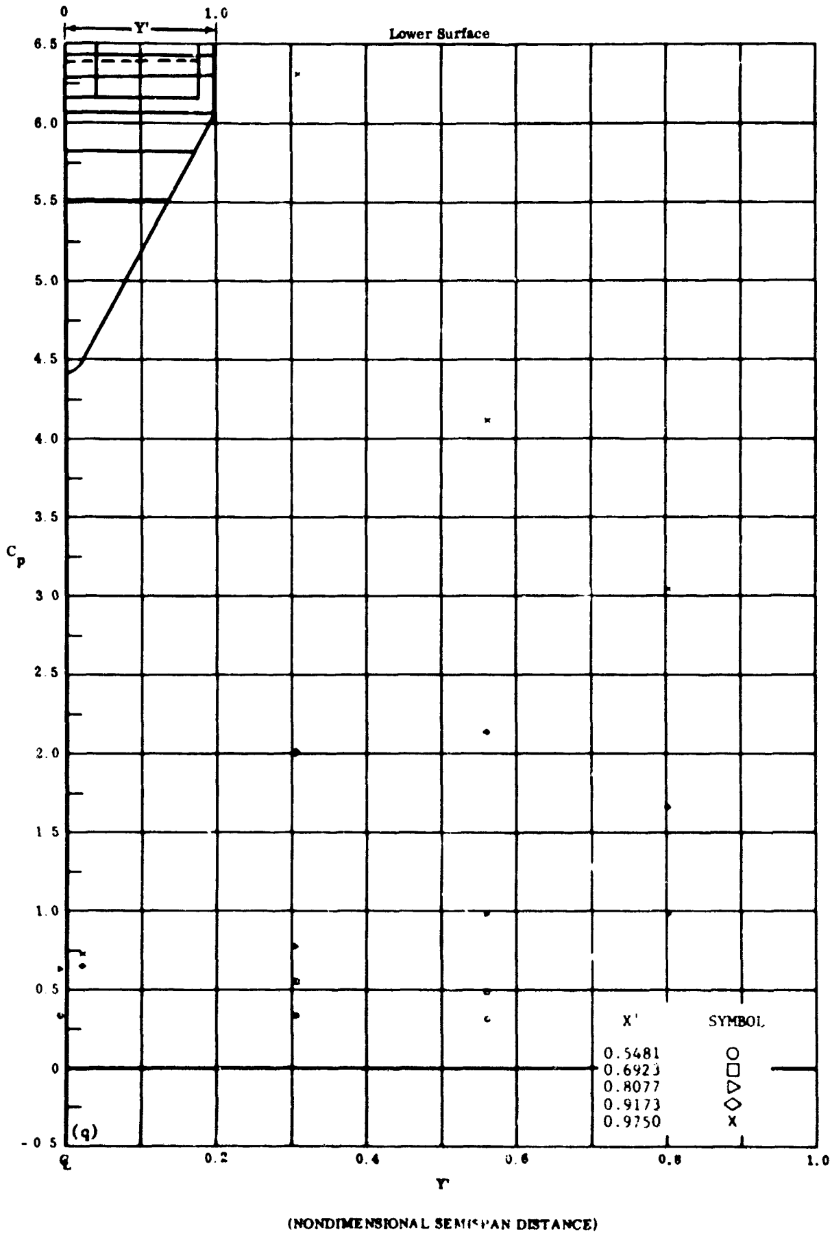
Fig. 7q Configuration I, \alpha_1 = +20 , \alpha_2 = \alpha_3 = +39
