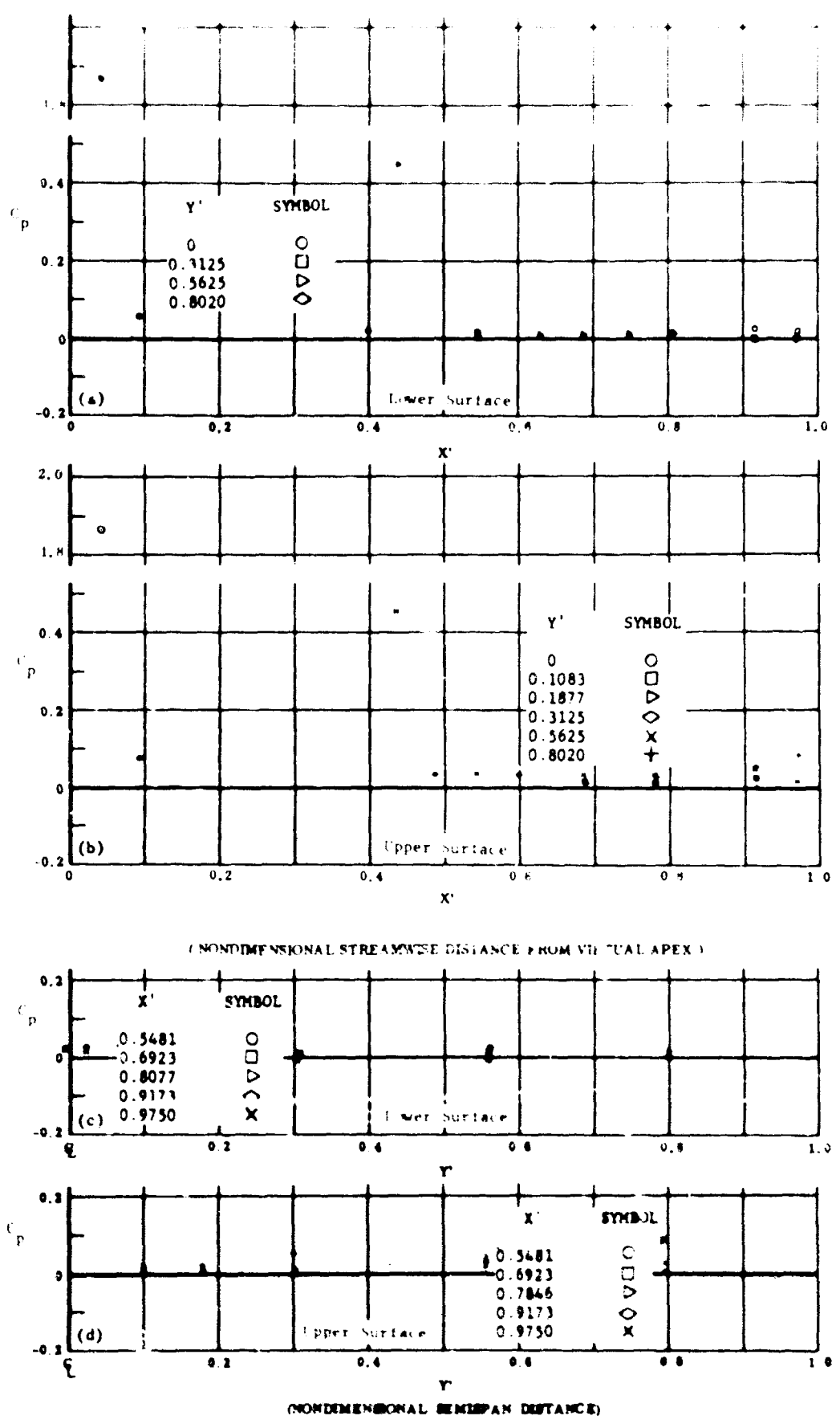
Fig. 4 Configuration I, \alpha = 0^\circ , \beta_1 = \beta_2 = -10^\circ
