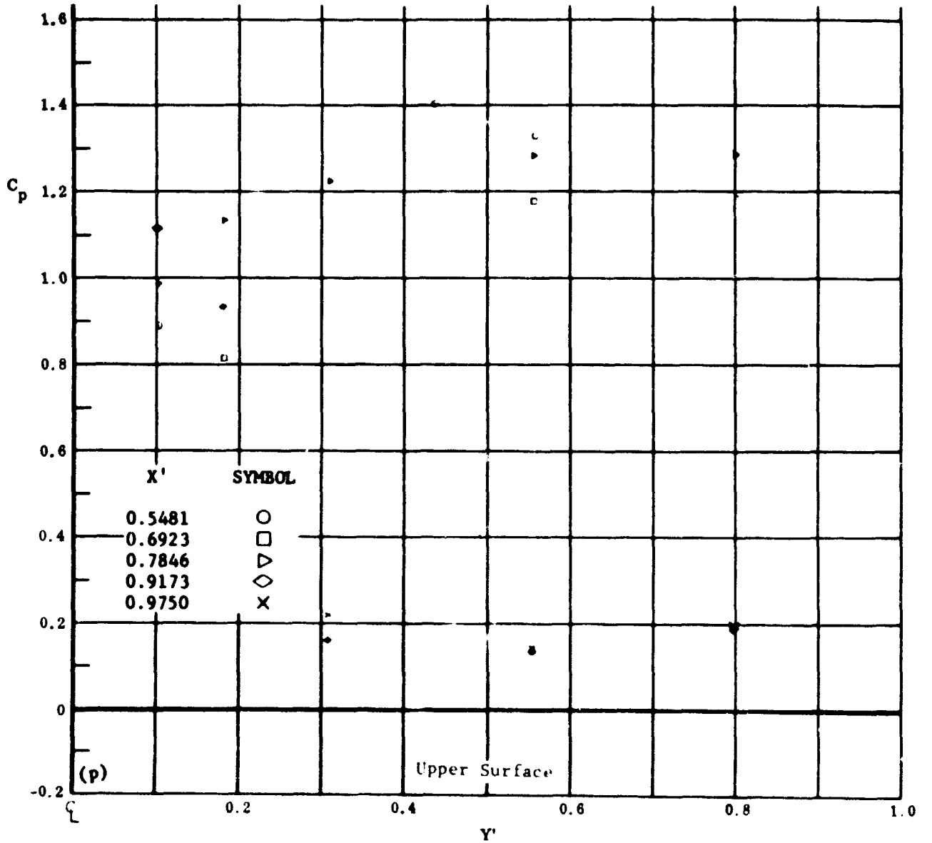
Fig. 27 Configuration I, \alpha = -50 , \beta_2 = \beta_3 = +39
