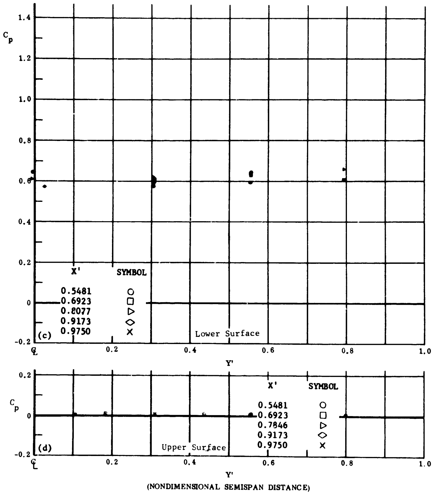
Fig. 9 Configuration I, \alpha = +30 , \delta_2 = \delta_3 = 0
