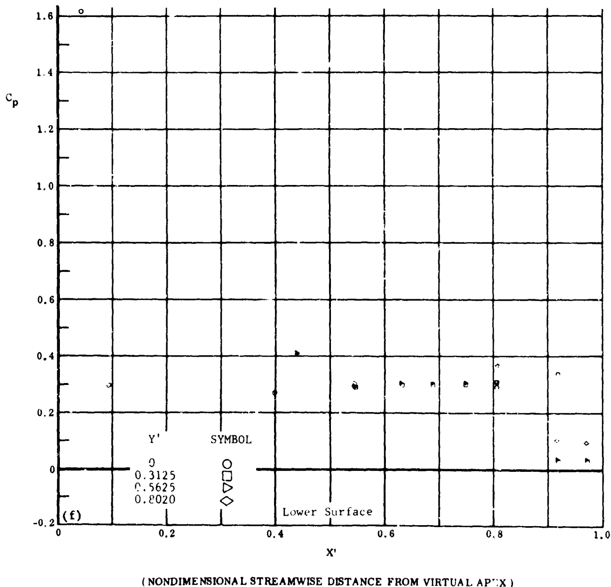
Fig. 34 Configuration IV, \alpha = +20^\circ , \delta_2 = \delta_3 = -20^\circ
