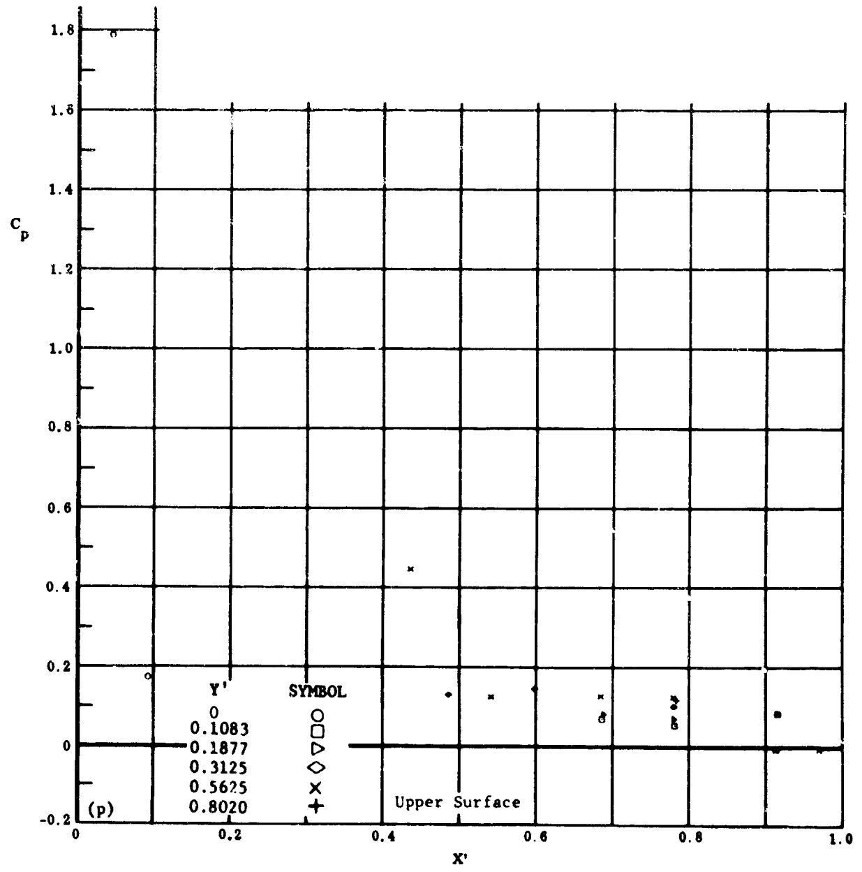
Fig. 16 Configuration I, \alpha = -10 , \delta_2 = \delta_3 = +30
