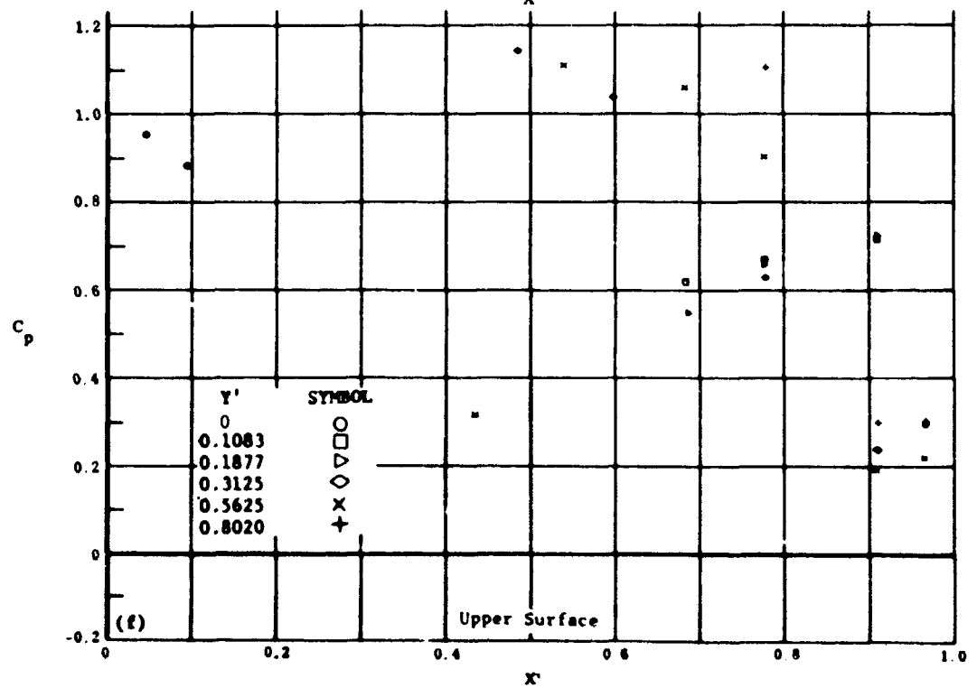
Fig. 25 Configuration I, \alpha = -40 , \delta_2 = \delta_3 = +20
