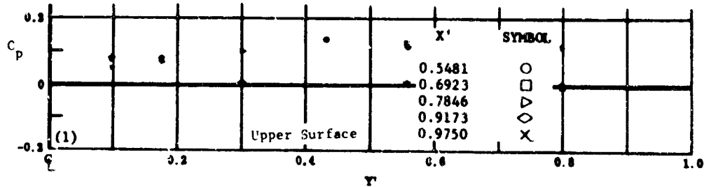
Fig. 16 Configuration I, \alpha = -10 , \delta_2 = \delta_3 = +20
