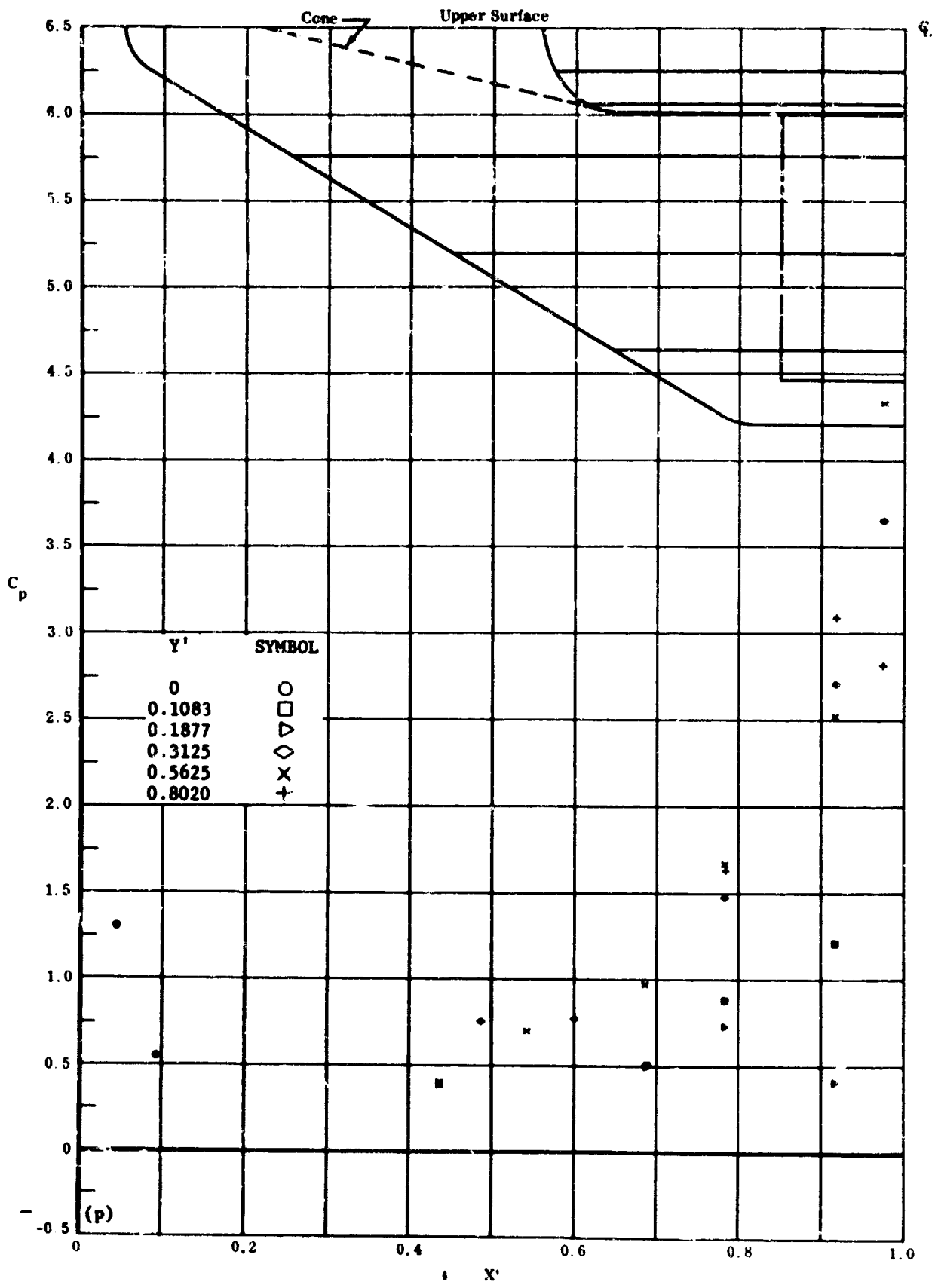
Fig. 23p Configuration I, \alpha = -30 , b_2 = b_3 = -39
