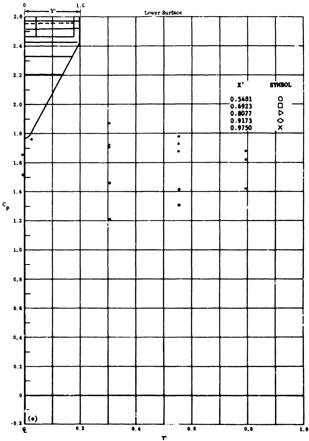
Fig. 13e Configuration i, \alpha = +50 , \delta_2 = \delta_3 = +10
