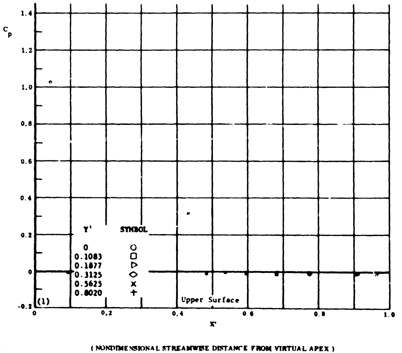
Fig. 37 Configuration IV, \alpha = +40 , \delta_2 = \delta_3 = +20
