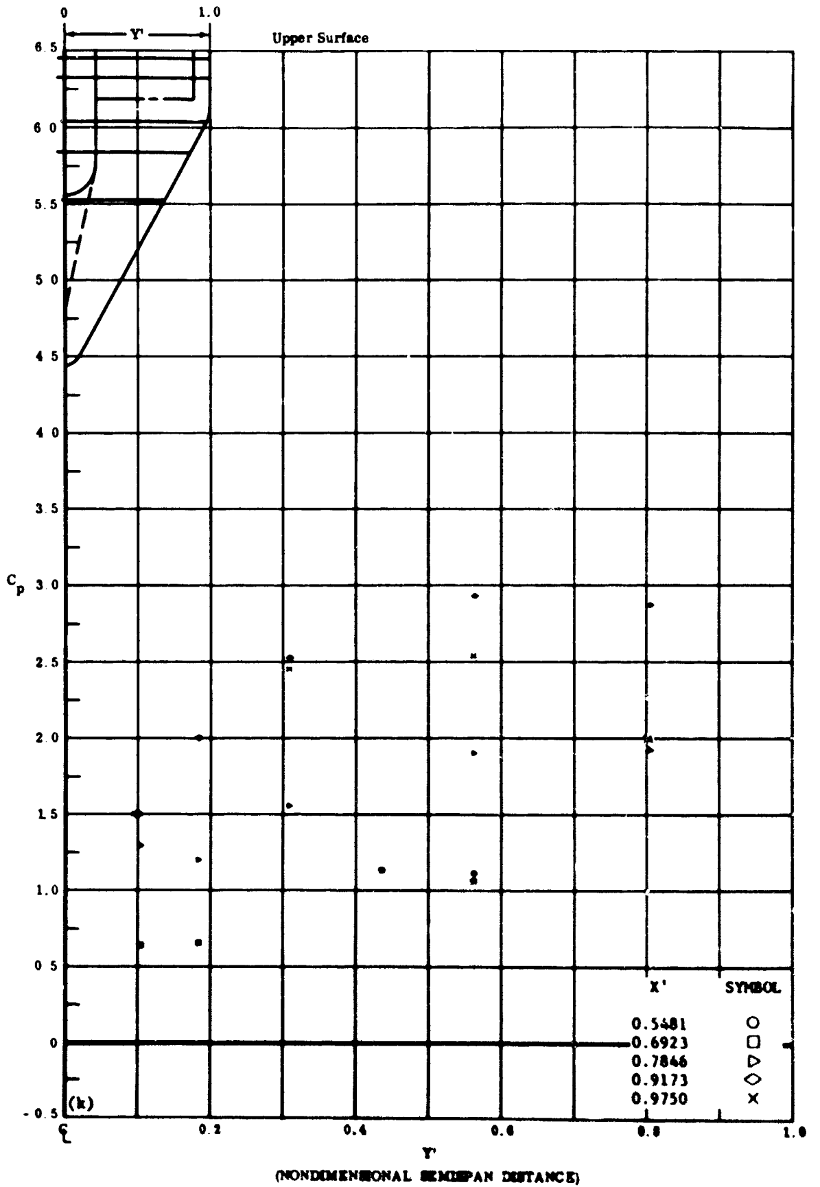
Fig. 26k Configuration I, \alpha = -40 , \delta_2 = \delta_3 = -30
