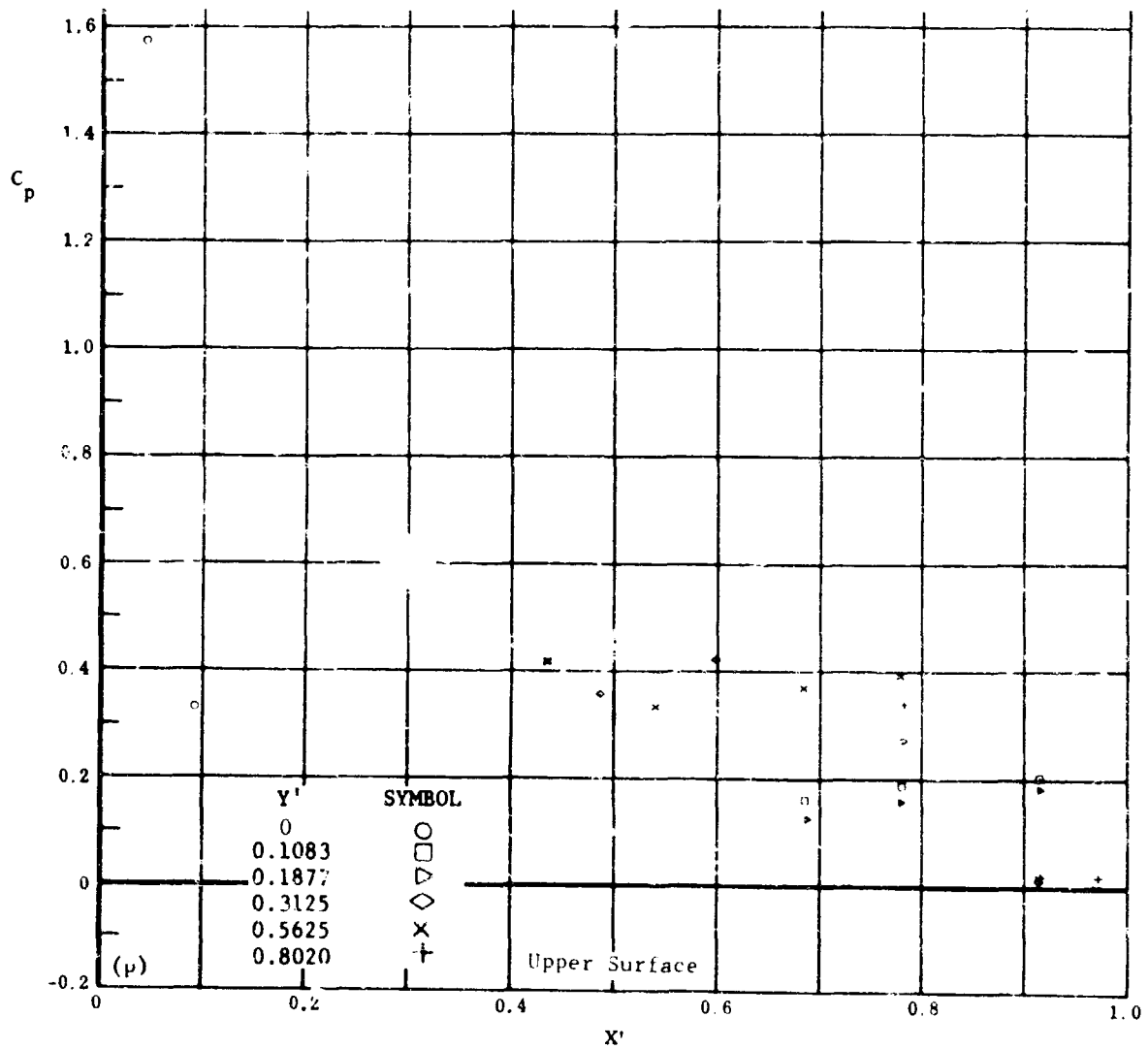
Fig. 19 Configuration I, \alpha = -20 , \beta_2 = \beta_3 = +30
