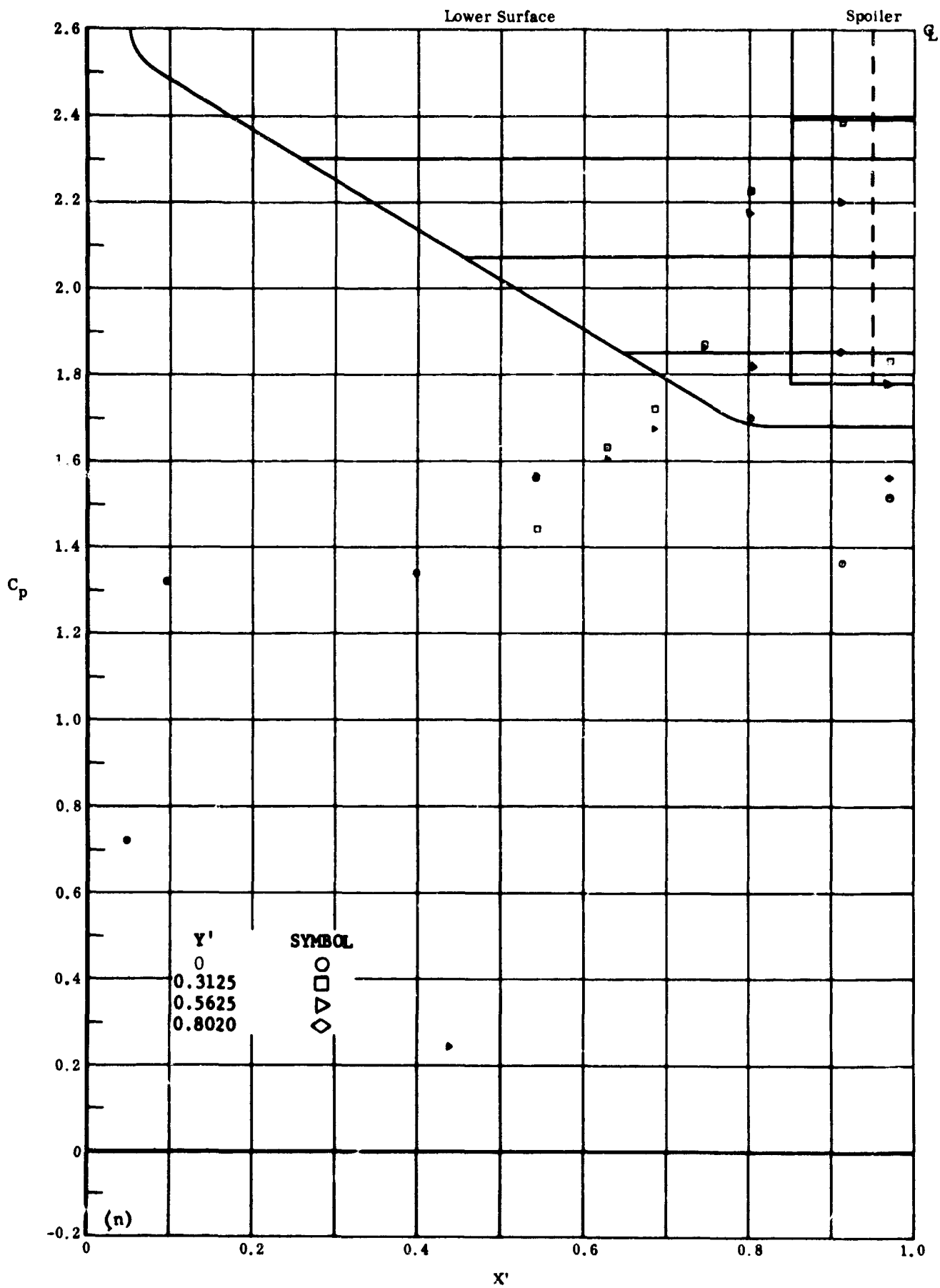
Fig. 13n Configuration I, \alpha = +50 , \delta_2 = \delta_2 = +39
