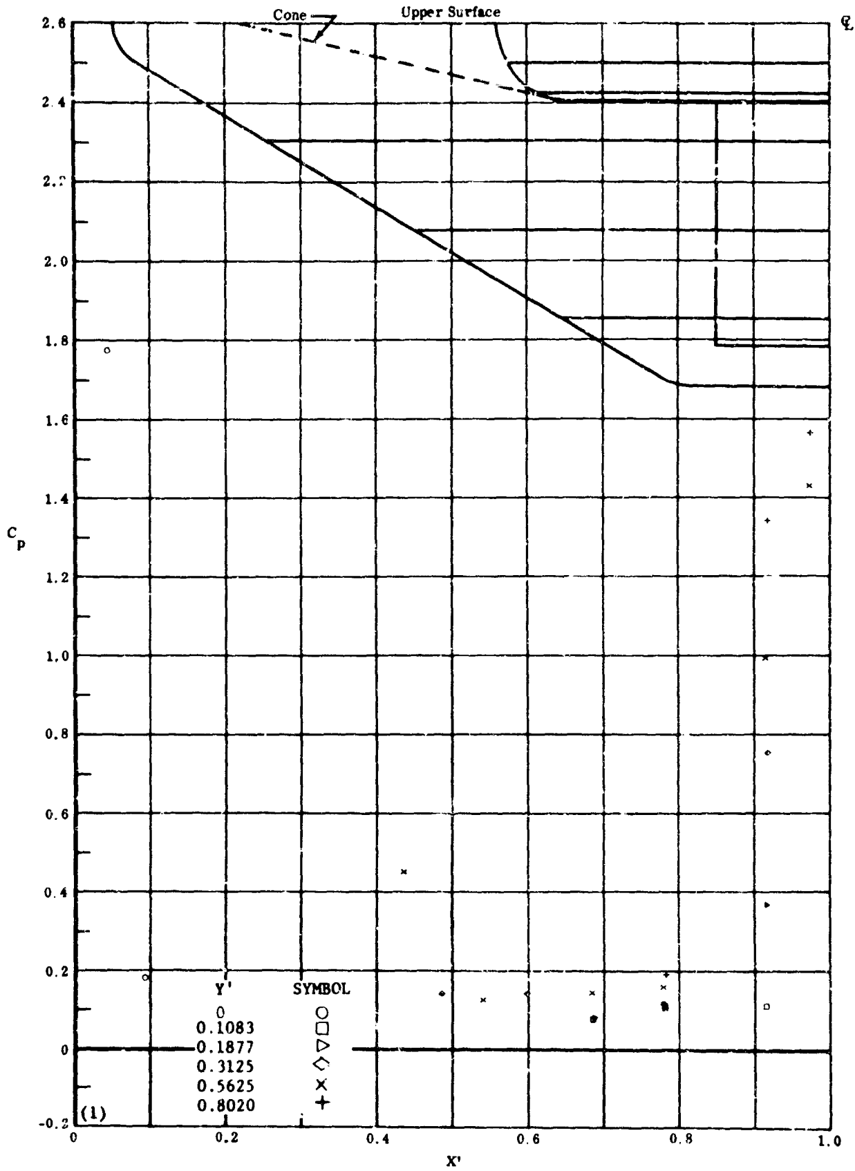
Fig. 171 Configuration I, \alpha = -10 , \delta_2 = \delta_3 = -30
