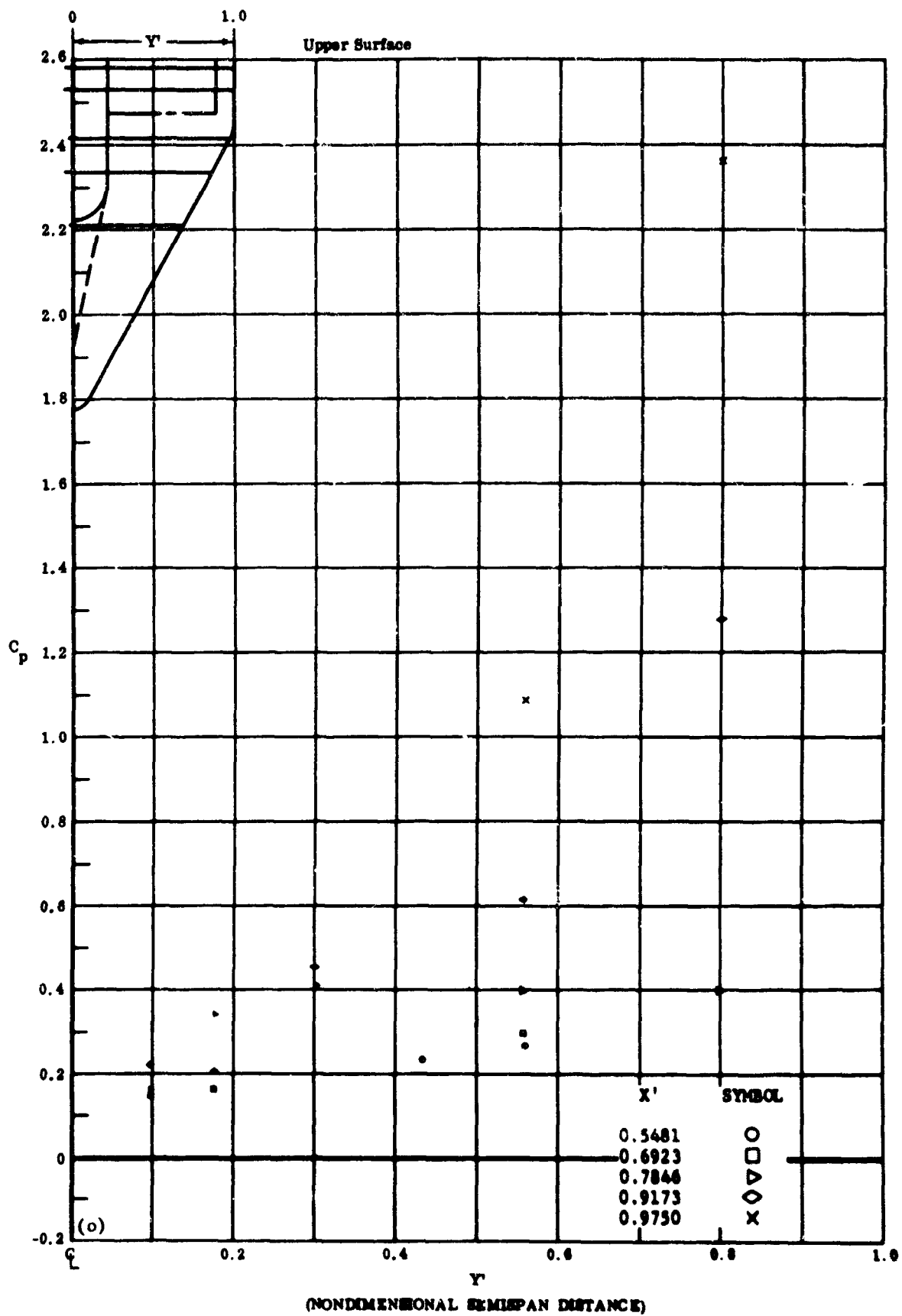
Fig. 41a Configuration IV, \alpha = -10 , \delta_2 = \delta_3 = -39
