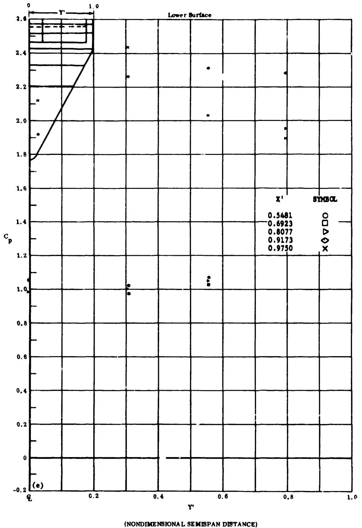
Fig. 37e Configuration IV, \alpha = +40 , \delta_2 = \delta_3 = +10
