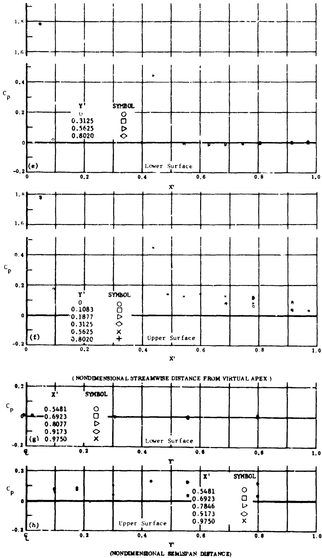
Fig. 16 Configuration I, \alpha = -10 , \delta_2 = \delta_3 = +10
