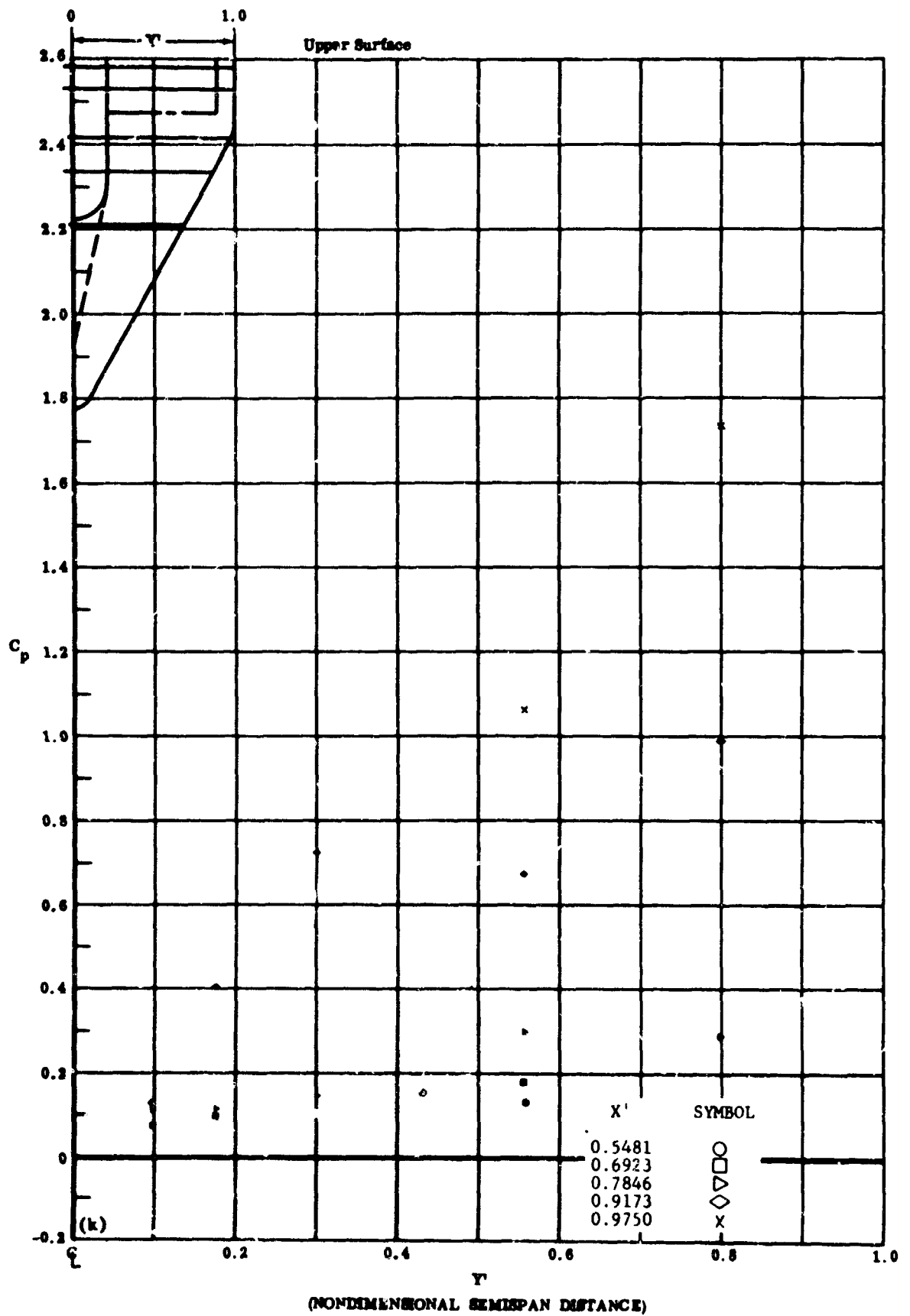
Fig. 41k Configuration IV, \alpha = -10 , b_2 = b_3 = -30
