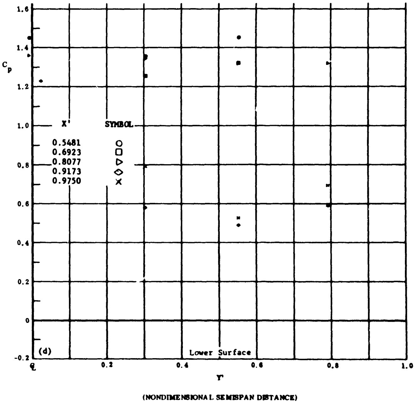
Fig. 14 Configuration I, \alpha = +50 , \beta_2 = \beta_3 = -20
