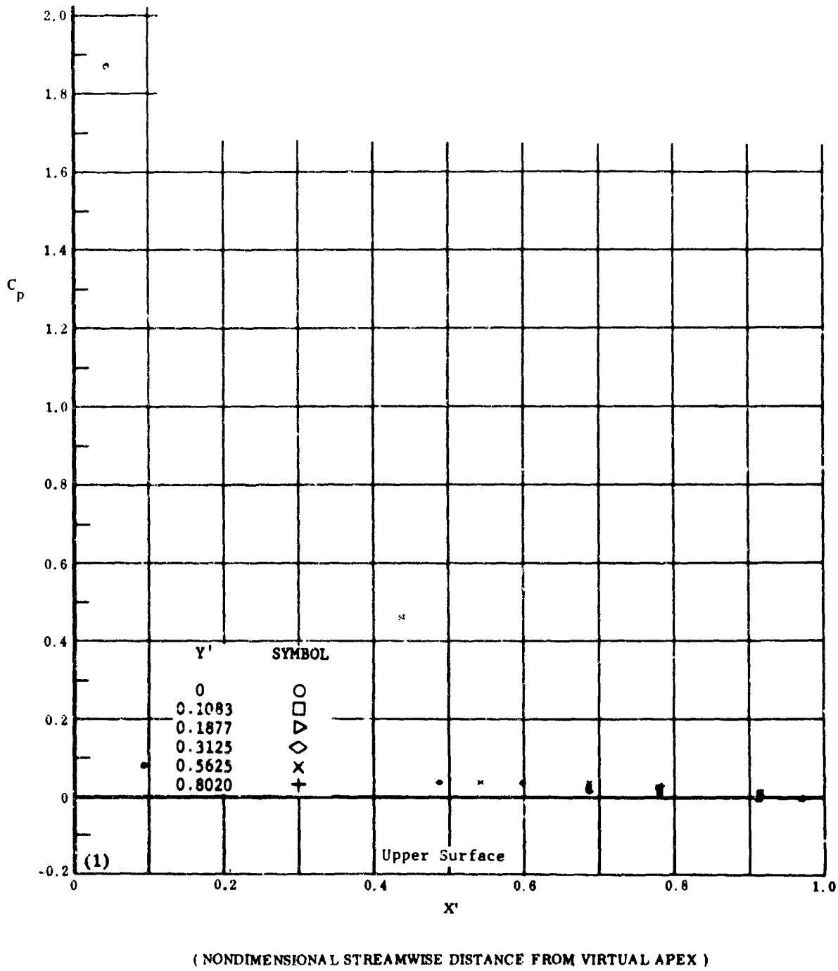
Fig. 3 Configuration I, \alpha = 0 , \delta_2 = \delta_3 = +20
