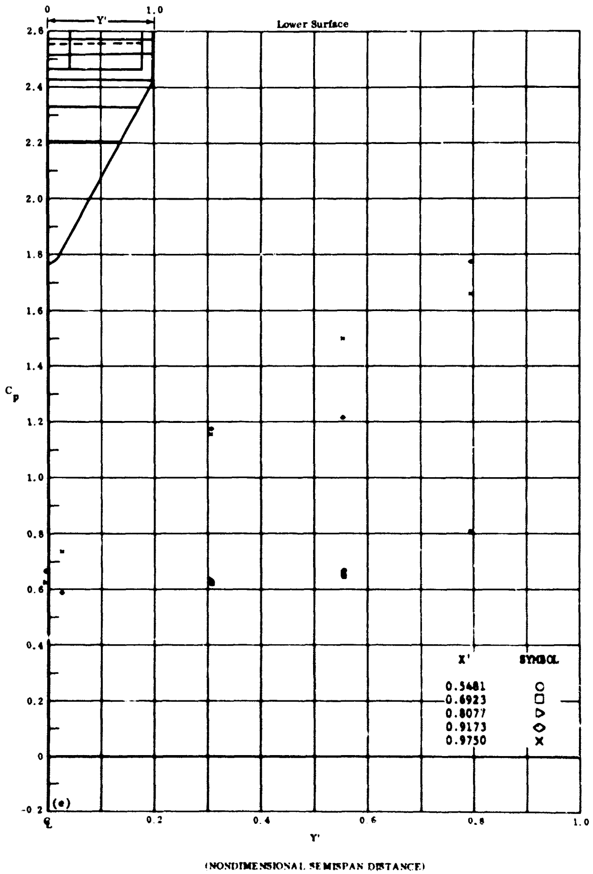
Fig. 35e Configuration IV, \alpha_1 = +30 , \alpha_2 = \alpha_3 = +10
