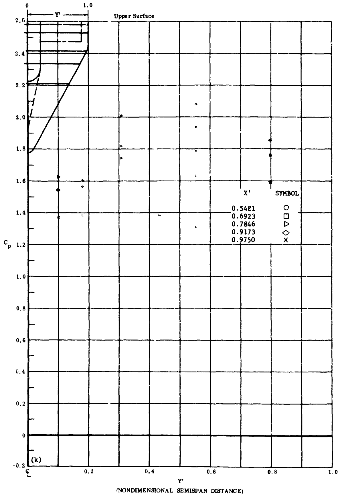
Fig. 28k Configuration I, \alpha = -50 , \delta_2 = \delta_3 = -30
