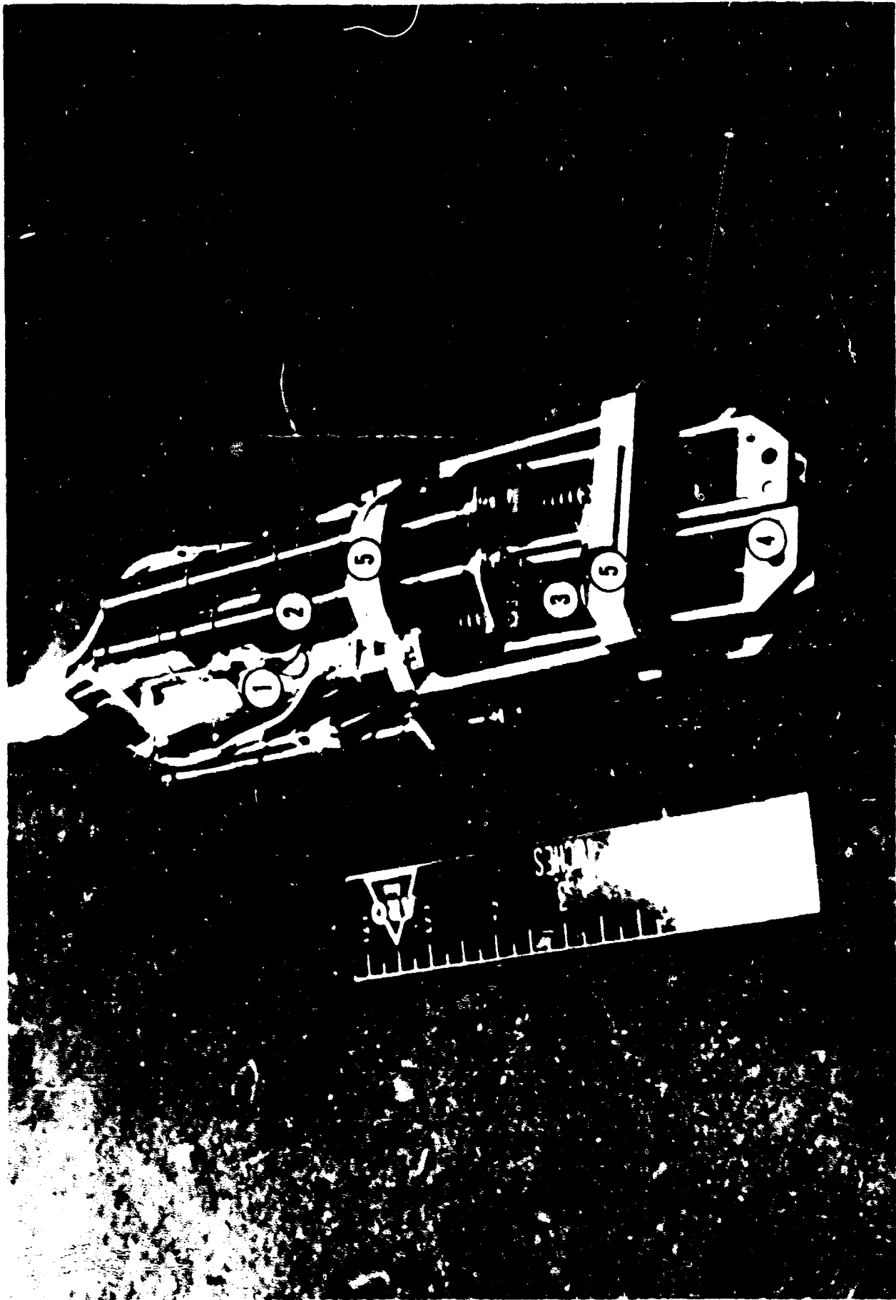
Figure 1/ Photograph - Actuator Assembly (1) Electric Motors, (2) Potentiometers, (3) Lead Screws, (4) Control Rods (5) Water Cooled Bulkheads
