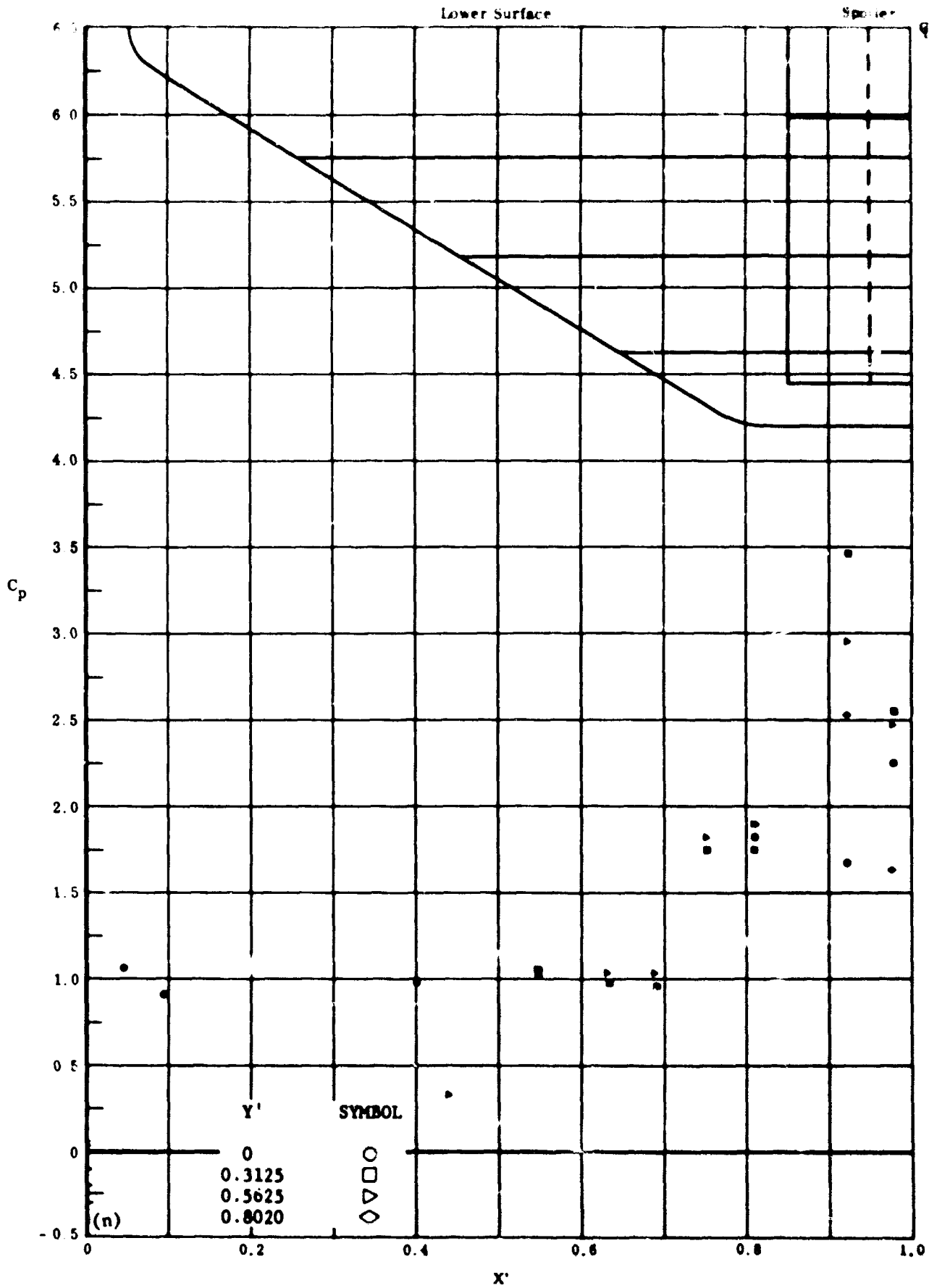
Fig. 11n Configuration I, \alpha = +40 , \delta_2 = \delta_3 = +30
