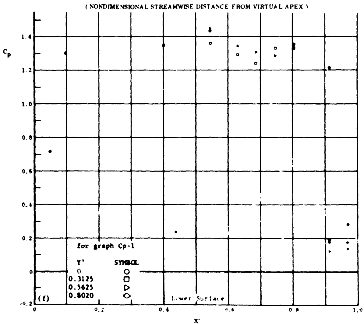
Fig. 14 Configuration I, \alpha_1 = +50 , \alpha_2 = \alpha_3 = -39
