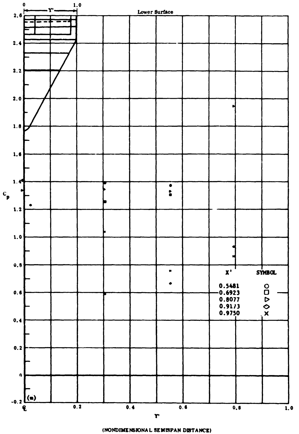
Fig. 39m Configuration IV, \alpha = +50 , \delta_2 = \delta_3 = -20
