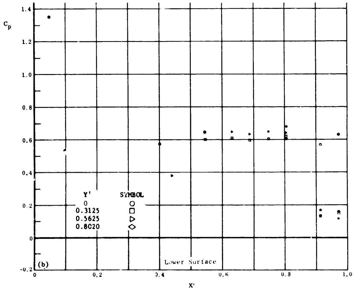
Fig. 10 Configuration I, \alpha = +30 , \beta_2 = \beta_3 = -20
