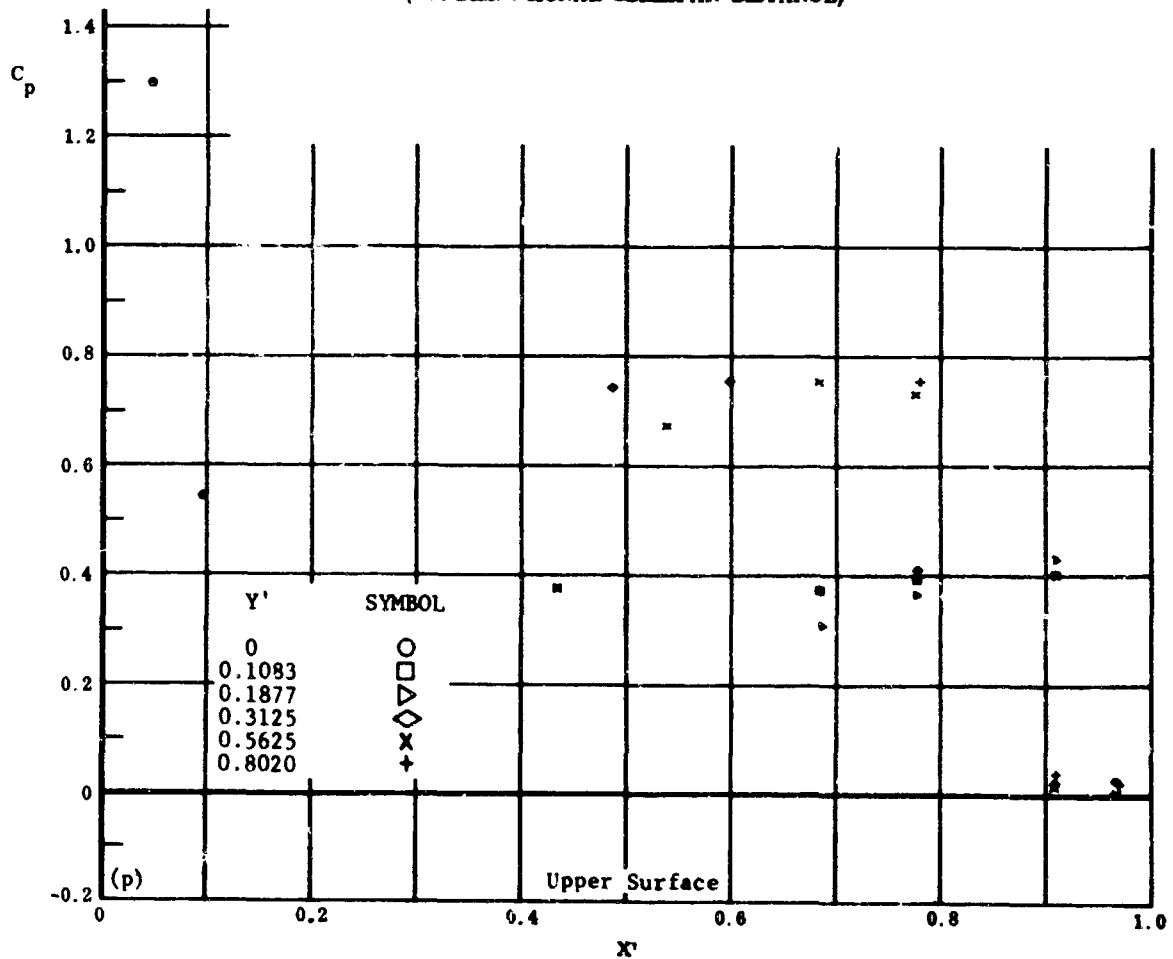
Fig. 22 Configuration I, \alpha = -30 , \delta_2 = \delta_3 = +39
