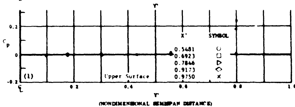
Fig. 6 Configuration I, \alpha = +10 , \beta_2 = \beta_3 = -30
