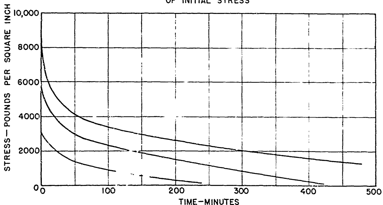
Fig. 22 - Effect of Work Hardening on Relaxation Rate
