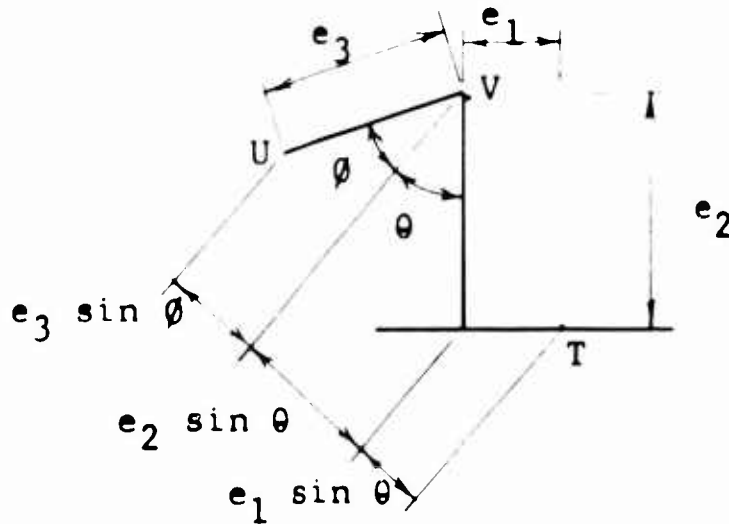
Figure 10 TARGET ERRORS
