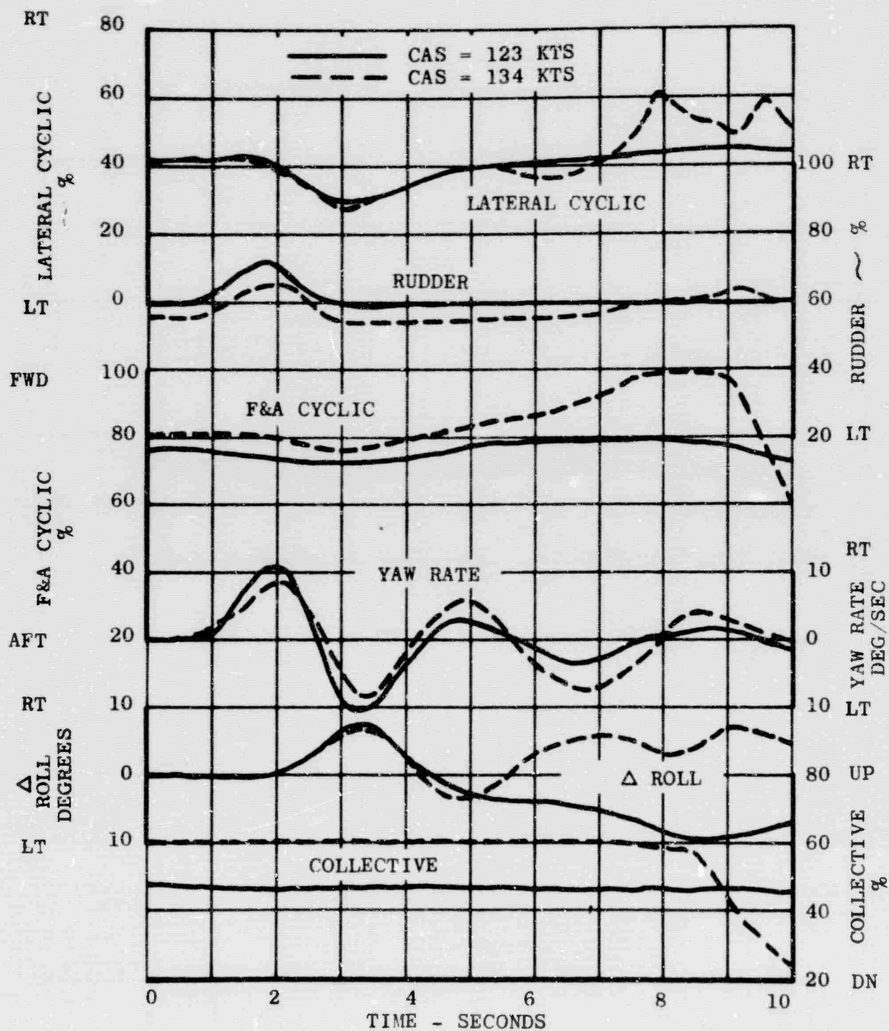
Figure 12. HELICOPTER RESPONSE TO A SIMULATED SIDE GUST FROM THE LEFT, T_J = 800 POUNDS
