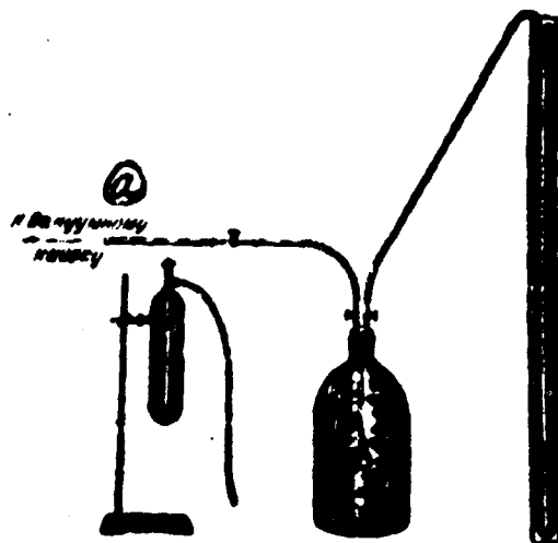
Figure 1. Unit for determining the bactericidal activity of gaseous disinfectants. a. - to the vacuum pump.
