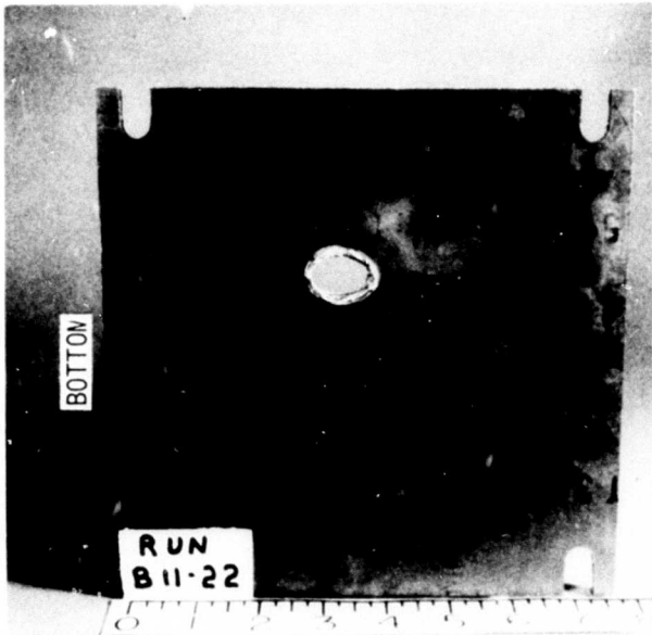
Figure 3 Run 22, 3/16 Inch Diameter Solid Copper Sphere, Oblique Impact at 13,570 Feet/Sec.
