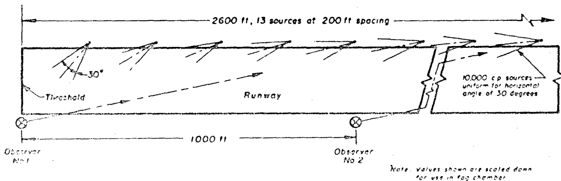
Fig. 10 - Plan view of lights used for determining visual range.
