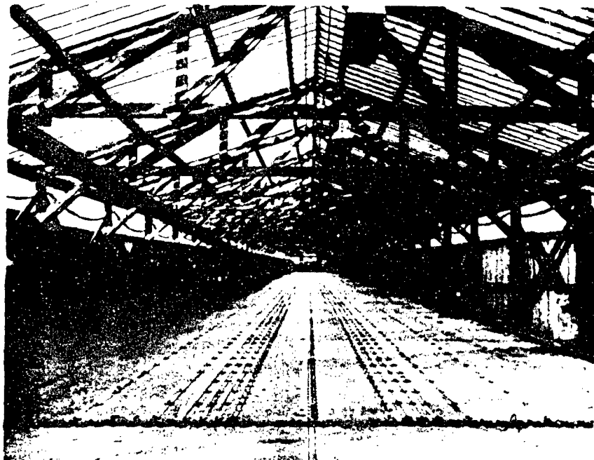
Fig.2 Interior view of fog chamber from threshold showing tramway rails and lighting fixtures. The overhead plastic panels allow low visibility tests to be conducted under day and night conditions.
