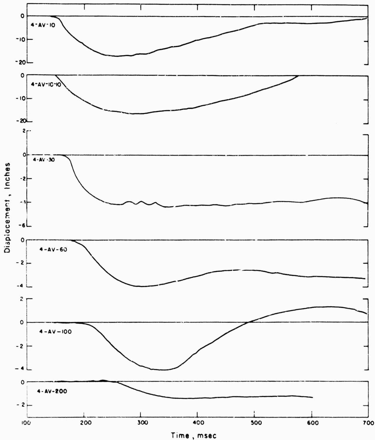
Figure 4.6 Vertical displacement, Station F-1.5-9012.01.
