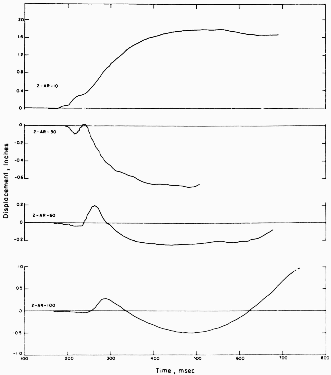
Figure 4.13 Radial displacement, Station F-1.5-9012.02.
