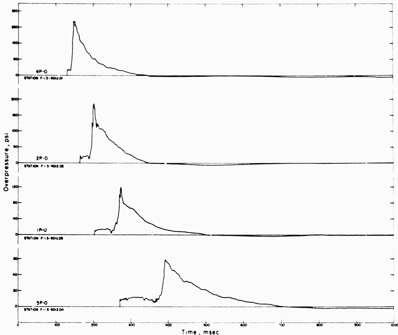
Figure 4.1 Overpressure incident on ground surface, F-1.5-9012 Stations.
