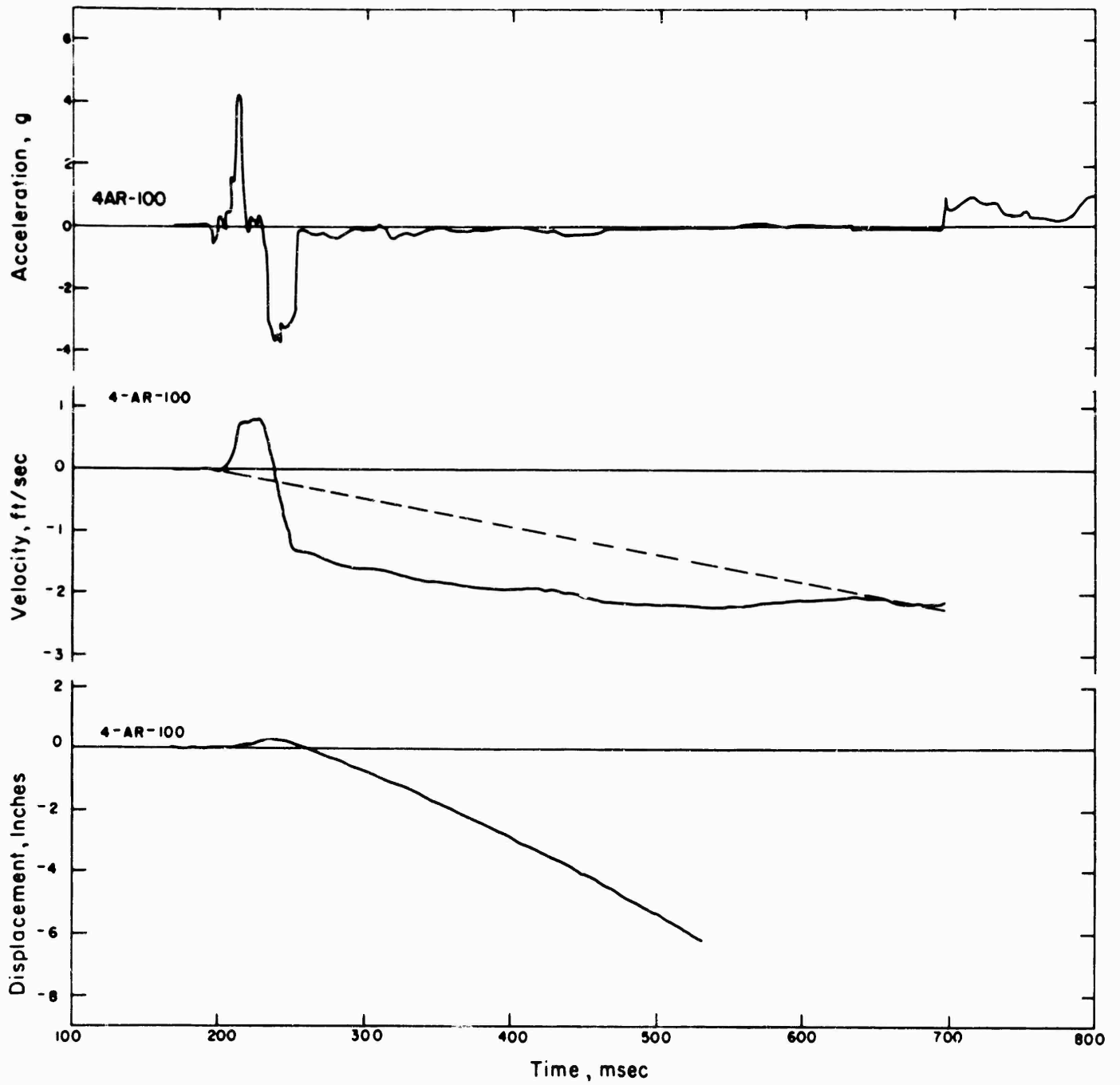
Figure 4.7 Radial acceleration, velocity, and displacement, Station F-1.5-9012.01.
