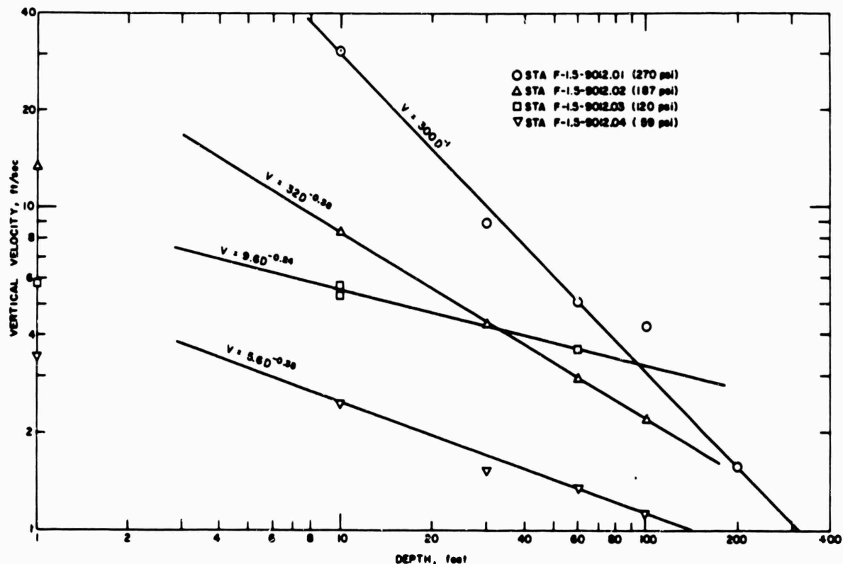
Figure 5.3 Peak vertical particle velocity attenuation.
