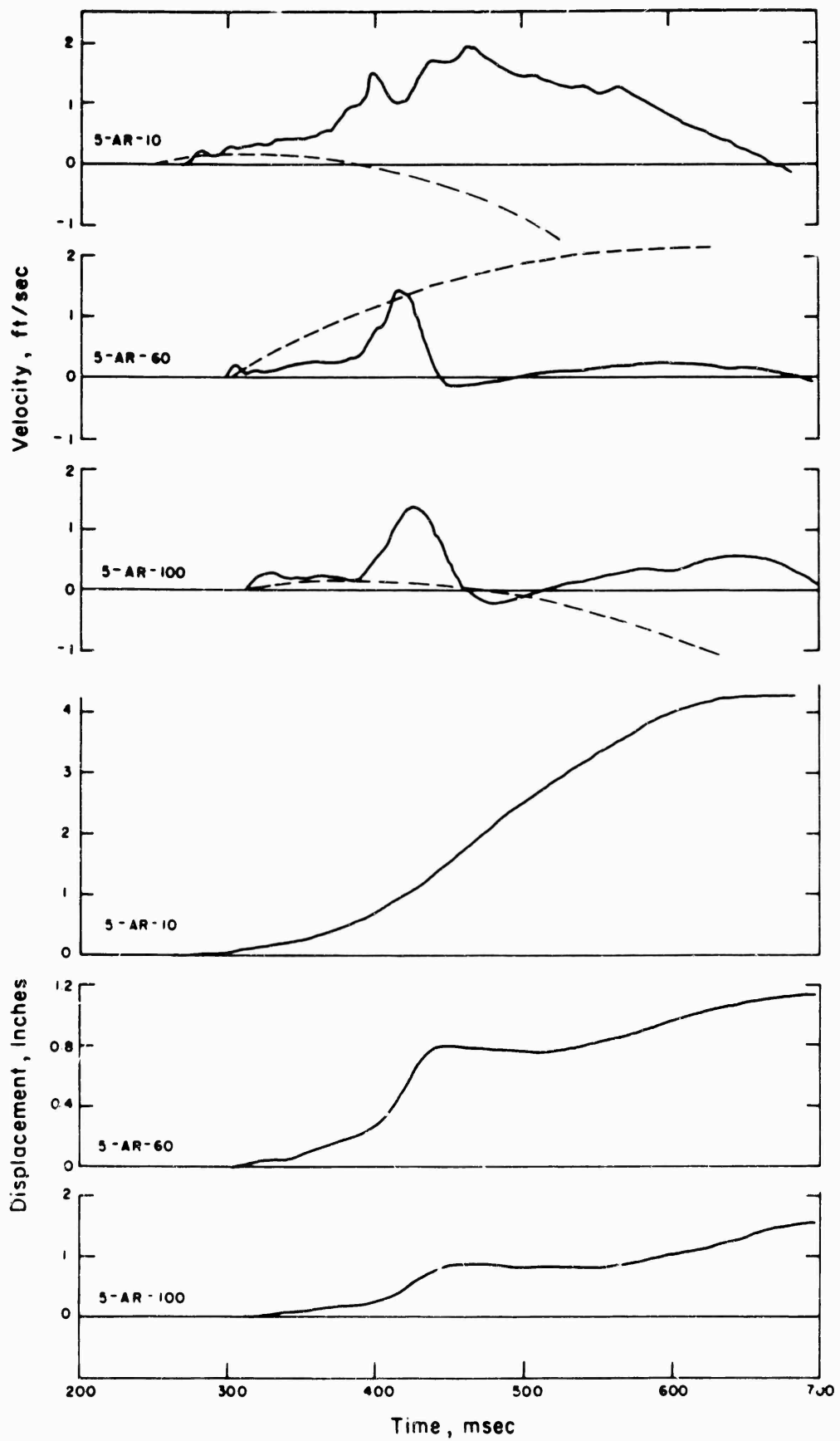
Figure 4.23 Radial velocity and displacement, Station F-1.5-9012.04.
