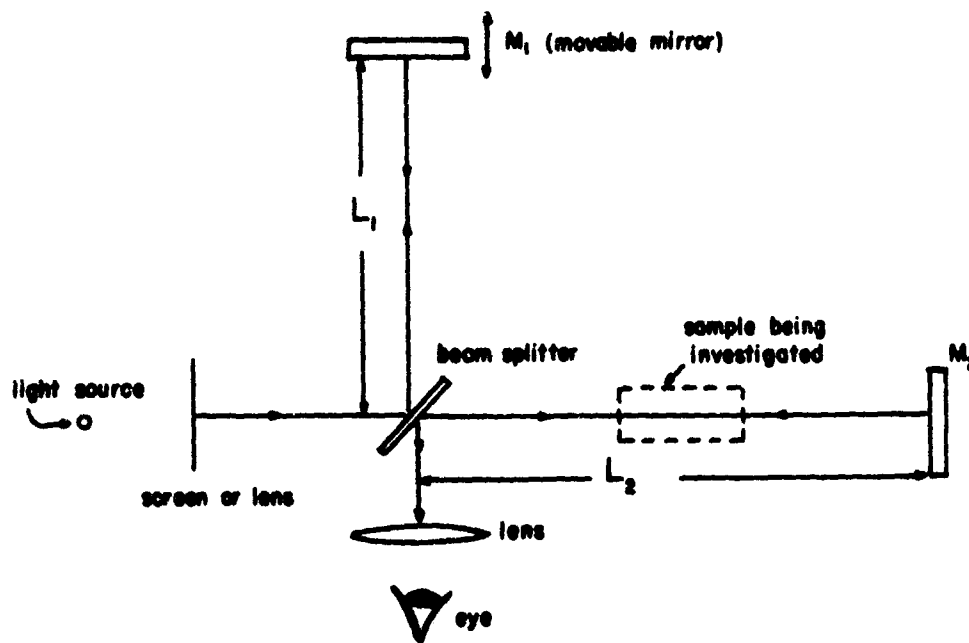
Figure 3.1. Michelson Interferometer
