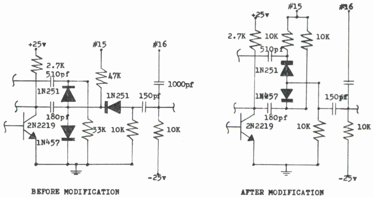
PRECEDENCE CIRCUIT MODIFICATION FIGURE 3.5A
