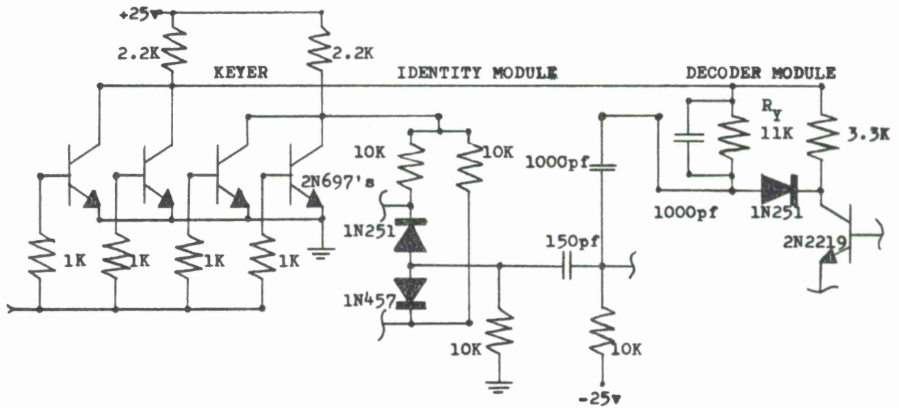
PRECEDENCE CIRCUIT MODIFICATION FIGURE 3.5A
