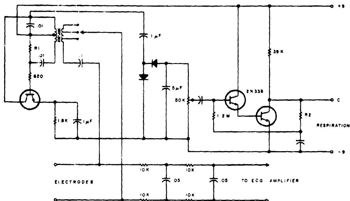
Figure 42. An Impedance Pneumograph for Quantitative Measurement
