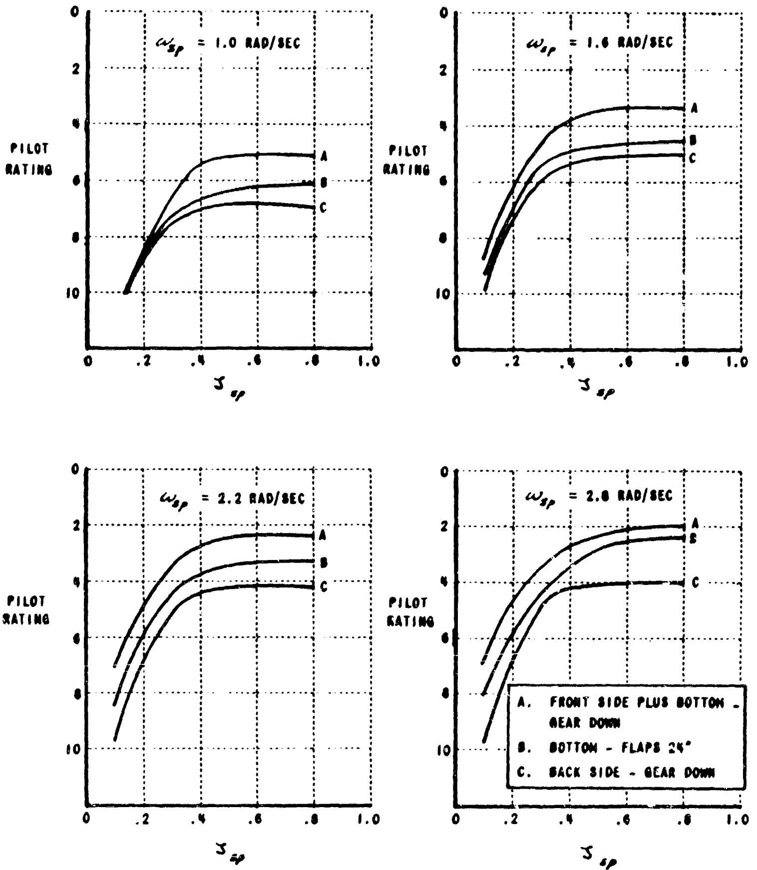
Figure 10 Calculated Pilot Ratings
