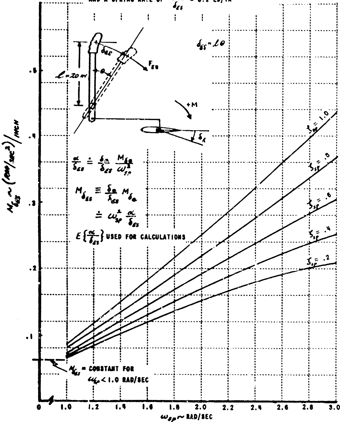
Figure 14 Longitudinal Control Authority Selected by Pilot for Landing Approach Task
