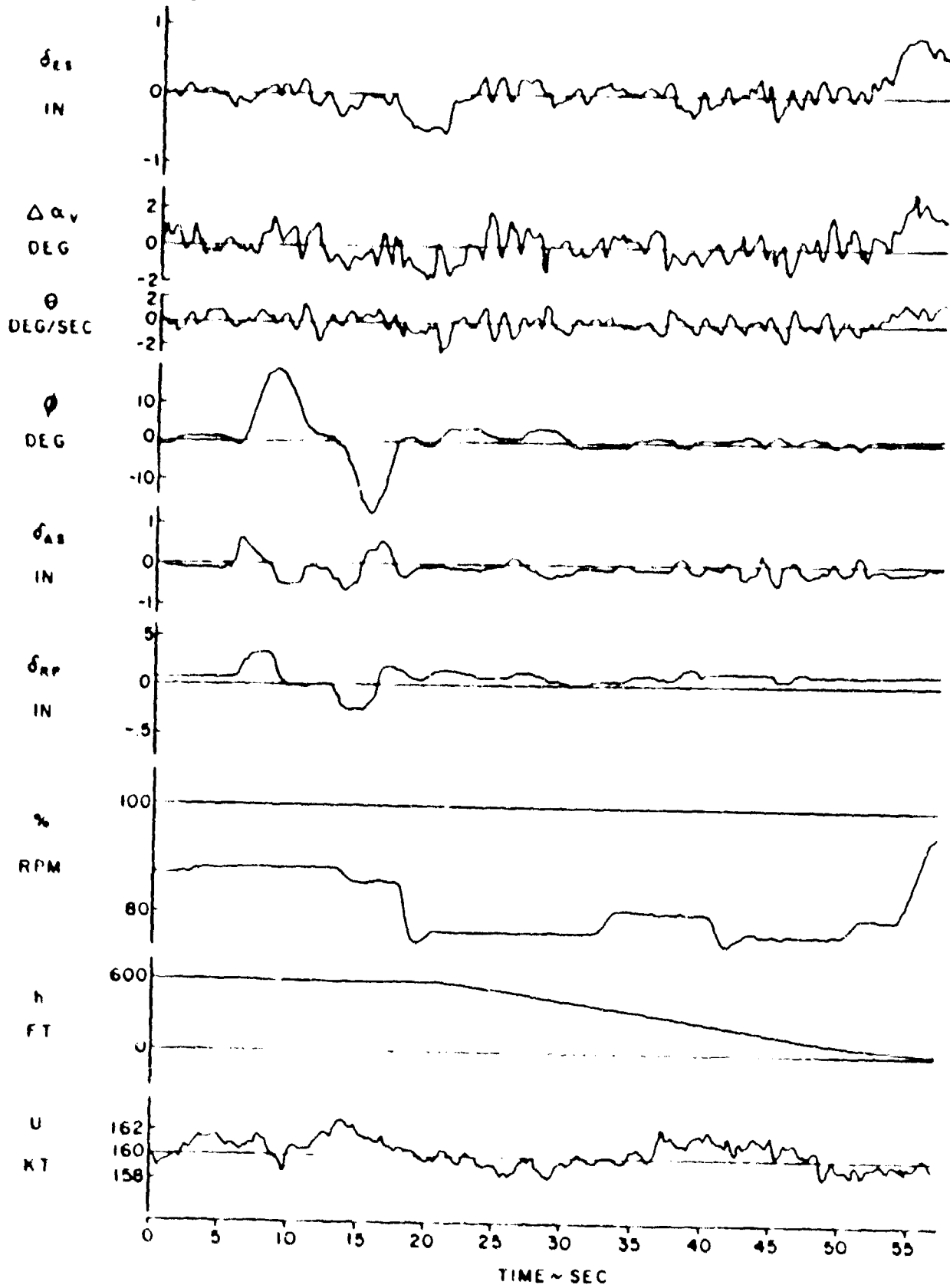
Figure 17 Time Histories of Landing Approaches h. Configuration 2 \frac{1}{2} -73-2 Bottom Flaps, \omega_{sp} = 2.76 Rad/Sec, \zeta_{sp} = .58
