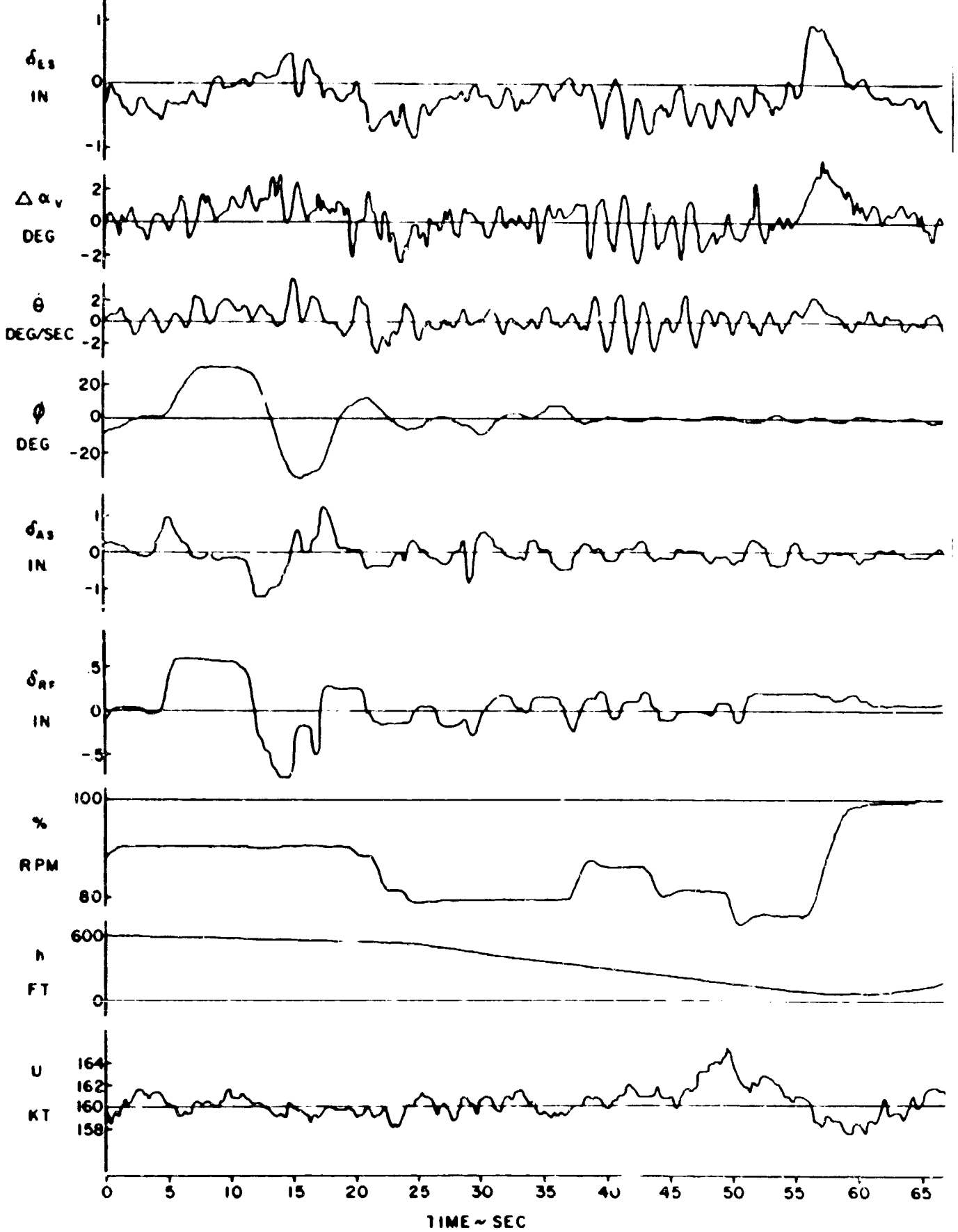
Figure 17 Time Histories of Landing Approaches
