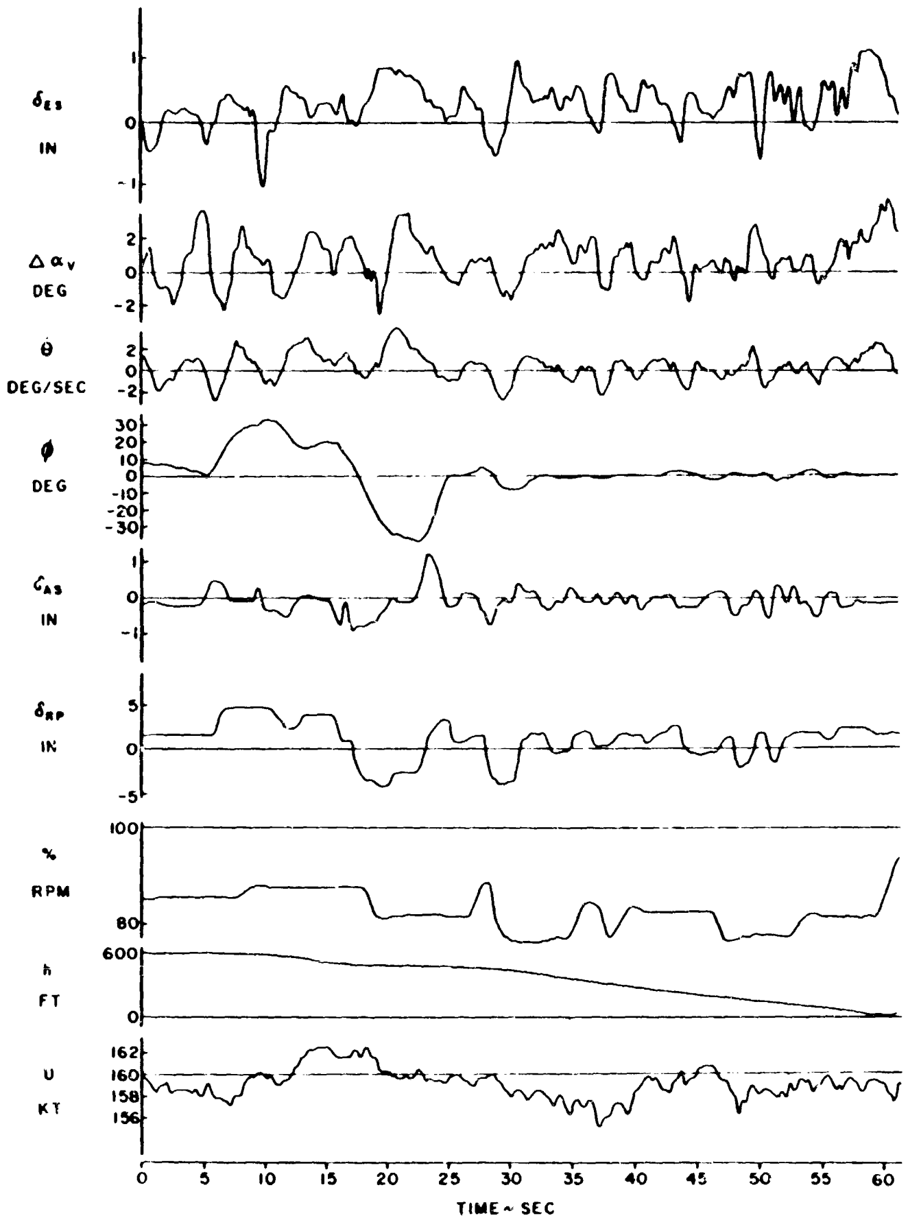
Figure 17 Time Histories of Landing Approaches
