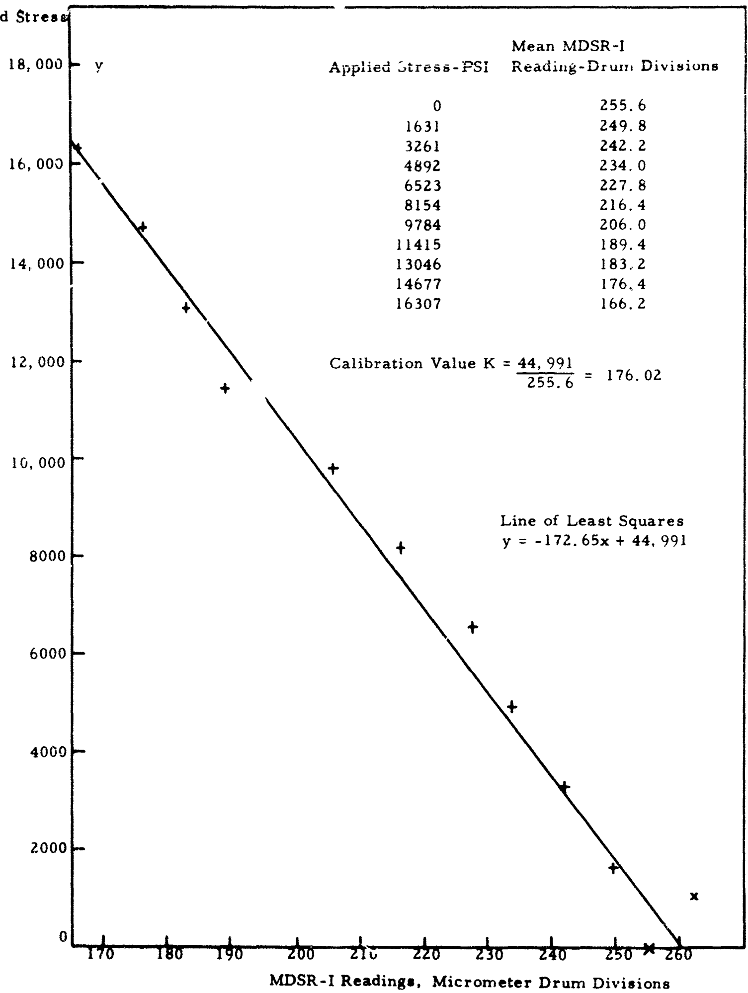
Figure 2 - Representative Calibration Results for Chemcor Glass
