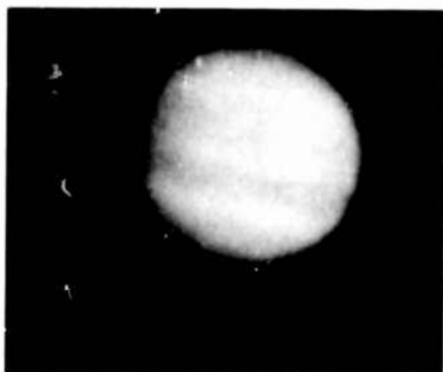
Figure 11. Jupiter, 82-inch telescope, direct photograph exposure 2 sec. same date as Fig. 10. Planet low in sky, seeing poor.
