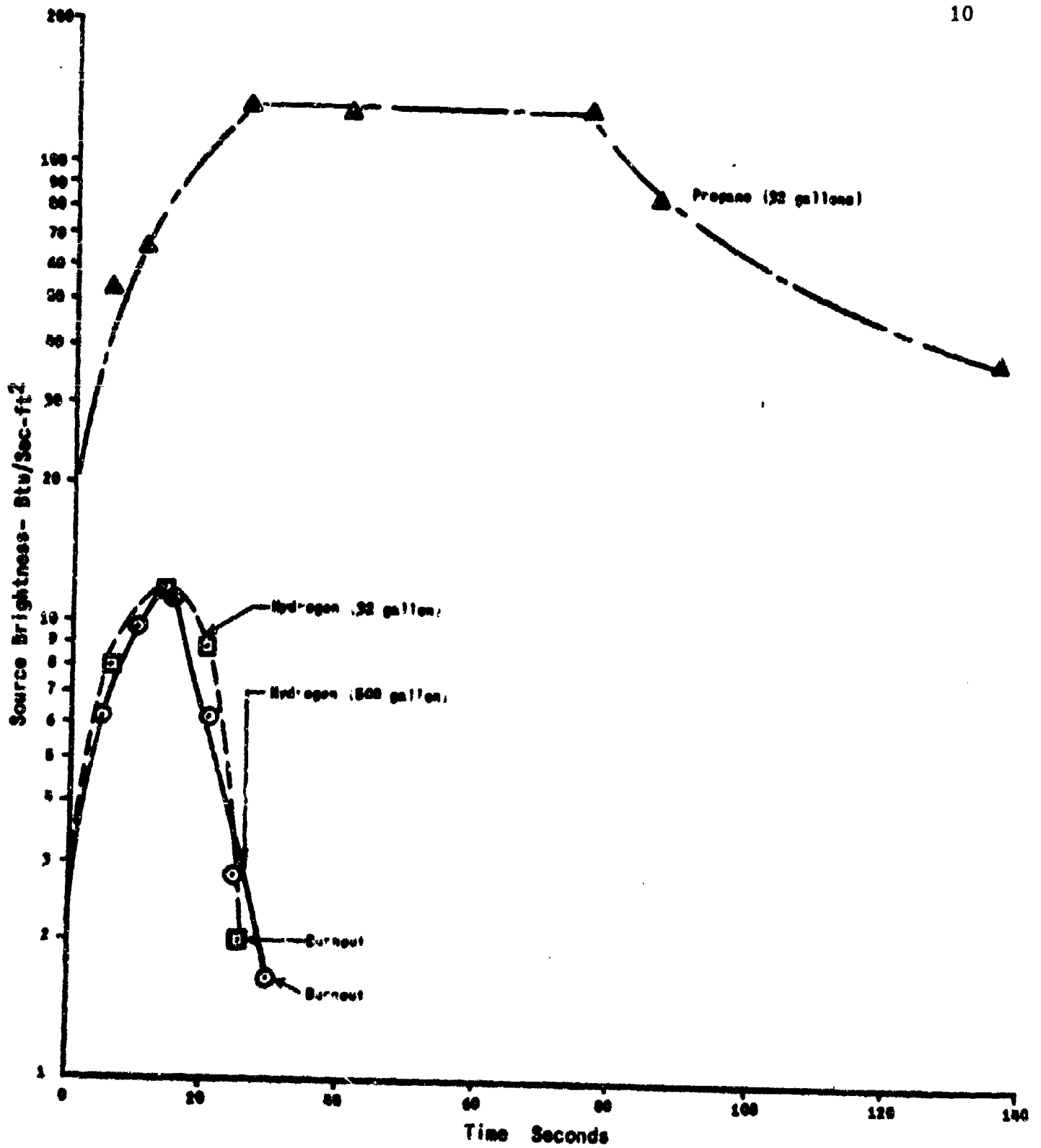
Fig 2 RADIATION FROM FUEL-AIR FLAMES
