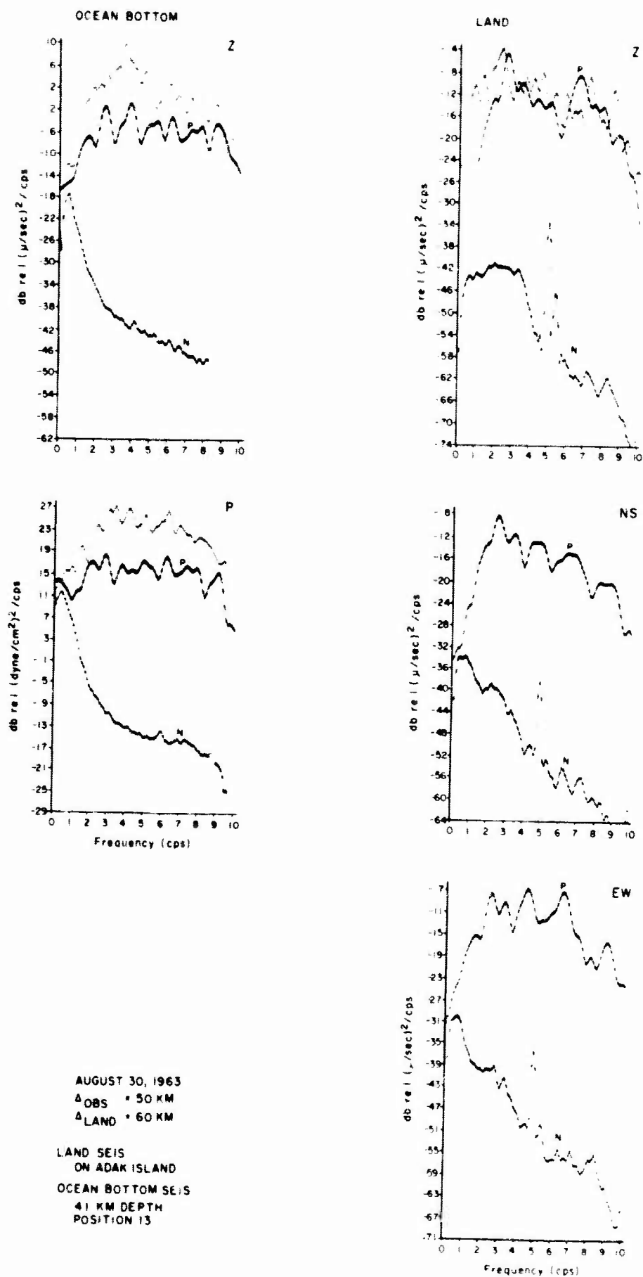
Figure 17. Local Event No. 14 Spectra
