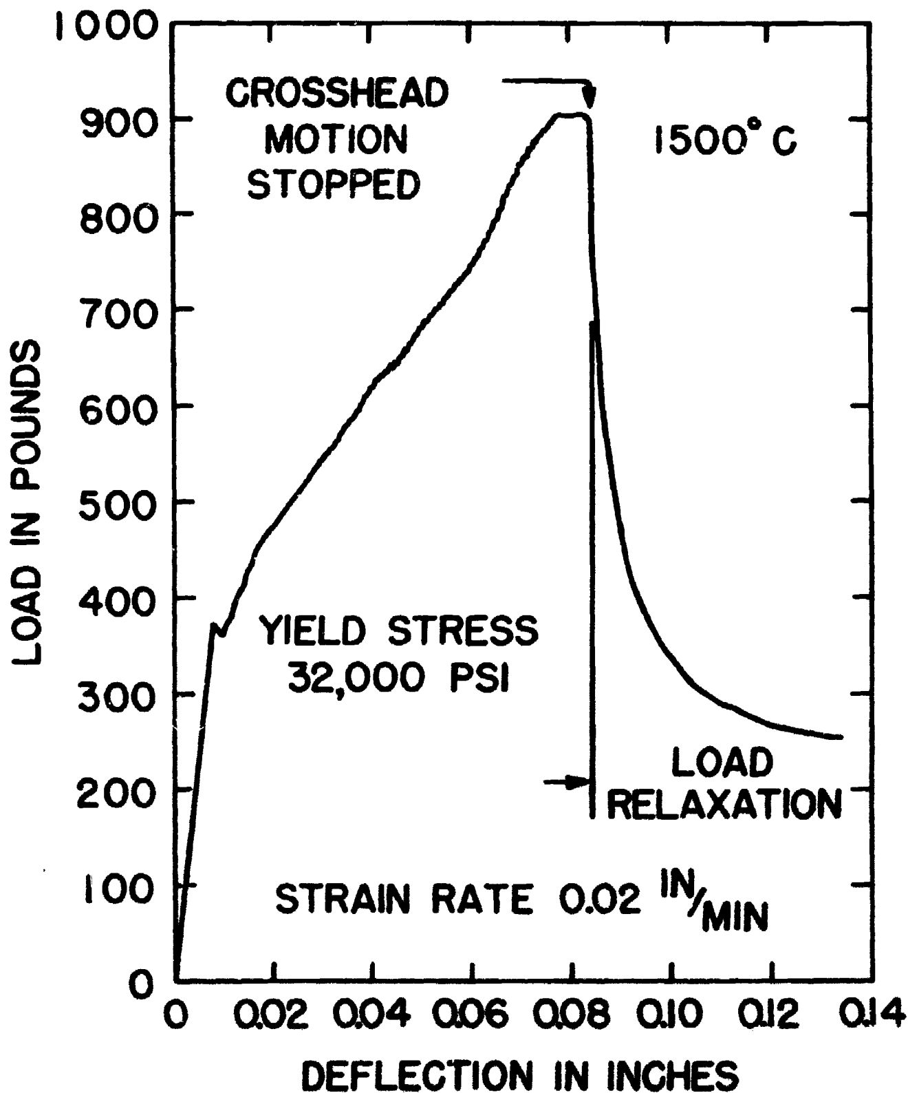
Figure 11. Load versus deflection for alumina-rich spinel single crystal with a [110] load axis tested at 1500°C.
