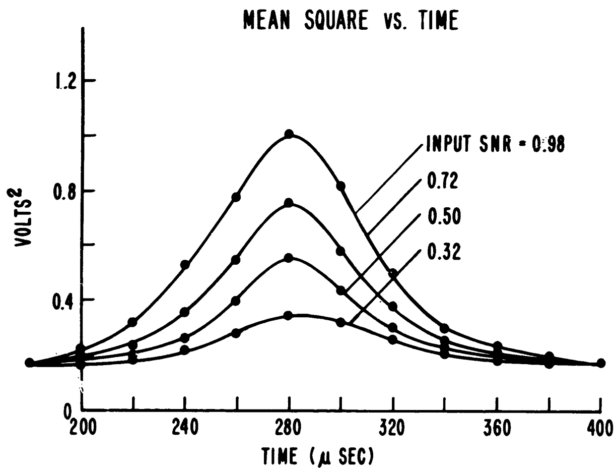
FIG. 22 MEAN SQUARE FOR HALF-WAVE SQUARE LAW DEVICE WITH CONSTANT INPUT NOISE POWER ( \sigma^2 )
