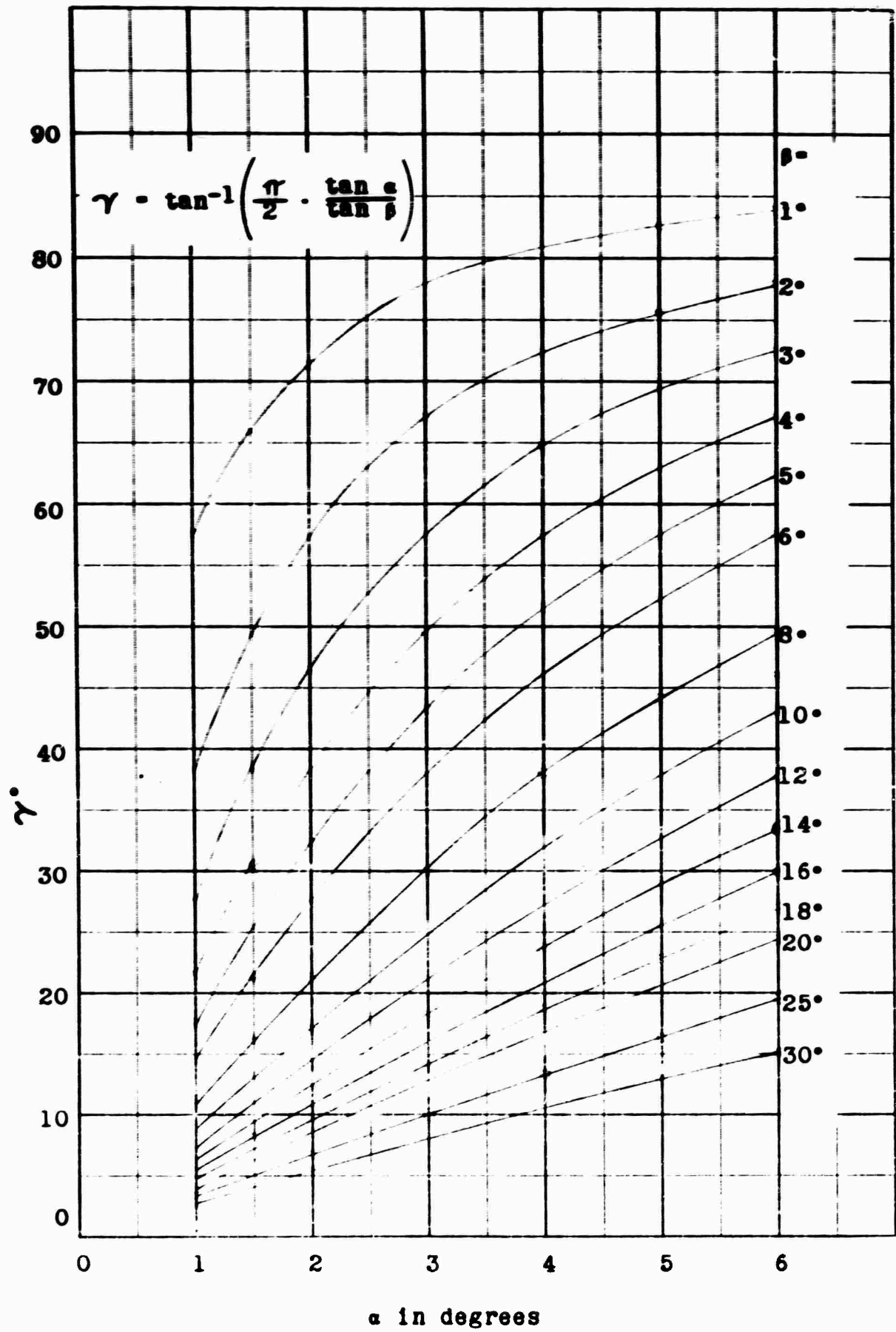
Figure 7 - Angle \gamma between Stagnation Line and Centerline in Plan View.
