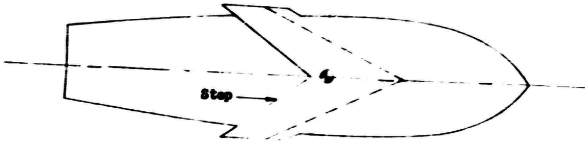
Figure 10a - Local Extensions Added to Planing Bottom (Flat on Bottom and Curved on Top)
