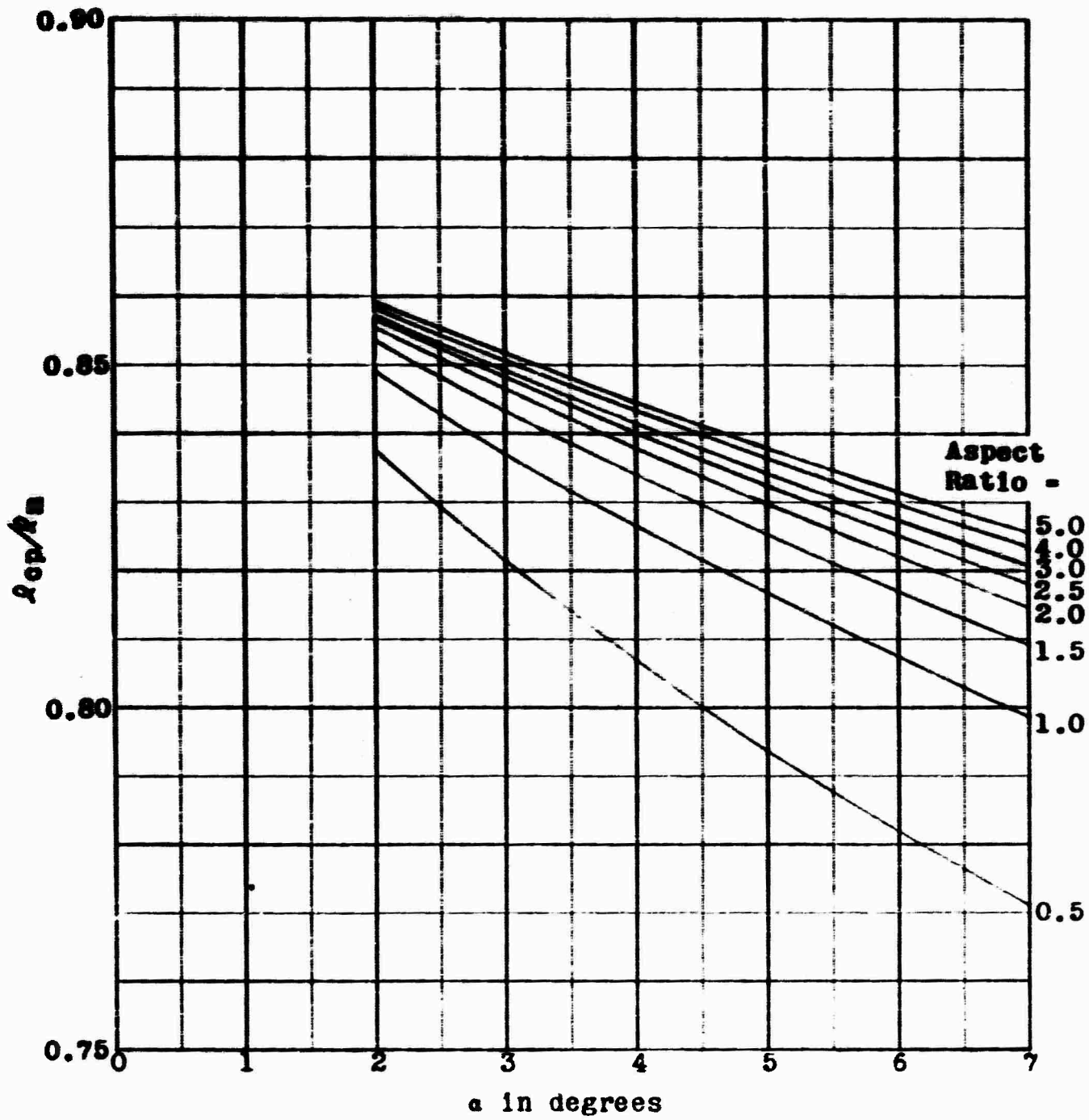
Figure 6 - Center-of-Pressure/Mean-Wetted-Length Ratio versus Angle of Attack for Planing Hulls of Various Aspect Ratios (12.5 Degree Deadrise)
