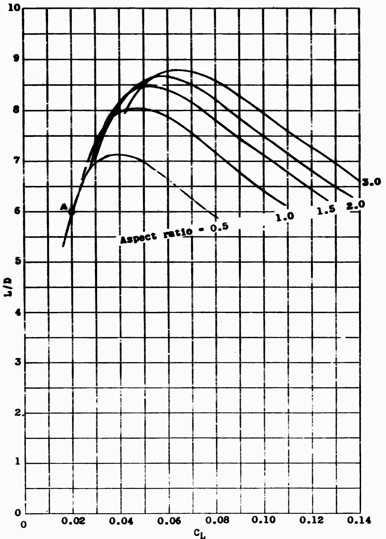
Figure 3 - Lift-Drag Ratio versus Lift Coefficient for Planing Hulls of Various Aspect Ratios (12.5 Degree Deadrise, 0.0004 \Delta C_f )
