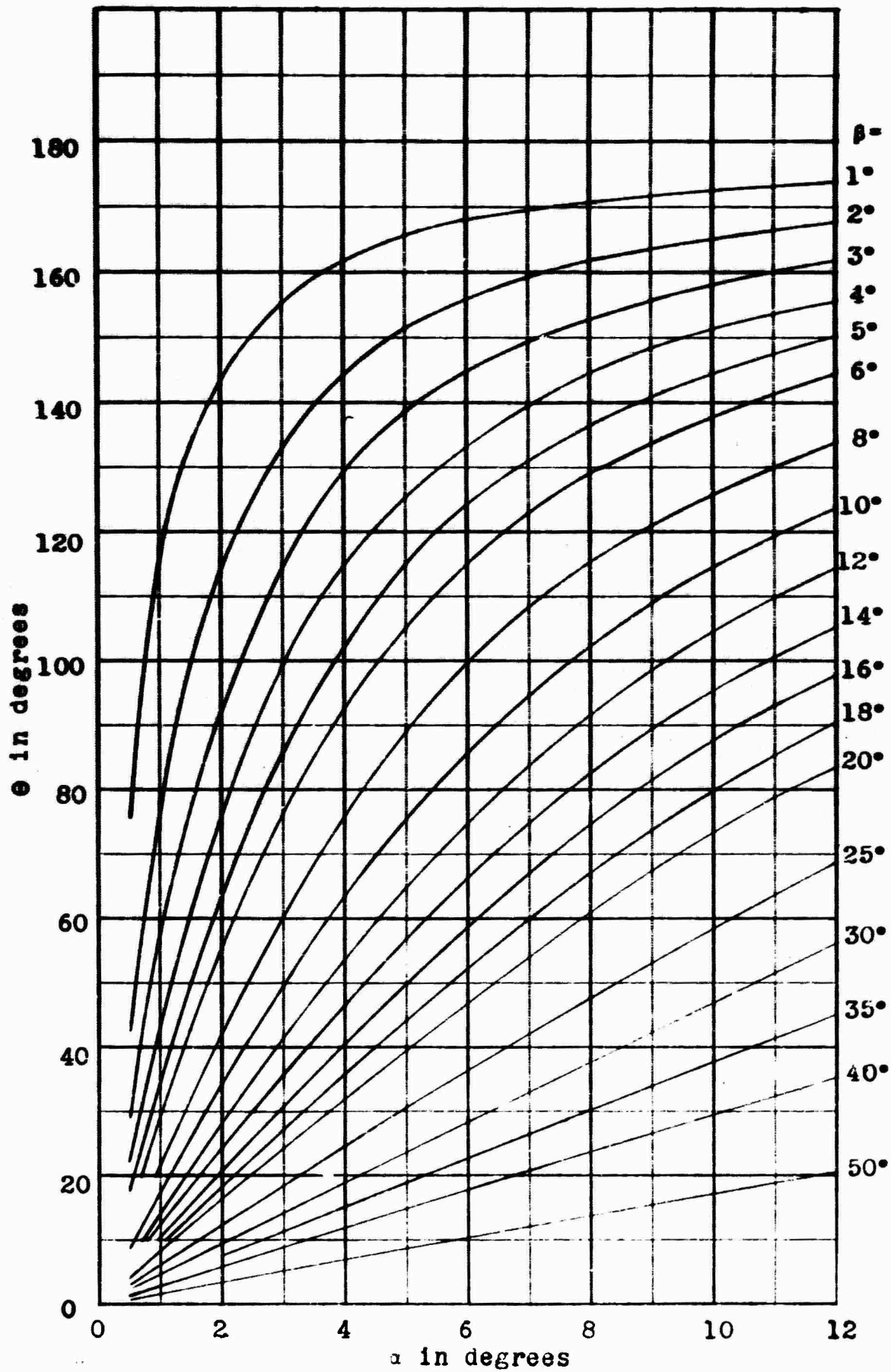
Figure 8 - Angle \theta between Spray Direction and Centerline in Plan View.
