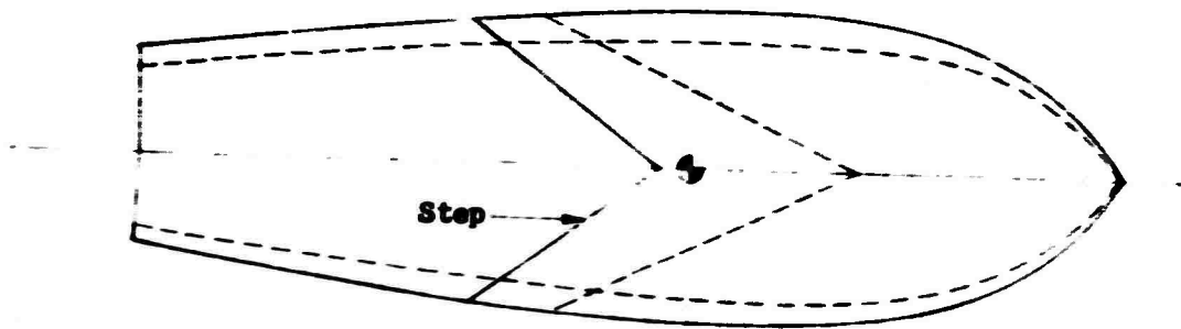
Figure 10b - Chine Width Increased throughout Hull Length
