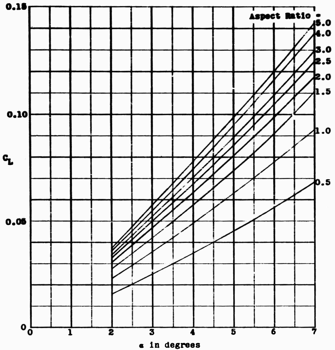
Figure 5 - Lift Coefficient versus Angle of Attack for Planing Hulls of Various Aspect Ratios. (12.5 Degree Deadrise)
