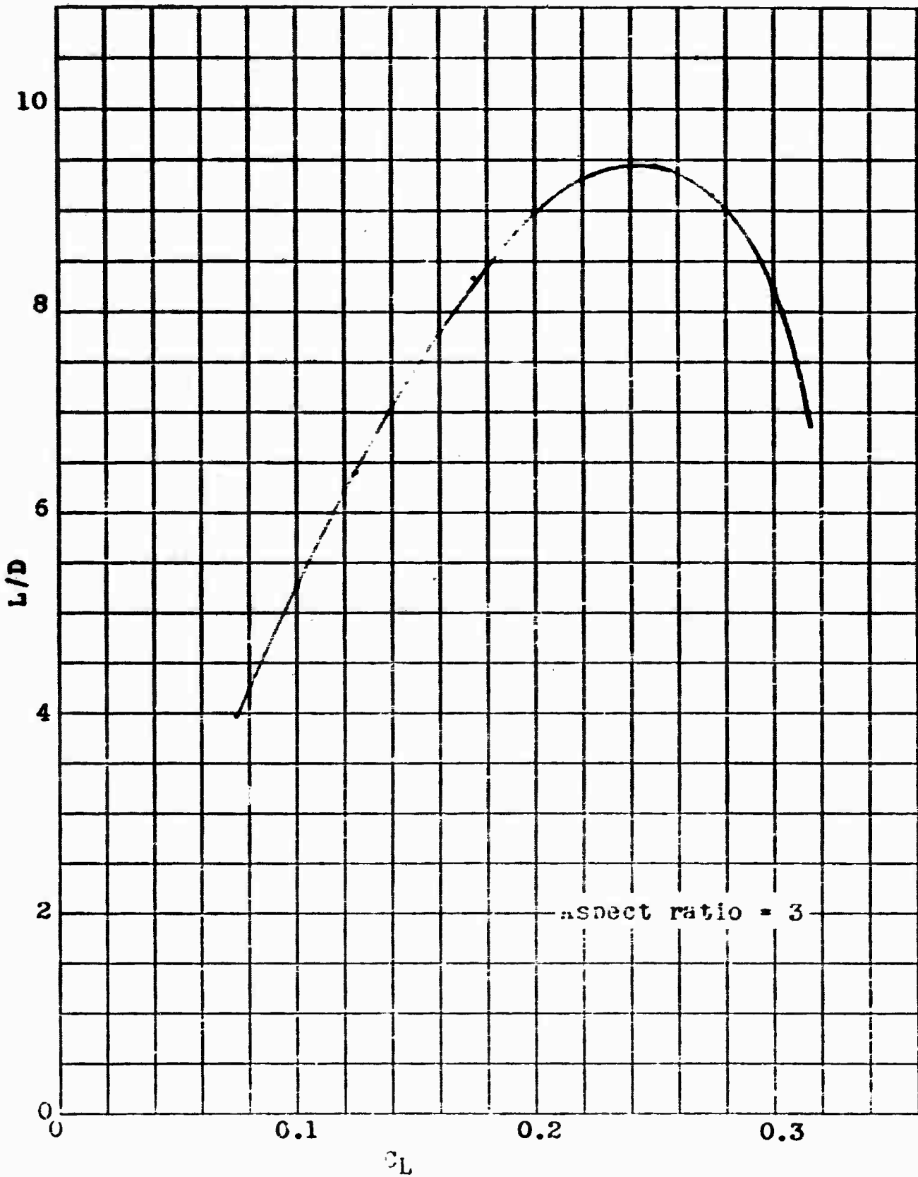
Figure 2 - Lift-Drag Ratio versus Lift Coefficient for a Typical Hydrofoil-Strut-Nacelle Configuration
