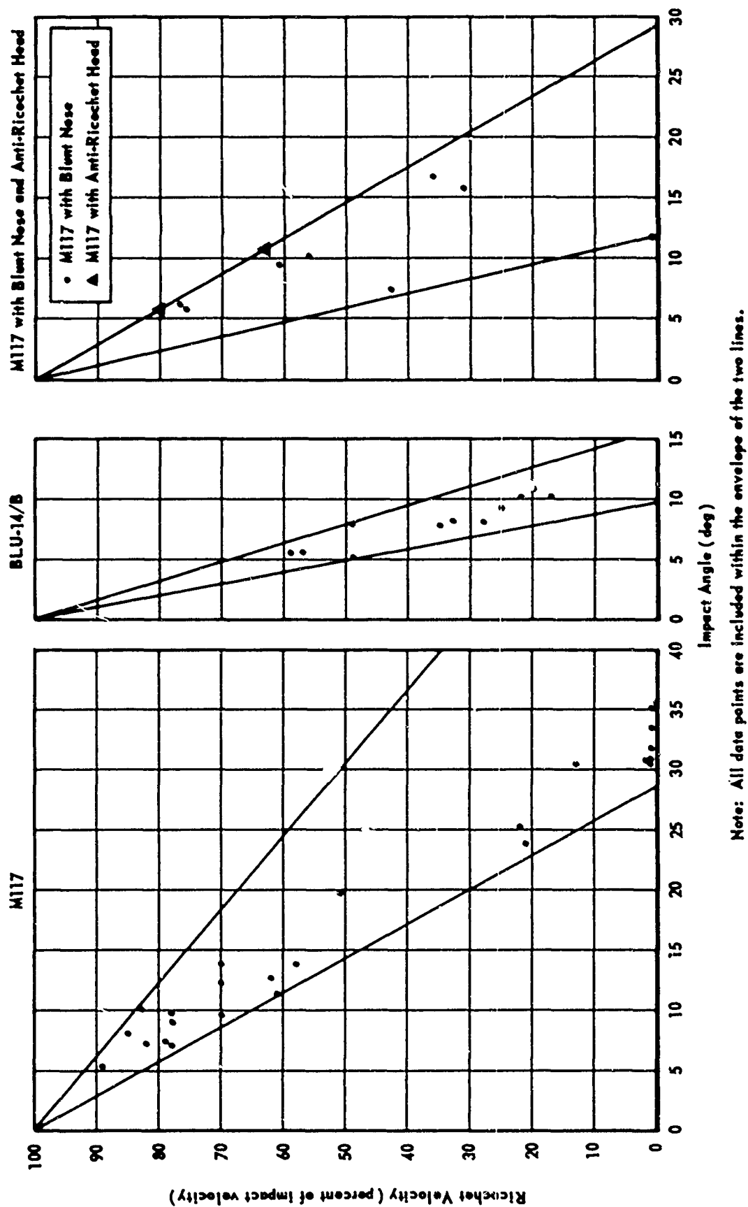
Fig. 9: Relative Ricochet Velocity Versus Impact Angle for Bombs Tested.
