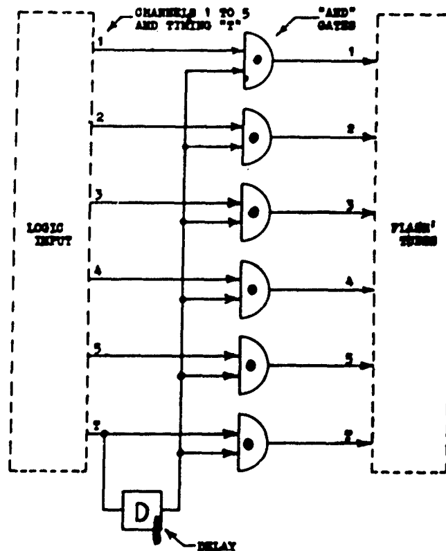
Figure 4-17. Circuit Logic
