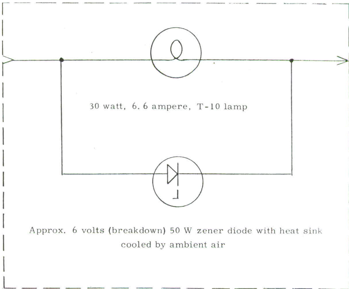
LAMP ASSEMBLY
