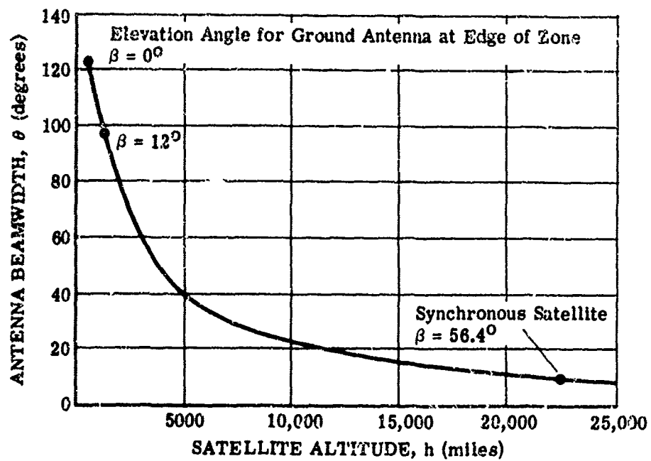
FIGURE 25. SATELLITE ANTENNA BEAMWIDTH FOR COVERAGE OF THE NORTH ATLANTIC REGION. Region based upon a 4000-mile diameter circle centered at 37^\circ\text{W} , 43^\circ\text{N} ; nominal coverage 30^\circ\text{N} to 70^\circ\text{N} and 0^\circ\text{W} to 75^\circ\text{W} .
