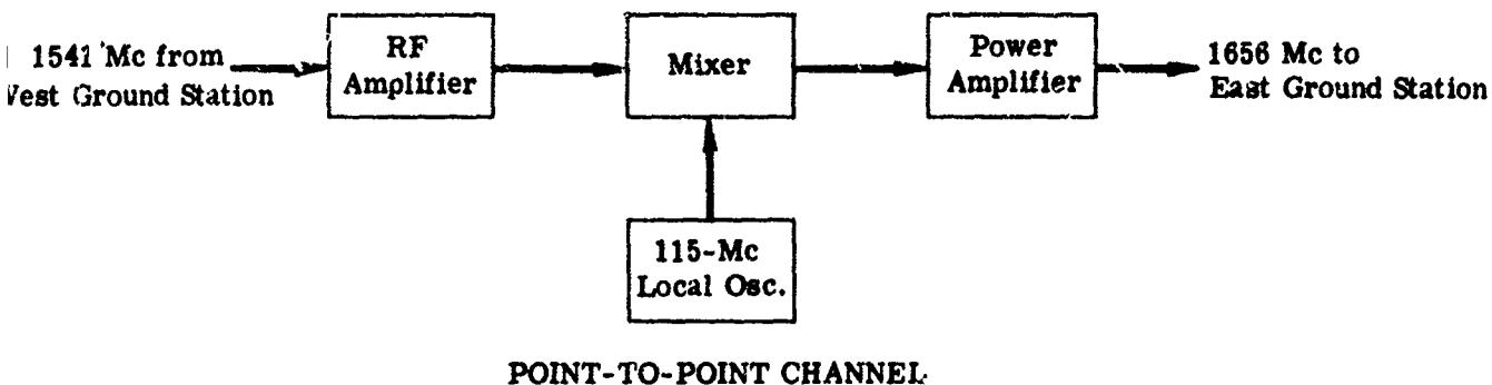
FIGURE 29. FREQUENCY TRANSLATORS
