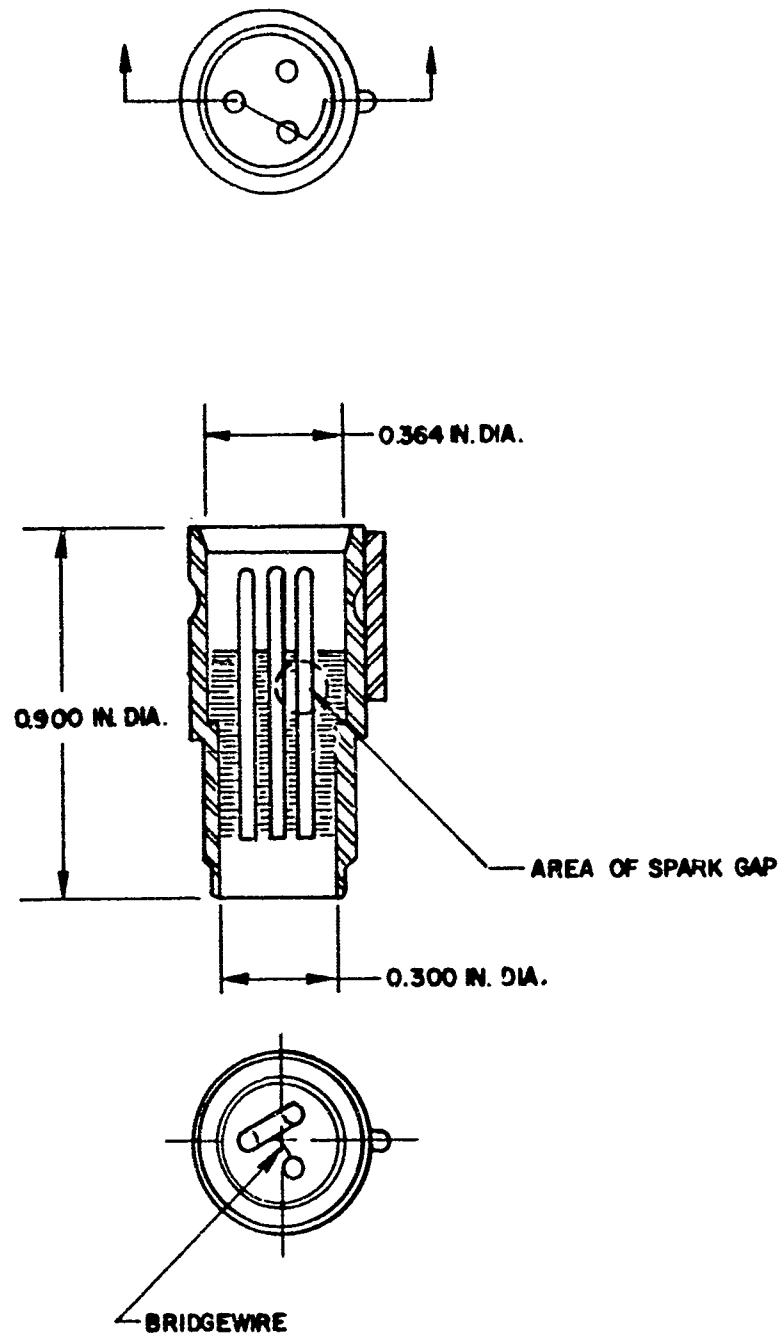
Figure 3. General Design Configuration, NOLC TM 55-80 Initiator.
