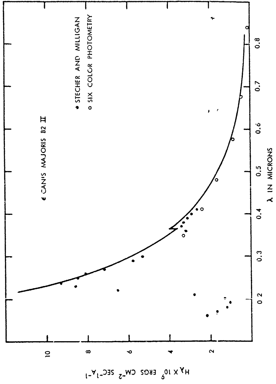
Figure 2. Spectrum of \epsilon Canis Majoris. The solid curve is the model atmosphere of Saito (1956) T_e = 20,400 , \log g = 3.80 .
