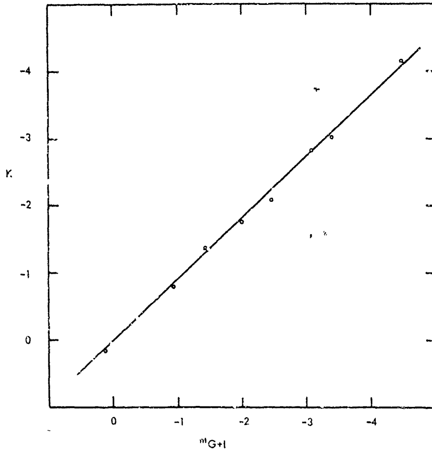
Figure I-8. Comparison of the K Magnitude of Johnson with m_{G+I} of Lunn.
