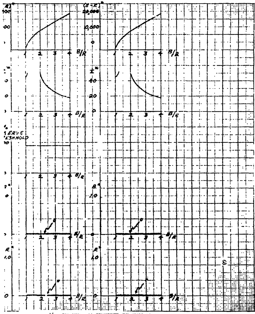
Figure 10 TWO DIMENSIONAL PLOT OF THE STANDARD CASE FIRE POWER
