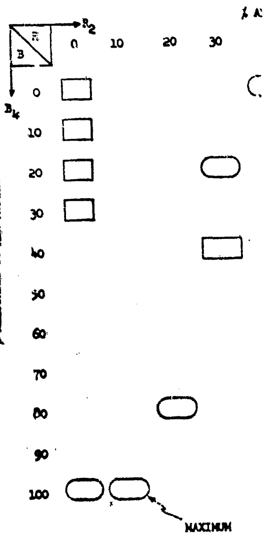
Figure 8. Game Theoretic Solution - Three-Player Case
