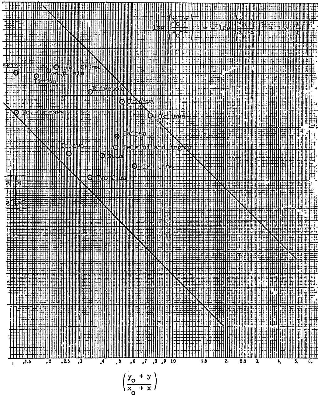
Figure 4. CASUALTY VS. AVERAGE FORCE DURING BATTLE (ON BOTH SIDES) RATIOS FOR WORLD WAR II PACIFIC ISLAND CAMPAIGNS
