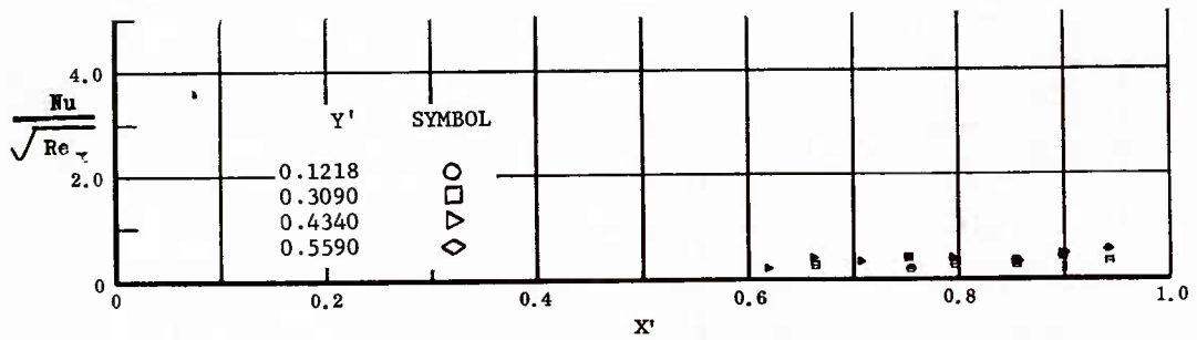
Fig. 41 Streamwise Distributions of Aerodynamic Heating Rates; Basic Configuration, No Flap Deflections, \alpha = 0^\circ , \beta = +12^\circ , Re_\infty/ft = 3,300,000 .
