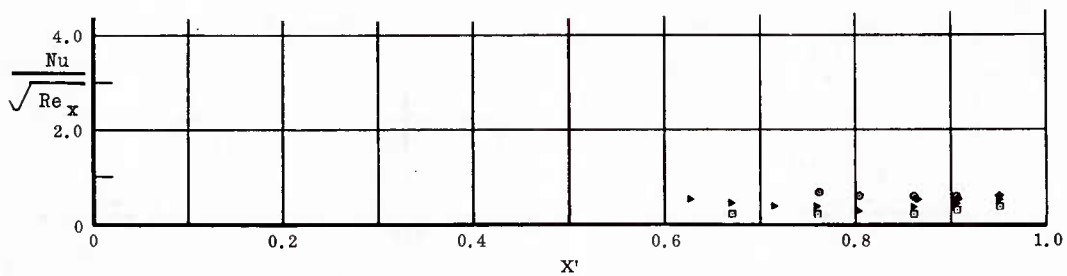
Fig. 23 Streamwise Distributions of Aerodynamic Heating Rates; Basic Configuration + Canards, Left and Right (Upper) Flaps Deflected -20^\circ , \alpha = 0^\circ , \beta = 0^\circ , Re_\infty/ft = 3,300,000 .
