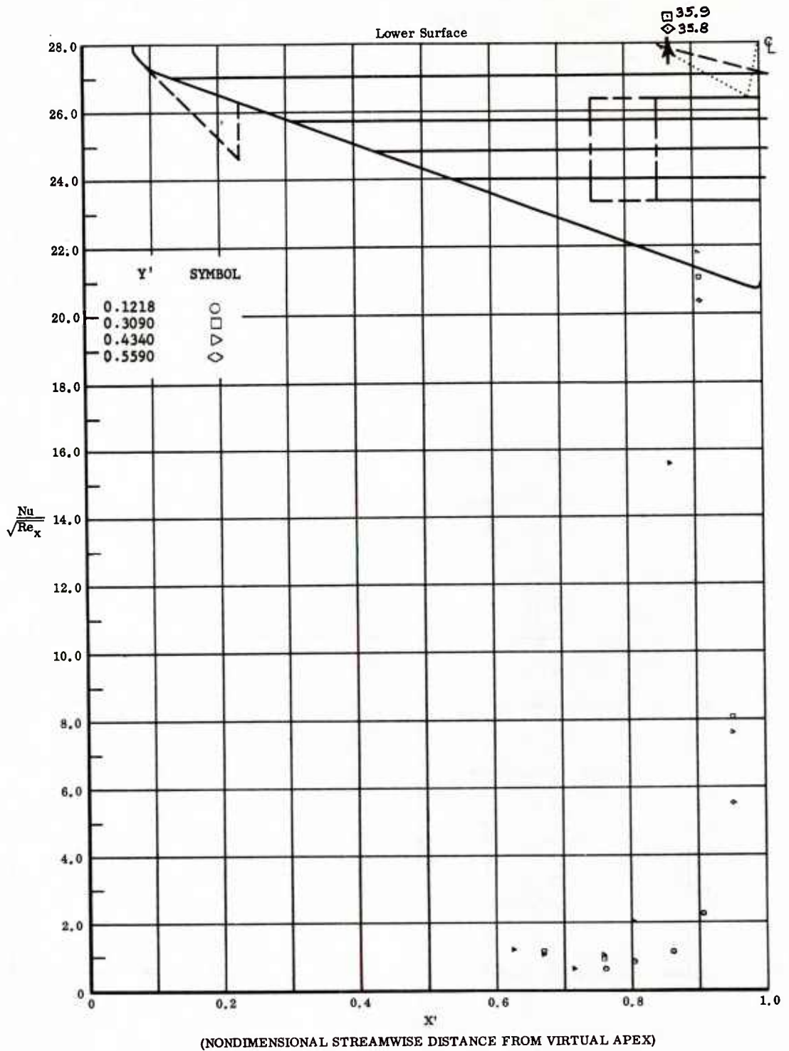
Fig. 69 Streamwise Distributions of Aerodynamic Heating Rates; Basic Configuration, Bottom Flaps Deflected +40°, \alpha = +14.3^\circ , \beta = 0^\circ , Re_\infty/ft = 1,100,000 .
