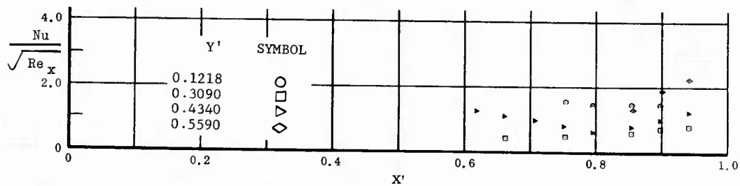
Fig. 17 Streamwise Distributions of Aerodynamic Heating Rates; Basic Configuration + Canards, Left and Right (Upper) Flaps Deflected -40^\circ , \alpha = 0^\circ , \beta = 0^\circ , Re_\infty/ft = 3,300,000 .
