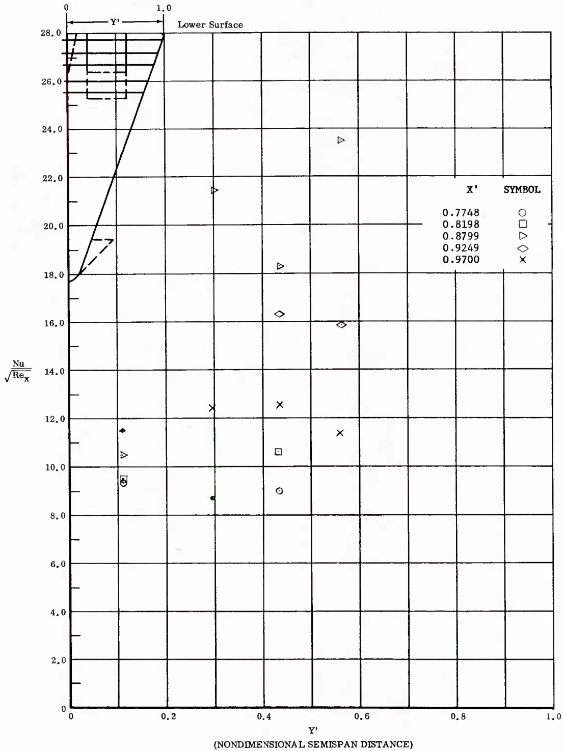
Fig. 78 Spanwise Distributions of Aerodynamic Heating Rates; Basic Configuration, Bottom Flaps Deflected +20°, \alpha = +45^\circ , \beta = 0^\circ , Re_\infty/ft = 3,300,000 .
