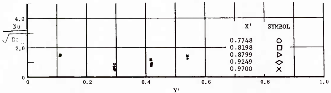
Fig. 27 Spanwise Distribution of Aerodynamic Heating Rates; Basic Configuration + Canards, No Flap Deflections, \alpha = 0^\circ , \beta = 0^\circ , Re_\infty/ft = 3,300,000 .
