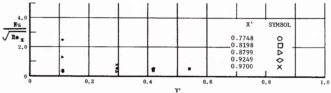
Fig. 43 Spanwise Distributions of Aerodynamic Heating Rates; Basic Configuration + Fin ( \delta = 0 ), No Flap Deflections, \alpha = 0^\circ , \beta = +12^\circ , Re_\infty/ft = 3,300,000 .
