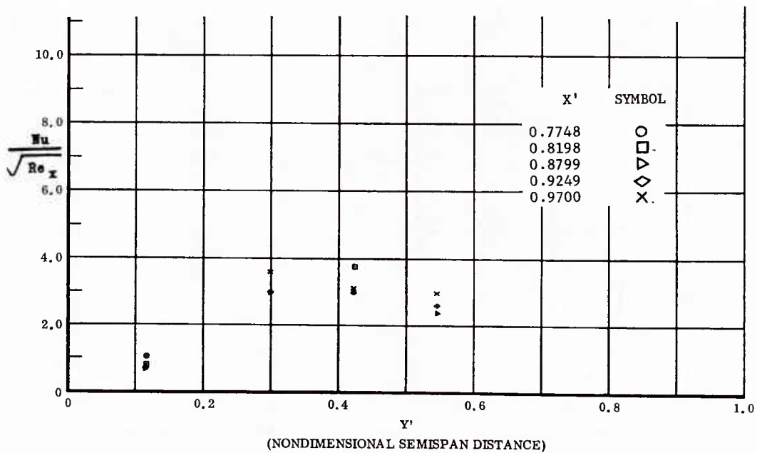
Fig. 36 Spanwise Distributions of Aerodynamic Heating Rates; Basic Configuration + Longer Chord Flaps, Bottom Flaps Deflected +20°, \alpha = 0^\circ , \beta = 0^\circ , Re_\infty/ft = 3,300,000 .
