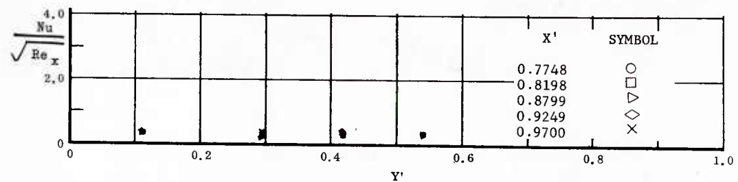
Fig. 8 Spanwise Distributions of Aerodynamic Heating Rates; Basic Configuration, Left and Right (Upper) Flaps Deflected -20^\circ , \alpha = -45^\circ , \beta = 0^\circ , Re_\infty/ft = 3,300,000 .
