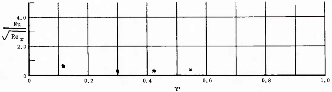
Fig. 16 Spanwise Distributions of Aerodynamic Heating Rates; Basic Configuration, Right (Upper) Flap Deflected -40^\circ , \alpha = 0^\circ , \beta = 0^\circ , Re_\infty/ft = 3,300,000 .
