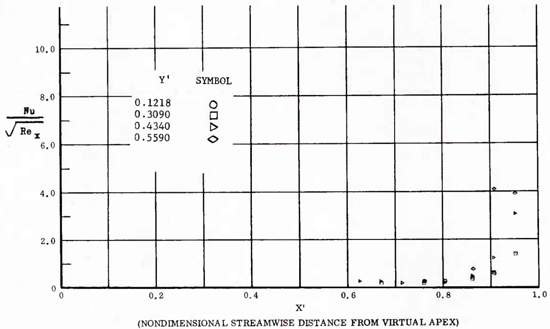
Fig. 31 Streamwise Distributions of Aerodynamic Heating Rates; Basic Configuration, Bottom Flaps Deflected +20°, \alpha = 0^\circ , \beta = 0^\circ , Re_\infty/ft = 1,100,000 .
