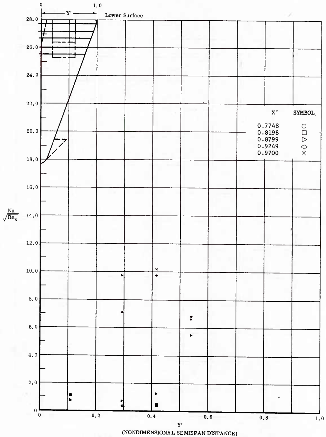
Fig. 37 Spanwise Distributions of Aerodynamic Heating Rates; Basic Configuration, Bottom Flaps Deflected +30°, \alpha = 0^\circ , \beta = 0^\circ , Re_\infty/ft = 3,300,000 .
