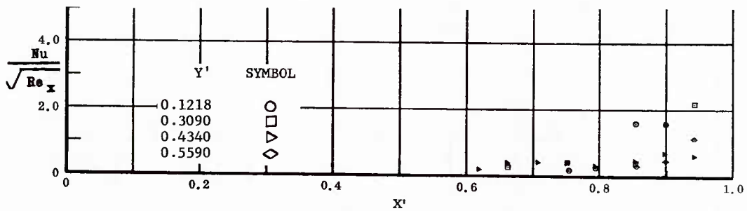
Fig. 44 Streamwise Distributions of Aerodynamic Heating Rates; Basic Configuration + Fin ( \delta = 15^\circ ), No Flap Deflections, \alpha = 0^\circ , \beta = +12^\circ , Re_\infty/ft = 3,300,000
