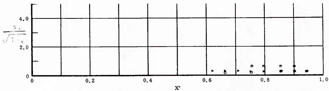
Fig. 24 Streamwise Distributions of Aerodynamic Heating Rates; Basic Configuration, Left and Right (Upper) Flaps Deflected -10^\circ , \alpha = 0^\circ , \beta = 0^\circ , Re_\infty/ft = 3,300,000 .
