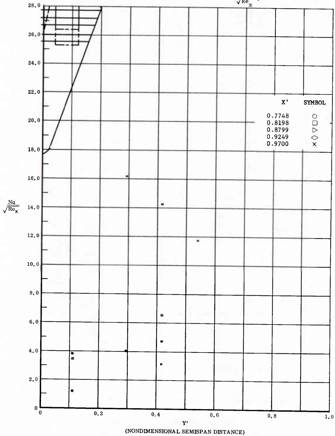
Fig. 70 Spanwise Distributions of Aerodynamic Heating Rates; Basic Configuration, Bottom Flaps Deflected +40°, \alpha = +14.3^\circ , \beta = 0^\circ , Re_\infty/ft = 3,300,000 .
