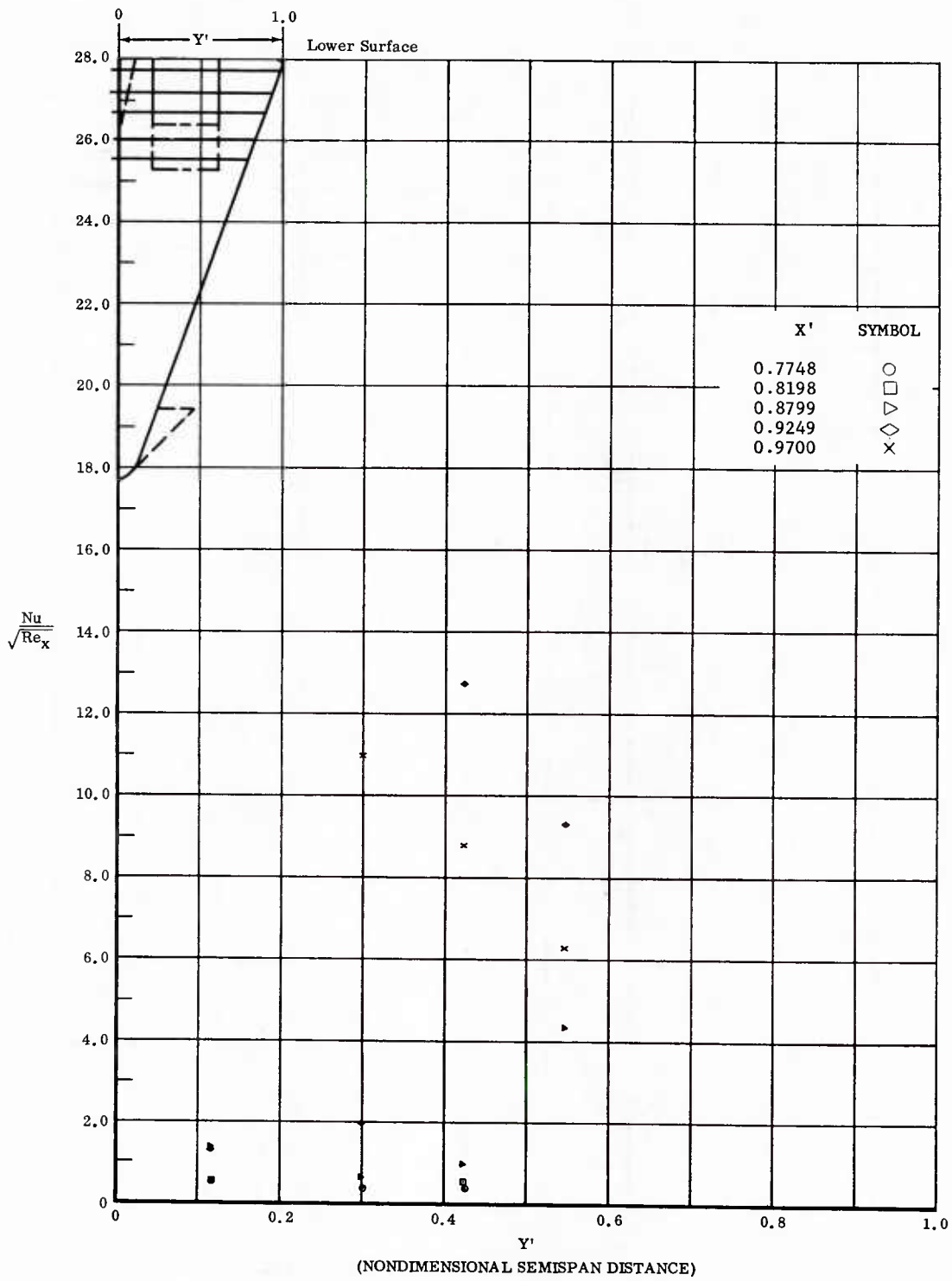
Fig. 38 Spanwise Distributions of Aerodynamic Heating Rates; Basic Configuration, Bottom Flaps Deflected +40°, \alpha = 0^\circ , \beta = 0^\circ , Re_\infty/ft = 1,100,000 .
