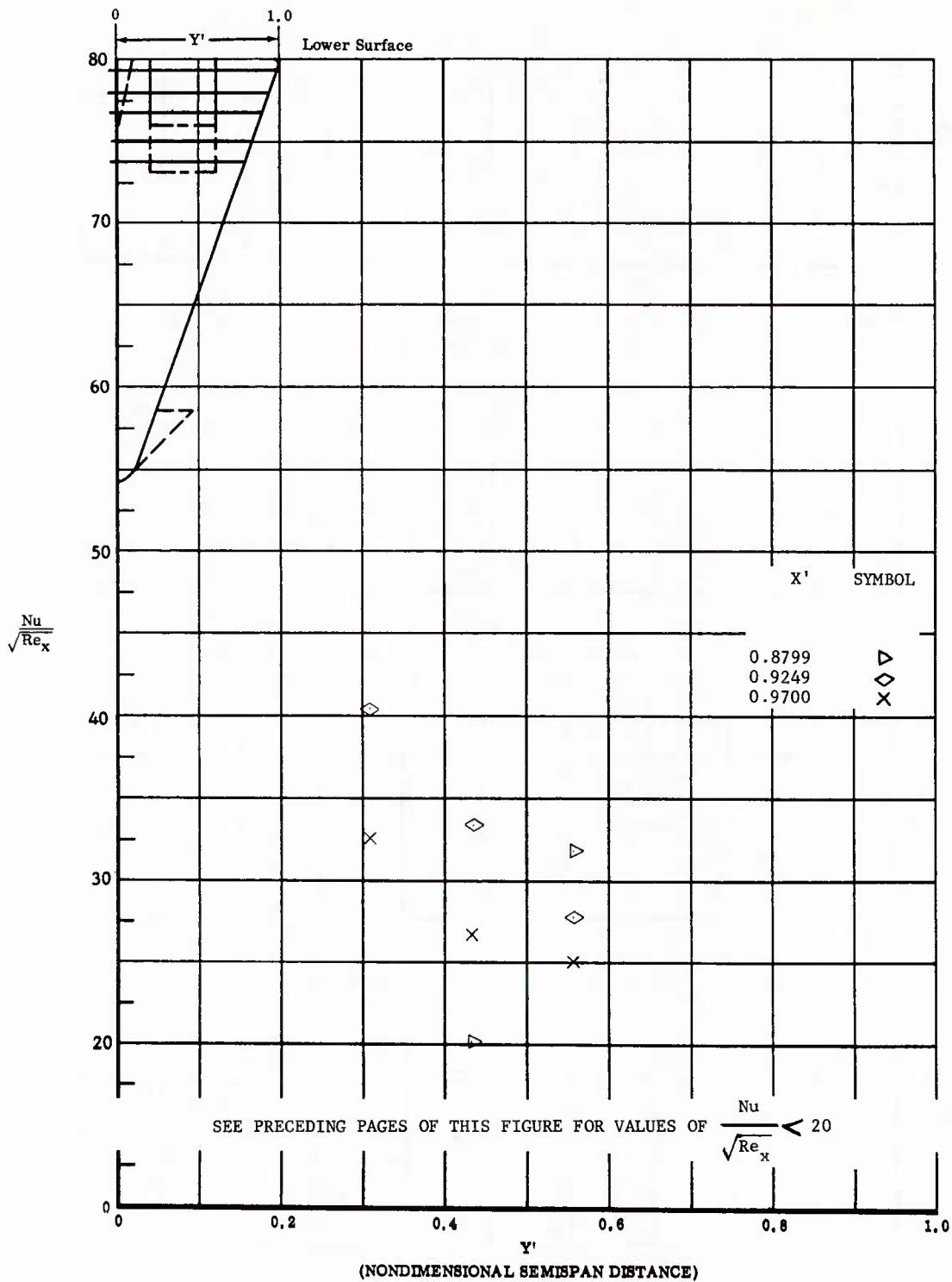
Fig. 40 Spanwise Distributions of Aerodynamic Heating Rates; Basic Configuration + Canards, Bottom Flaps Deflected +40°, \alpha = 0^\circ , \beta = 0^\circ , Re_\infty / ft = 3,300,000 .
