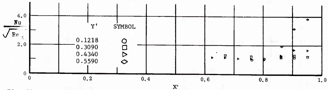
Fig. 50 Streamwise Distributions of Aerodynamic Heating Rates; Basic Configuration, Right (Upper) Flap Deflected -40^\circ , \alpha = +14.3^\circ , \beta = 0^\circ , Re_\infty/ft = 3,300,000 .
