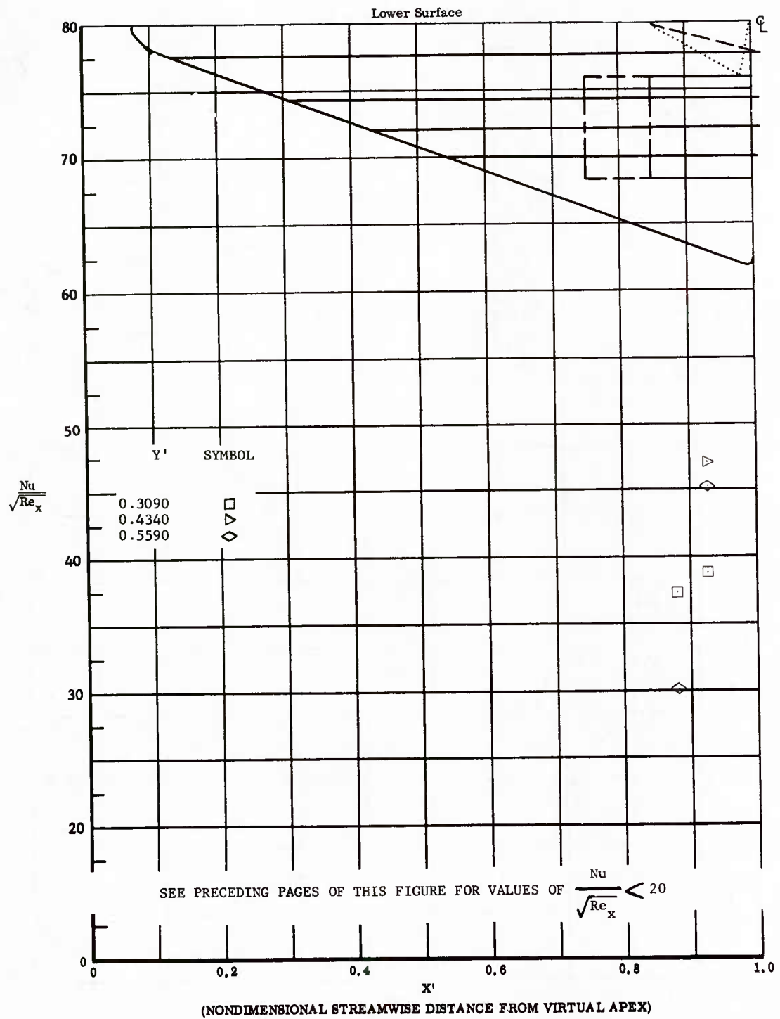
Fig. 70 Streamwise Distributions of Aerodynamic Heating Rates; Basic Configuration, Bottom Flaps Deflected +40^\circ , \alpha = +14.3^\circ , \beta = 0^\circ , Re_\infty/ft = 3,300,000 .
