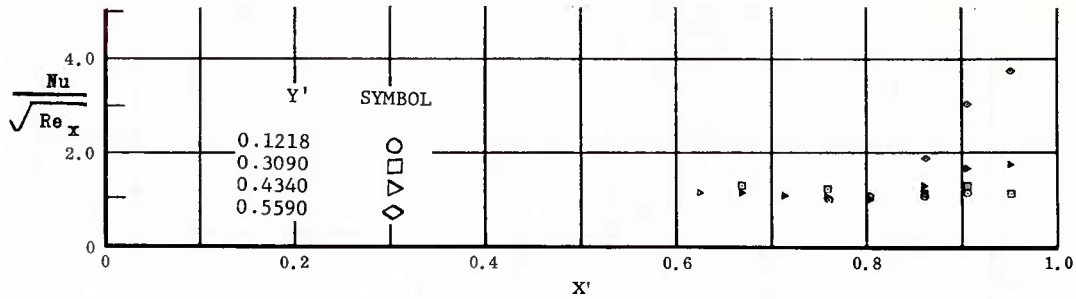
Fig. 49 Streamwise Distributions of Aerodynamic Heating Rates; Basic Configuration, Left (Upper) Flap Deflected -40^\circ , \alpha = +14.3^\circ , \beta = 0^\circ , Re_\infty/ft = 3,300,000 .
