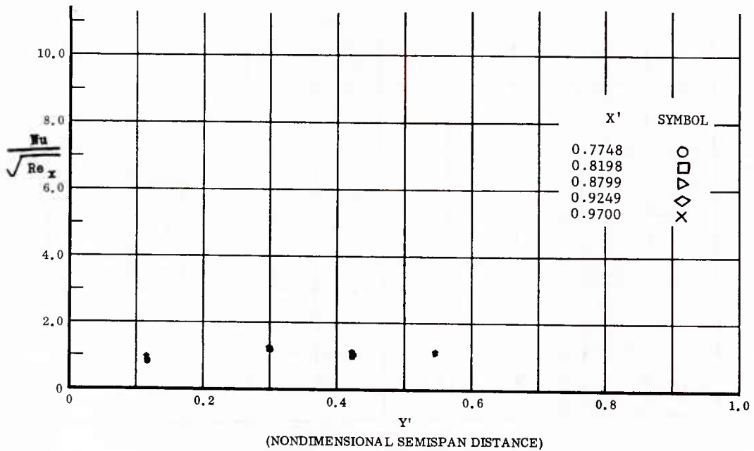
Fig. 59 Spanwise Distributions of Aerodynamic Heating Rates; Basic Configuration, No Flap Deflections, \alpha = +14.3^\circ , \beta = 0^\circ , Re_\infty/ft = 1,100,000 .
