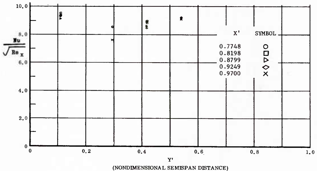
Fig. 76 Spanwise Distributions of Aerodynamic Heating Rates; Basic Configuration, Left and Right (Upper) Flaps Deflected -40^\circ , \alpha = +45^\circ , \beta = 0^\circ , Re_\infty/ft = 3,300,000 .
