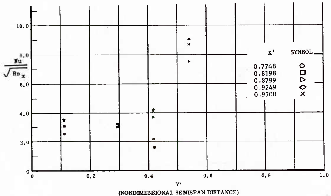
Fig. 57 Spanwise Distributions of Aerodynamic Heating Rates; Basic Configuration + Canards, Left and Right (Upper) Flaps Deflected -20^\circ , \alpha = +14.3^\circ , \beta = 0^\circ , Re_\infty/ft = 3,300,000 .
