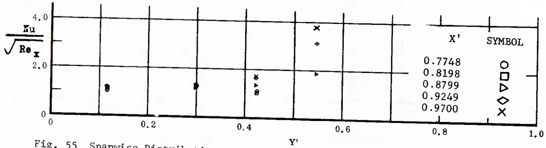
Fig. 55 Spanwise Distributions of Aerodynamic Heating Rates; Basic Configuration, Left (Upper) Flap Deflected -20^\circ , \alpha = +14.3^\circ , \beta = 0^\circ , Re_\infty/ft = 3,300,000 .
