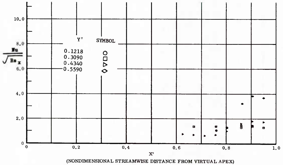
Fig. 61 Streamwise Distributions of Aerodynamic Heating Rates; Basic Configuration + Canards, No Flap Deflections, \alpha = +14.3^\circ , \beta = 0^\circ , Re_\infty/ft = 3,300,000 .
