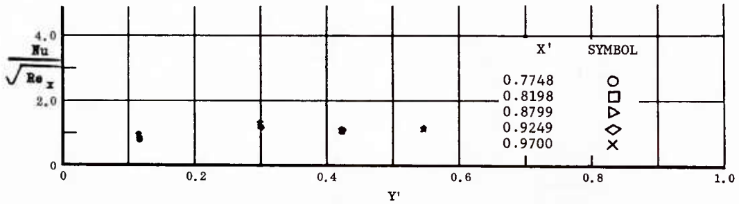
Fig. 47 Spanwise Distributions of Aerodynamic Heating Rates; Basic Configuration, Left and Right (Upper) Flaps Deflected -40^\circ , \alpha = +14.3^\circ , \beta = 0^\circ , Re_\infty/ft = 1,100,000 .
