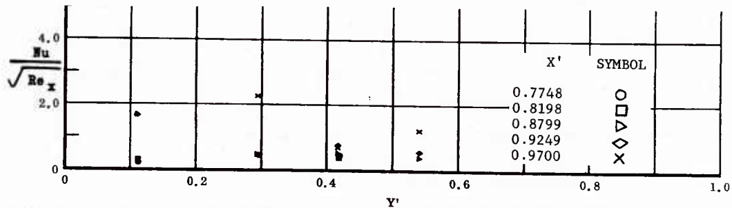
Fig. 44 Spanwise Distributions of Aerodynamic Heating Rates; Basic Configuration + Fin ( \delta = 15^\circ ), No Flap Deflections, \alpha = 0^\circ , \beta = +12^\circ , Re_\infty/ft = 3,300,000 .
