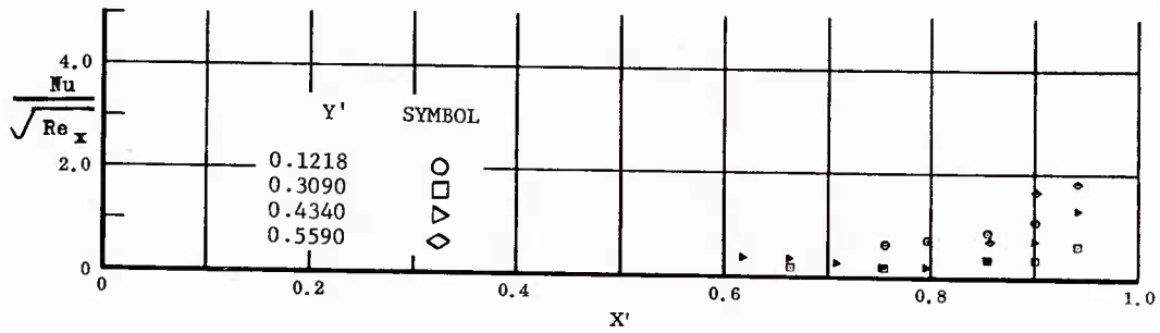
Fig. 30 Streamwise Distributions of Aerodynamic Heating Rates; Basic Configuration, Bottom Flaps Deflected +10^\circ , \alpha = 0^\circ , \beta = 0^\circ , Re_\infty/ft = 3,300,000 .
