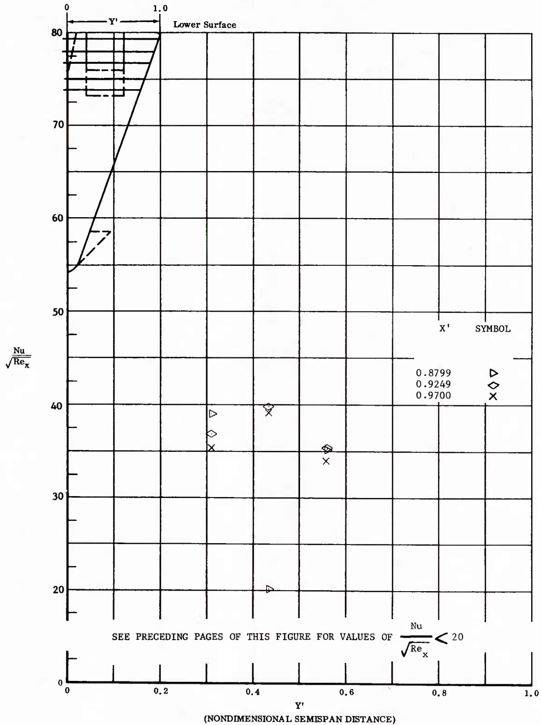
Fig. 65 Spanwise Distributions of Aerodynamic Heating Rates; Basic Configuration + Canards, Bottom Flaps Deflected +20°, \alpha = +14.3^\circ , \beta = 0^\circ , Re_\infty / ft = 3,300,000 .
