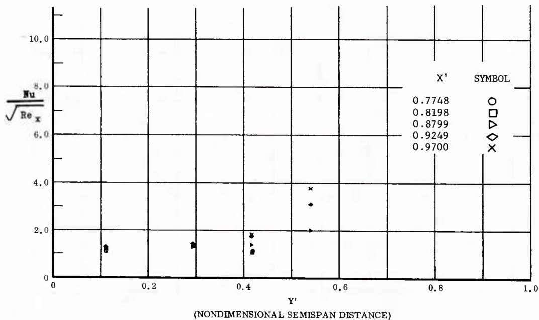
Fig. 60 Spanwise Distributions of Aerodynamic Heating Rates; Basic Configuration, No Flap Deflections, \alpha = +14.3^\circ , \beta = 0^\circ , Re_\infty / ft = 3,300,000 .
