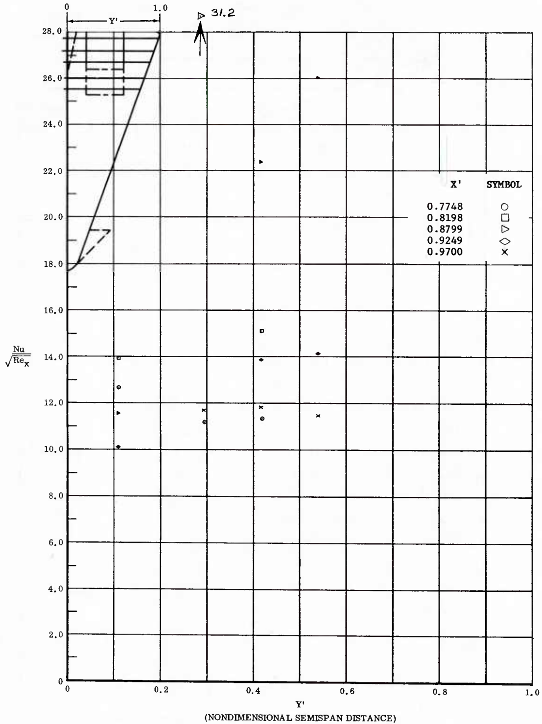
Fig. 79 Spanwise Distributions of Aerodynamic Heating Rates; Basic Configuration, Bottom Flaps Deflected +40°, \alpha = +45^\circ , \beta = 0^\circ , Re_\infty/ft = 3,300,000 .
