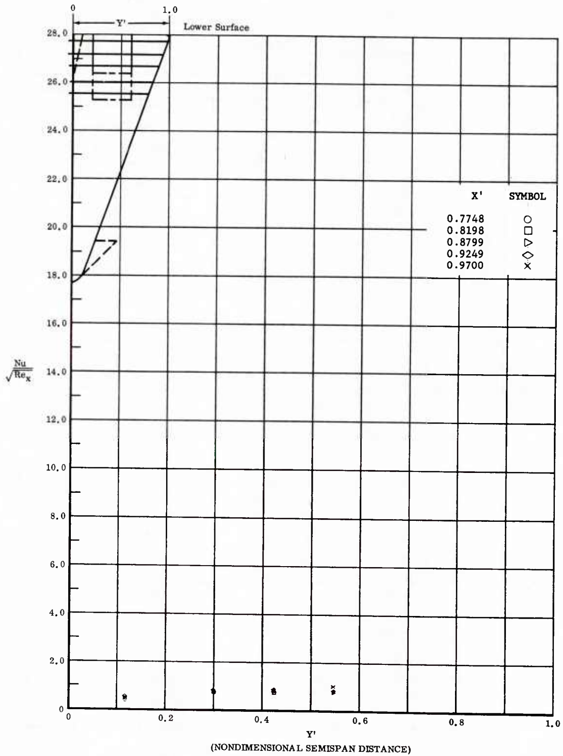
Fig. 45 Spanwise Distributions of Aerodynamic Heating Rates; Basic Configuration, Left and Right (Upper) Flaps Deflected -40^\circ , \alpha = +7^\circ , \beta = 0^\circ , Re_\infty/ft = 3,300,000 .
