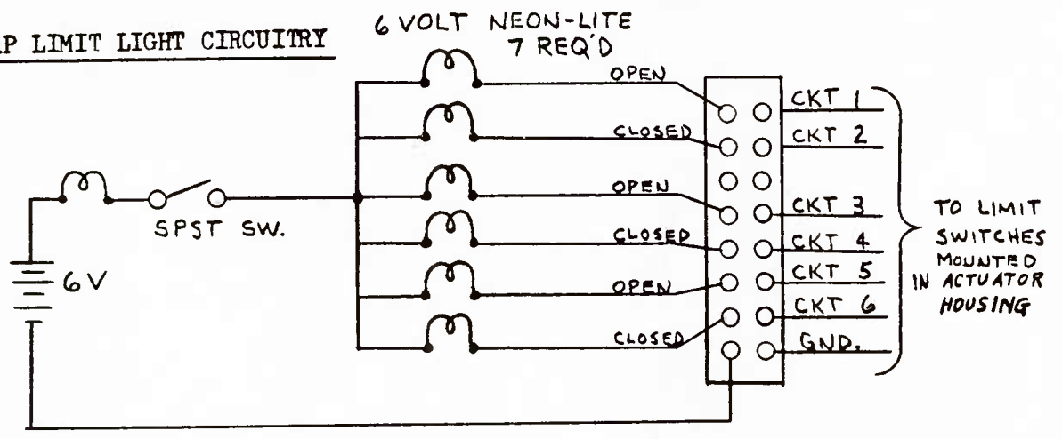
Fig. 5 Electrical Circuits for Remotely Controlled Flaps
