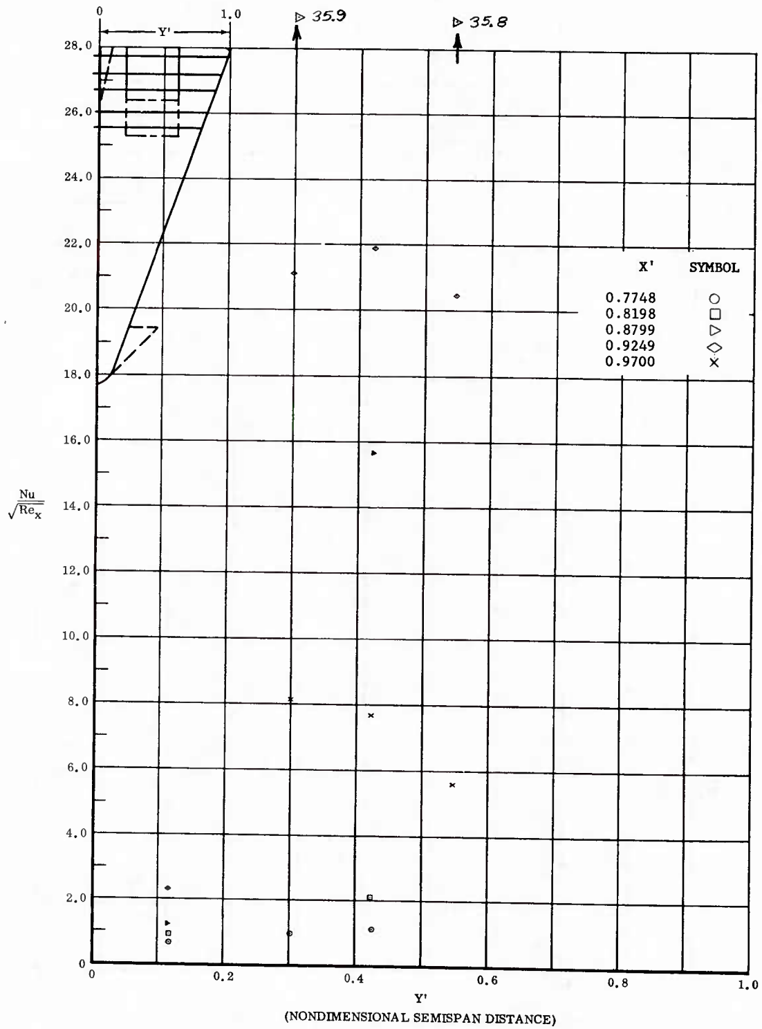
Fig. 69 Spanwise Distributions of Aerodynamic Heating Rates; Basic Configuration, Bottom Flaps Deflected +40°, \alpha = +14.3^\circ , \beta = 0^\circ , Re_\infty/ft = 1,100,000 .
