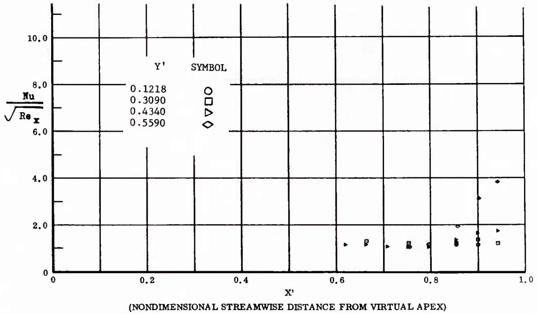
Fig. 52 Streamwise Distributions of Aerodynamic Heating Rates; Basic Configuration, Left and Right (Upper) Flaps Deflected -30^\circ , \alpha = +14.3^\circ , \beta = 0^\circ , Re_\infty / ft = 3,300,000 .
