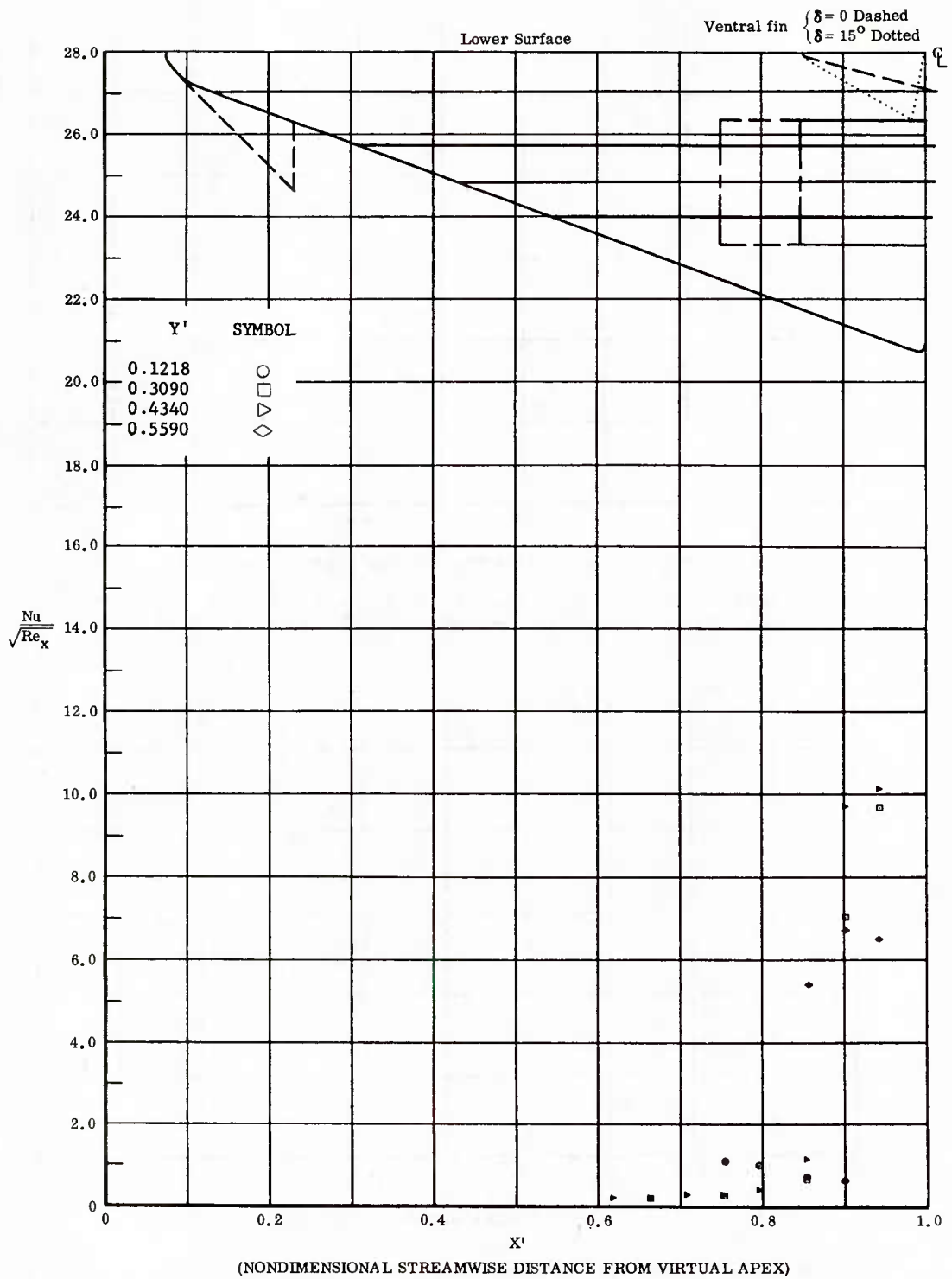
Fig. 37 Streamwise Distributions of Aerodynamic Heating Rates; Basic Configuration, Bottom Flaps Deflected +30°, \alpha = 0^\circ , \beta = 0^\circ , Re_\infty/ft = 3,300,000 .
