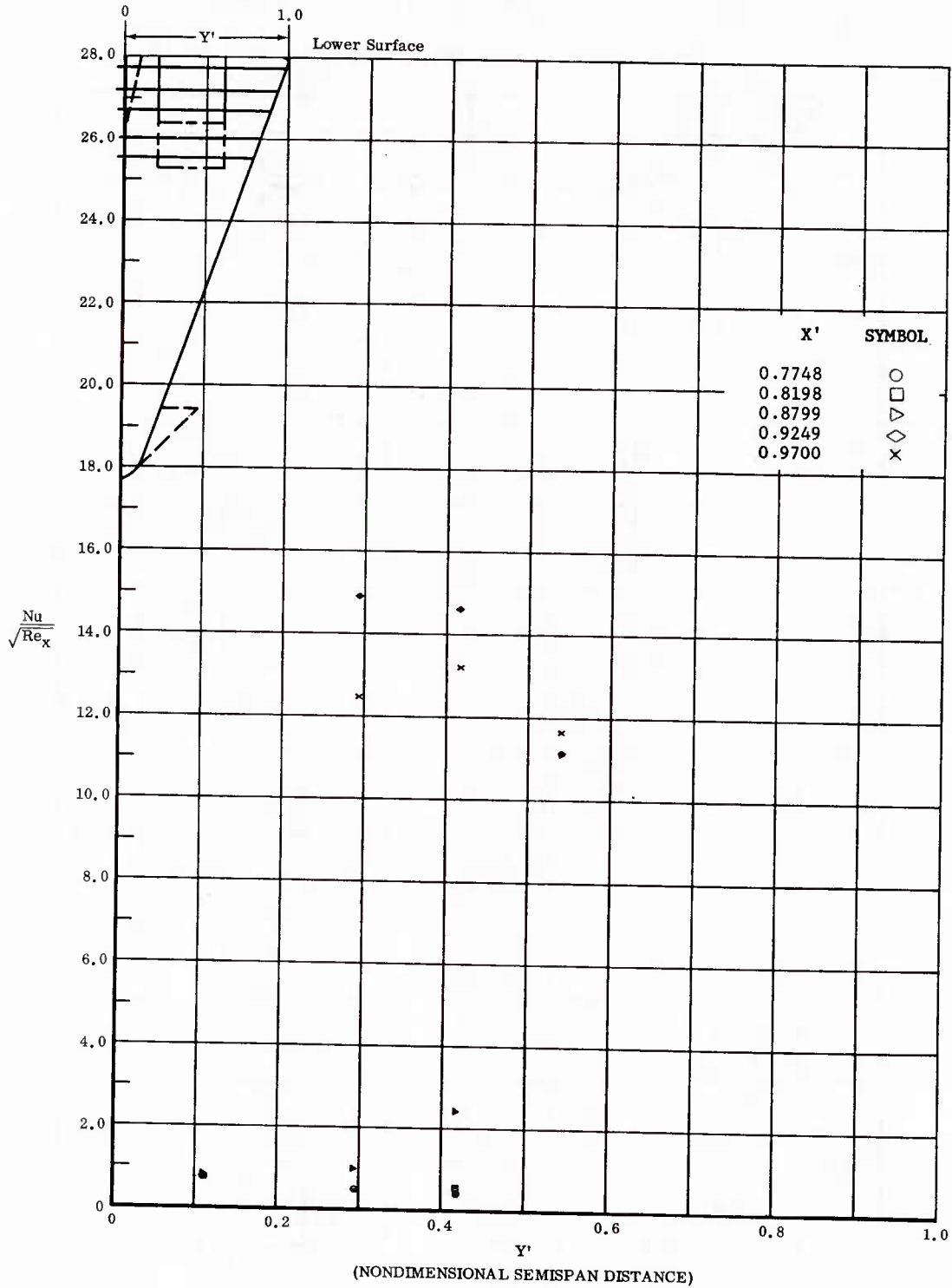
Fig. 39 Spanwise Distributions of Aerodynamic Heating Rates; Basic Configuration, Bottom Flaps Deflected +40°, \alpha = 0^\circ , \beta = 0^\circ , Re_\infty/ft' = 3,300,000 .
