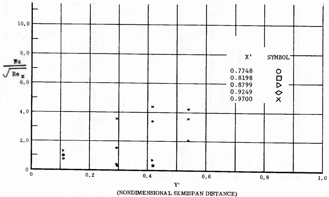
Fig. 32 Spanwise Distributions of Aerodynamic Heating Rates; Basic Configuration, Bottom Flaps Deflected +20°, \alpha = 0^\circ , \beta = 0^\circ , Re_\infty/ft = 3,300,000 .
