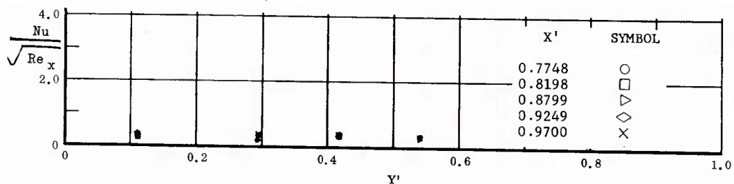
Fig. 10 Spanwise Distributions of Aerodynamic Heating Rates; Basic Configuration, Bottom Flap Deflected +40^\circ , \alpha = -45^\circ , \beta = 0^\circ , Re_\infty/ft = 3,300,000 .
