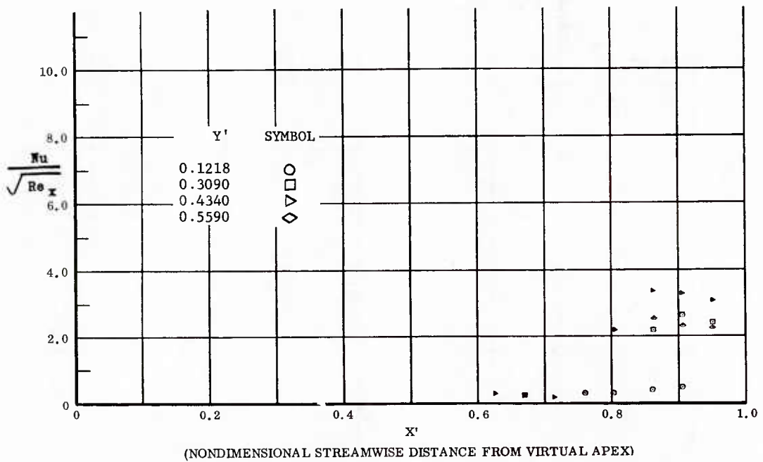
Fig. 35 Streamwise Distributions of Aerodynamic Heating Rates; Basic Configuration + Longer Chord Flaps, Bottom Flaps Deflected +20°, \alpha = 0^\circ , \beta = 0^\circ , Re_\infty/ft = 1,100,000 .
