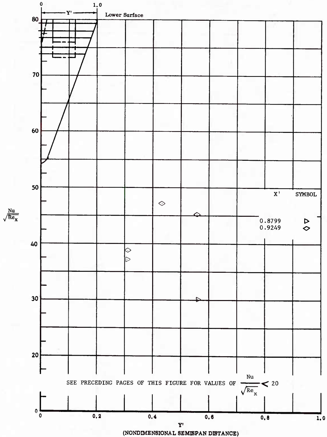
Fig. 70 Spanwise Distributions of Aerodynamic Heating Rates; Basic Configuration, Bottom Flaps Deflected +40°, \alpha = +14.3^\circ , \beta = 0^\circ , Re_\infty/ft = 3,300,000 .
