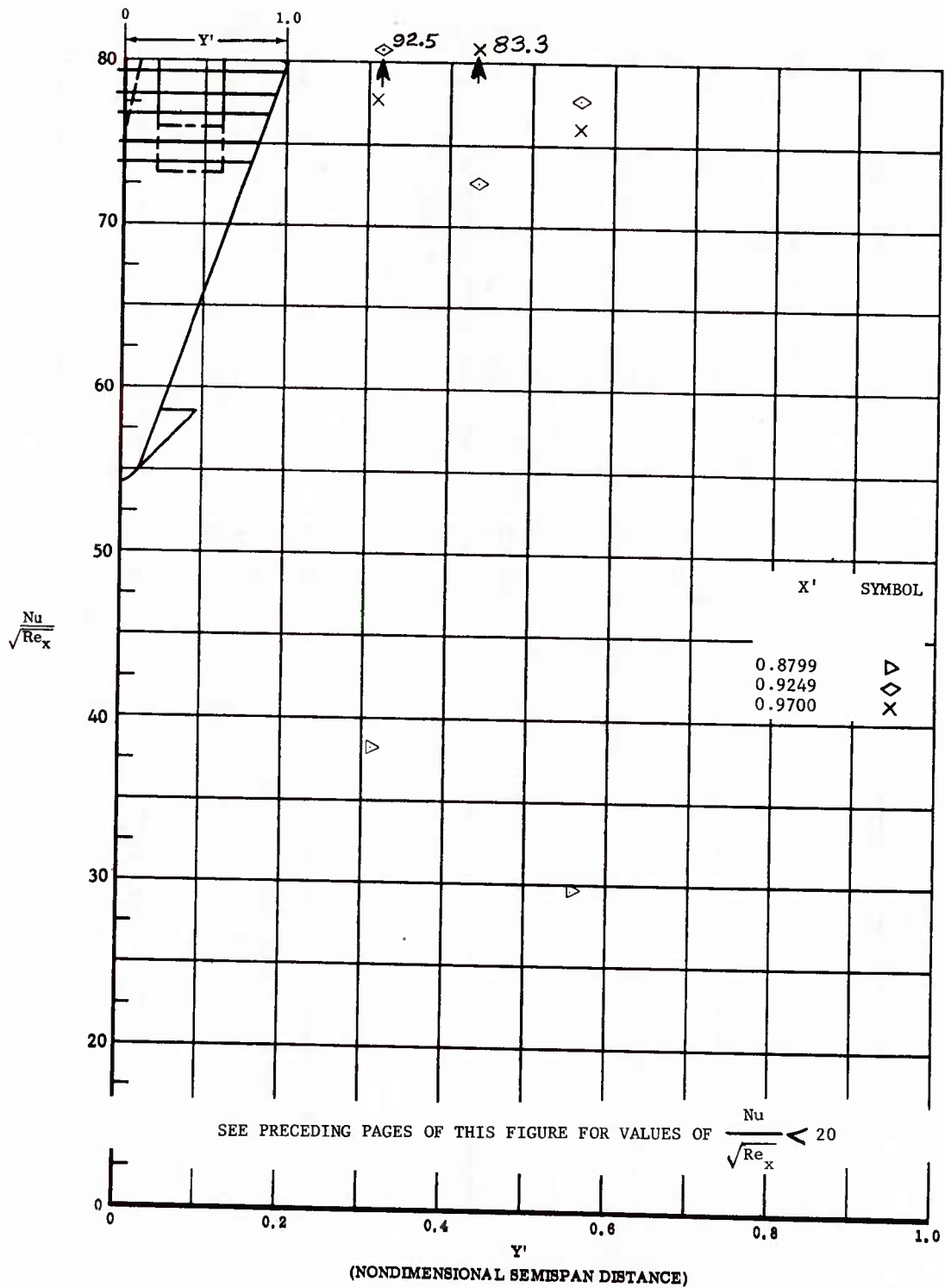
Fig. 71 Spanwise Distributions of Aerodynamic Heating Rates; Basic Configuration + Canards, Bottom Flaps Deflected +40°, \alpha = +14.3^\circ , \beta = 0^\circ , Re_\infty/ft = 3,300,000 .
