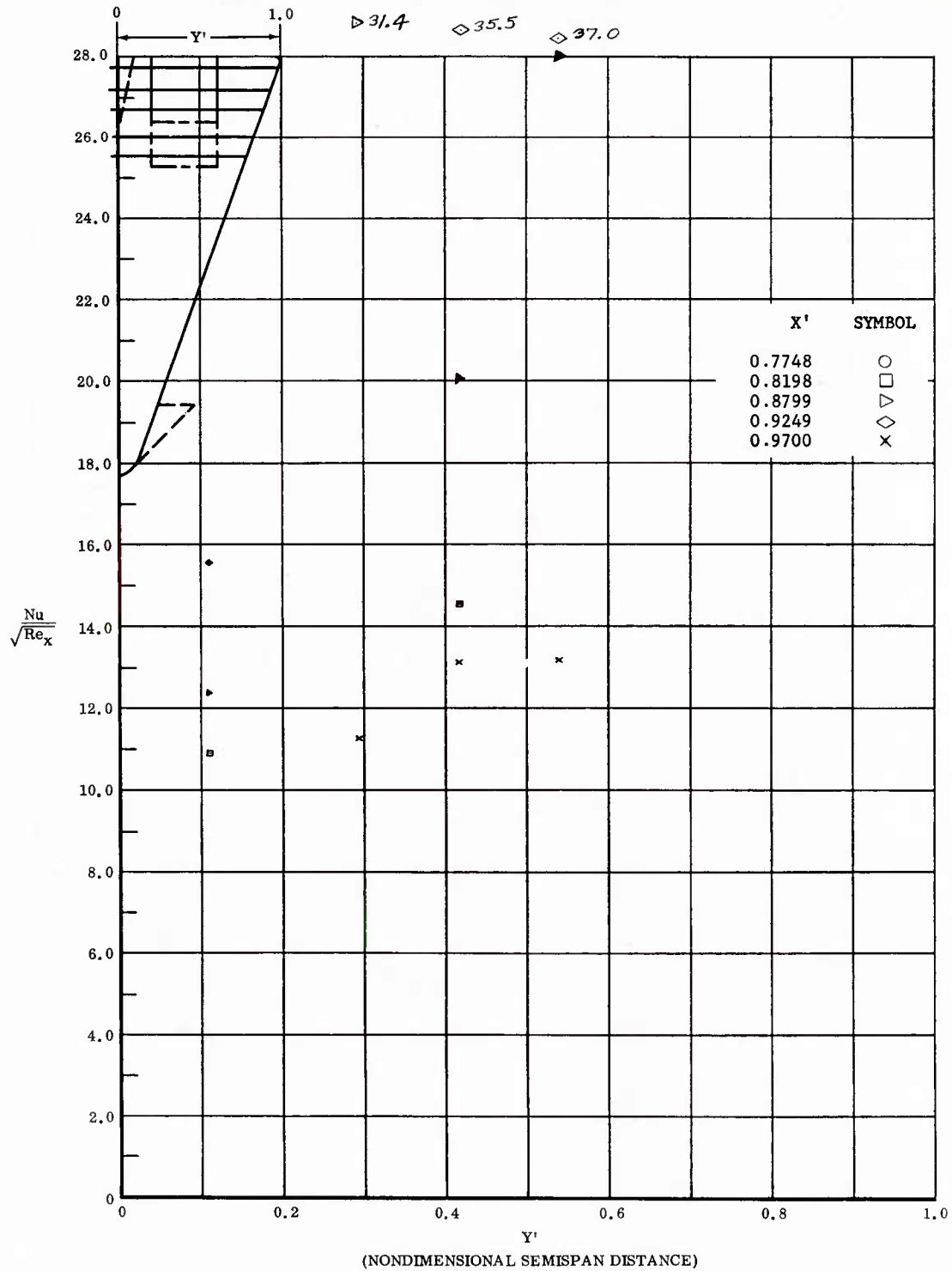
Fig. 75 Spanwise Distributions of Aerodynamic Heating Rates; Basic Configuration, Bottom Flaps Deflected +40°, \alpha = +33^\circ , \beta = 0^\circ , Re_\infty/ft = 3,300,000 .
