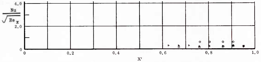
Fig. 15 Streamwise Distributions of Aerodynamic Heating Rates; Basic Configuration, Left (Upper) Flap Deflected -40^\circ , \alpha = 0^\circ , \beta = 0^\circ , Re_\infty/ft = 3,300,000 .
