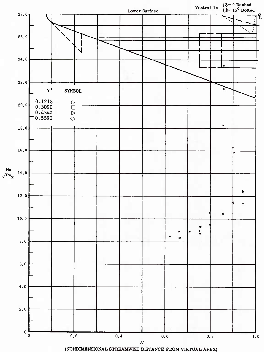
Fig. 78 Streamwise Distributions of Aerodynamic Heating Rates; Basic Configuration, Bottom Flaps Deflected +20°, \alpha = +45^\circ , \beta = 0^\circ , Re_\infty / ft = 3,300,000 .
