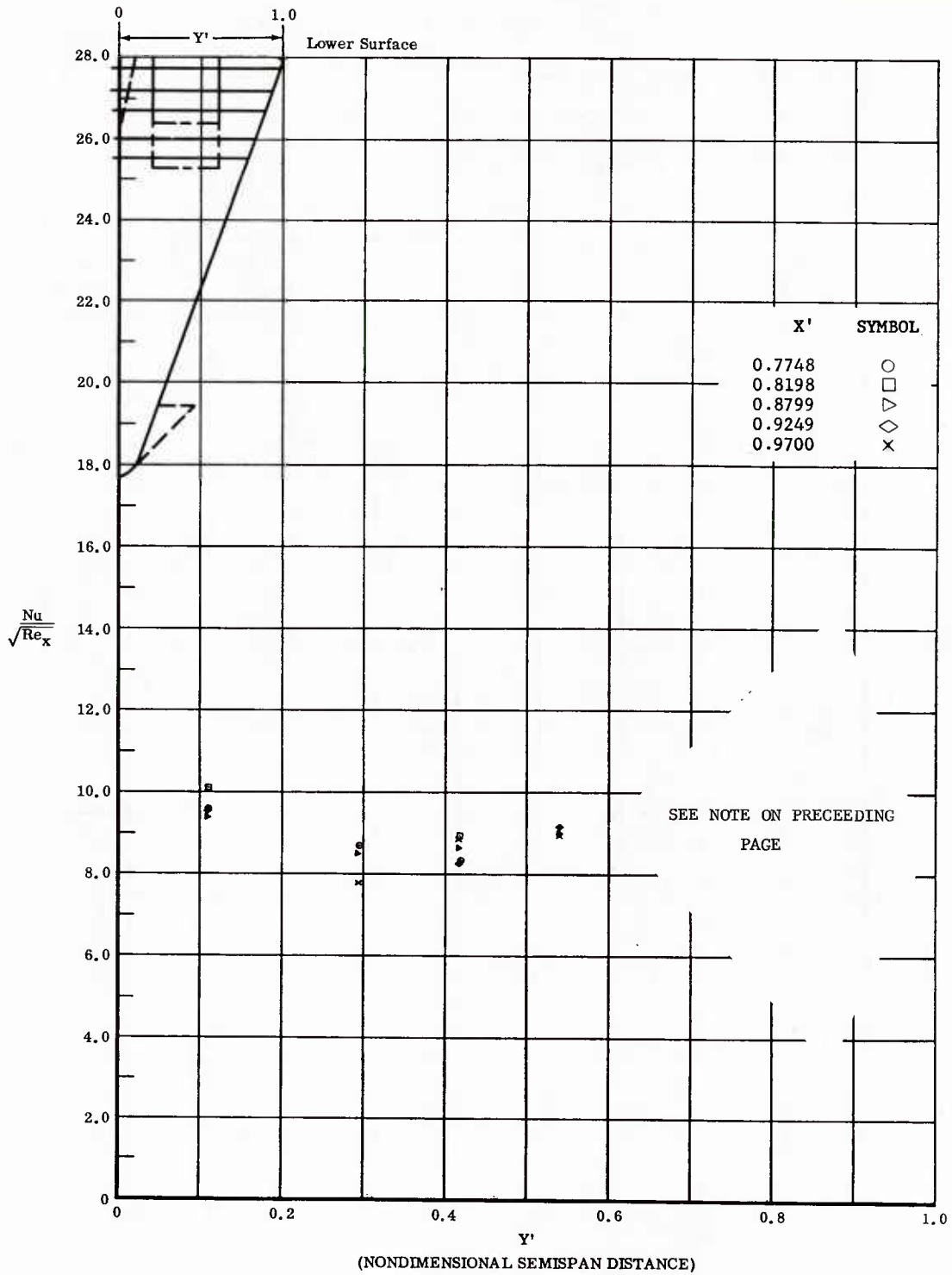
Fig. 80 Spanwise Distributions of Aerodynamic Heating Rates; Basic Configuration, Left and Right (Upper) Flaps Deflected -40^\circ , \alpha = +54^\circ , \beta = 0^\circ , Re_\infty/ft = ? .
