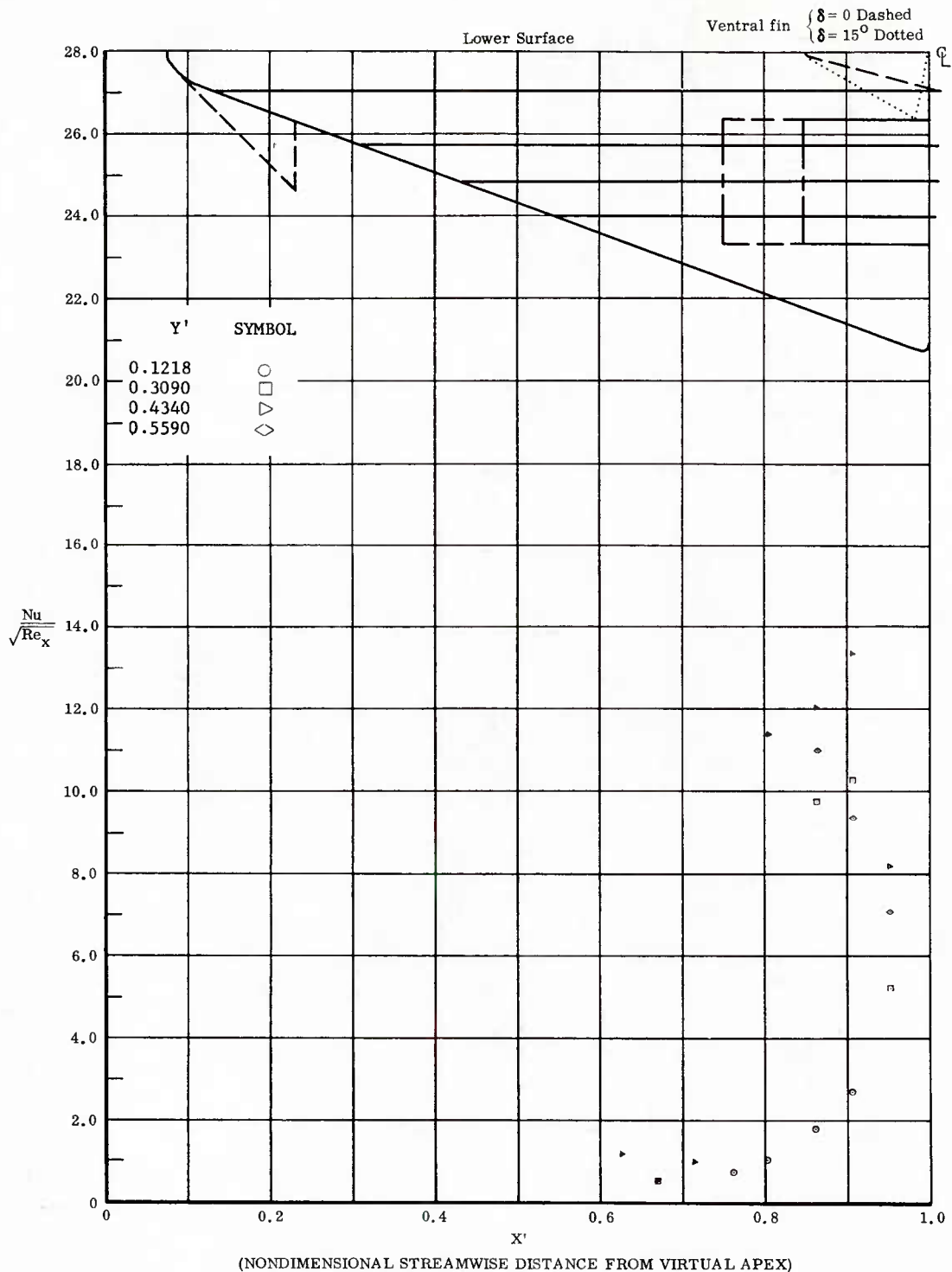
Fig. 66 Streamwise Distributions of Aerodynamic Heating Rates; Basic Configuration + Longer Chord Flaps, Bottom Flaps Deflected +20°, \alpha = +14.3^\circ , \beta = 0^\circ , Re_\infty/ft = 1,100,000 .
