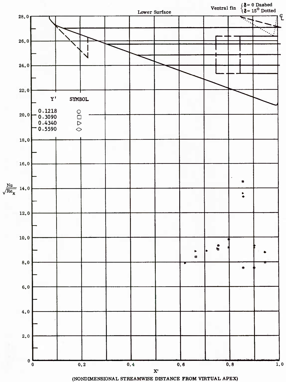
Fig. 82 Streamwise Distributions of Aerodynamic Heating Rates; Basic Configuration, Bottom Flaps Deflected +40^\circ , \alpha = +54^\circ , \beta = 0^\circ , Re_\infty / ft = 3,300,000 .
