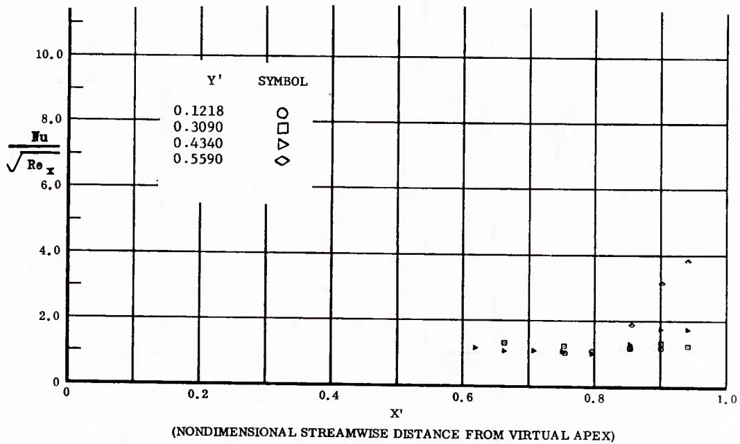
Fig. 58 Streamwise Distributions of Aerodynamic Heating Rates; Basic Configuration, Left and Right (Upper) Flaps Deflected -10^\circ , \alpha = +14.3^\circ , \beta = 0^\circ , Re_\infty / ft = 3,300,000 .
