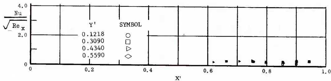
Fig. 10 Streamwise Distributions of Aerodynamic Heating Rates; Basic Configuration, Bottom Flap Deflected +40^\circ , \alpha = -45^\circ , \beta = 0^\circ , Re_\infty/ft = 3,300,000 .
