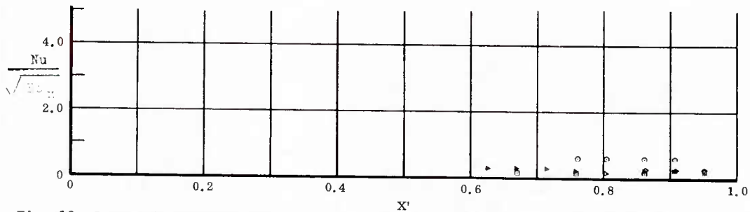
Fig. 18 Streamwise Distributions of Aerodynamic Heating Rates; Basic Configuration, Left and Right (Upper) Flaps Deflected -30^\circ , \alpha = 0^\circ , \beta = 0^\circ , Re_\infty/ft = 3,300,000 .
