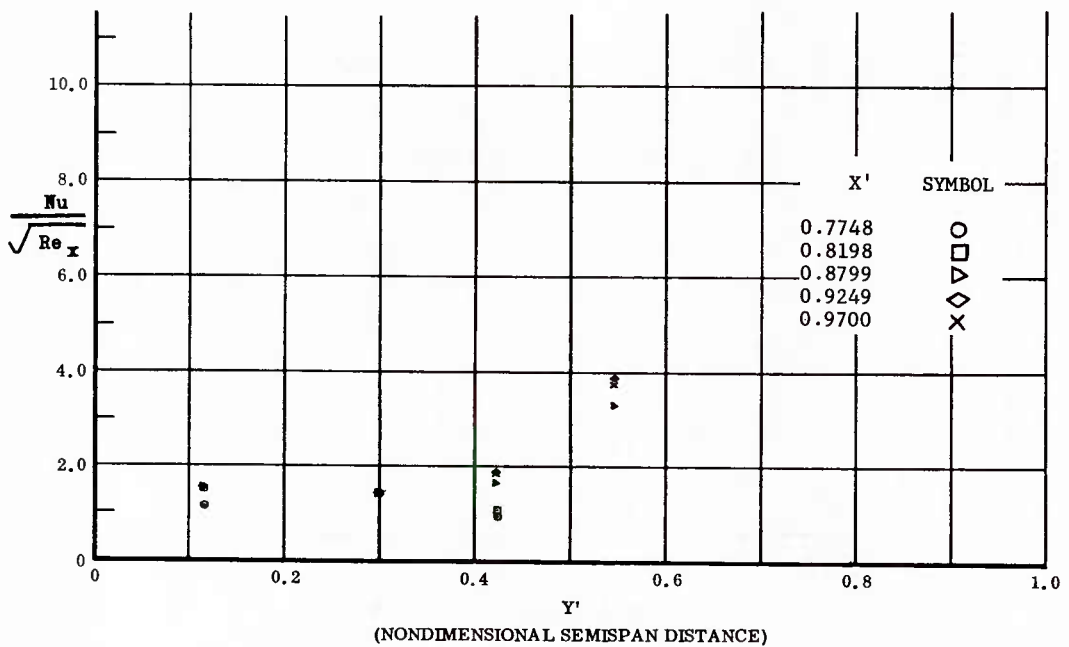
Fig. 61 Spanwise Distributions of Aerodynamic Heating Rates; Basic Configuration + Canards, No Flap Deflections, \alpha = +14.3^\circ , \beta = 0^\circ , Re_\infty/ft = 3,300,000 .
