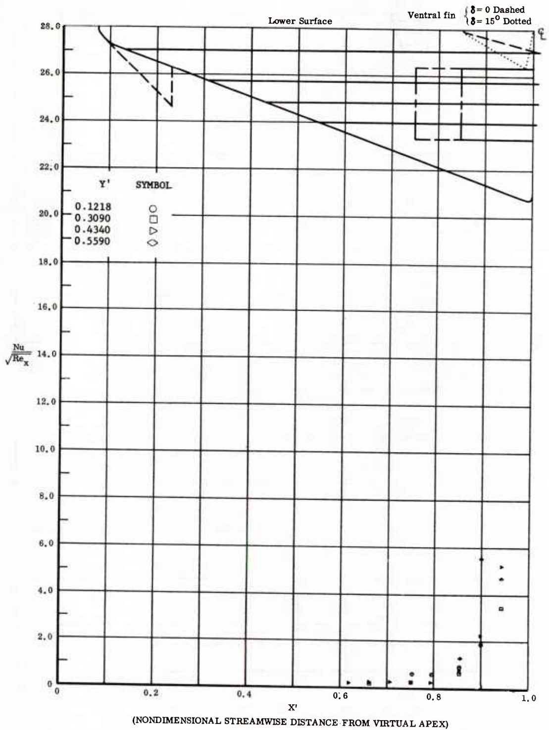
Fig. 34 Streamwise Distributions of Aerodynamic Heating Rates; Basic Configuration + Fin ( \delta = 0 ), Bottom Flaps Deflected +20^\circ , \alpha = 0^\circ , \beta = .0^\circ , Re_\infty / ft = 3,300,000 .
