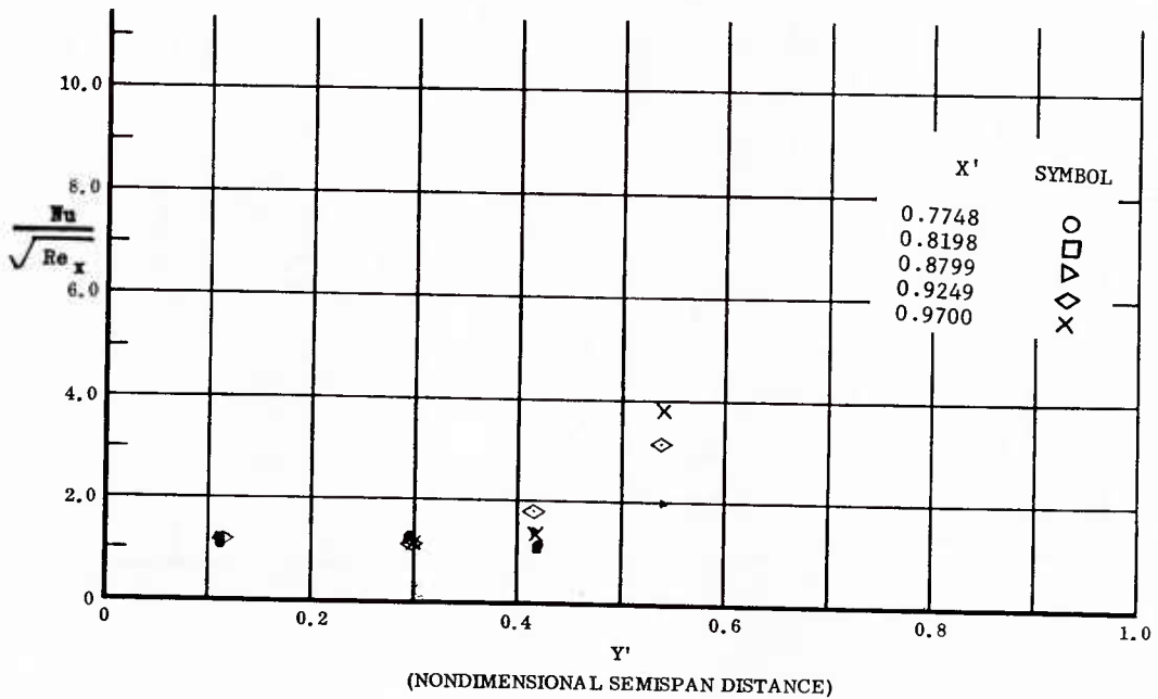
Fig. 58 Spanwise Distributions of Aerodynamic Heating Rates; Basic Configuration, Left and Right (Upper) Flaps Deflected -10^\circ , \alpha = +14.3^\circ , \beta = 0^\circ , Re_\infty / ft = 3,300,000 .
