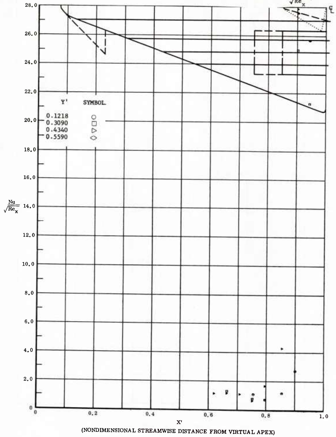
Fig. 68 Streamwise Distributions of Aerodynamic Heating Rates; Basic Configuration, Bottom Flaps Deflected +30°, \alpha = +14.3^\circ , \beta = 0^\circ , Re_\infty/ft = 3,300,000 .
