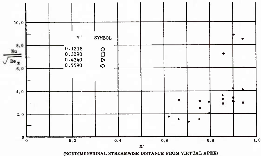
Fig. 51 Streamwise Distributions of Aerodynamic Heating Rates; Basic Configuration + Canards, Left and Right (Upper) Flaps Deflected -40^\circ , \alpha = +14.3^\circ , \beta = 0^\circ , Re_\infty/ft = 3,300,000 .
