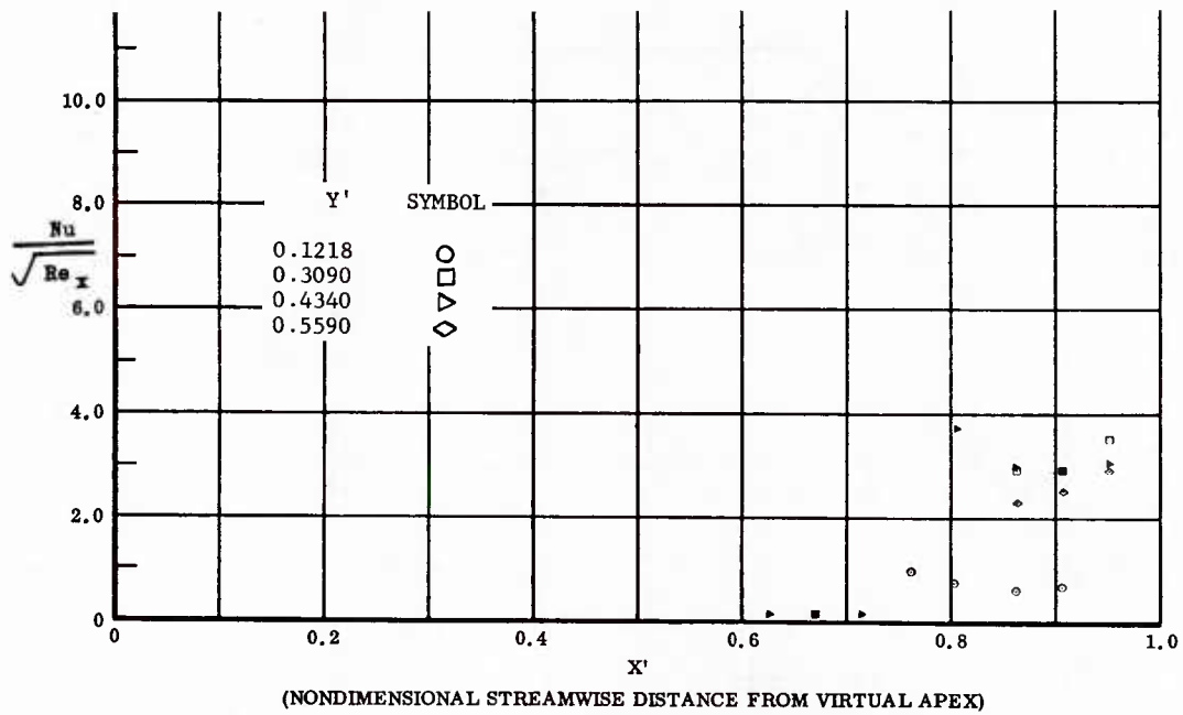
Fig. 36 Streamwise Distributions of Aerodynamic Heating Rates; Basic Configuration + Longer Chord Flaps, Bottom Flaps Deflected +20°, \alpha = 0^\circ , \beta = 0^\circ , Re_\infty/ft = 3,300,000 .
