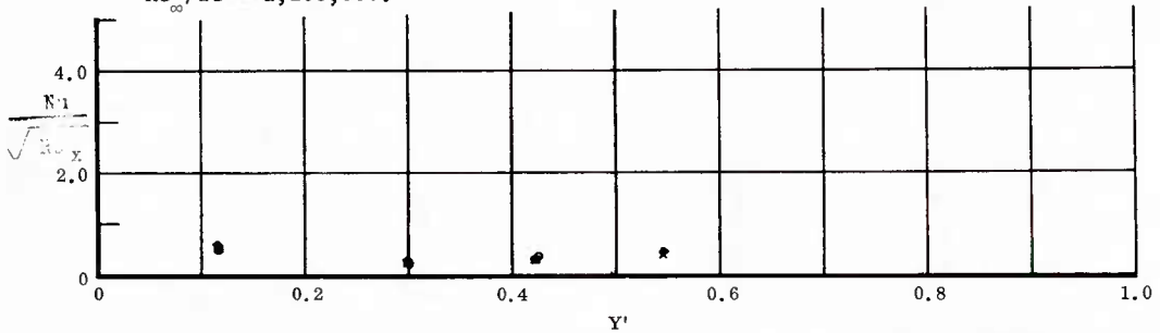
Fig. 19 Spanwise Distributions of Aerodynamic Heating Rates; Basic Configuration, Left and Right (Upper) Flaps Deflected -20^\circ , \alpha = 0^\circ , \beta = 0^\circ , Re_\infty/ft = 1,100,000 .
