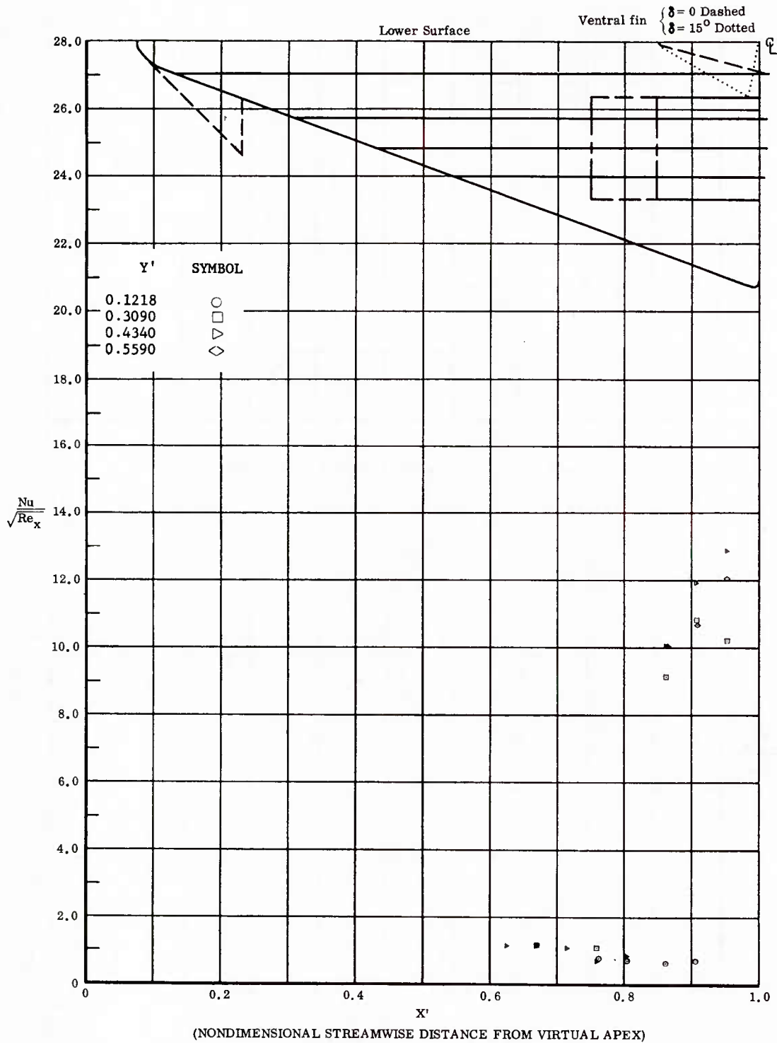
Fig. 63 Streamwise Distributions of Aerodynamic Heating Rates; Basic Configuration, Bottom Flaps Deflected +20^\circ , \alpha = +14.3^\circ , \beta = 0^\circ , Re_\infty/ft = 1,100,000 .
