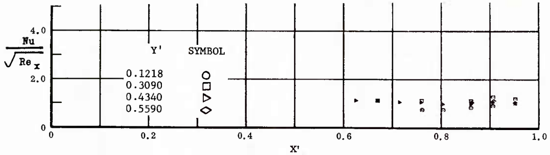
Fig. 47 Streamwise Distributions of Aerodynamic Heating Rates; Basic Configuration, Left and Right (Upper) Flaps Deflected -40^\circ , \alpha = +14.3^\circ , \beta = 0^\circ , Re_\infty/ft = 1,100,000 .
