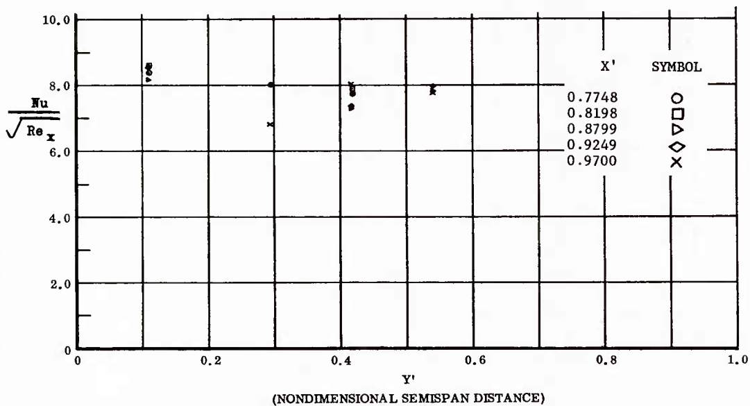
Fig. 72 Spanwise Distributions of Aerodynamic Heating Rates; Basic Configuration, Left and Right (Upper) Flaps Deflected -40^\circ , \alpha = +33^\circ , \beta = 0^\circ , Re_\infty / ft = 3,300,000 .
