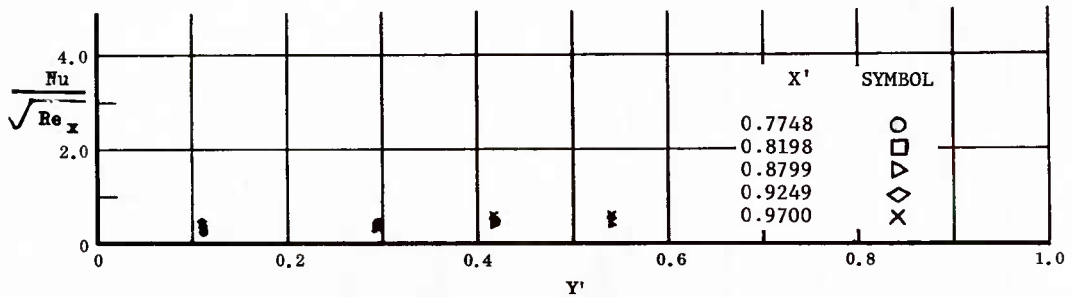
Fig. 41 Spanwise Distributions of Aerodynamic Heating Rates; Basic Configuration No Flap Deflections, \alpha = 0^\circ , \beta = +12^\circ , Re_\infty/ft = 3,300,000 .
