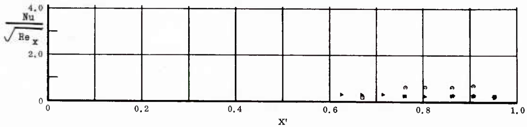
Fig. 14 Streamwise Distributions of Aerodynamic Heating Rates; Basic Configuration, Left and Right (Upper) Flaps Deflected -40^\circ , \alpha = 0^\circ , \beta = 0^\circ , Re_\infty/ft = 3,300,000 .
