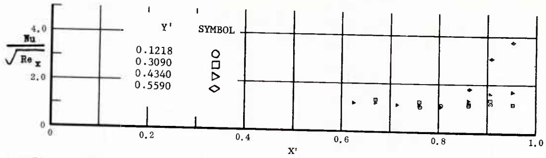
Fig. 55 Streamwise Distributions of Aerodynamic Heating Rates; Basic Configuration, Left (Upper) Flap Deflected -20^\circ , \alpha = +14.3^\circ , \beta = 0^\circ , Re_\infty/ft = 3,300,000 .
