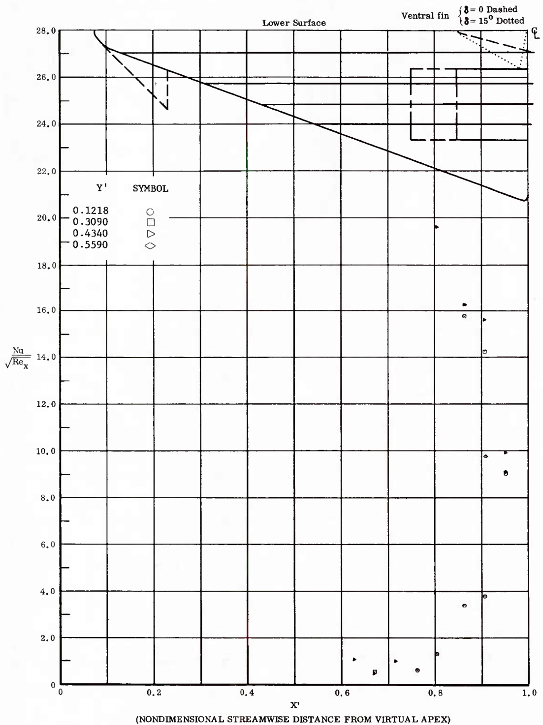
Fig. 67 Streamwise Distributions of Aerodynamic Heating Rates; Basic Configuration + Longer Chord Flaps, Bottom Flaps Deflected +20°, \beta = 0^\circ , \alpha = +14.3^\circ , Re_\infty/ft = 3,300,000 .
