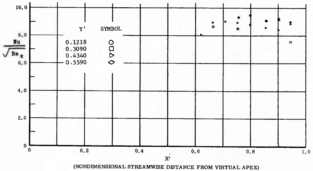
Fig. 76 Streamwise Distributions of Aerodynamic Heating Rates; Basic Configuration, Left and Right (Upper) Flaps Deflected -40^\circ , \alpha = +45^\circ , \beta = 0^\circ , Re_\infty/ft = 3,300,000 .
