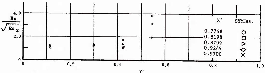
Fig. 48 Spanwise Distributions of Aerodynamic Heating Rates; Basic Configuration, Left and Right (Upper) Flaps Deflected -40^\circ , \alpha = +14.3^\circ , \beta = 0^\circ , Re_\infty/ft = 3,300,000 .
