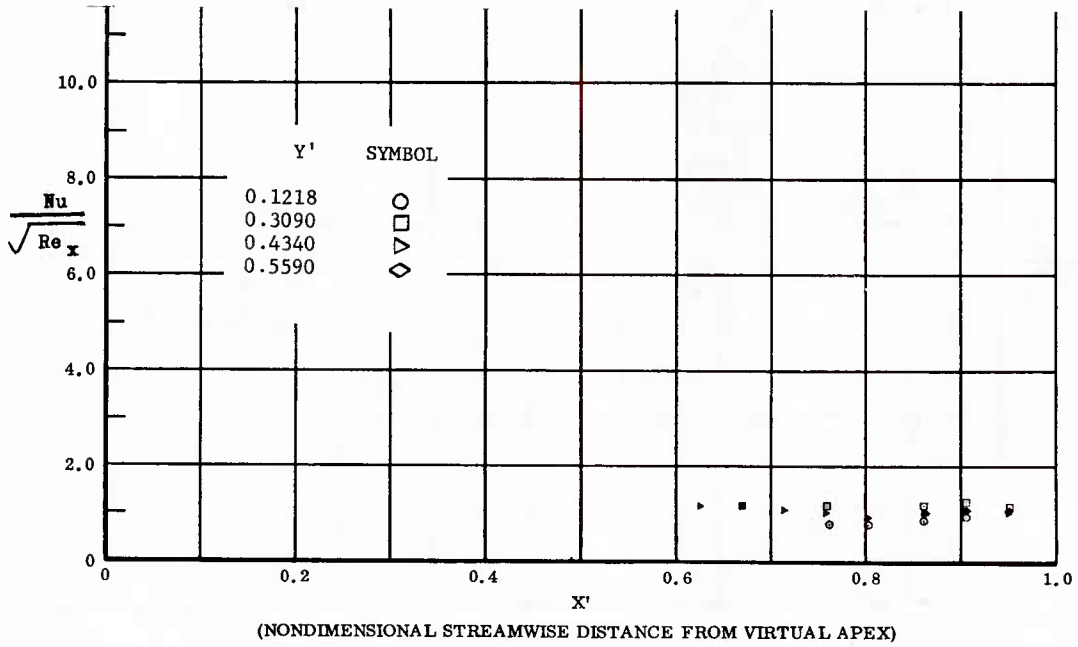
Fig. 59 Streamwise Distributions of Aerodynamic Heating Rates; Basic Configuration, No Flap Deflections, \alpha = +14.3^\circ , \beta = 0^\circ , Re_\infty/ft = 1,100,000 .
