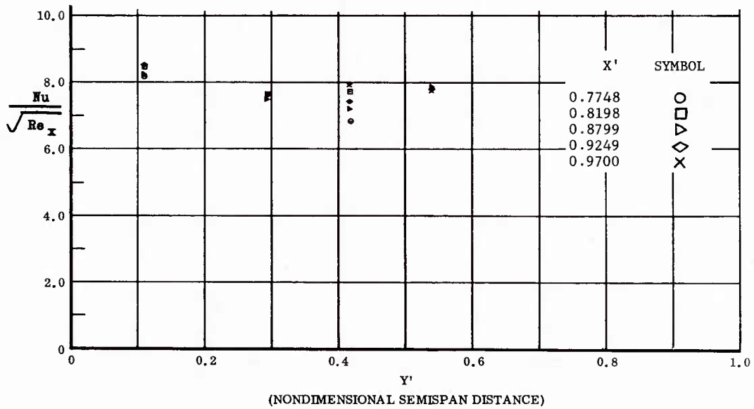
Fig. 73 Spanwise Distributions of Aerodynamic Heating Rates; Basic Configuration, No Flap Deflections, \alpha = +33^\circ , \beta = 0^\circ , Re_\infty/ft = 3,300,000 .
