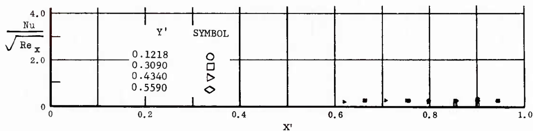
Fig. 9 Streamwise Distributions of Aerodynamic Heating Rates; Basic Configuration, No Flap Deflections, \alpha = -45^\circ , \beta = 0^\circ , Re_\infty/ft = 3,300,000 .
