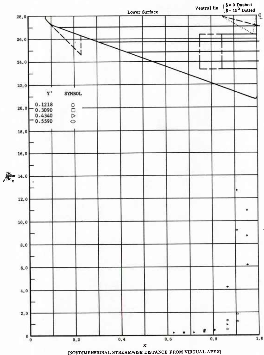
Fig. 38 Streamwise Distributions of Aerodynamic Heating Rates; Basic Configuration, Bottom Flaps Deflected +40°, \alpha = 0^\circ , \beta = 0^\circ , Re_\infty/ft = 1,100,000 .
