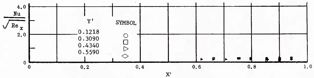
Fig. 7 Streamwise Distributions of Aerodynamic Heating Rates; Basic Configuration, Left and Right (Upper) Flaps Deflected -40^\circ , \alpha = -45^\circ , \beta = 0^\circ , Re_\infty/ft = 3,300,000 .
