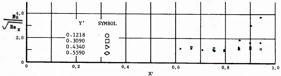
Fig. 48 Streamwise Distributions of Aerodynamic Heating Rates; Basic Configuration, Left and Right (Upper) Flaps Deflected -40^\circ , \alpha = +14.3^\circ , \beta = 0^\circ , Re_\infty/ft = 3,300,000 .
