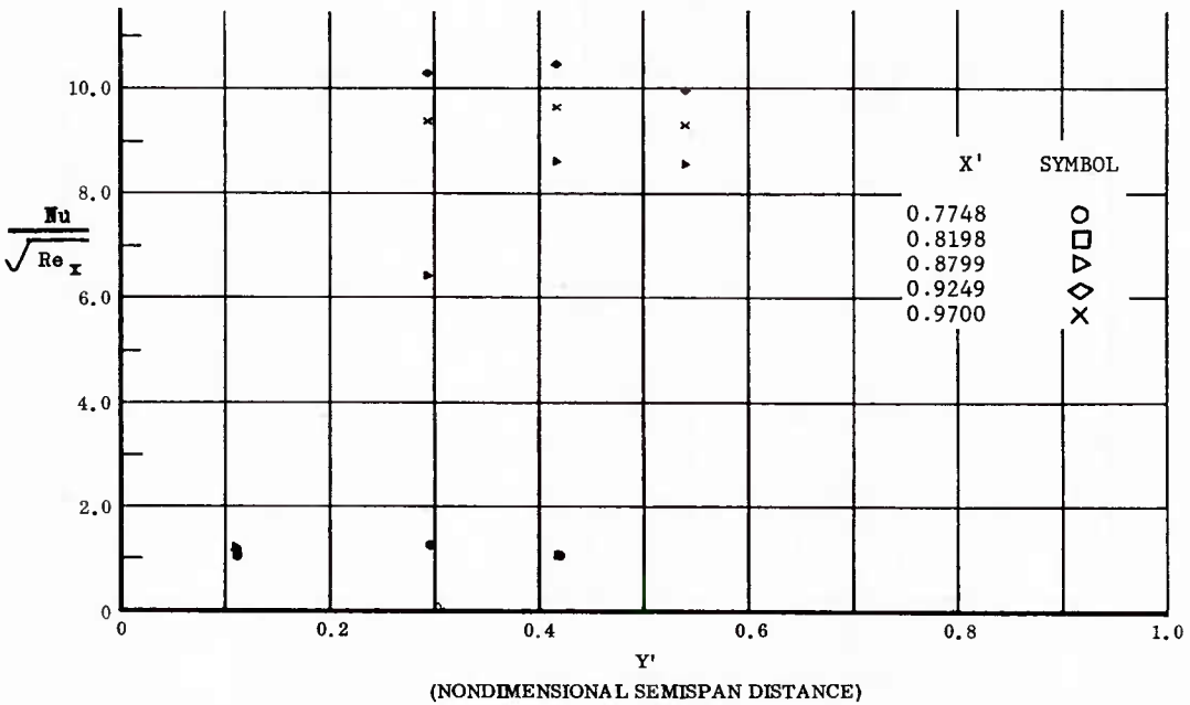
Fig. 62 Spanwise Distributions of Aerodynamic Heating Rates; Basic Configuration, Bottom Flaps Deflected +10°, \beta = 0^\circ , \alpha = +14.3^\circ , Re_\infty/ft = 3,300,000 .
