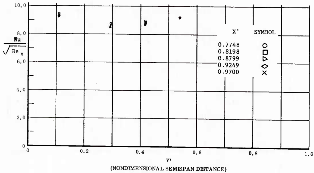
Fig. 77 Spanwise Distributions of Aerodynamic Heating Rates; Basic Configuration, No Flap Deflections, \alpha = +45^\circ , \beta = 0^\circ , Re_\infty/ft = 3,300,000 .
