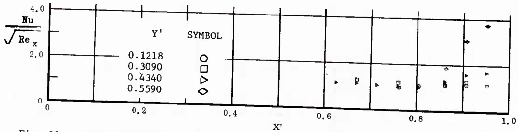
Fig. 56 Streamwise Distributions of Aerodynamic Heating Rates; Basic Configuration, Right (Upper) Flap Deflected -20^\circ , \alpha = +14.3^\circ , \beta = 0^\circ , Re_\infty/ft = 3,300,000 .
