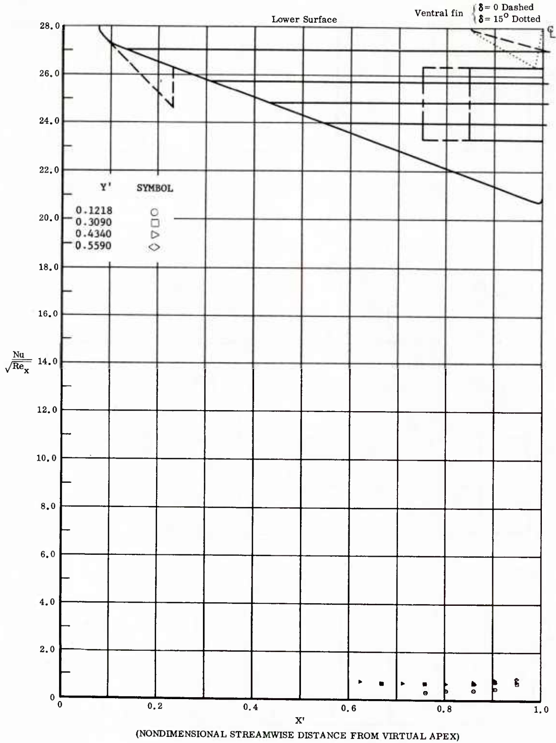
Fig. 45 Streamwise Distributions of Aerodynamic Heating Rates; Basic Configuration, Left and Right (Upper) Flaps Deflected -40^\circ , \alpha = +7^\circ , \beta = 0^\circ , Re_\infty/ft = 3,300,000 .
