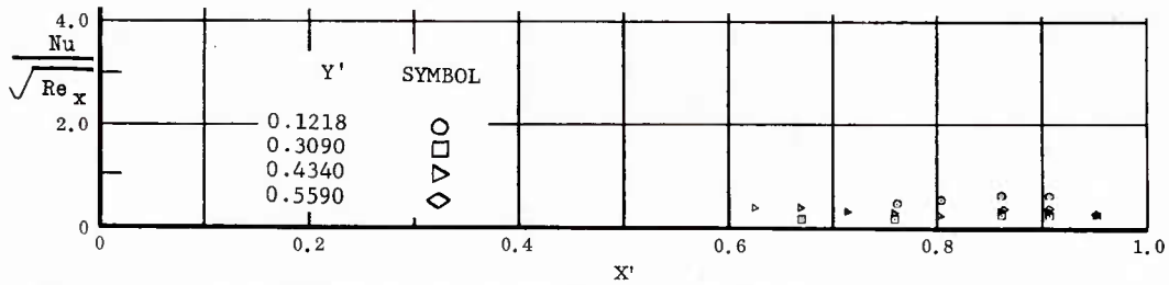
Fig. 13 Streamwise Distributions of Aerodynamic Heating Rates; Basic Configuration, Left and Right (Upper) Flaps Deflected -40^\circ , \alpha = 0^\circ , \beta = 0^\circ , Re_\infty/ft = 1,100,000 .
