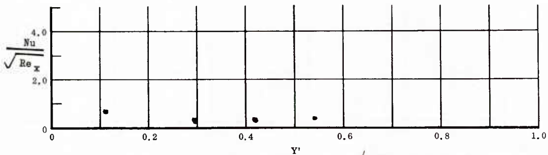
Fig. 24 Spanwise Distributions of Aerodynamic Heating Rates; Basic Configuration, Left and Right (Upper) Flaps Deflected -10^\circ , \alpha = 0^\circ , \beta = 0^\circ , Re_\infty/ft = 3,300,000 .
