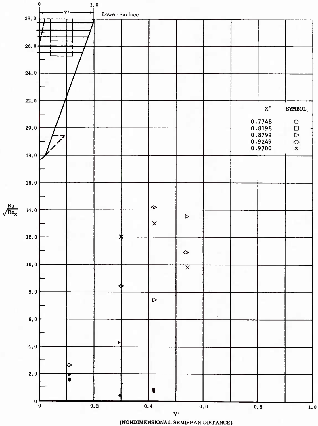
Fig. 33 Spanwise Distributions of Aerodynamic Heating Rates; Basic Configuration + Canards, Bottom Flaps Deflected +20°, \alpha = 0^\circ , \beta = 0^\circ , Re_\infty / ft = 3,300,000 .
