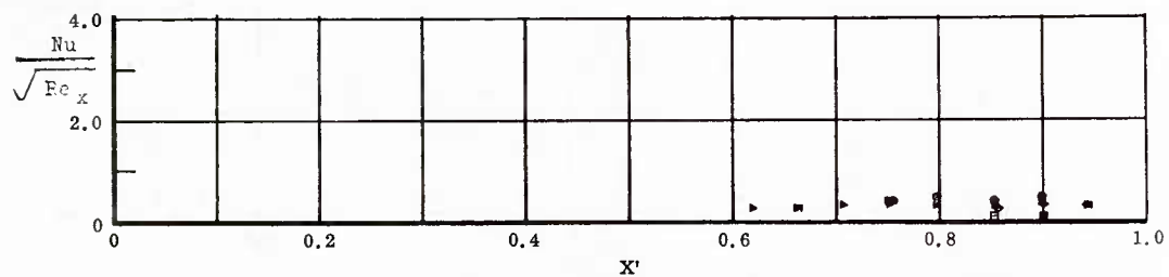
Fig. 12 Streamwise Distributions of Aerodynamic Heating Rates; Basic Configuration, No Flap Deflections, \alpha = -33^\circ , \beta = 0^\circ , Re_\infty/ft = 3,300,000 .
