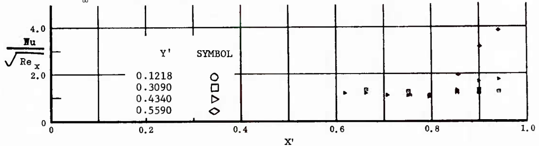
Fig. 54 Streamwise Distributions of Aerodynamic Heating Rates; Basic Configuration, Left and Right (Upper) Flaps Deflected -20^\circ , \alpha = +14.3^\circ , \beta = 0^\circ , Re_\infty/ft = 3,300,000 .
