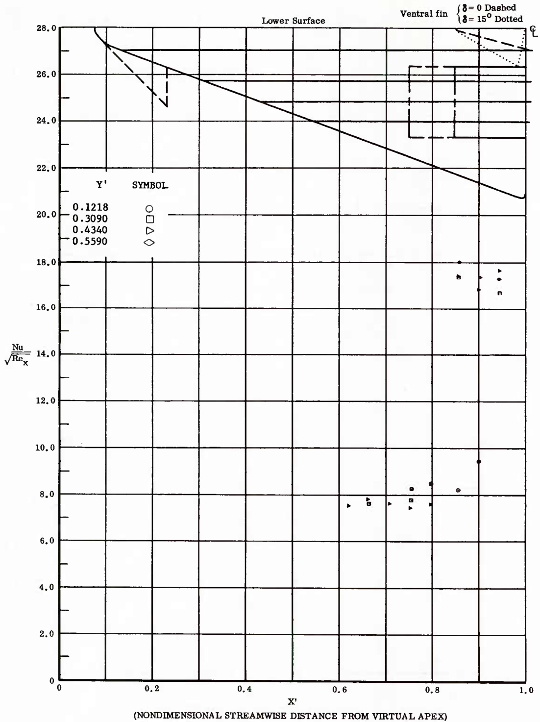
Fig. 74 Streamwise Distributions of Aerodynamic Heating Rates; Basic Configuration, Bottom Flaps Deflected +20°, \alpha = +33^\circ , \beta = 0^\circ , Re_\infty / ft \approx 3,300,000 .
