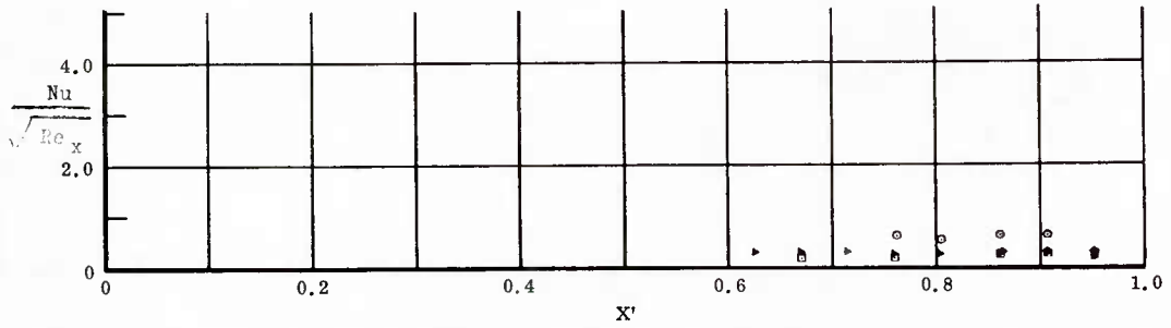
Fig. 16 Streamwise Distributions of Aerodynamic Heating Rates; Basic Configuration, Right (Upper) Flap Deflected -40^\circ , \alpha = 0^\circ , \beta = 0^\circ , Re_\infty/ft = 3,300,000 .
