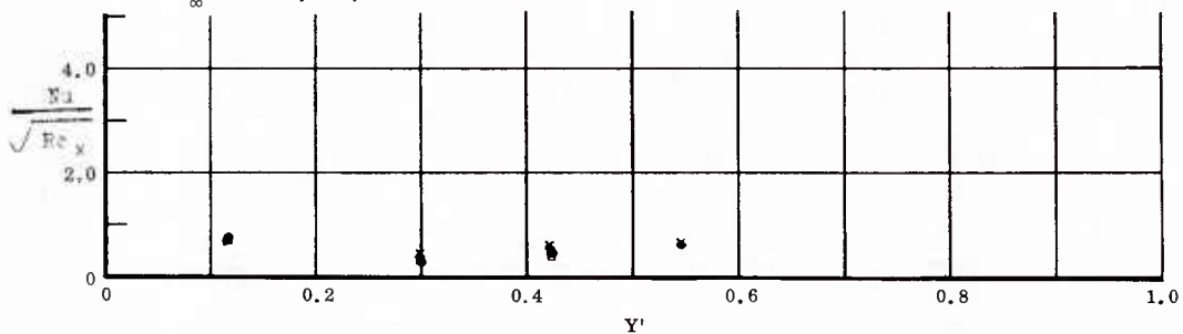
Fig. 23 Spanwise Distributions of Aerodynamic Heating Rates; Basic Configuration + Canards, Left and Right (Upper) Flaps Deflected -20^\circ , \alpha = 0^\circ , \beta = 0^\circ , Re_\infty/ft = 3,300,000 .
