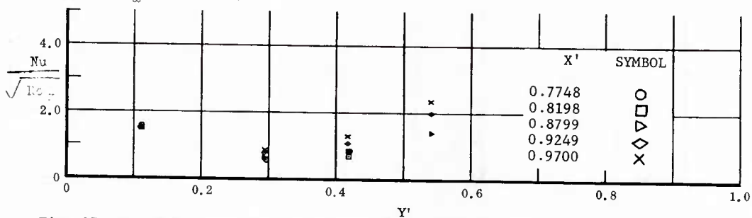
Fig. 17 Spanwise Distributions of Aerodynamic Heating Rates; Basic Configuration + Canards, Left and Right (Upper) Flaps Deflected -40^\circ , \alpha = 0^\circ , \beta = 0^\circ , Re_\infty/ft = 3,300,000 .
