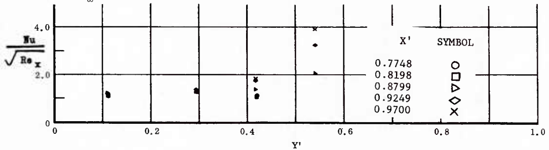
Fig. 54 Spanwise Distributions of Aerodynamic Heating Rates; Basic Configuration, Left and Right (Upper) Flaps Deflected -20^\circ , \alpha = +14.3^\circ , \beta = 0^\circ , Re_\infty/ft = 3,300,000 .
