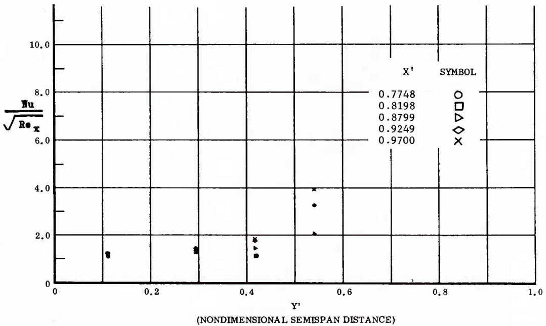
Fig. 52 Spanwise Distributions of Aerodynamic Heating Rates; Basic Configuration, Left and Right (Upper) Flaps Deflected -30^\circ , \alpha = +14.3^\circ , \beta = 0^\circ , Re_\infty / ft = 3,300,000 .
