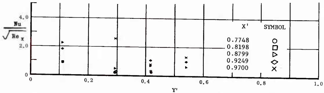
Fig. 29 Spanwise Distributions of Aerodynamic Heating Rates; Basic Configuration + Fin ( \delta = 15^\circ ), No Flap Deflections, \alpha = 0^\circ , \beta = 0^\circ , Re_\infty/ft = 3,300,000 .
