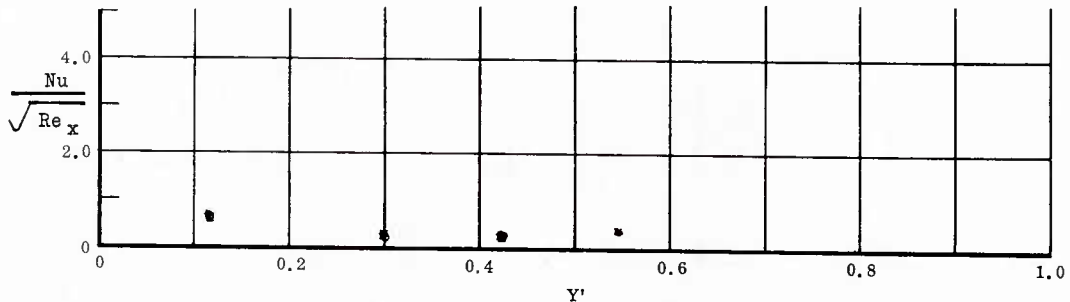
Fig. 22 Spanwise Distributions of Aerodynamic Heating Rates; Basic Configuration, Right (Upper) Flap Deflected -20^\circ , \alpha = 0^\circ , \beta = 0^\circ , Re_\infty/ft = 3,300,000 .
