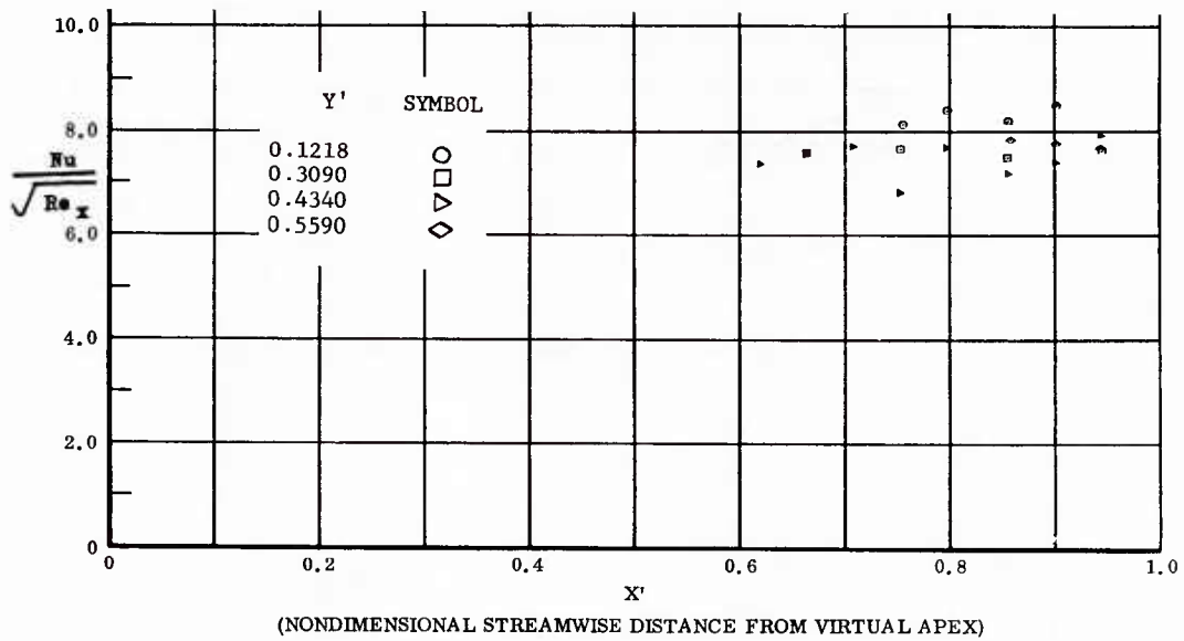
Fig. 73 Streamwise Distributions of Aerodynamic Heating Rates; Basic Configuration, No Flap Deflections, \alpha = +33^\circ , \beta = 0^\circ , Re_\infty/ft = 3,300,000 .
