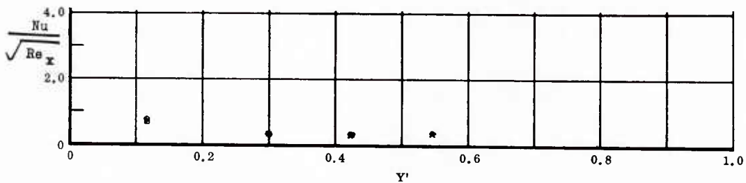
Fig. 14 Spanwise Distributions of Aerodynamic Heating Rates; Basic Configuration, Left and Right (Upper) Flaps Deflected -40^\circ , \alpha = 0^\circ , \beta = 0^\circ , Re_\infty/ft = 3,300,000 .
