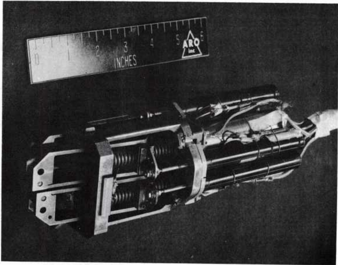
Fig. 4 Actuators for Remotely Controlled Flaps
