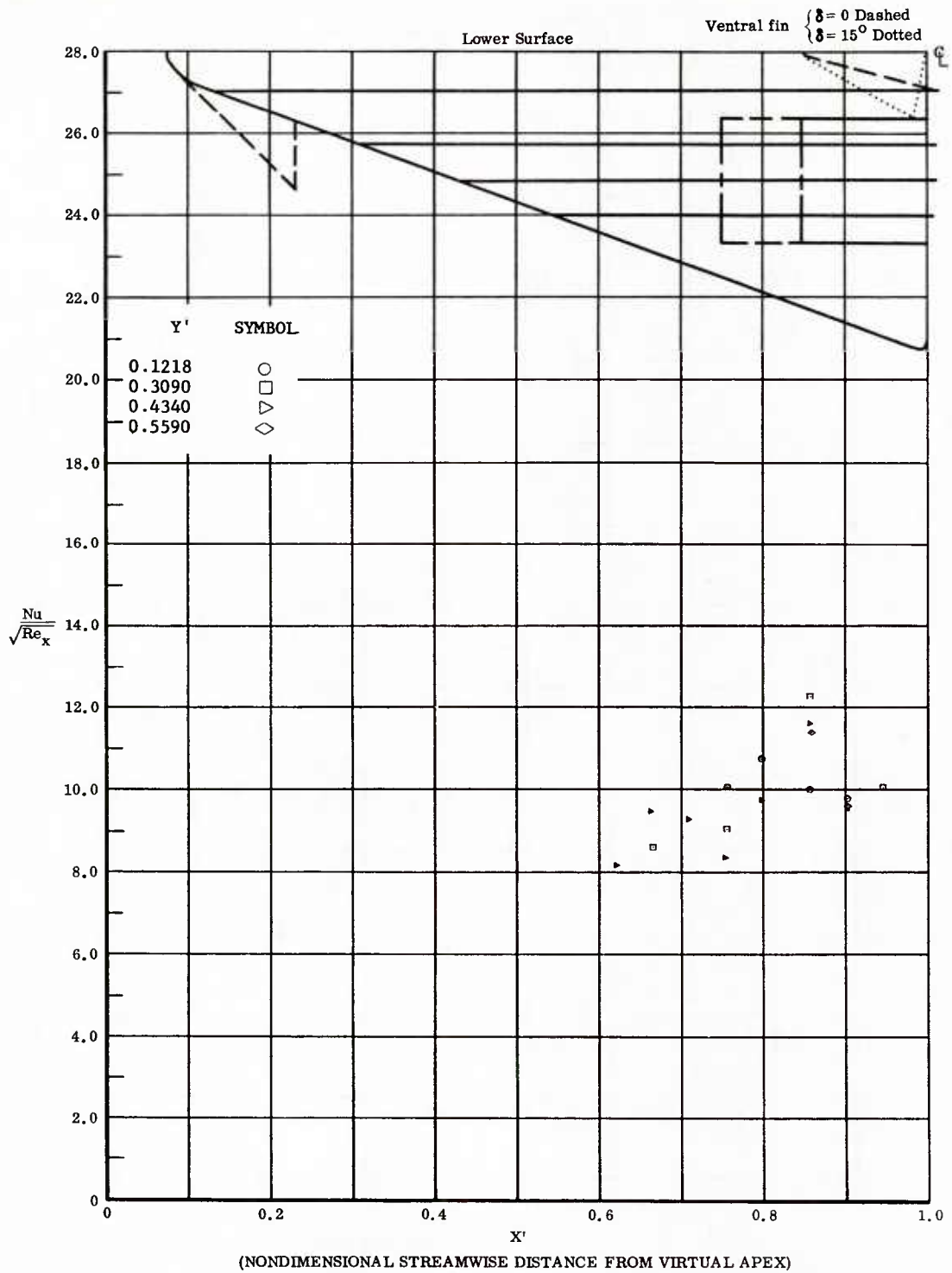
Fig. 81 Streamwise Distributions of Aerodynamic Heating Rates; Basic Configuration, Bottom Flaps Deflected +20°, \alpha = +54^\circ , \beta = 0^\circ , Re_\infty / ft = 3,300,000 .
