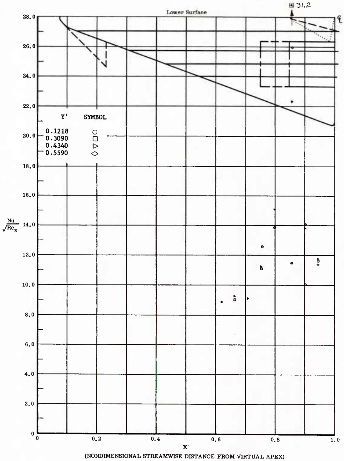
Fig. 79 Streamwise Distributions of Aerodynamic Heating Rates; Basic Configuration, Bottom Flaps Deflected +40°, \alpha = +45^\circ , \beta = 0^\circ , Re_\infty/ft = 3,300,000 .
