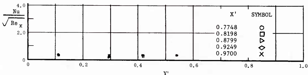
Fig. 9 Spanwise Distributions of Aerodynamic Heating Rates; Basic Configuration, No Flap Deflections, \alpha = -45^\circ , \beta = 0^\circ , Re_\infty/ft = 3,300,000 .
