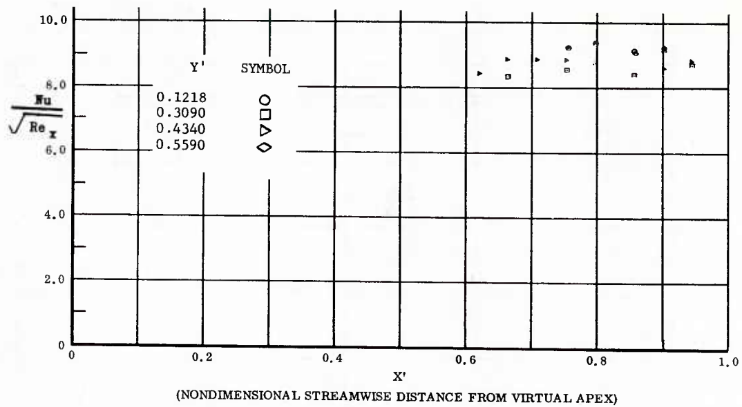
Fig. 77 Streamwise Distributions of Aerodynamic Heating Rates; Basic Configuration, No Flap Deflections, \alpha = +45^\circ , \beta = 0^\circ , Re_\infty/ft = 3,300,000 .
