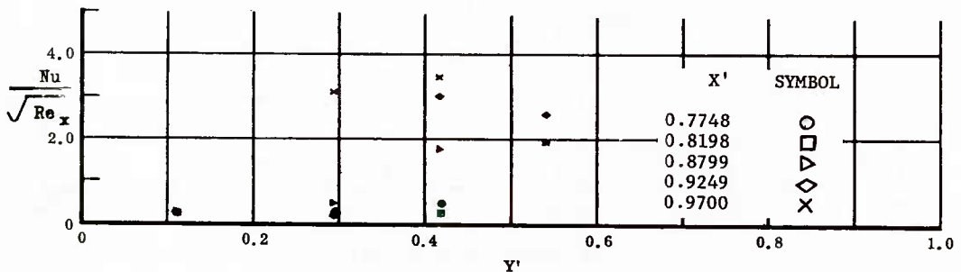
Fig. 42 Spanwise Distributions of Aerodynamic Heating Rates; Basic Configuration, Bottom Flaps Deflected +20^\circ , \alpha = 0^\circ , \beta = +12^\circ , Re_\infty/ft = 3,300,000 .
