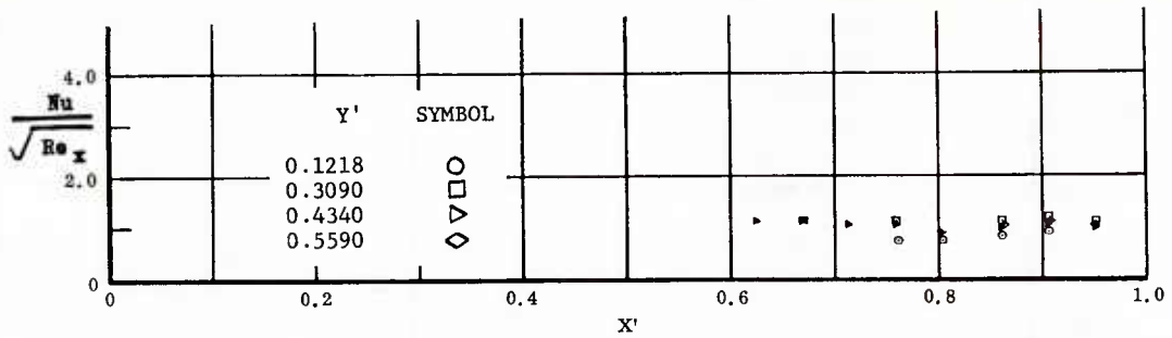
Fig. 53 Streamwise Distributions of Aerodynamic Heating Rates; Basic Configuration, Left and Right (Upper) Flaps Deflected -20^\circ , \alpha = +14.3^\circ , \beta = 0^\circ , Re_\infty/ft = 1,100,000 .
