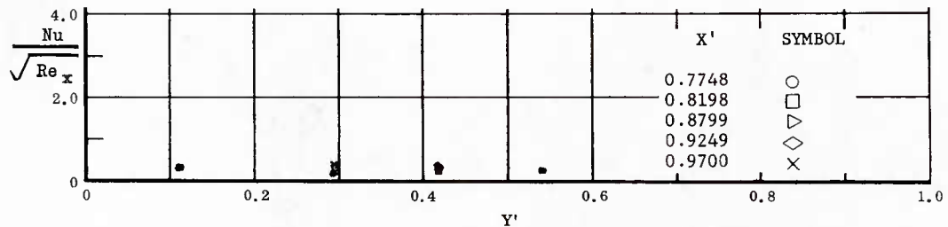
Fig. 7 Spanwise Distributions of Aerodynamic Heating Rates; Basic Configuration, Left and Right (Upper) Flaps Deflected -40^\circ , \alpha = -45^\circ , \beta = 0^\circ , Re_\infty/ft = 3,300,000 .
