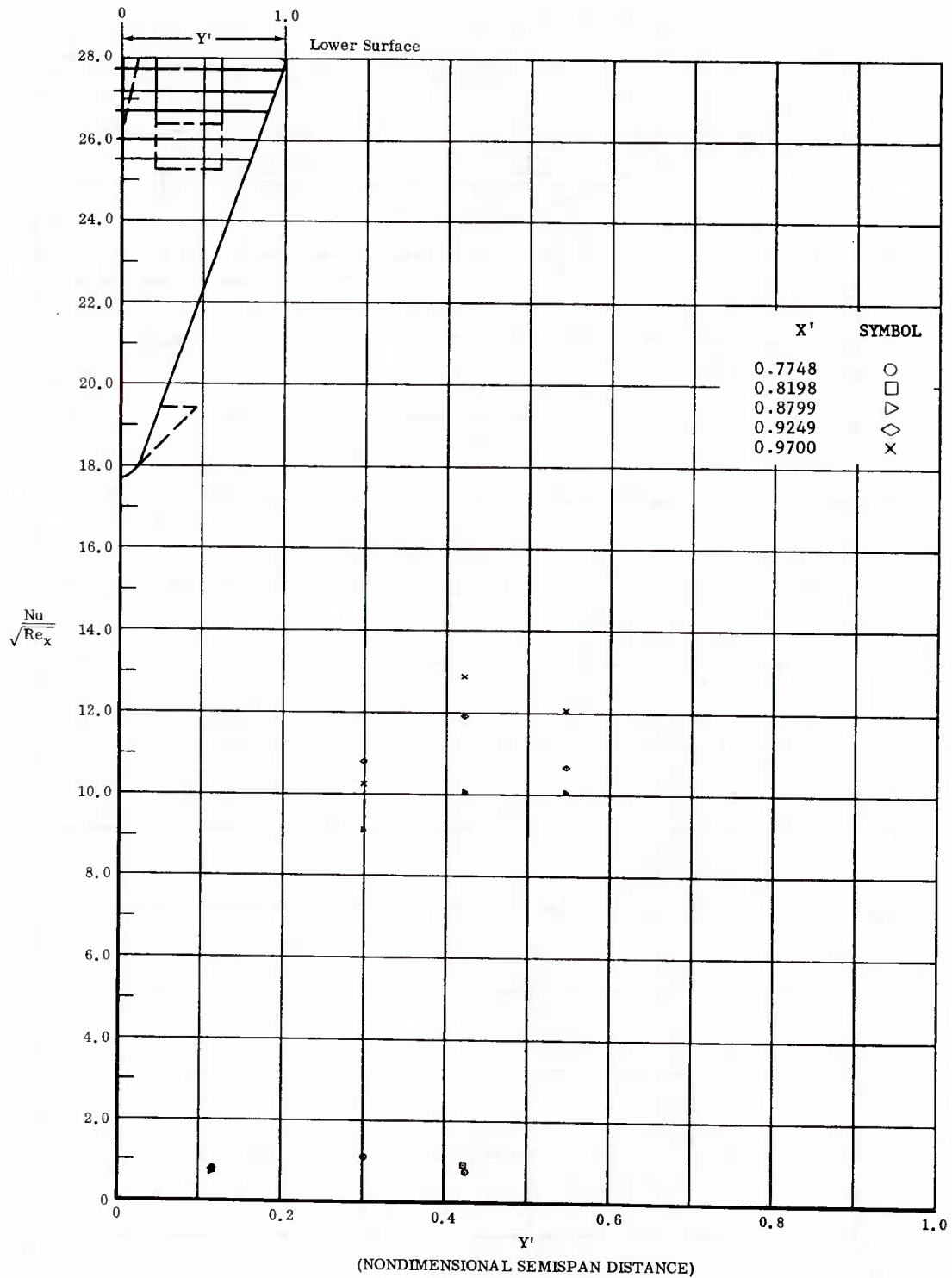
Fig. 63 Spanwise Distributions of Aerodynamic Heating Rates; Basic Configuration, Bottom Flaps Deflected +20°, \alpha = +14.3^\circ , \beta = 0^\circ , Re_\infty / ft = 1,100,000 .
