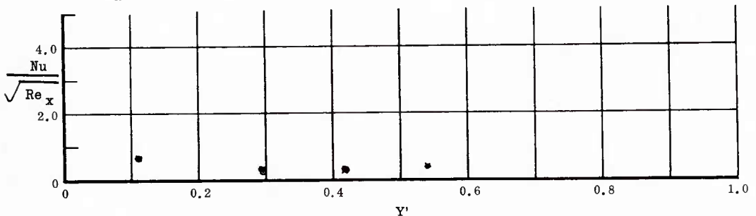
Fig. 20 Spanwise Distributions of Aerodynamic Heating Rates; Basic Configuration, Left and Right (Upper) Flaps Deflected -20^\circ , \alpha = 0^\circ , \beta = 0^\circ , Re_\infty/ft = 3,300,000 .
