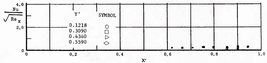
Fig. 8 Streamwise Distributions of Aerodynamic Heating Rates; Basic Configuration, Left and Right (Upper) Flaps Deflected -20^\circ , \alpha = -45^\circ , \beta = 0^\circ , Re_\infty/ft = 3,300,000 .
