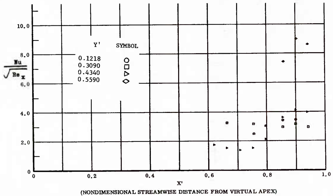
Fig. 57 Streamwise Distributions of Aerodynamic Heating Rates; Basic Configuration + Canards, Left and Right (Upper) Flaps Deflected -20^\circ , \alpha = +14.3^\circ , \beta = 0^\circ , Re_\infty/ft = 3,300,000 .
