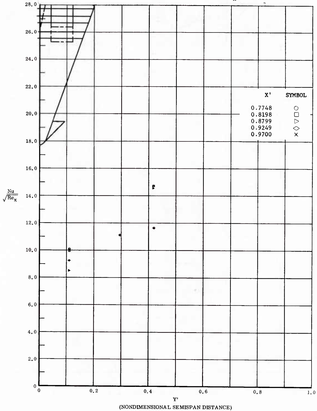
Fig. 71 Spanwise Distributions of Aerodynamic Heating Rates; Basic Configuration + Canards, Bottom Flaps Deflected +40°, \alpha = +14.3^\circ , \beta = 0^\circ , Re_\infty / ft = 3,300,000 .
