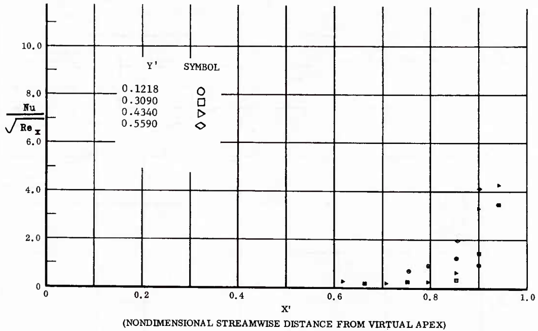
Fig. 32 Streamwise Distributions of Aerodynamic Heating Rates; Basic Configuration, Bottom Flaps Deflected +20°, \alpha = 0^\circ , \beta = 0^\circ , Re_\infty/ft = 3,300,000 .
