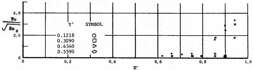
Fig. 42 Streamwise Distributions of Aerodynamic Heating Rates; Basic Configuration, Bottom Flaps Deflected +20^\circ , \alpha = 0^\circ , \beta = +12^\circ , Re_\infty/ft = 3,300,000 .
