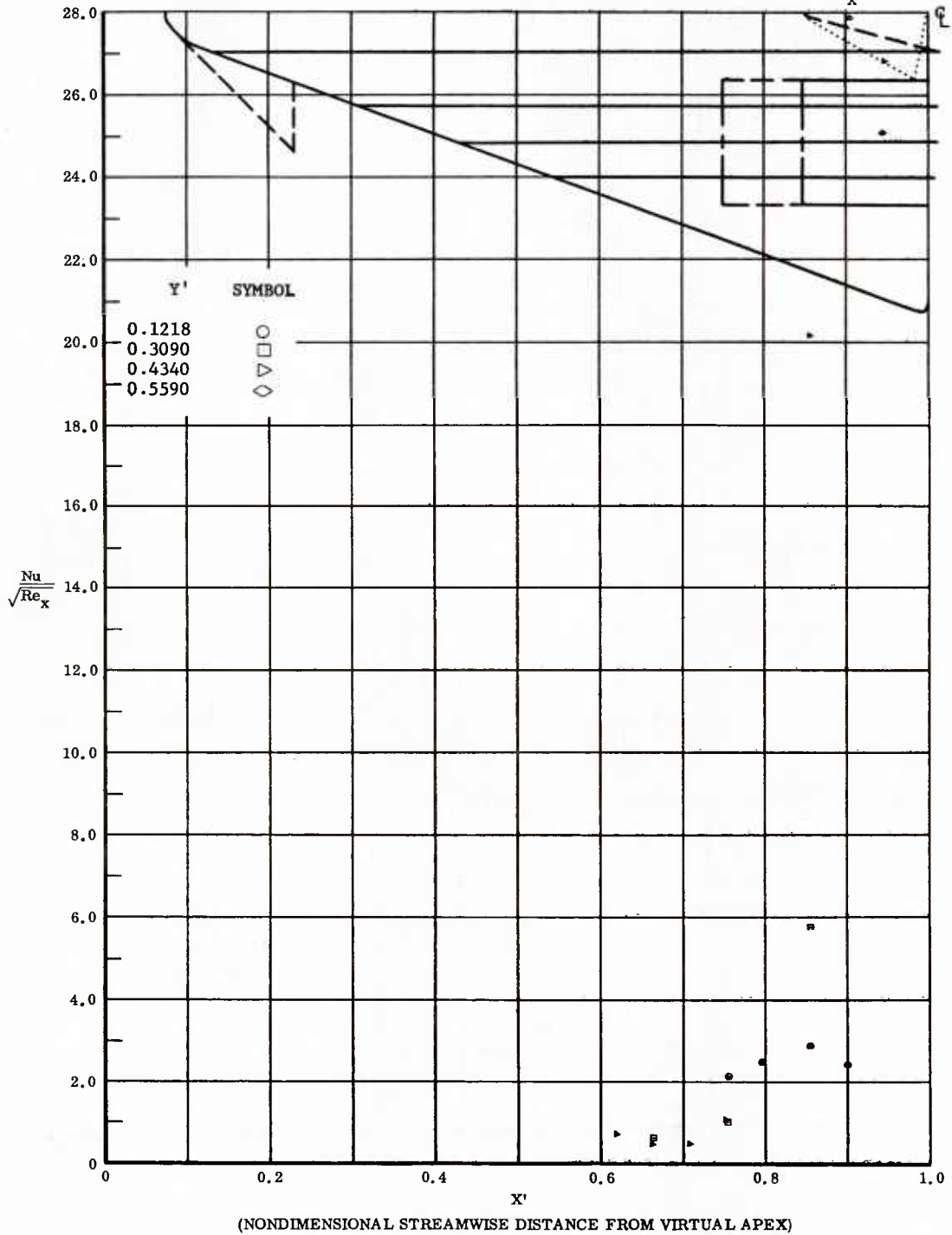
Fig. 40 Streamwise Distributions of Aerodynamic Heating Rates; Basic Configuration + Canards, Bottom Flaps Deflected +40°, \alpha = 0^\circ , \beta = 0^\circ , Re_\infty/ft = 3,300,000 .
