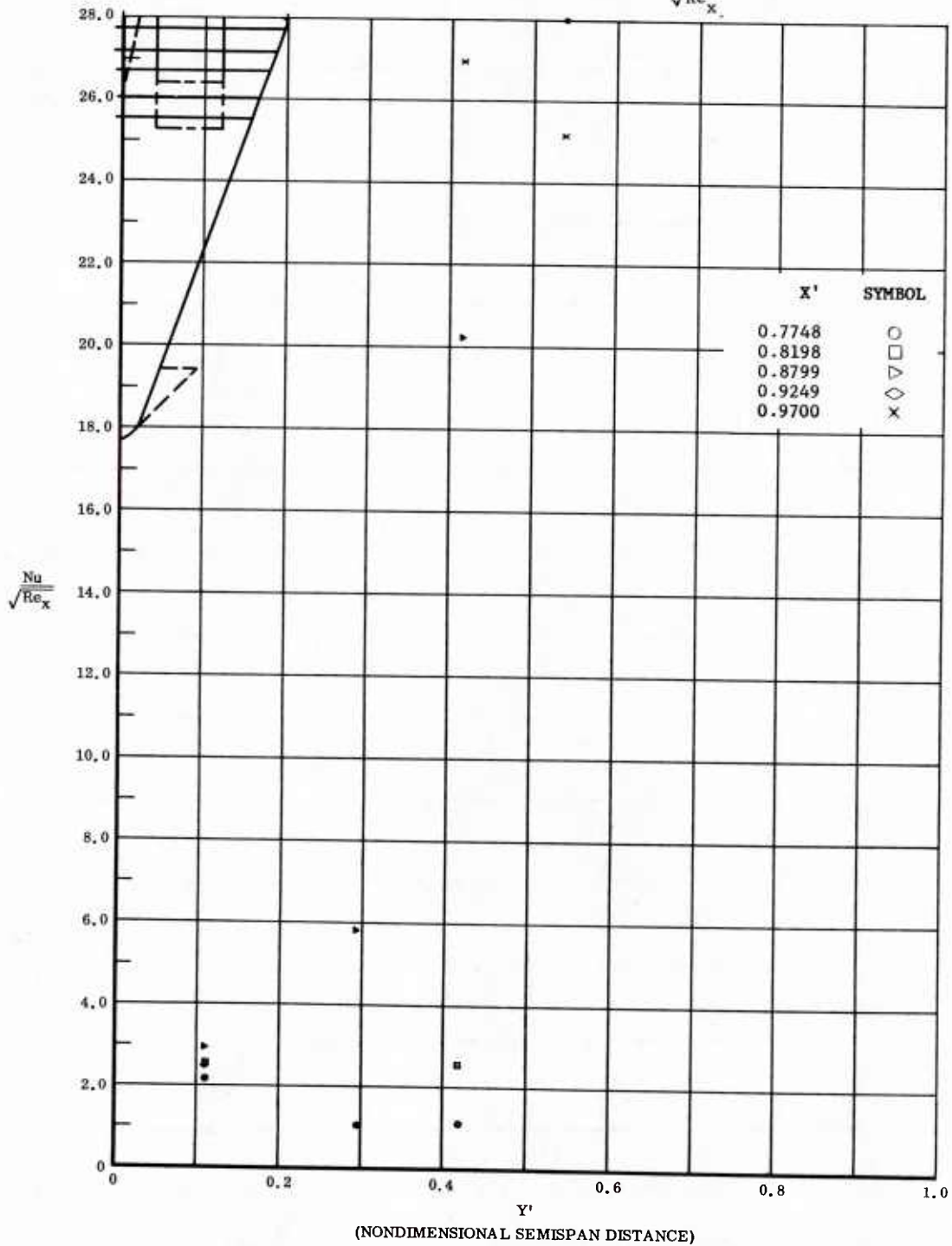
Fig. 40 Spanwise Distributions of Aerodynamic Heating Rates; Basic Configuration + Canards, Bottom Flaps Deflected +40°, \alpha = 0^\circ , \beta = 0^\circ , Re_\infty/ft = 3,300,000 .
