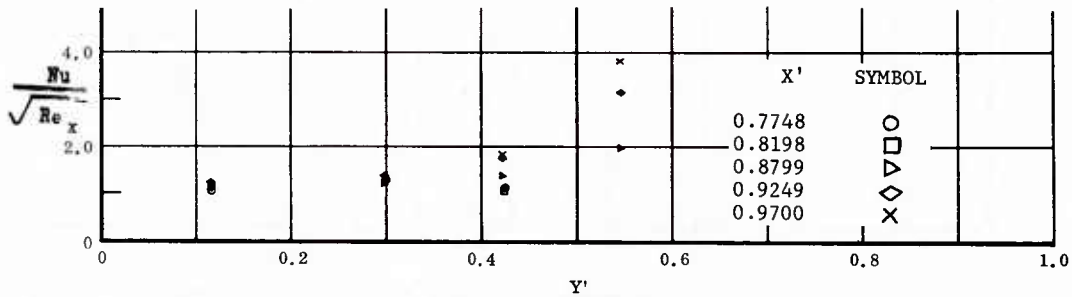
Fig. 49 Spanwise Distributions of Aerodynamic Heating Rates; Basic Configuration, Left (Upper) Flap Deflected -40^\circ , \alpha = +14.3^\circ , \beta = 0^\circ , Re_\infty/ft = 3,300,000 .
