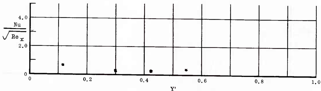
Fig. 18 Spanwise Distributions of Aerodynamic Heating Rates; Basic Configuration, Left and Right (Upper) Flaps Deflected -30^\circ , \alpha = 0^\circ , \beta = 0^\circ , Re_\infty/ft = 3,300,000 .
