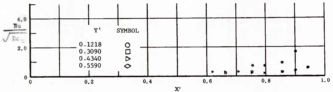
Fig. 28 Streamwise Distributions of Aerodynamic Heating Rates; Basic Configuration + Fin ( \delta = 0 ), No Flap Deflections, \alpha = 0^\circ , \beta = 0^\circ , Re_\infty/ft = 3,300,000 .
