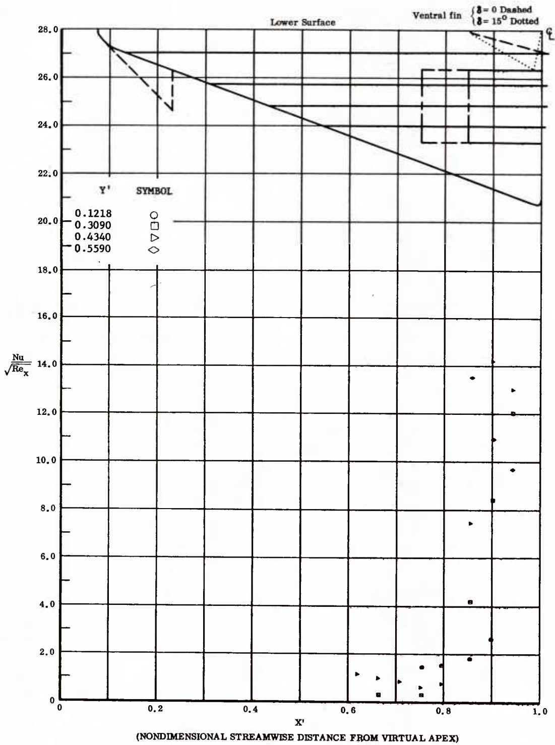
Fig. 33 Streamwise Distributions of Aerodynamic Heating Rates; Basic Configuration + Canards, Bottom Flaps Deflected +20°, \alpha = 0^\circ , \beta = 0^\circ , Re_\infty / ft = 3,300,000 .
