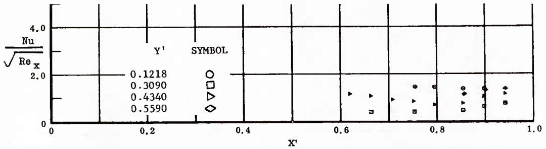
Fig. 27 Streamwise Distributions of Aerodynamic Heating Rates; Basic Configuration + Canards, No Flap Deflections, \alpha = 0^\circ , \beta = 0^\circ , Re_\infty/ft = 3,300,000 .
