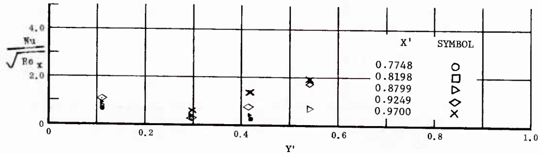
Fig. 30 Spanwise Distributions of Aerodynamic Heating Rates; Basic Configuration, Bottom Flaps Deflected +10^\circ , \alpha = 0^\circ , \beta = 0^\circ , Re_\infty/ft = 3,300,000 .
