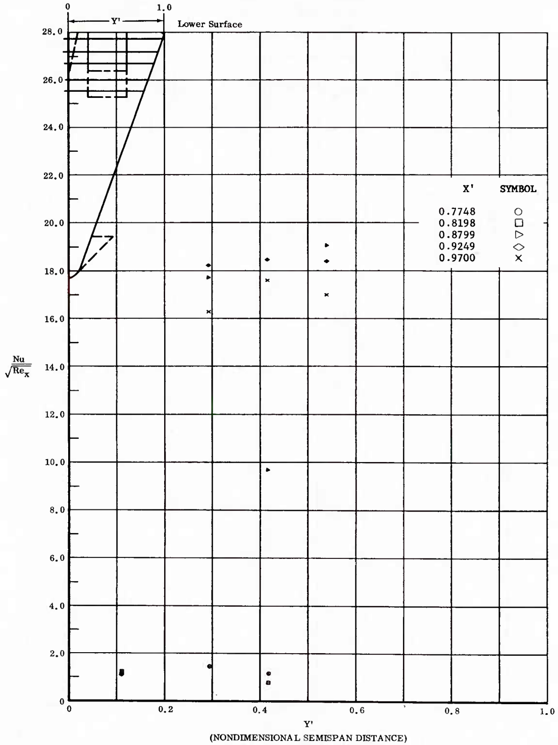
Fig. 64 Spanwise Distributions of Aerodynamic Heating Rates; Basic Configuration, Bottom Flaps Deflected +20°, \alpha = +14.3^\circ , \beta = 0^\circ , Re_\infty/ft = 3,300,000 .
