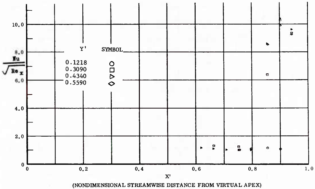
Fig. 62 Streamwise Distributions of Aerodynamic Heating Rates; Basic Configuration, Bottom Flaps Deflected +10°, \alpha = +14.3^\circ , \beta = 0^\circ , Re_\infty/ft = 3,300,000 .
