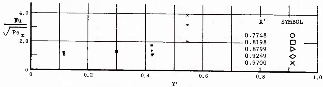
Fig. 50 Spanwise Distributions of Aerodynamic Heating Rates; Basic Configuration, Right (Upper) Flap Deflected -40^\circ , \alpha = +14.3^\circ , \beta = 0^\circ , Re_\infty/ft = 3,300,000 .
