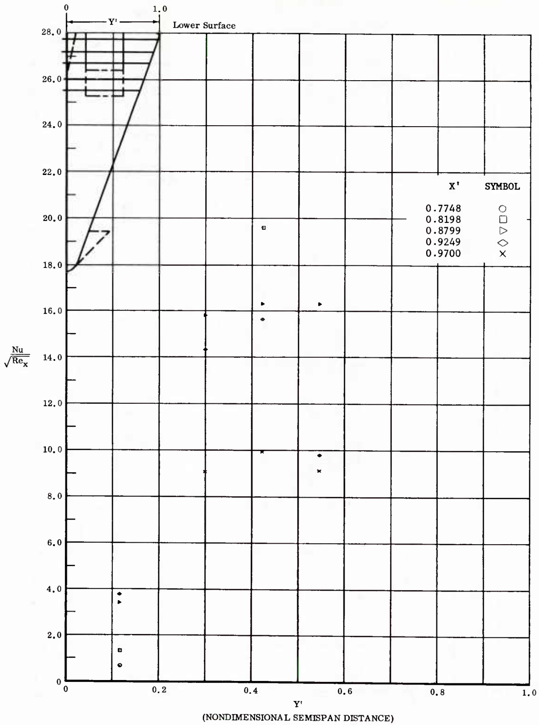
Fig. 67 Spanwise Distributions of Aerodynamic Heating Rates; Basic Configuration + Longer Chord Flaps, Bottom Flaps Deflected +20°, \beta = 0^\circ , \alpha = +14.3^\circ , Re_\infty/ft = 3,300,000 .
