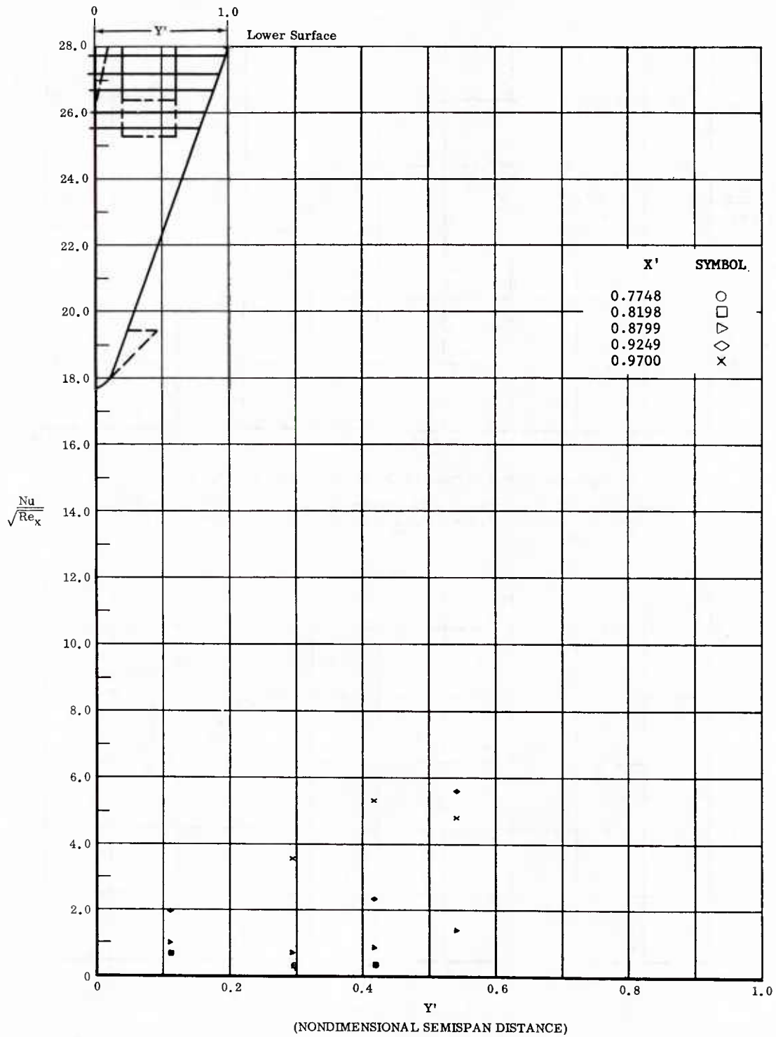
Fig. 34 Spanwise Distributions of Aerodynamic Heating Rates; Basic Configuration + Fin ( \delta = 0 ), Bottom Flaps Deflected +20^\circ , \alpha = 0^\circ , \beta = 0^\circ , Re_\infty/ft = 3,300,000 .
