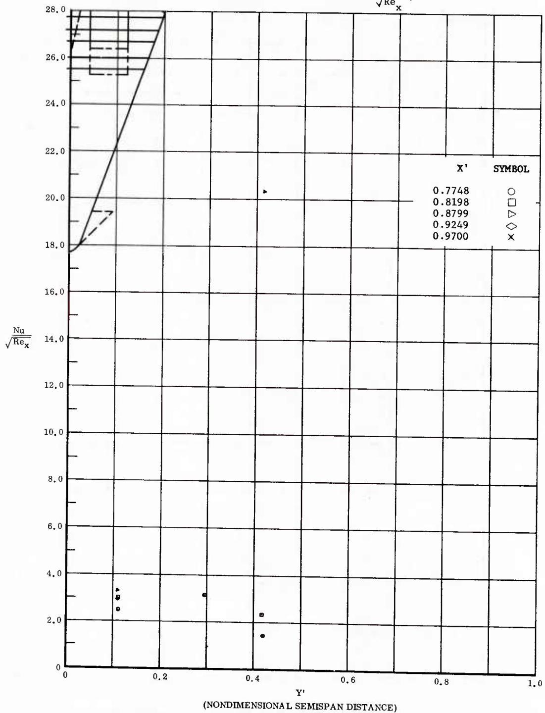
Fig. 65 Spanwise Distributions of Aerodynamic Heating Rates; Basic Configuration + Canards, Bottom Flaps Deflected +20°, \alpha = +14.3^\circ , \beta = 0^\circ , Re_\infty / ft = 3,300,000 .
