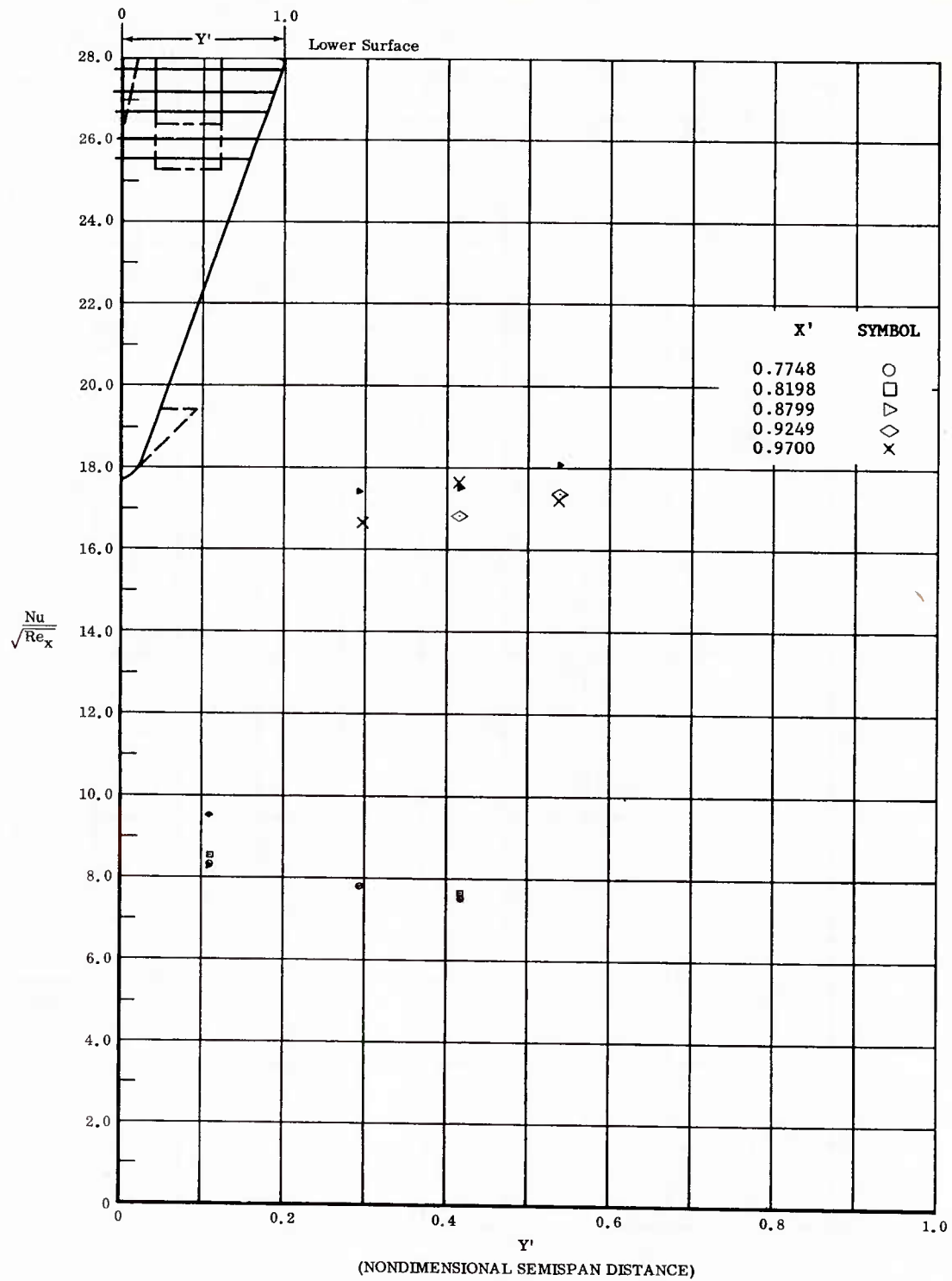
Fig. 74 Spanwise Distributions of Aerodynamic Heating Rates; Basic Configuration, Bottom Flaps Deflected +20°, \alpha = +33^\circ , \beta = 0^\circ , Re_\infty / ft = 3,300,000 .
