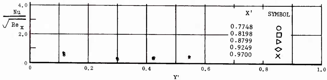
Fig. 13 Spanwise Distributions of Aerodynamic Heating Rates; Basic Configuration, Left and Right (Upper) Flaps Deflected -40^\circ , \alpha = 0^\circ , \beta = 0^\circ , Re_\infty/ft = 1,100,000 .
