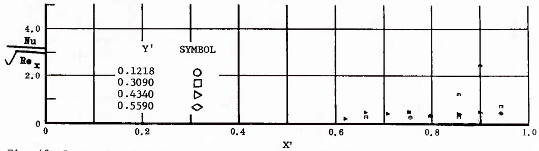
Fig. 43 Streamwise Distributions of Aerodynamic Heating Rates; Basic Configuration + Fin ( \delta = 0 ), No Flap Deflections, \alpha = 0^\circ , \beta = +12^\circ , Re_\infty/ft = 3,300,000 .
