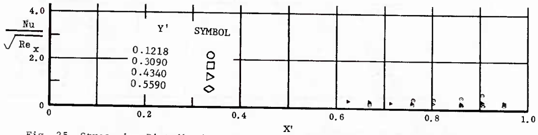
Fig. 25 Streamwise Distributions of Aerodynamic Heating Rates; Basic Configuration, No Flap Deflections, \alpha = 0^\circ , \beta = 0^\circ , Re_\infty/ft = 1,100,000 .
