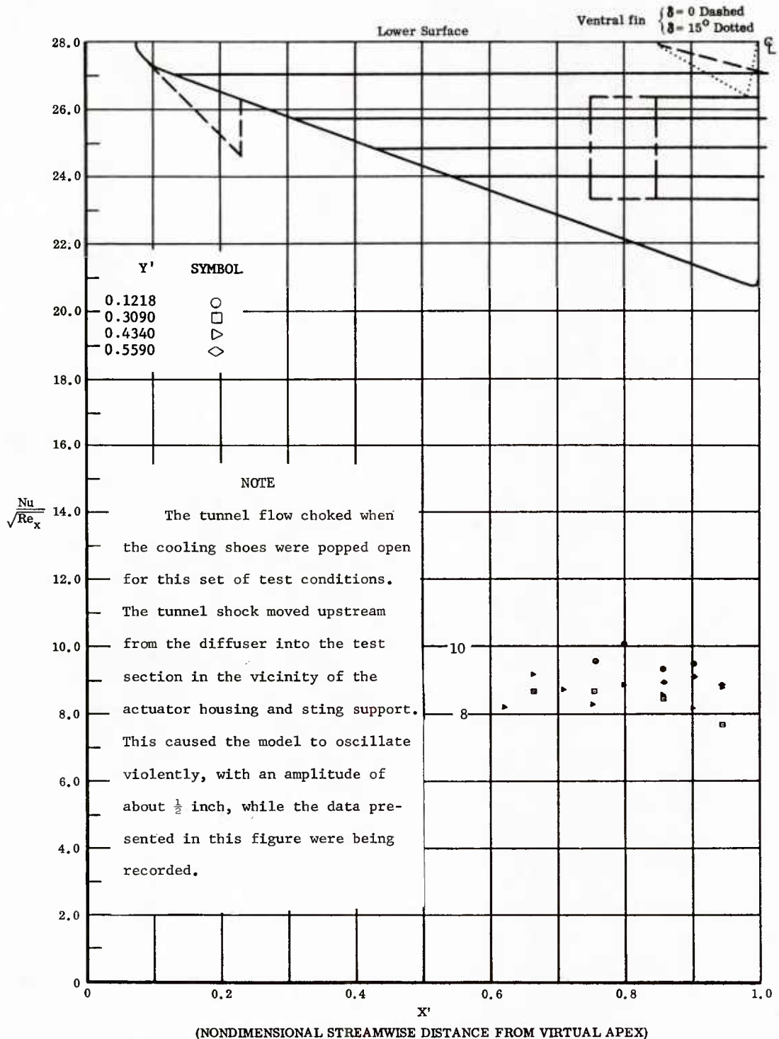
Fig. 80 Streamwise Distributions of Aerodynamic Heating Rates; Basic Configuration, Left and Right (Upper) Flaps Deflected -40^\circ , \alpha = +54^\circ , \beta = 0^\circ , Re_\infty / ft = 7 .
