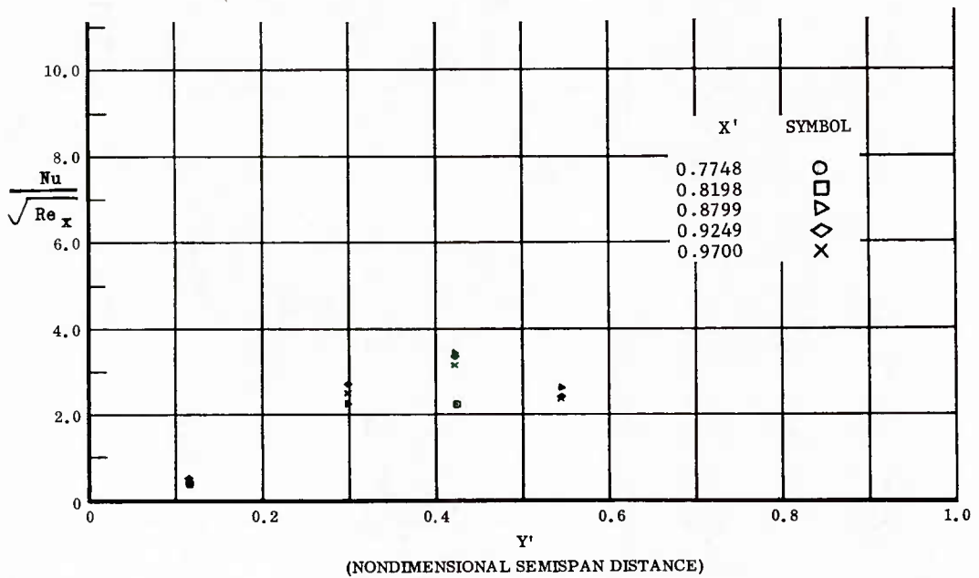
Fig. 35 Spanwise Distributions of Aerodynamic Heating Rates; Basic Configuration + Longer Chord Flaps, Bottom Flaps Deflected +20°, \alpha = 0^\circ , \beta = 0^\circ , Re_\infty/ft = 1,100,000 .
