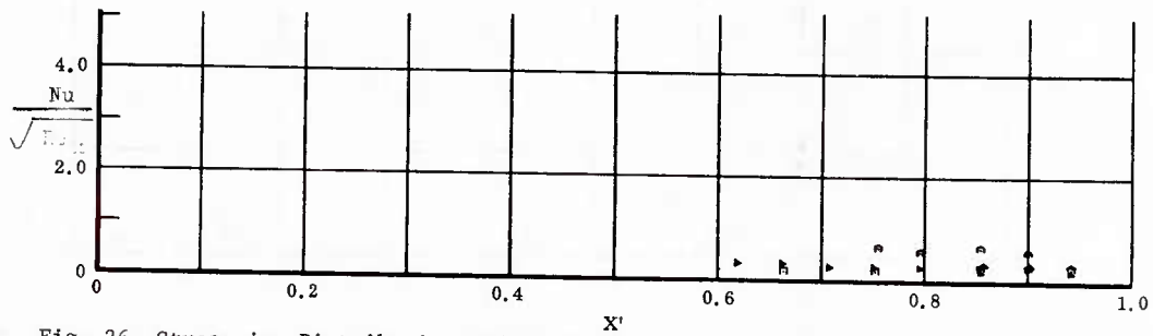
Fig. 26 Streamwise Distributions of Aerodynamic Heating Rates; Basic Configuration, No Flap Deflections, \alpha = 0^\circ , \beta = 0^\circ , Re_\infty/ft = 3,300,000 .
