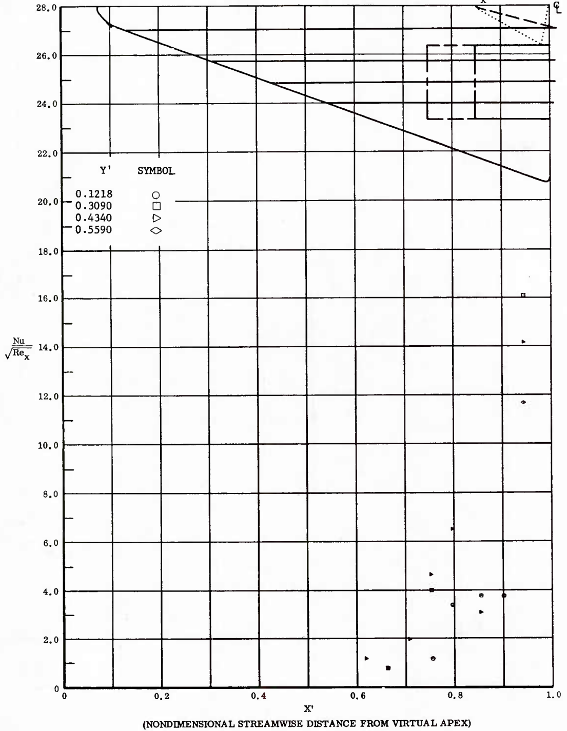
Fig. 70 Streamwise Distributions of Aerodynamic Heating Rates; Basic Configuration, Bottom Flaps Deflected +40°, \alpha = +14.3^\circ , \beta = 0^\circ , Re_\infty / ft = 3,300,000 .
