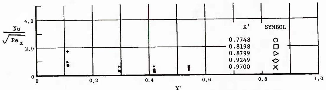
Fig. 28 Spanwise Distributions of Aerodynamic Heating Rates; Basic Configuration + Fin ( \delta = 0 ), No Flap Deflections, \alpha = 0^\circ , \beta = 0^\circ , Re_\infty/ft = 3,300,000 .
