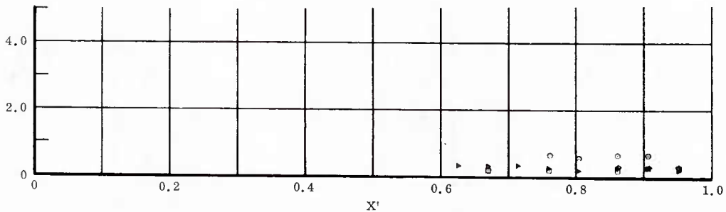
Fig. 22 Streamwise Distributions of Aerodynamic Heating Rates; Basic Configuration, Right (Upper) Flap Deflected -20^\circ , \alpha = 0^\circ , \beta = 0^\circ , Re_\infty/ft = 3,300,000 .
