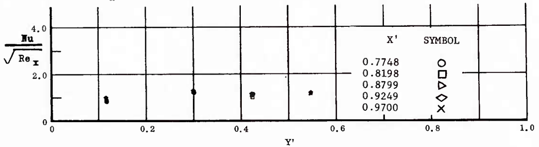
Fig. 53 Spanwise Distributions of Aerodynamic Heating Rates; Basic Configuration, Left and Right (Upper) Flaps Deflected -20^\circ , \alpha = +14.3^\circ , \beta = 0^\circ , Re_\infty/ft = 1,100,000 .
