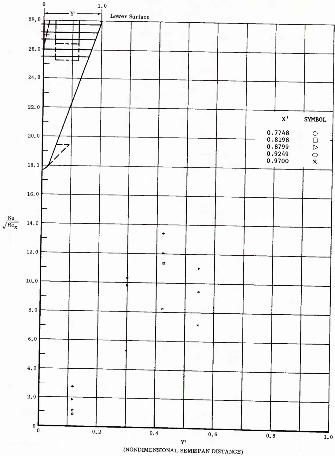
Fig. 66 Spanwise Distributions of Aerodynamic Heating Rates; Basic Configuration + Longer Chord Flaps, Bottom Flaps Deflected +20°, \alpha = +14.3^\circ , \beta = 0^\circ , Re_\infty/ft = 1,100,000 .
