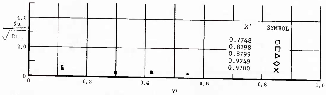
Fig. 25 Spanwise Distributions of Aerodynamic Heating Rates; Basic Configuration, No Flap Deflections, \alpha = 0^\circ , \beta = 0^\circ , Re_\infty/ft = 1,100,000 .
