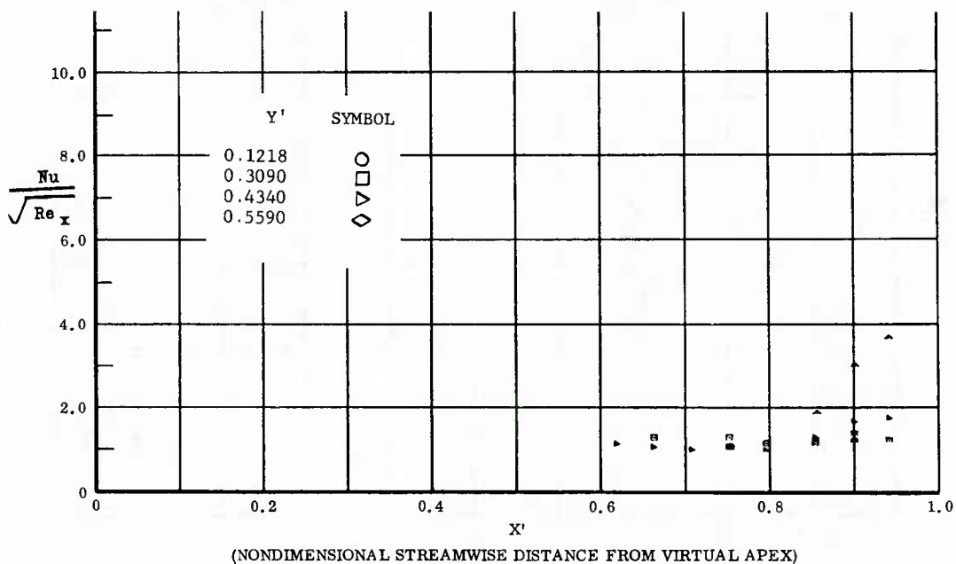
Fig. 60 Streamwise Distributions of Aerodynamic Heating Rates; Basic Configuration, No Flap Deflections, \alpha = +14.3^\circ , \beta = 0^\circ , Re_\infty / ft = 3,300,000 .
