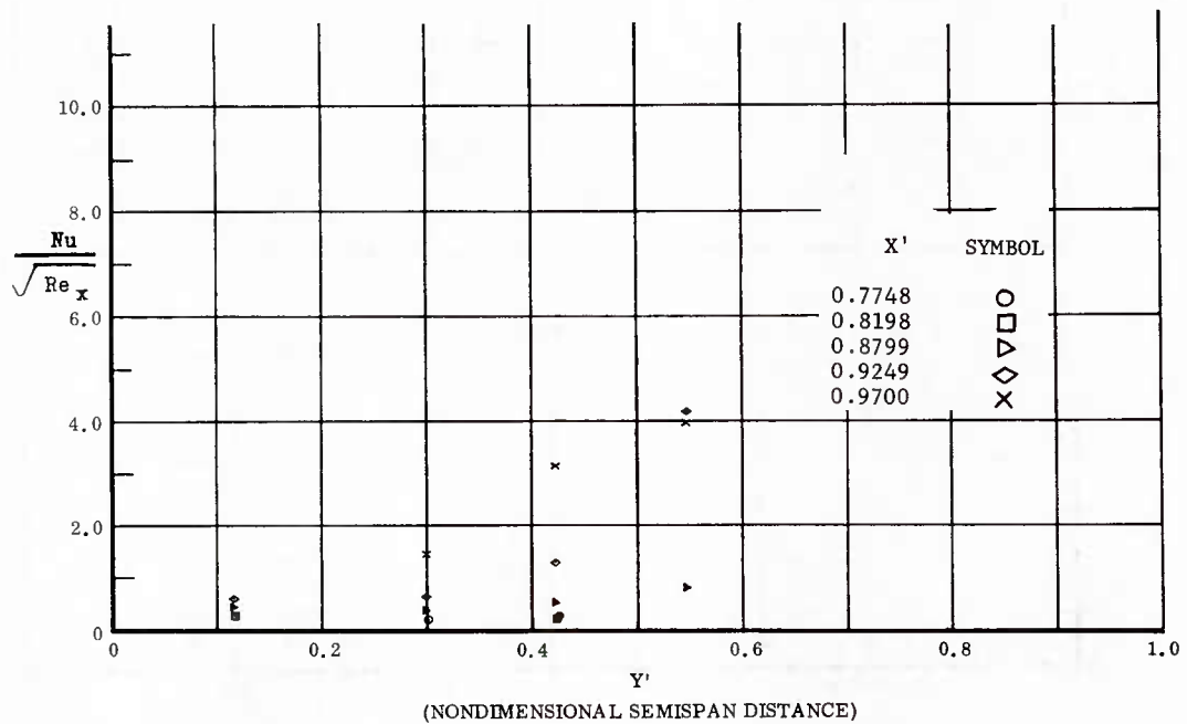
Fig. 31 Spanwise Distributions of Aerodynamic Heating Rates; Basic Configuration, Bottom Flaps Deflected +20°, \alpha = 0^\circ , \beta = 0^\circ , Re_\infty/ft = 1,100,000 .
