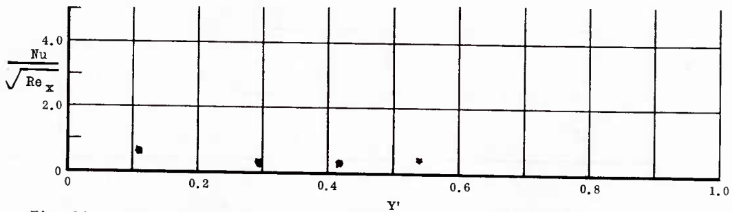
Fig. 26 Spanwise Distributions of Aerodynamic Heating Rates; Basic Configuration, No Flap Deflections, \alpha = 0^\circ , \beta = 0^\circ , Re_\infty/ft = 3,300,000 .
