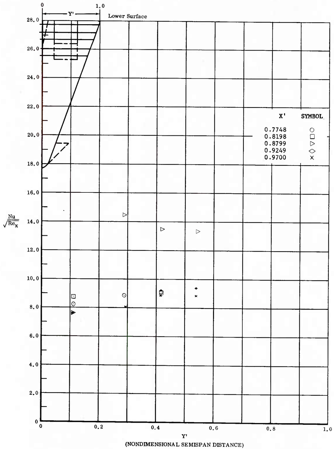
Fig. 82 Spanwise Distributions of Aerodynamic Heating Rates; Basic Configuration, Bottom Flaps Deflected +40°, \alpha = +54^\circ , \beta = 0^\circ , Re_\infty/\bar{t} = 3,300,000 .
