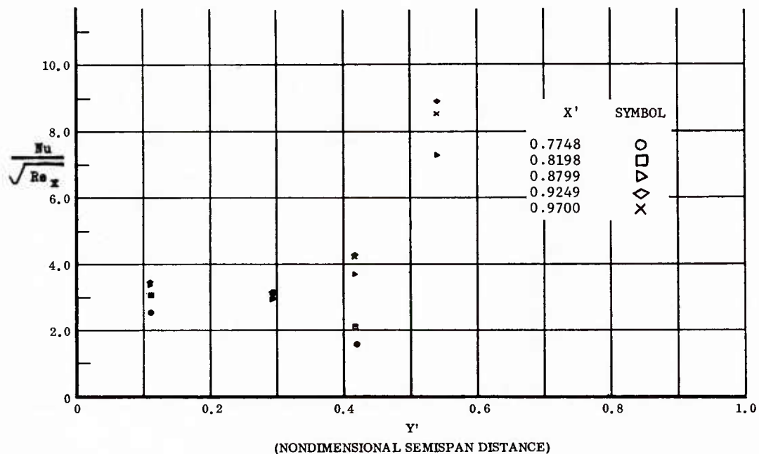
Fig. 51 Spanwise Distributions of Aerodynamic Heating Rates; Basic Configuration + Canards, Left and Right (Upper) Flaps Deflected -40^\circ , \alpha = +14.3^\circ , \beta = 0^\circ , Re_\infty/ft = 3,300,000 .
