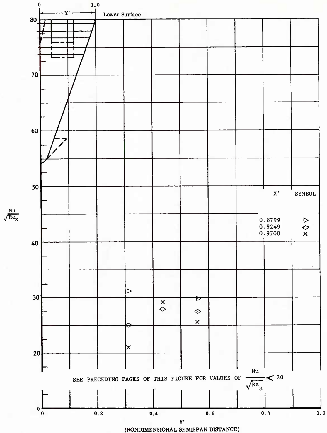
Fig. 68 Spanwise Distributions of Aerodynamic Heating Rates; Basic Configuration, Bottom Flaps Deflected +30°, \alpha = +14.3^\circ , \beta = 0^\circ , Re_\infty/ft = 3,300,000 .
