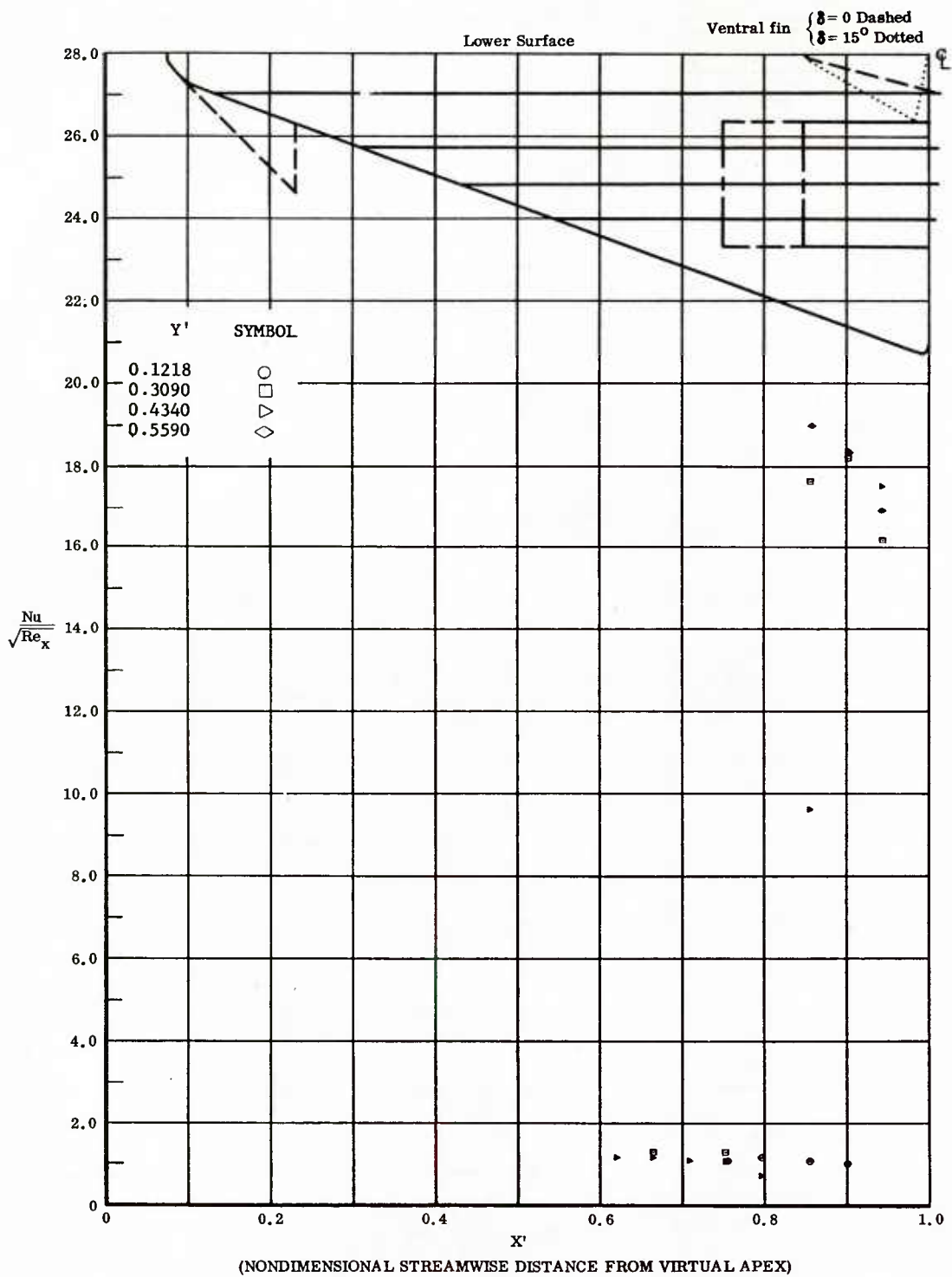
Fig. 64 Streamwise Distributions of Aerodynamic Heating Rates; Basic Configuration, Bottom Flaps Deflected +20^\circ , \alpha = +14.3^\circ , \beta = 0^\circ , Re_\infty/ft = 3,300,000 .
