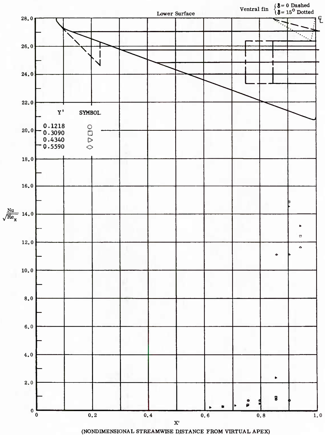
Fig. 39 Streamwise Distributions of Aerodynamic Heating Rates; Basic Configuration, Bottom Flaps Deflected +40°, \alpha = 0^\circ , \beta = 0^\circ , Re_\infty / ft = 3,300,000 .
