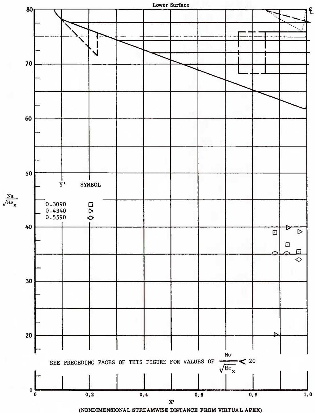
Fig. 65 Streamwise Distributions of Aerodynamic Heating Rates; Basic Configuration + Canards, Bottom Flaps Deflected +20°, \alpha = +14.3^\circ , \beta = 0^\circ , Re_\infty/ft = 3,300,000 .
