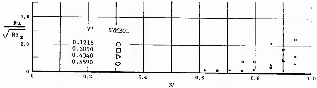
Fig. 29 Streamwise Distributions of Aerodynamic Heating Rates; Basic Configuration + Fin ( \delta = 15^\circ ), No Flap Deflections, \alpha = 0^\circ , \beta = 0^\circ , Re_\infty/ft = 3,300,000 .
