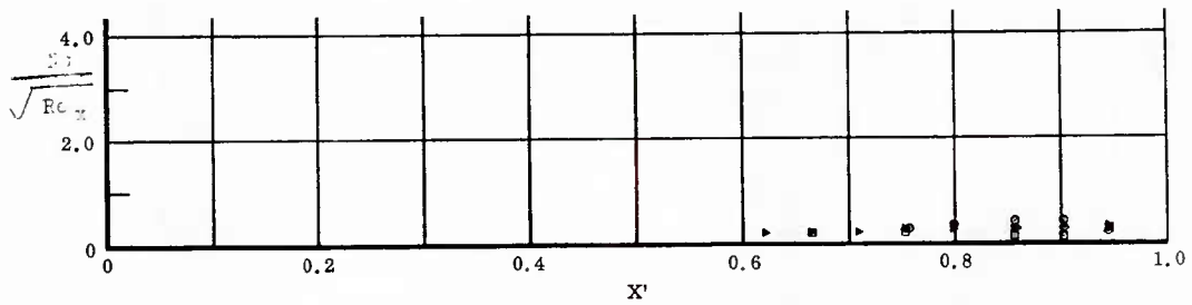
Fig. 11 Streamwise Distributions of Aerodynamic Heating Rates; Basic Configuration, Left and Right (Upper) Flaps Deflected -40^\circ , \alpha = -33^\circ , \beta = 0^\circ , Re_\infty/ft = 3,300,000 .
