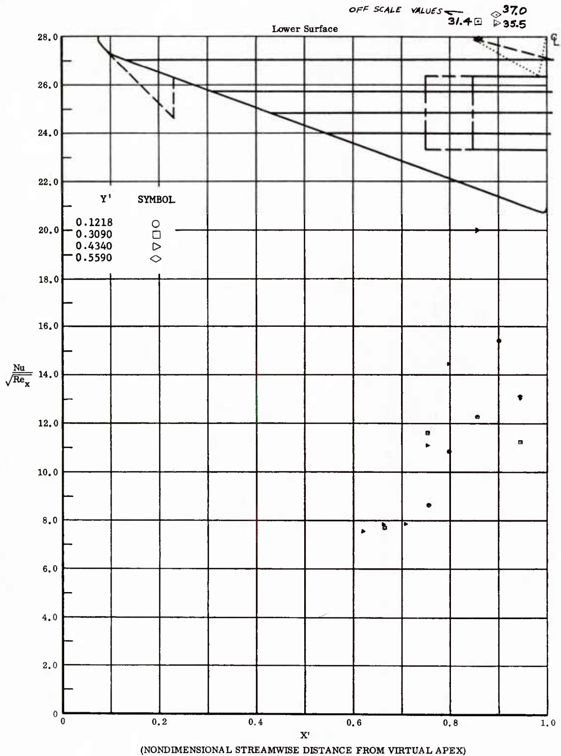
Fig. 75 Streamwise Distributions of Aerodynamic Heating Rates; Basic Configuration, Bottom Flaps Deflected +40°, \alpha = +33^\circ , \beta = 0^\circ , Re_\infty / l_t = 3,300,000 .
