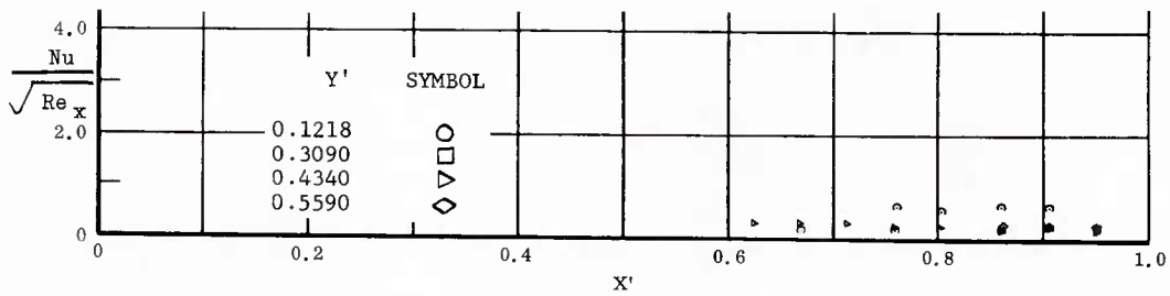
Fig. 21 Streamwise Distributions of Aerodynamic Heating Rates; Basic Configuration, Left (Upper) Flap Deflected -20^\circ , \alpha = 0^\circ , \beta = 0^\circ , Re_\infty/ft = 3,300,000 .
