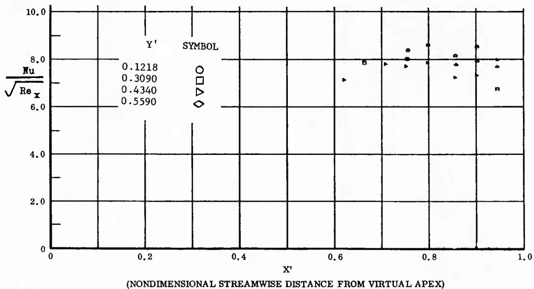
Fig. 72 Streamwise Distributions of Aerodynamic Heating Rates; Basic Configuration, Left and Right (Upper) Flaps Deflected -40^\circ , \alpha = +33^\circ , \beta = 0^\circ , Re_\infty / ft = 3,300,000 .
