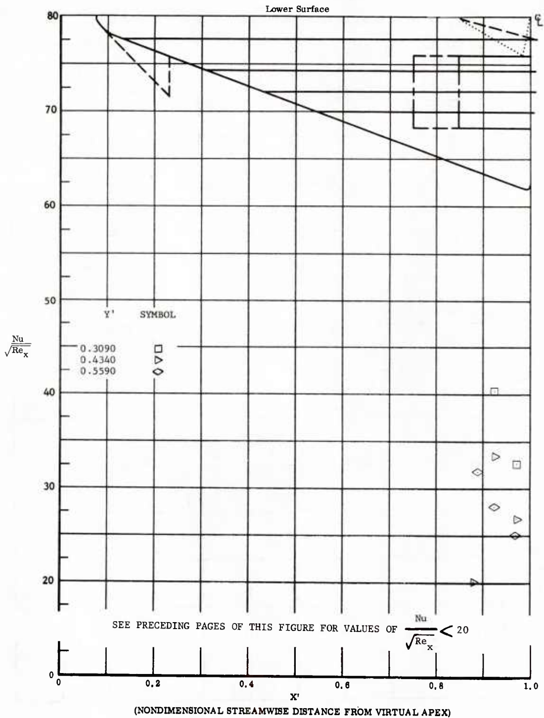
Fig. 40 Streamwise Distributions of Aerodynamic Heating Rates; Basic Configuration + Canards, Bottom Flaps Deflected +40°, \alpha = 0^\circ , \beta = 0^\circ , Re_\infty/ft = 3,300,000 .
