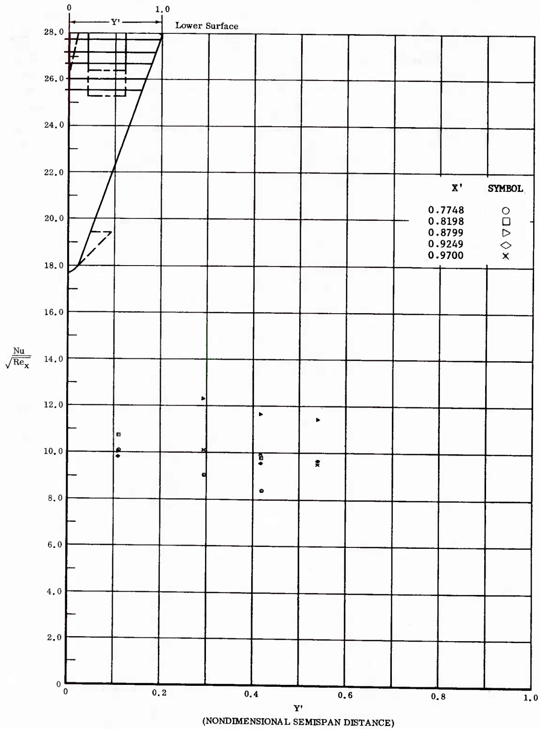
Fig. 81 Spanwise Distributions of Aerodynamic Heating Rates; Basic Configuration, Bottom Flaps Deflected +20°, \alpha = +54^\circ , \beta = 0^\circ , Re_\infty/ft = 3,300,000 .
