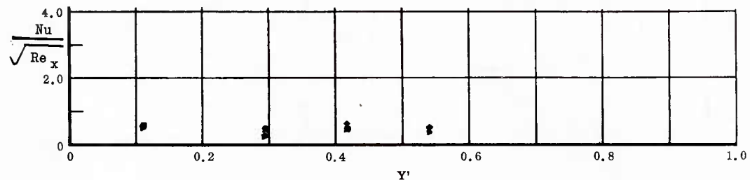
Fig. 12 Spanwise Distributions of Aerodynamic Heating Rates; Basic Configuration, No Flap Deflections, \alpha = -33^\circ , \beta = 0^\circ , Re_\infty/ft = 3,300,000 .
