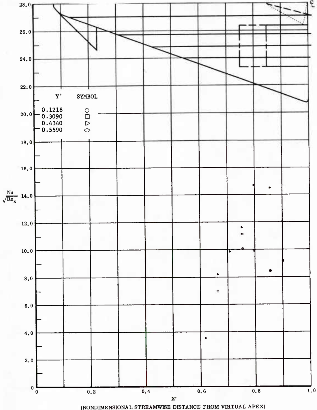
Fig. 71 Streamwise Distributions of Aerodynamic Heating Rates; Basic Configuration + Canards, Bottom Flaps Deflected +40°, \alpha = +14.3^\circ , \beta = 0^\circ , Re_\infty/ft = 3,300,000 .
