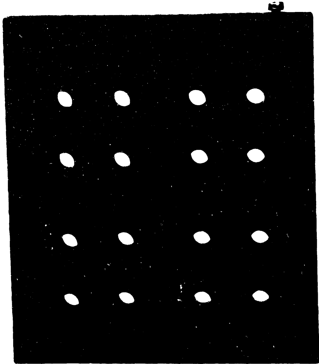
Figure 3. Carbon grid, 4" x 4" x 1/4", used in electrical resistivity study.
