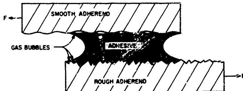
Fig. 4 - Effect of surface roughness on coplanarity of gas bubbles
