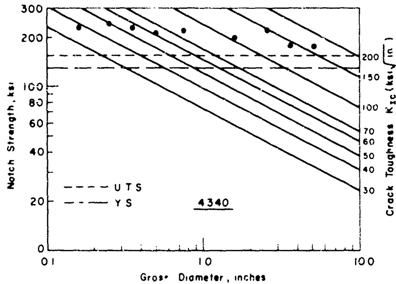
Figure 7. NOTCH STRENGTH VERSUS SECTION SIZE OF AISI 4340 WITH K_{Ic} AS THE PARAMETER
