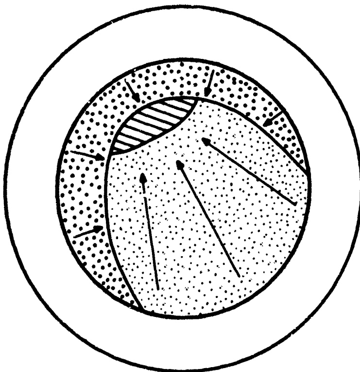
Figure 9A. FRACTURE SURFACE MARKINGS IN NOTCH ROUND SPECIMENS OF AISI 4340 STEEL
