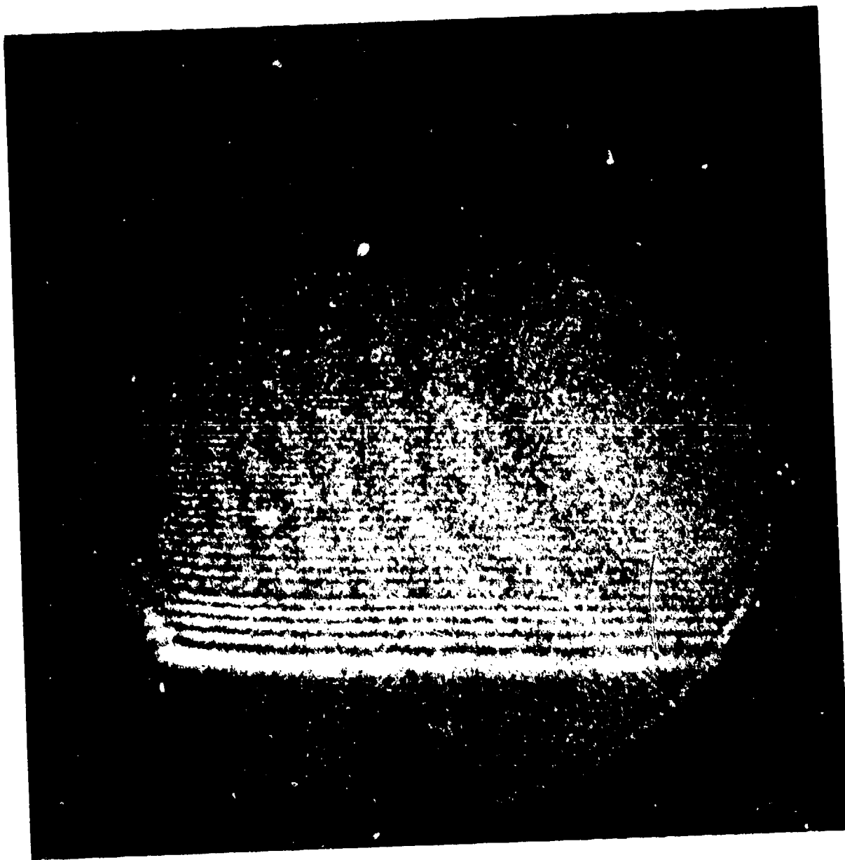
(U) Figure 3.16 Interferogram (6328.A) of Flowing Cryogenic Carbon Monoxide Laser System. P(N_2) = 380 torr, P(Ar) = 165 torr, \dot{m}(N_2) = 2.92 g/sec, \dot{m}(Ar) = 5.43 g/sec T \approx 80^\circ K . (U)
