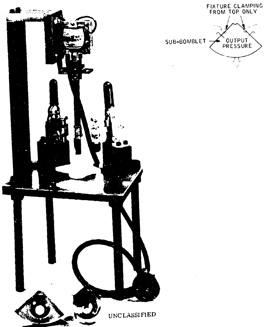
Figure 45. Redesigned Sub-bomblet Static Test Fixture
