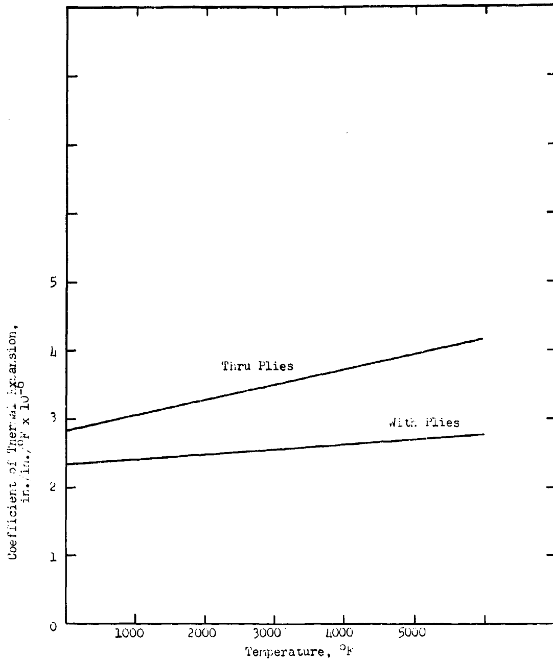
Figure 3 Coefficient of Thermal Expansion for Carborex-700
