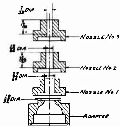
Rotating Rod Turbulence Creator Assembly
