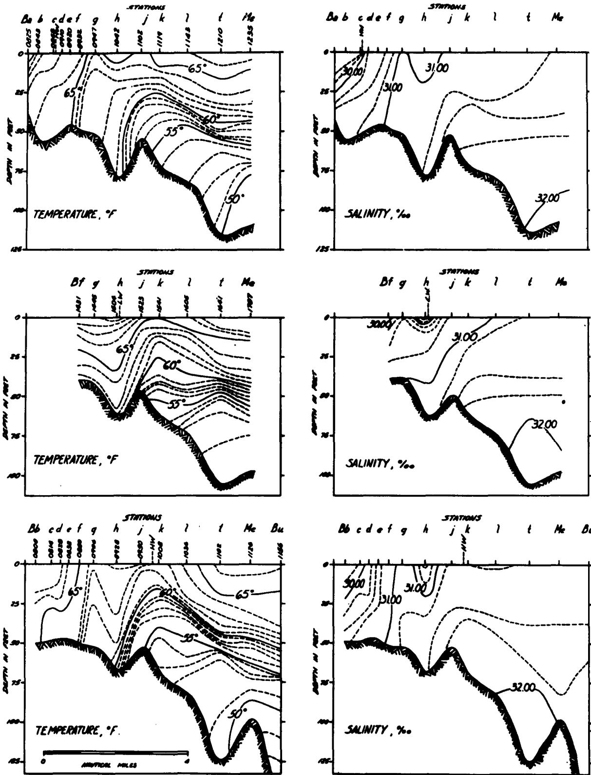
Fig. 7 Distribution of temperature and salinity near time of high water (upper figures) and low water (middle figures) on 12 September and high water (lower figures) on 13 September 1951. HAZEL III - Cruise 6.
