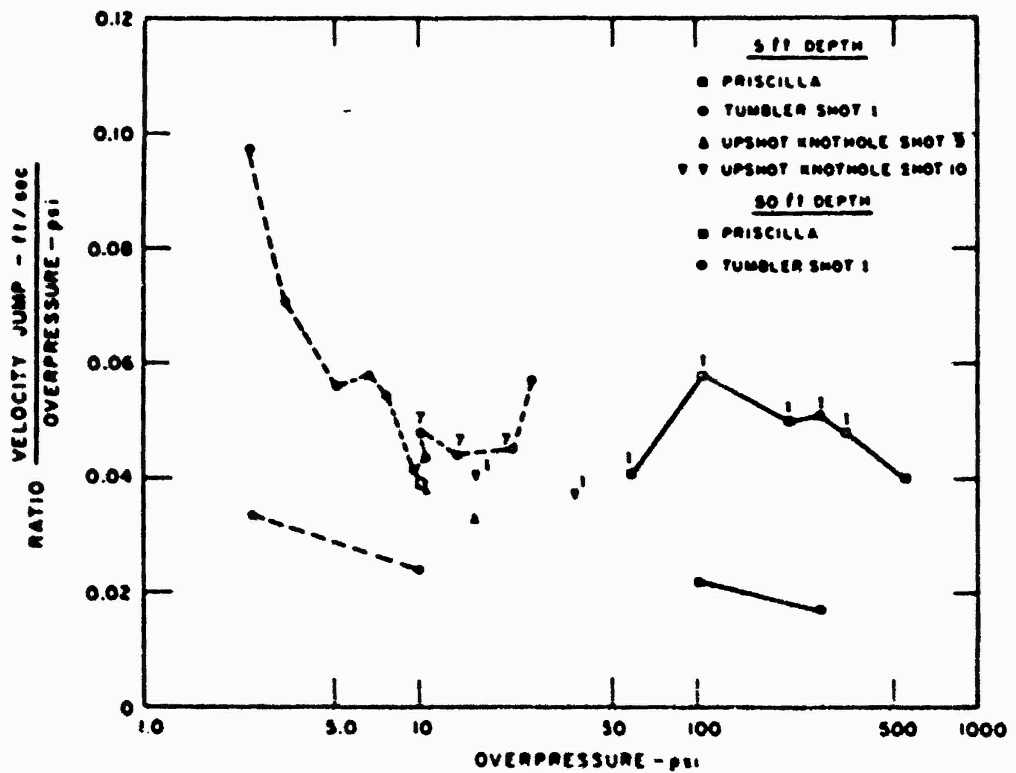
Figure 4.32 Vertical velocity, Frenchman Flat, 5-foot depth (numbers adjacent to data indicate overpressure wave form).
