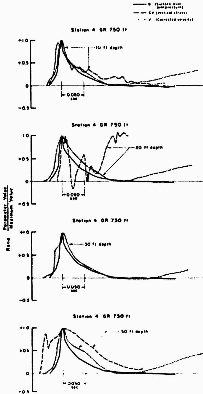
Figure 4.13 Overpressure, particle velocity, earth stress, normalized to maximum value, Station 4, Shot Priscilla.
