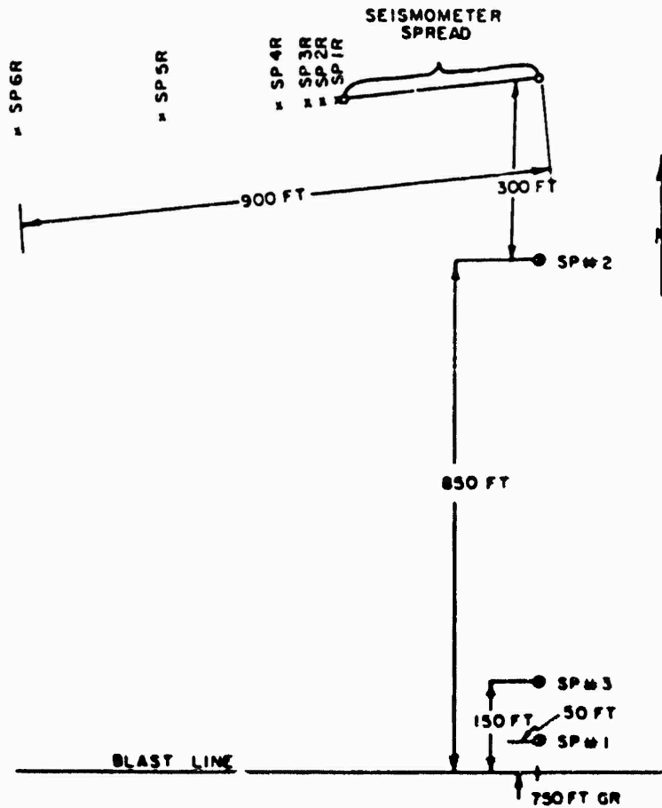
Figure 2.6 Seismic locations.
