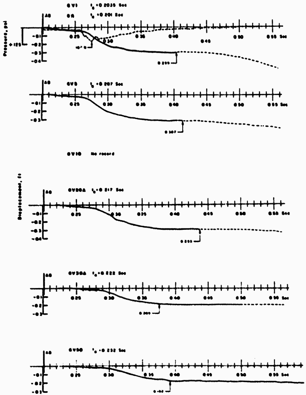
Figure 3.16 Vertical displacement versus time, Station 6 (GIT: 1,050 feet), Shot Priscilla.
