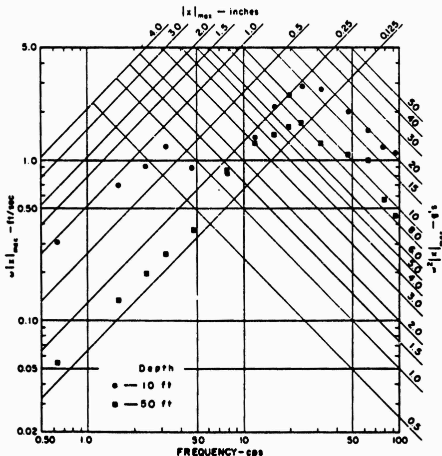
Figure 4.41a Horizontal velocity spectra, 275 psi, Shot Priscilla.
