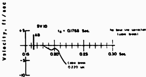
Figure 3.11 Horizontal velocity versus time, Station 4 (GR: 750 feet); vertical velocity versus time, Station 5 (GR: 95v feet); Shot Priscilla.
