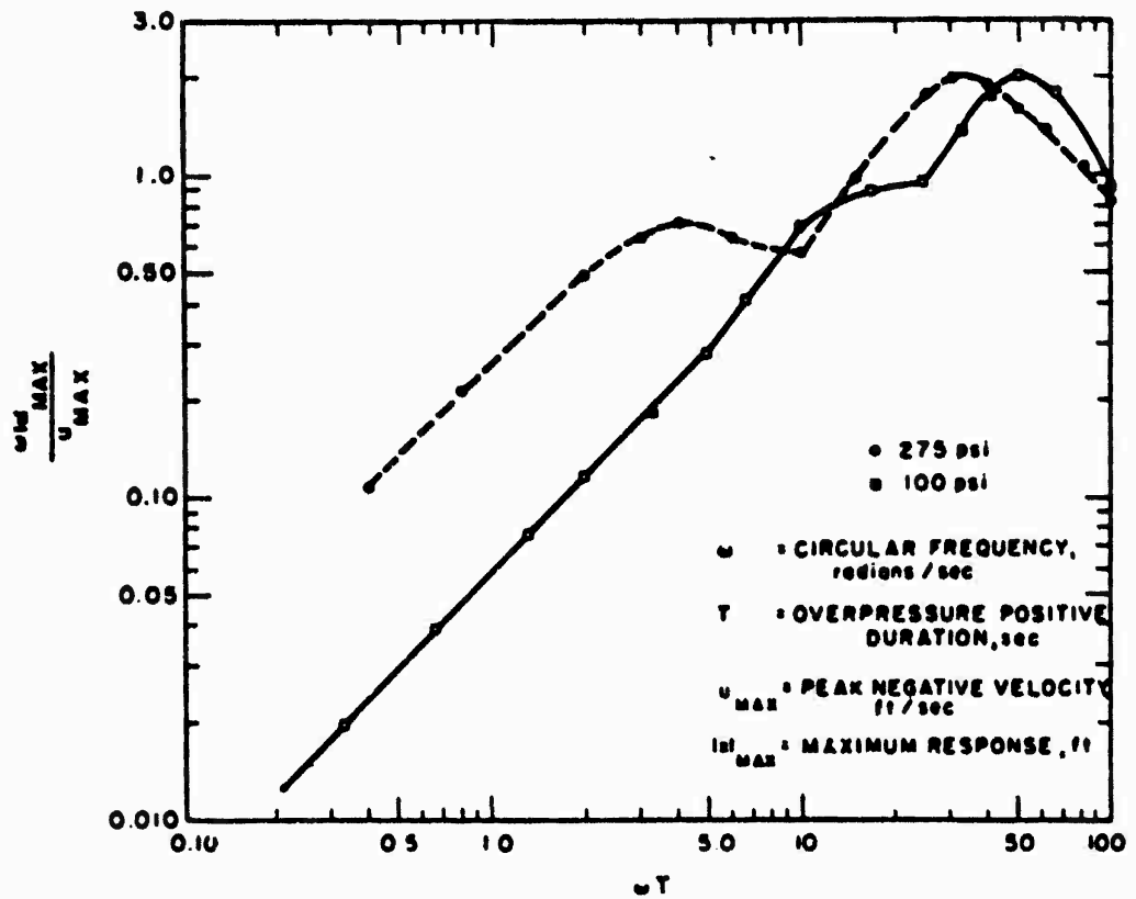
Figure 4.46 Normalized horizontal velocity spectra, Priscilla 10-foot depth, 0.5 percent critical damping.
