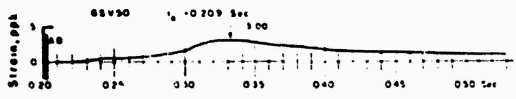
Figure 3.24 Vertical strain versus time, Station 4 (GR: 750 feet); Station 6 (GR: 1,050 feet); Shot Priscilla.
