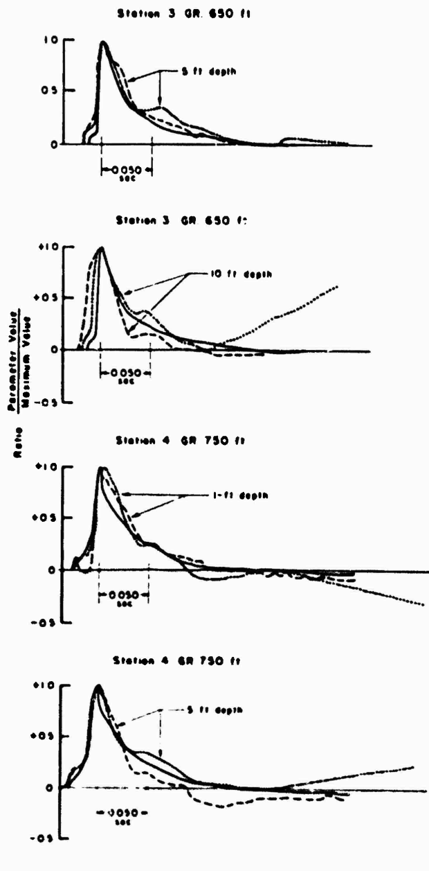
Figure 4.12 Overpressure, particle velocity, earth stress, normalized to maximum value, Stations 3 and 4, Shot Priscilla.
