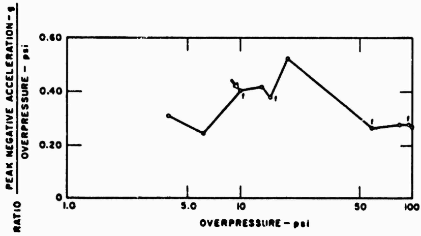
Figure 4.23 Vertical acceleration, Jangle HE-4, 5-foot depth (✓ indicates interpolated overpressure data).
