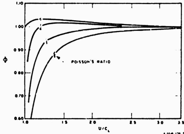
Figure 1.5 \phi versus U/C_L and Poisson's ratio.
