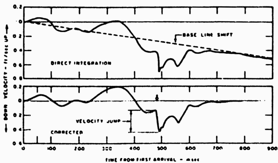
Figure C.2 Uncorrected and corrected vertical velocities.
