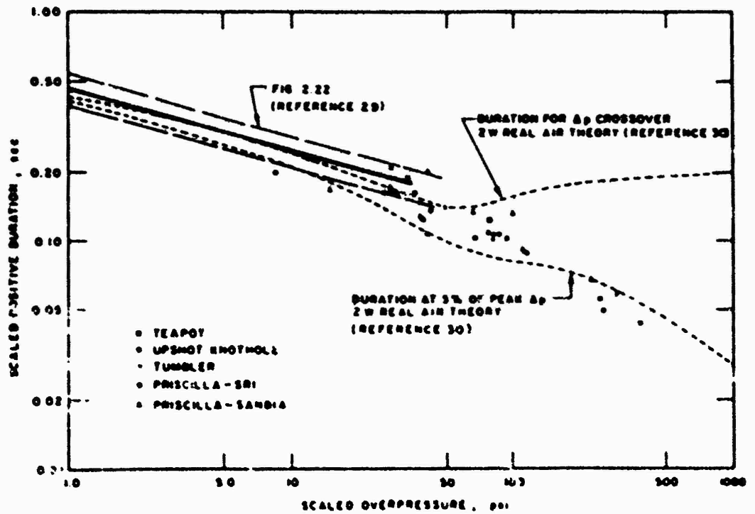
Figure D.2 Positive overpressure duration versus peak overpressure.
