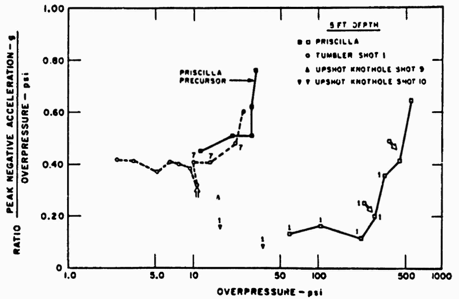
Figure 4.19 Vertical acceleration, Frenchman Flat, 5-foot depth (numbers indicate overpressure wave form).
