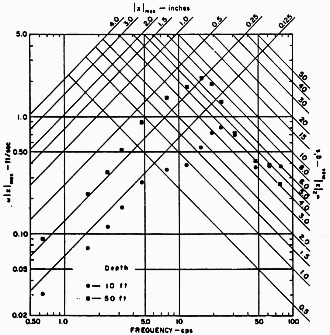
Figure 4.41b Horizontal velocity spectra, 100 psi, Slot Priscilla.
