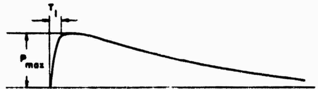
AIR BLAST WAVE FORM, GENERALIZED
