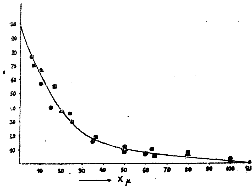
Fig. 1. Relative activity A/A_0 in dependence upon the thickness of the ground substance layer. \blacktriangle \blacksquare - sulfur compounds 30 minutes; \bullet - sulfur compounds 120 minutes.
