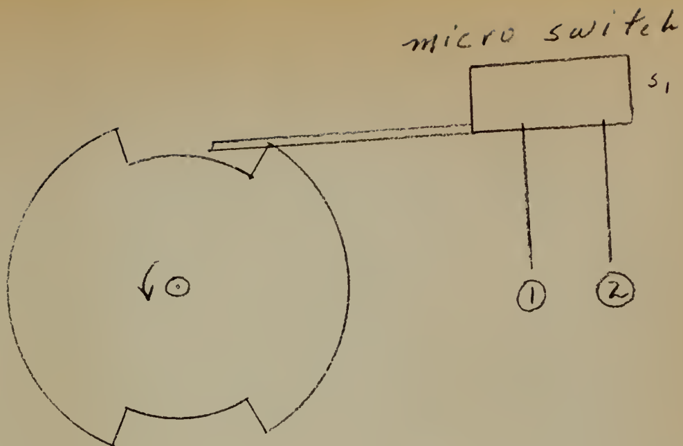
Figure 14. Timing wheel.
