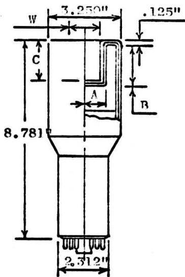
PHOTOMULTIPLIER TUBE with NaI(Tl) CRYSTAL [3]
