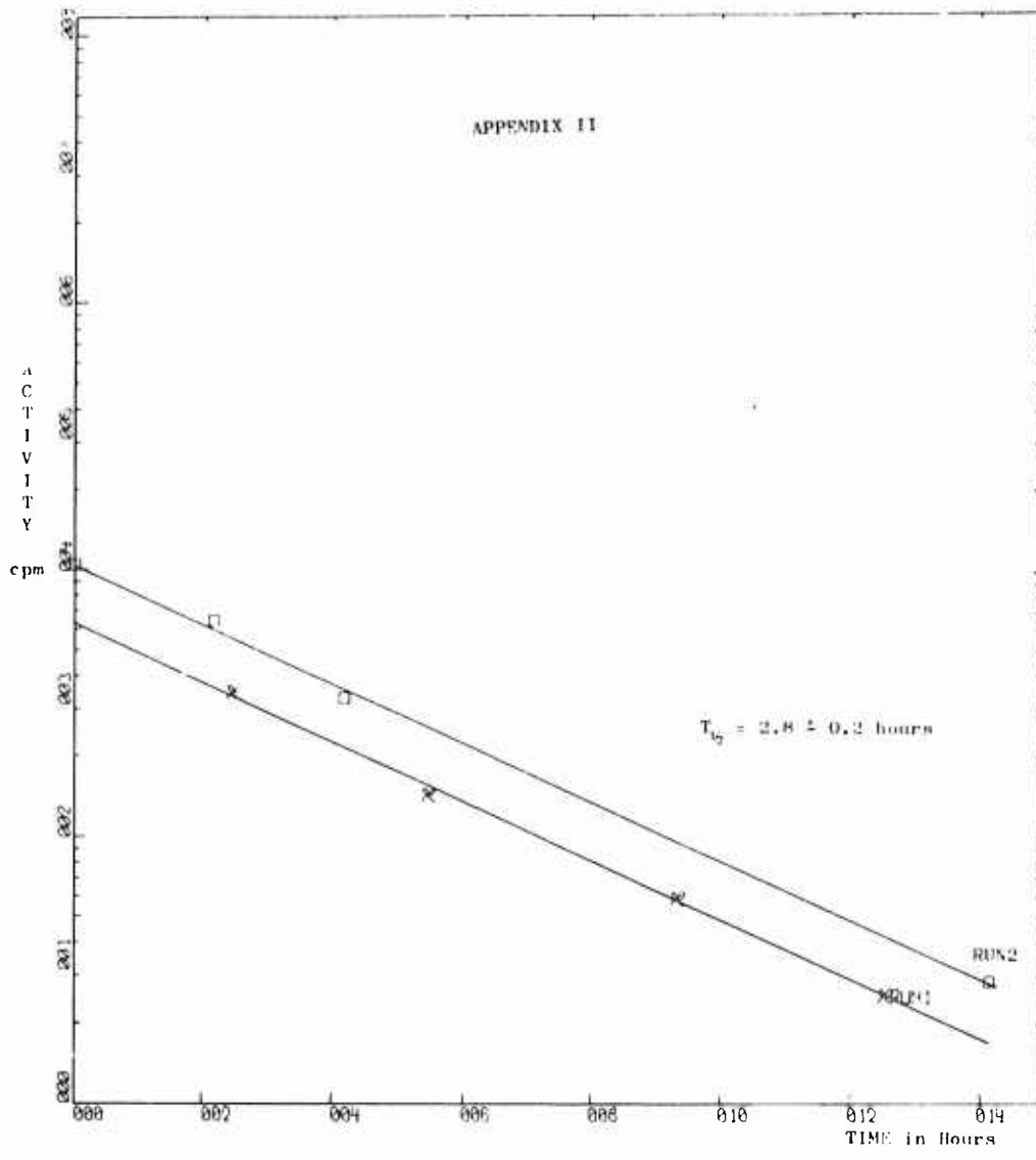
X-SCALE - 2 hours/inch Y-SCALE - 1 decade/2 inches DECAY OF PHOTOPEAK FROM UNIDENTIFIED SOURCES 1.4 MEV GAMMAS
