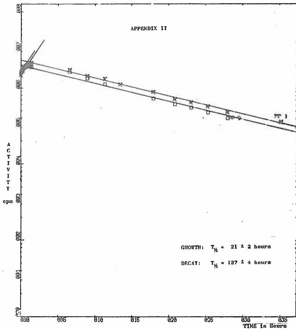
K-SCALE - 50 hours/inch Y-SCALE -1 decade/2 inches DECAY OF PHOTOPEAKS ONE AND TWO 0.030-0.081MEV GAMMAS FROM XE 133
