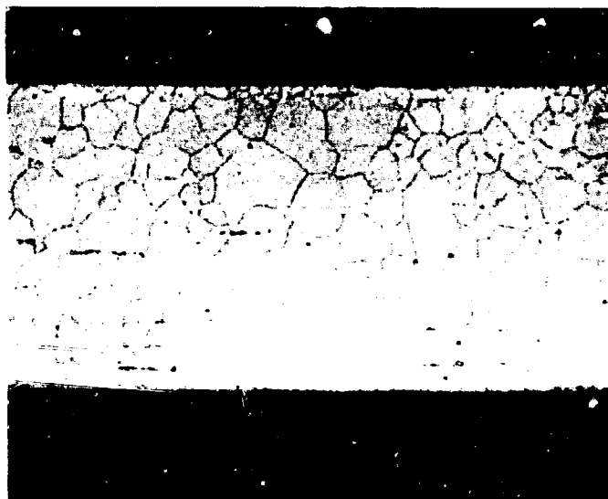
Inconel 600 - 150 x
