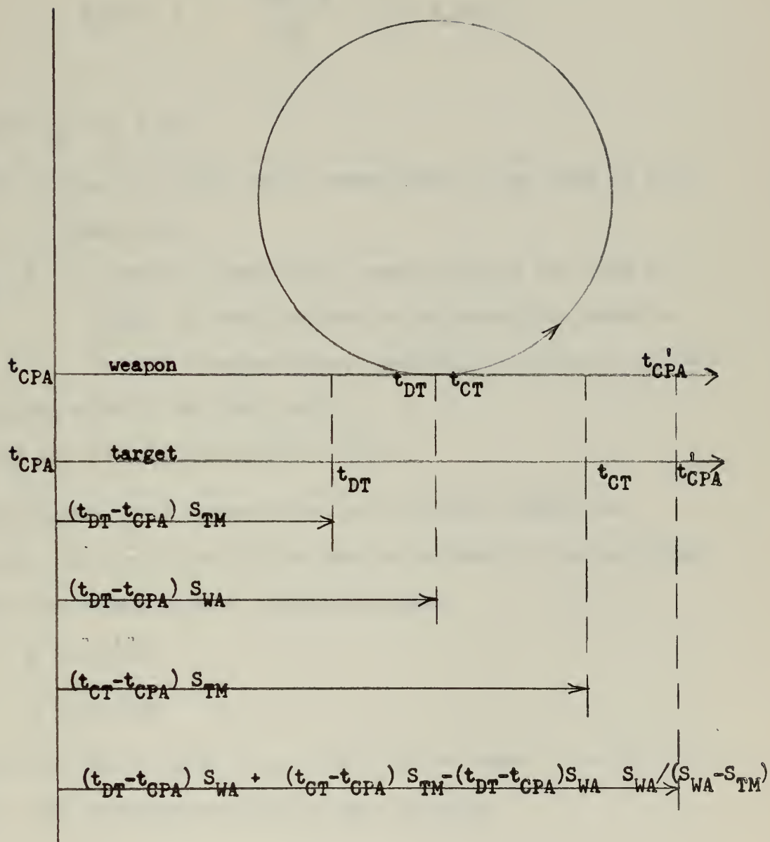
Figure 19: Geographic plot of weapon and target tracks separated to show time differences. The distances below the target track are measured from the joint position at time t_{CPA} .
