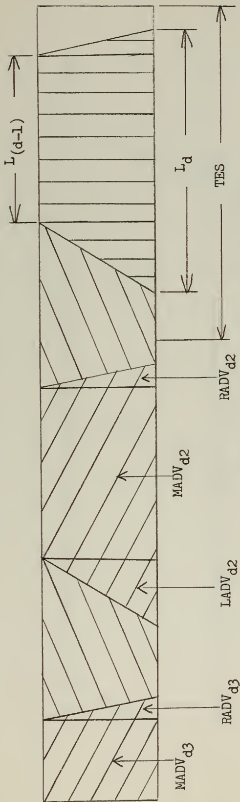
Figure 11: Cross-section of sample level L_d above critical depth CDA. Area actually scanned is lined vertically. Equivalent areas scanned have lines sloping down to the right. Areas of target escape have lines sloping down to the left.
