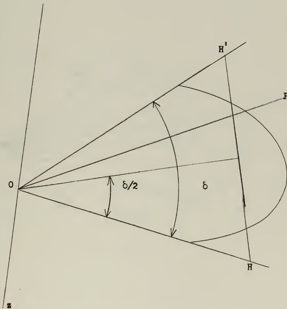
Figure 7: Equivalence of area A_j and isosceles triangle OHH' of altitude H_j and apex angle \delta .
