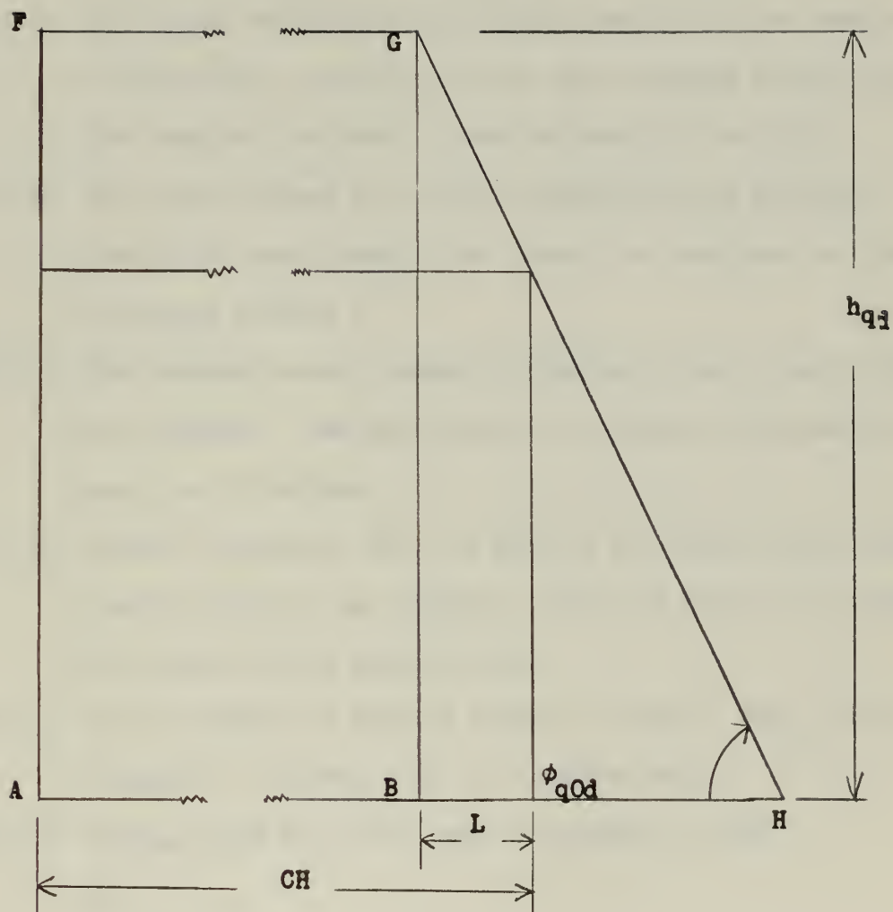
Figure 25: Computation of modified volume RqDV_{du} . Length FG is B_{qO(d-1)} - (u - 1) \text{ TES} . Area BGH represents the original volume RqDV_{du} . Line AF is part of the vertical through the weapon.
