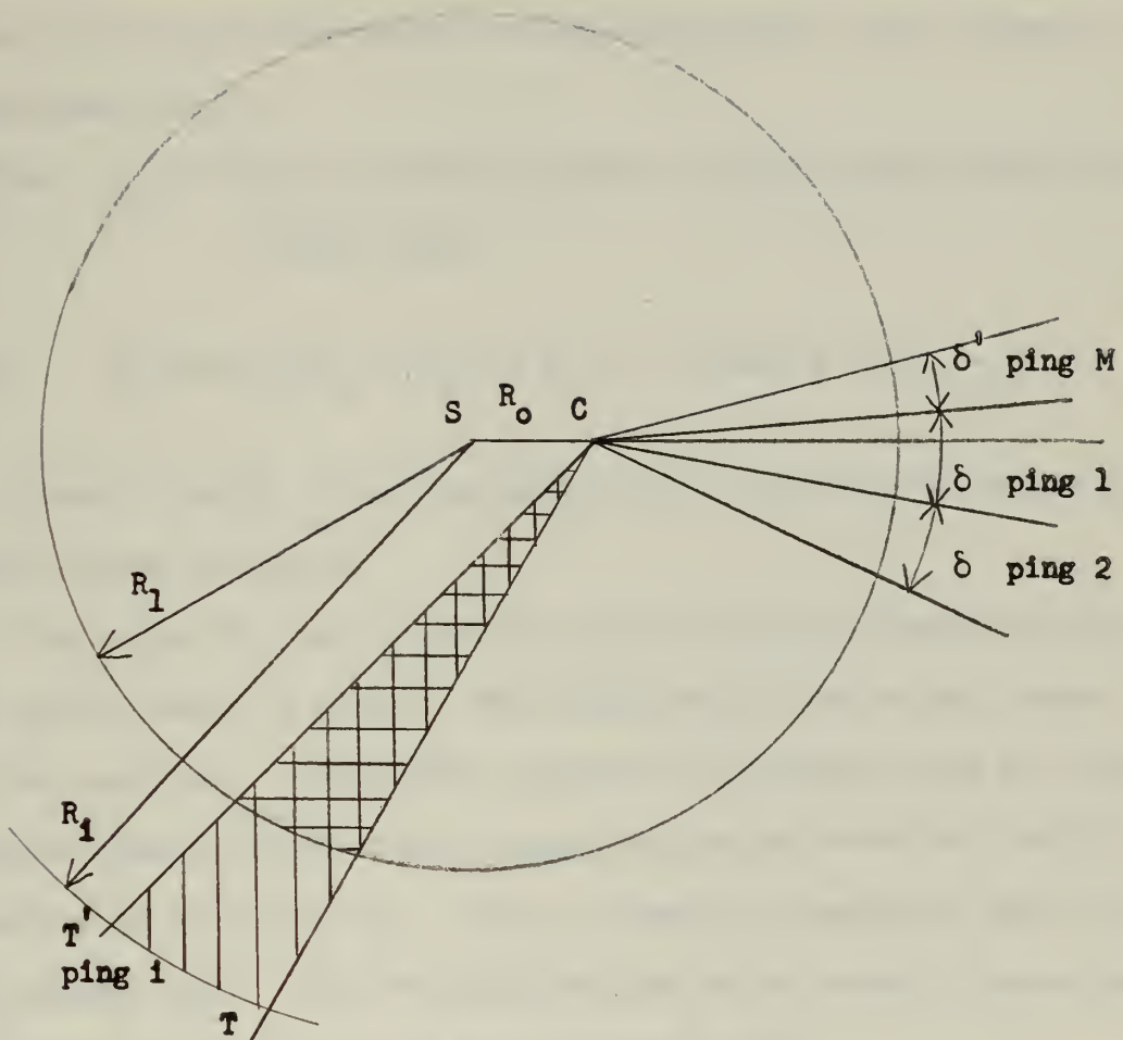
Figure 16: Top view of target cylinder of increasing volume .
