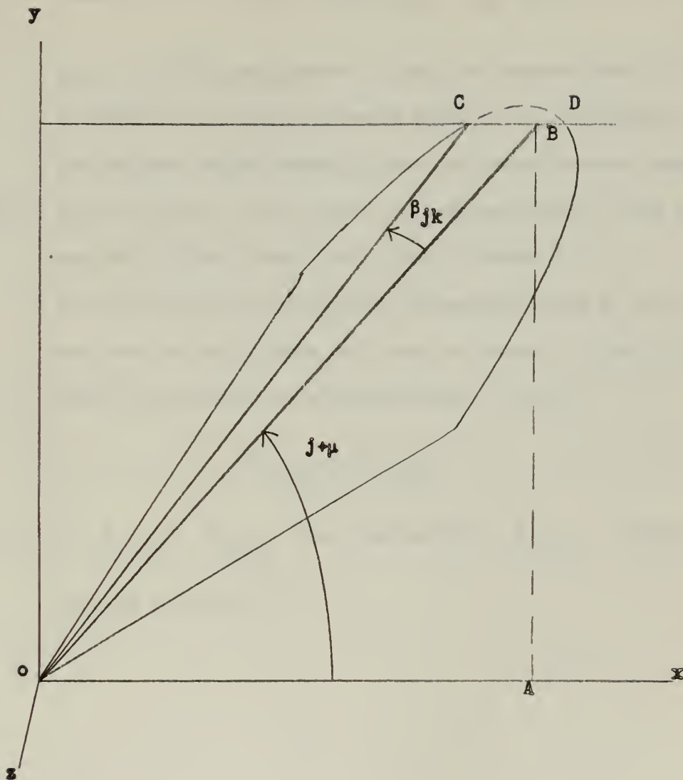
Figure 20. Computation of radial length for angle \beta_{jk} .
