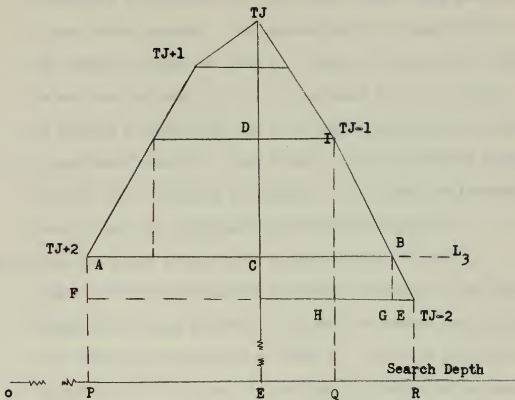
Figure 21: A sample volume portion for computation of L_d . The points (TJ^{\pm d}) are the radial endpoints of the corresponding planes. The level L_3 is under consideration and distance (AB = L_3) is to be computed. The following are equivalent:
