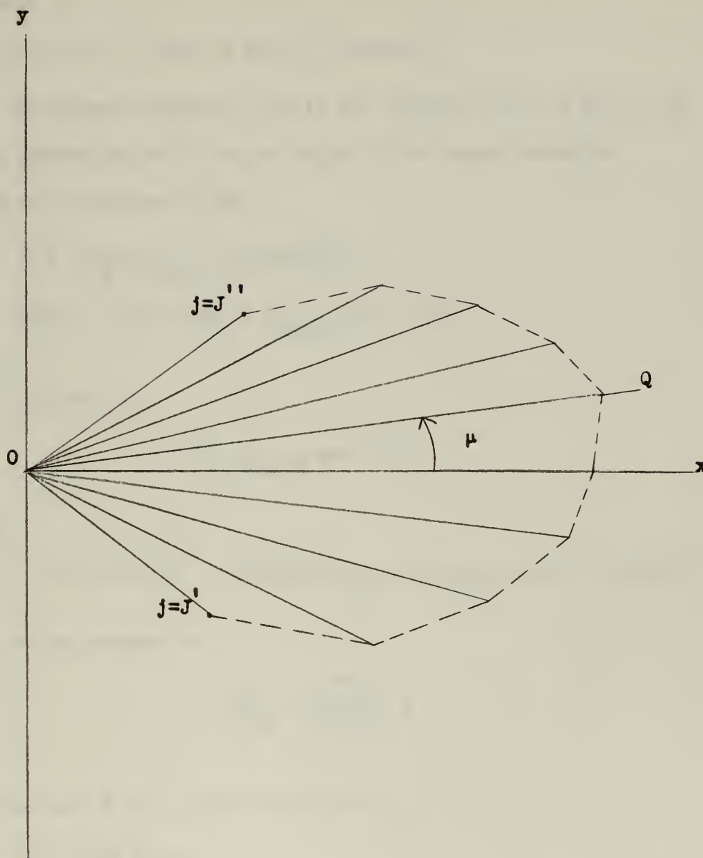
Figure 8: Vertical cross-section of insonified volume on ping zero. x is the horizontal axis, y is the vertical axis, and OQ is the transducer axis extension.
