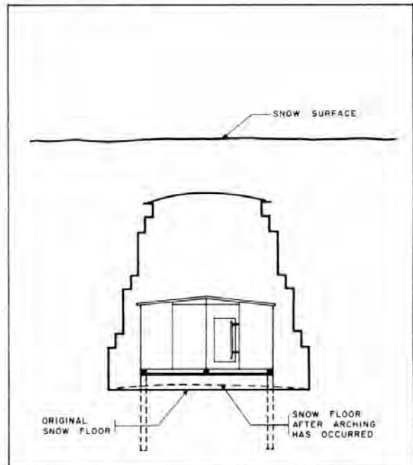
Figure 16. Piles spaced symmetrically with respect to floor centerline.
